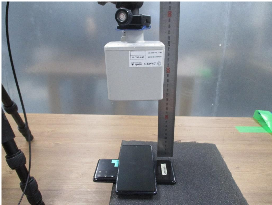
Top charger above client (20cm distance)
