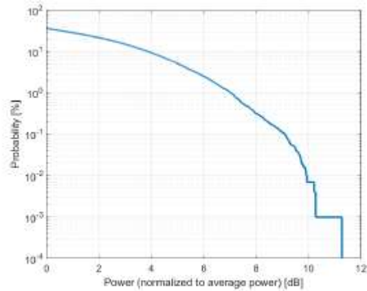
Complementary Cumulative Distribution Function (CCDF)
