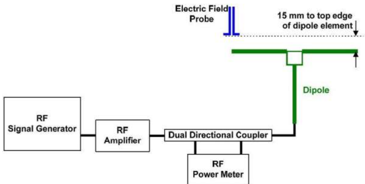
Setup diagram
