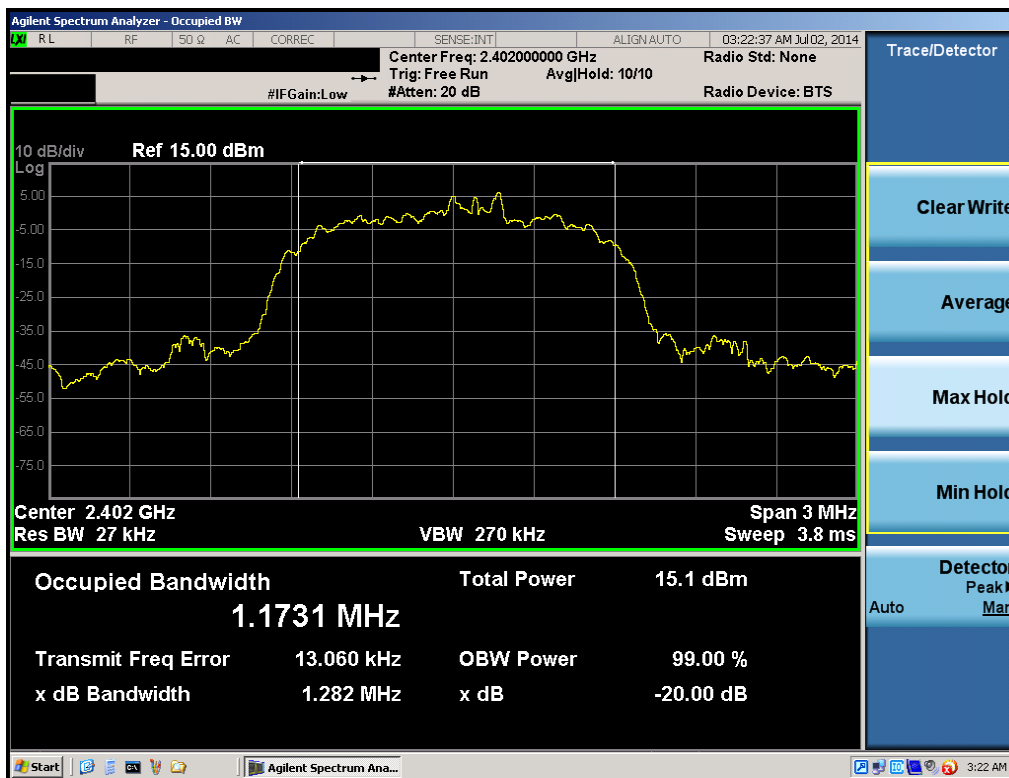
Plot 6-7. 20dB Bandwidth Plot (Bluetooth, 3Mbps – Ch. 0)
