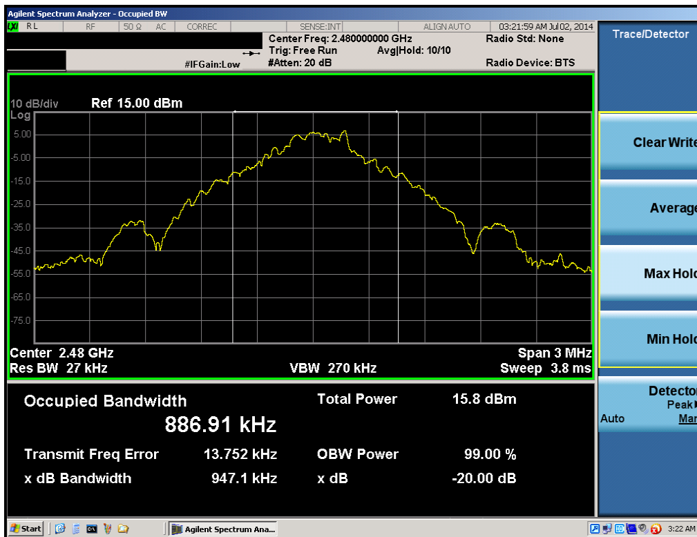
Plot 6-3. 20dB Bandwidth Plot (Bluetooth, 1Mbps – Ch. 78)
