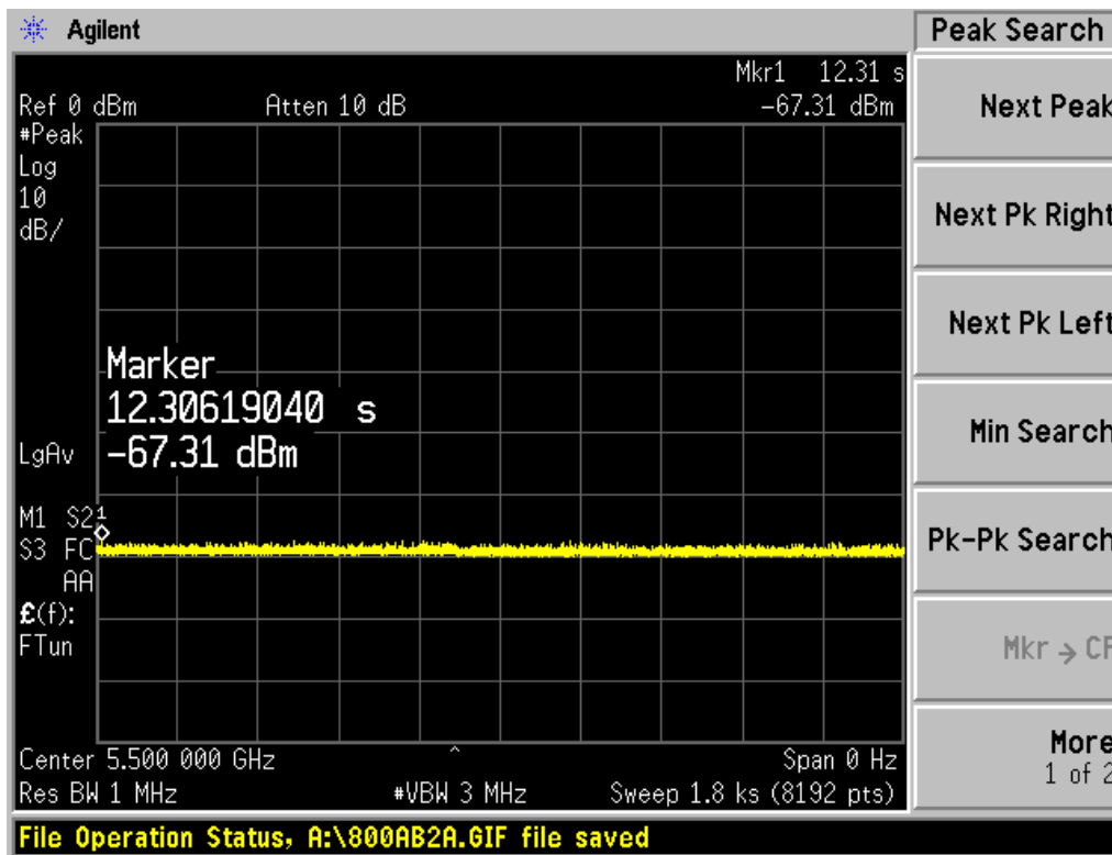
Figure 5-4. Band 2C Non-occupancy Period - Monitoring live spectrum - Elapse time 30 minutes
