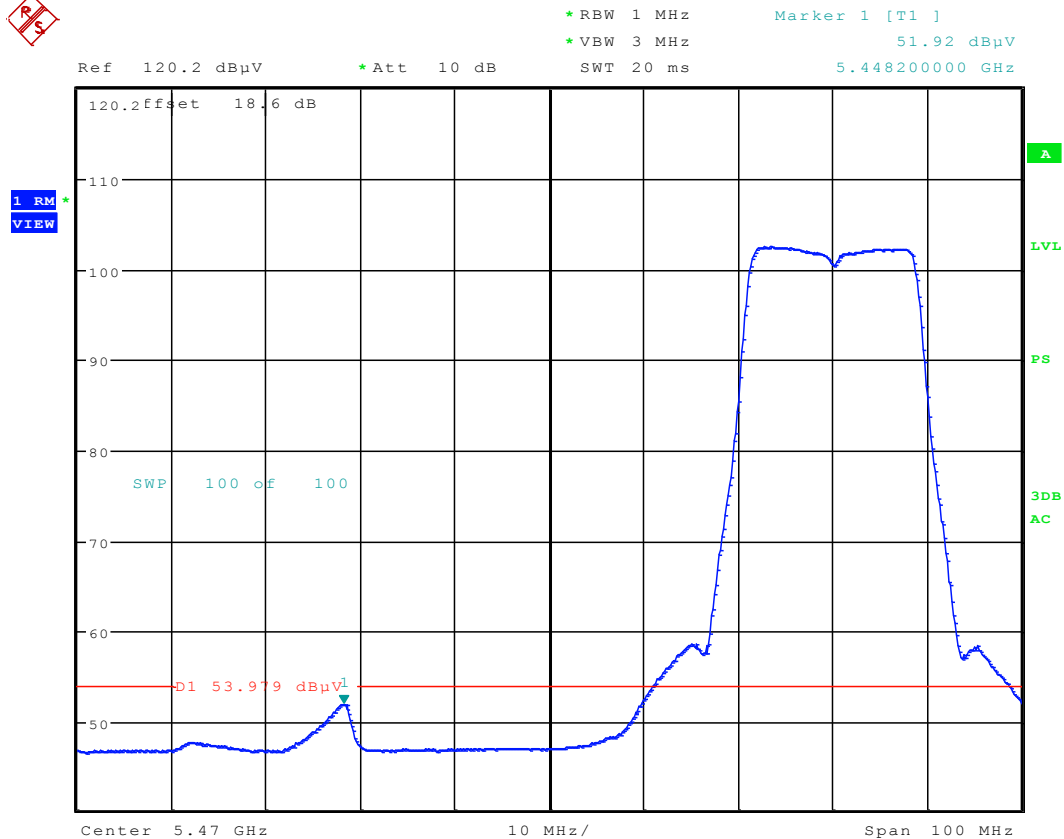
Plot 6-63. Radiated Restricted Lower Band Edge Plot (Average – UNII Band 2C)
