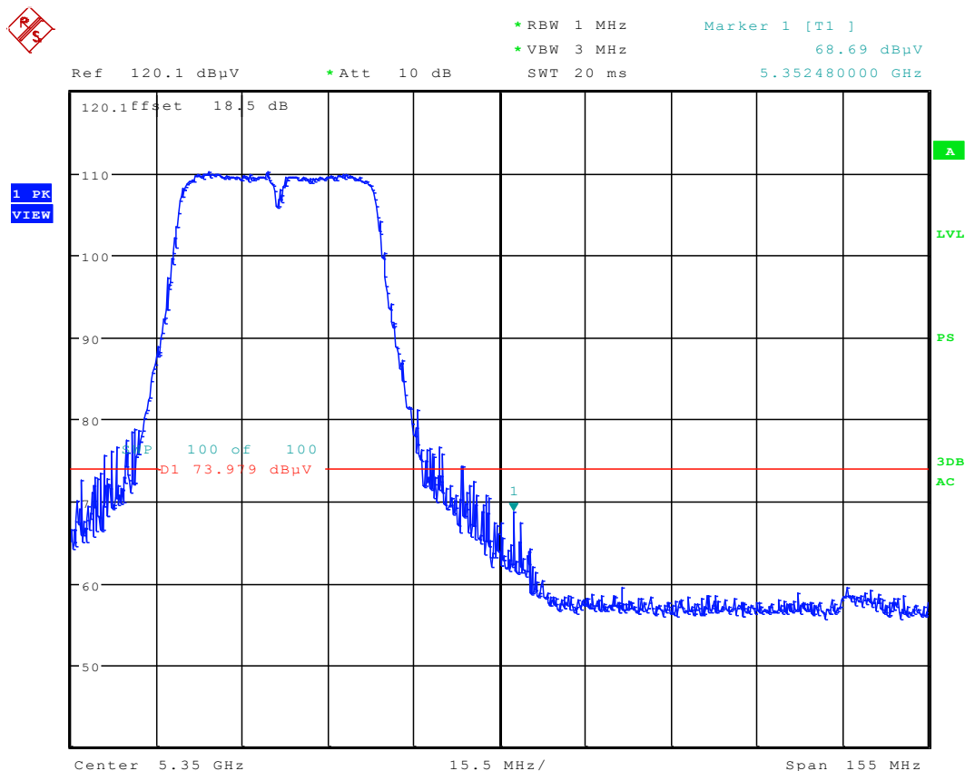
Plot 6-69. Radiated Restricted Upper Band Edge Plot (Peak – UNII Band 2A)
