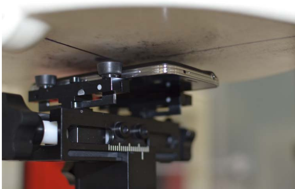
SAR Test Setup Photo 5 – Back Side at 10 mm
