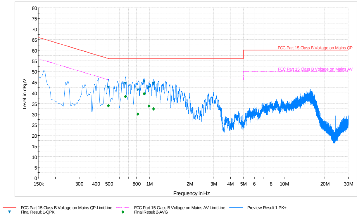
Plot 7-2. Line Conducted Plot (LN)
