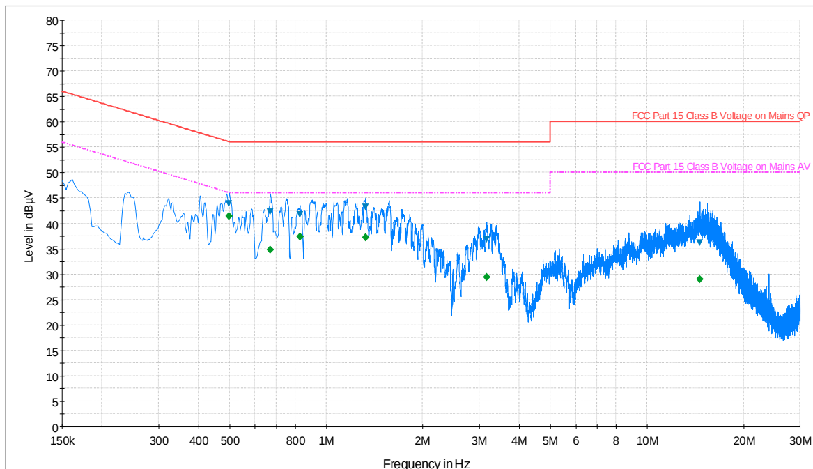
Plot 7-1. Line Conducted Plot (L1)
