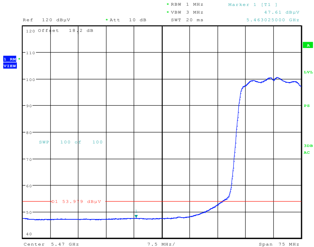
Plot 6-61. Radiated Restricted Lower Band Edge Plot (Average – UNII Band 2C)
