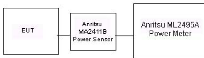
Figure 6-2. Test Instrument & Measurement Setup
