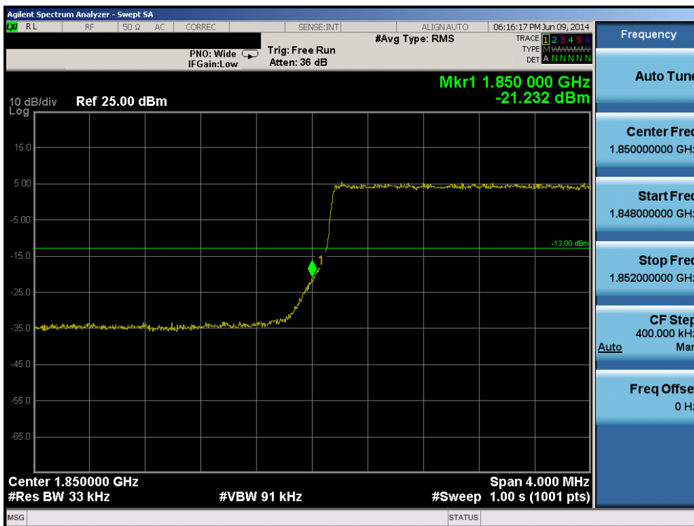
Plot 6-193. Lower Band Edge Plot (Band 2 – 3.0MHz QPSK – RB Size 15)
