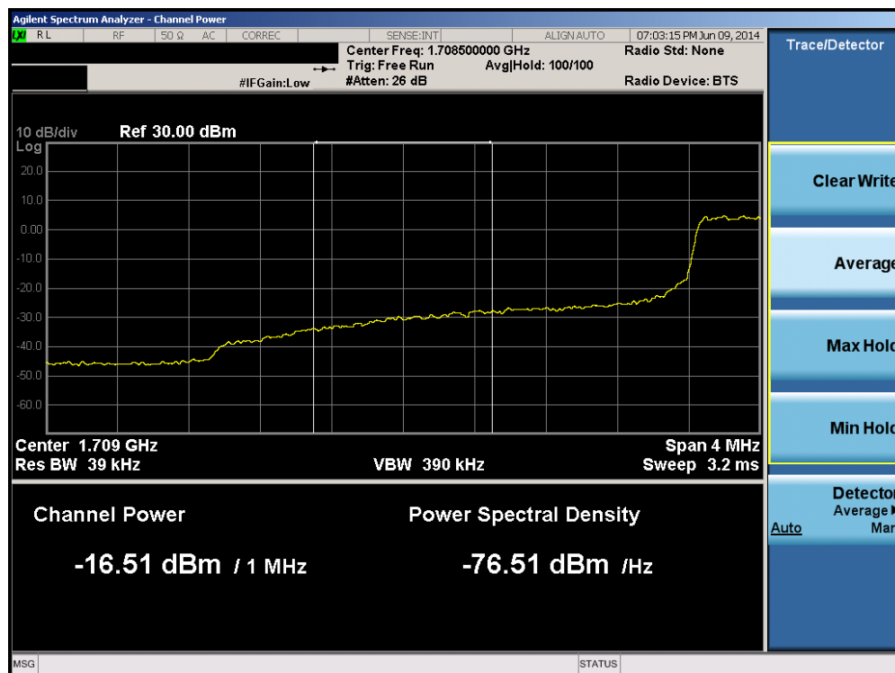
Plot 6-170. Lower Extended Band Edge Plot (Band 4 – 3.0MHz QPSK – RB Size 15)
