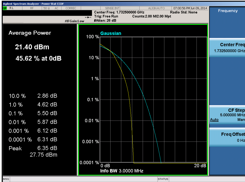
Plot 6-216. PAR Plot (Band 4 – 3.0MHz 16-QAM – RB Size 15)
