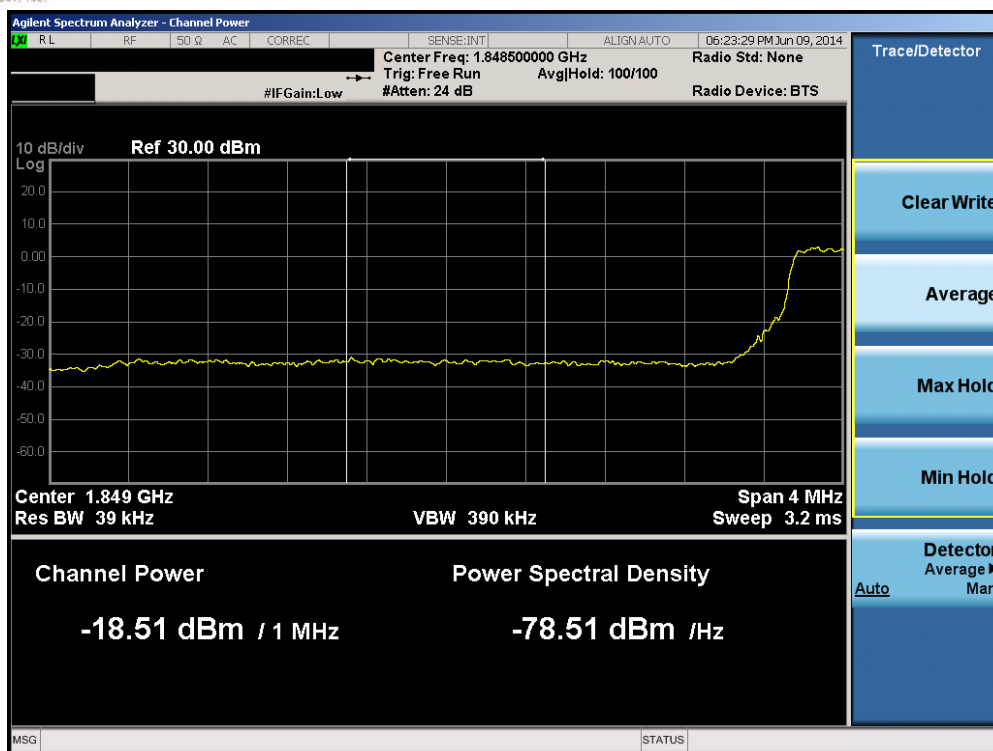
Plot 6-198. Lower Extended Band Edge Plot (Band 2 – 5.0MHz QPSK – RB Size 25)
