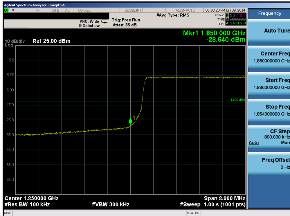
Plot 6-201. Lower Band Edge Plot (Band 2 – 10.0MHz QPSK – RB Size 50)
