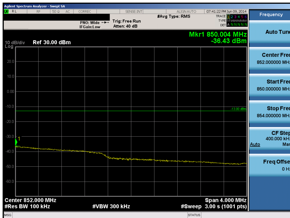
Plot 6-158. Upper Extended Band Edge Plot (Band 5 – Band 5 – 3.0MHz QPSK – RB Size 15)
