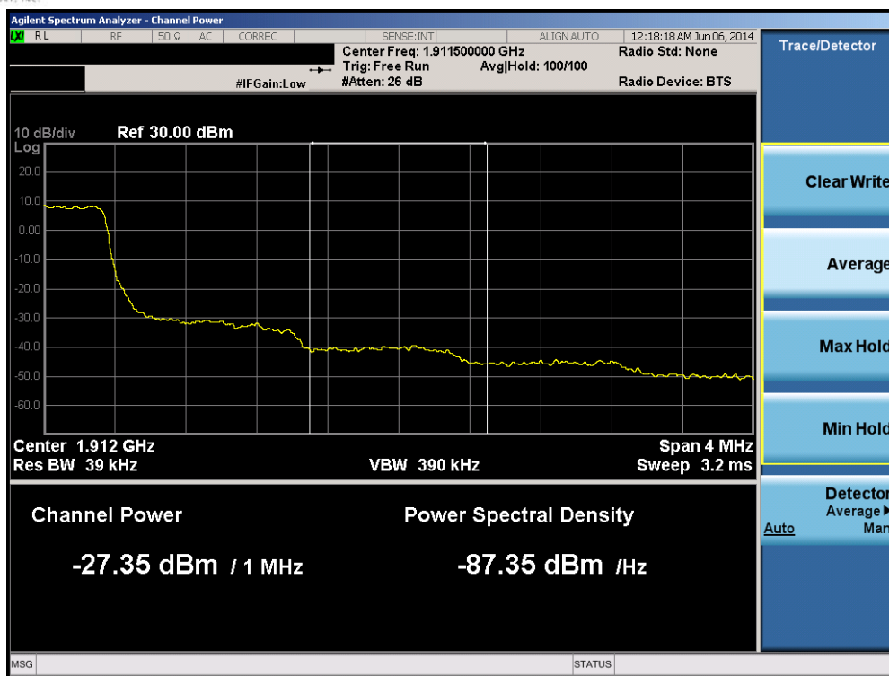
Plot 6-192. Upper Extended Band Edge Plot (Band 2 – 1.4MHz QPSK – RB Size 6)
