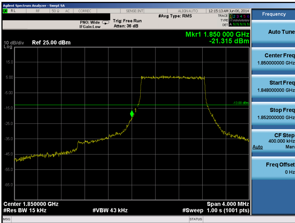
Plot 6-189. Lower Band Edge Plot (Band 2 – 1.4MHz QPSK – RB Size 6)
