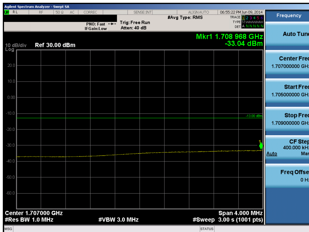
Plot 6-166. Lower Extended Band Edge Plot (Band 4 – 1.4MHz QPSK – RB Size 6)
