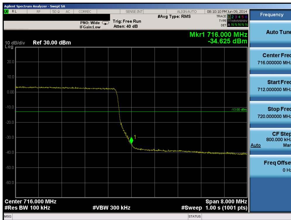
Plot 6-150. Upper Band Edge Plot (Band 17 – 10.0MHz QPSK – RB Size 50)
