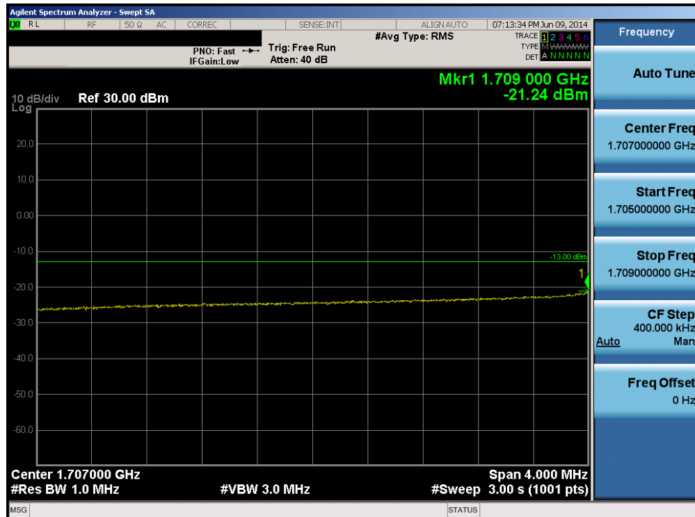
Plot 6-178. Lower Extended Band Edge Plot (Band 4 – 10.0MHz QPSK – RB Size 50)
