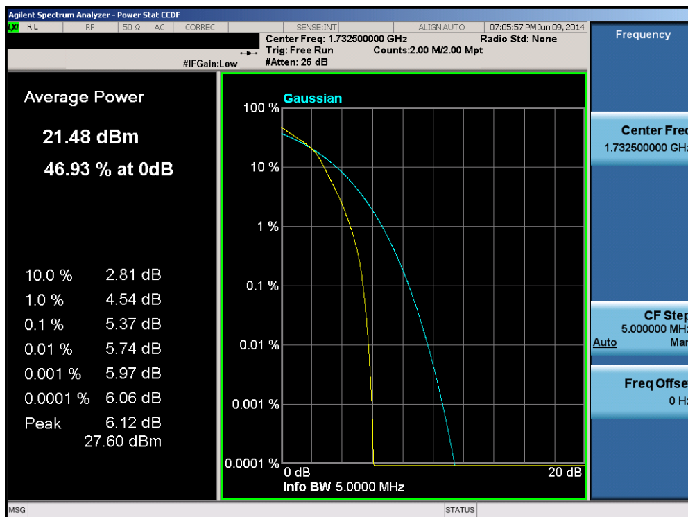
Plot 6-218. PAR Plot (Band 4 – 5.0MHz 16-QAM – RB Size 25)
