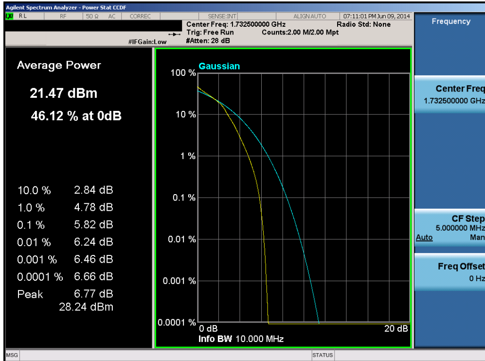
Plot 6-220. PAR Plot (Band 4 – 10.0MHz 16-QAM – RB Size 50)
