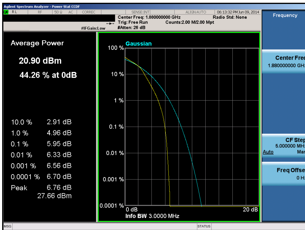
Plot 6-228. PAR Plot (Band 2 – 3.0MHz 16-QAM – RB Size 15)
