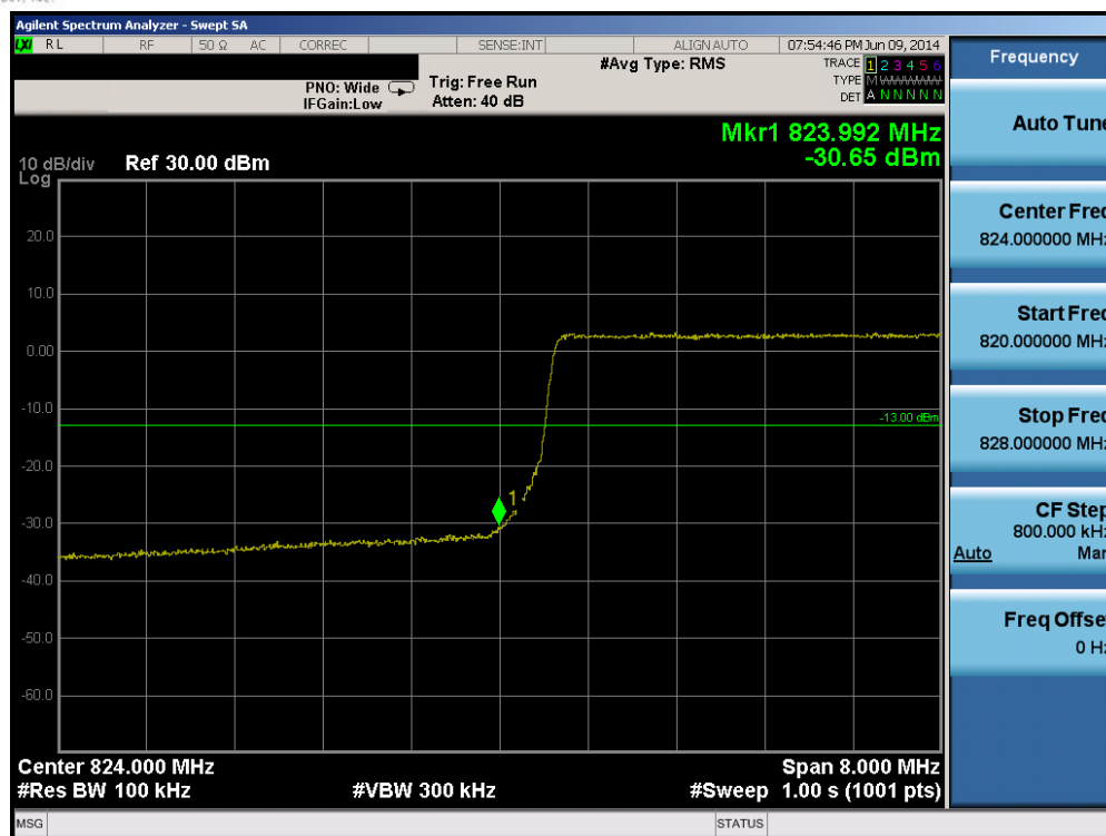
Plot 6-163. Lower Band Edge Plot (Band 5 – 10.0MHz QPSK – RB Size 50)
