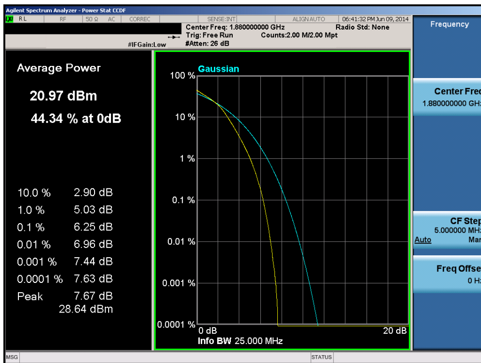
Plot 6-236. PAR Plot (Band 2 – 20.0MHz 16-QAM – RB Size 100)
