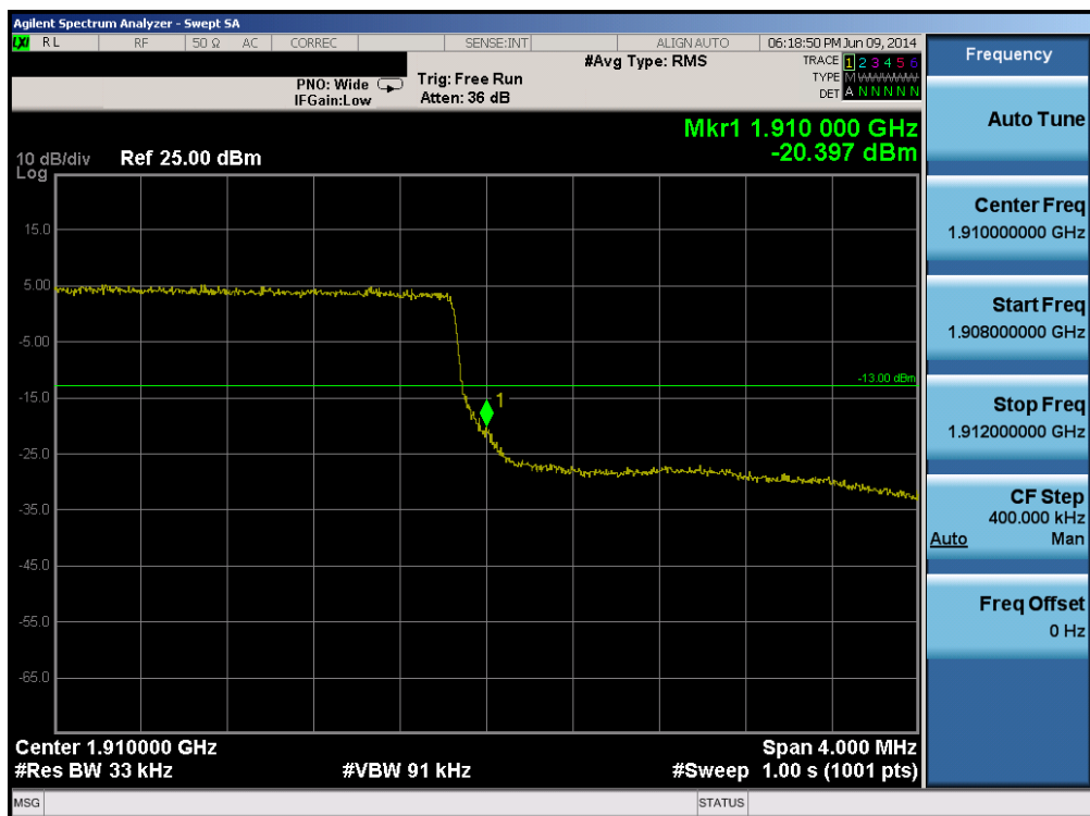
Plot 6-195. Upper Band Edge Plot (Band 2 – 3.0MHz QPSK – RB Size 15)
