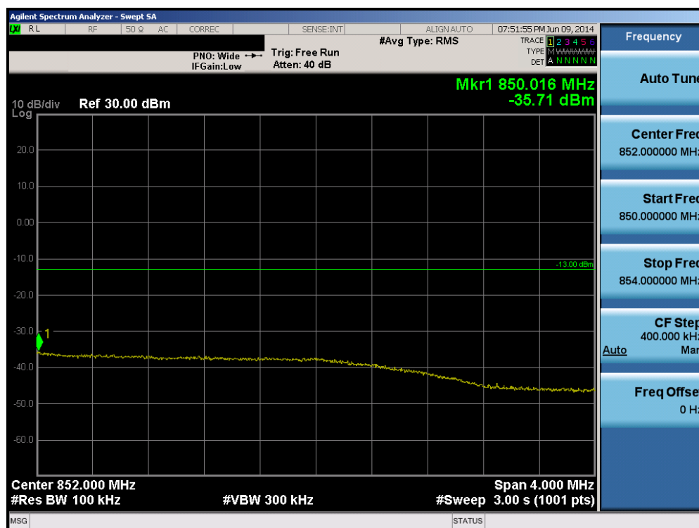
Plot 6-162. Upper Extended Band Edge Plot (Band 5 – 5.0MHz QPSK – RB Size 25)
