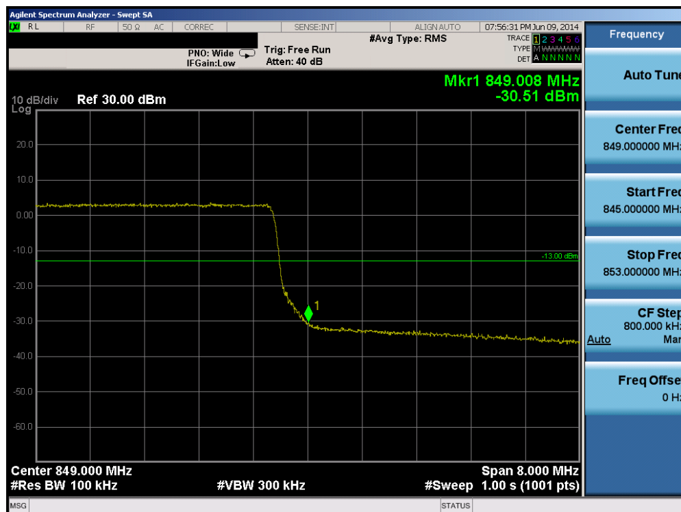
Plot 6-164. Upper Band Edge Plot (Band 5 – 10.0MHz QPSK – RB Size 50)
