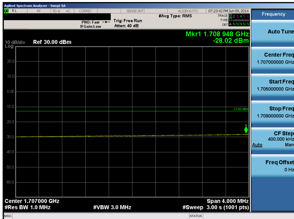
Plot 6-186. Lower Extended Band Edge Plot (Band 4 – 20.0MHz QPSK – RB Size 100)
