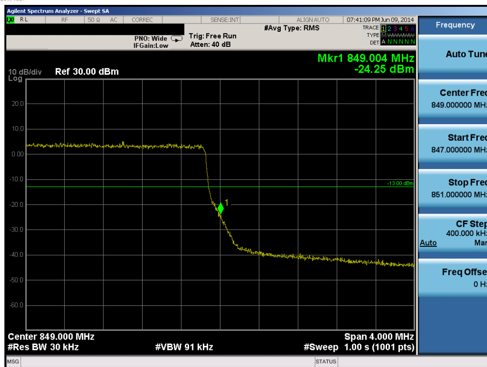
Plot 6-157. Upper Band Edge Plot (Band 5 – 3.0MHz QPSK – RB Size 15)
