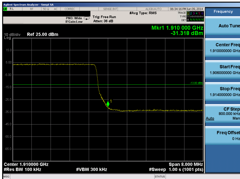
Plot 6-203. Upper Band Edge Plot (Band 2 – 10.0MHz QPSK – RB Size 50)
