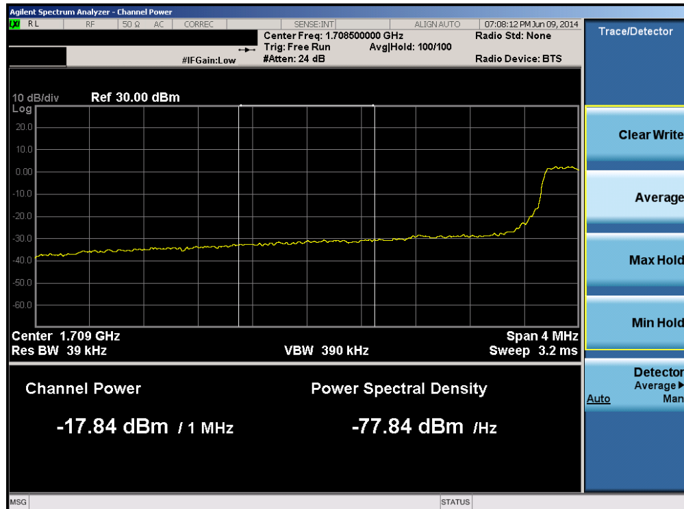
Plot 6-174. Lower Extended Band Edge Plot (Band 4 – 5.0MHz QPSK – RB Size 25)
