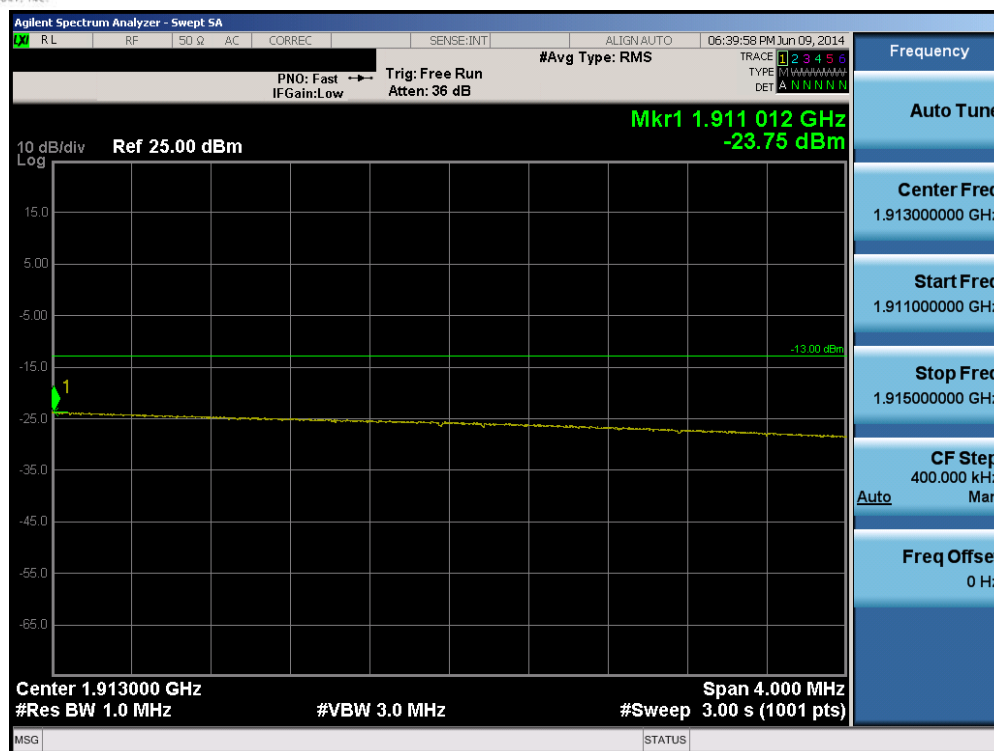
Plot 6-208. Upper Extended Band Edge Plot (Band 2 – 15.0MHz QPSK – RB Size 75)
