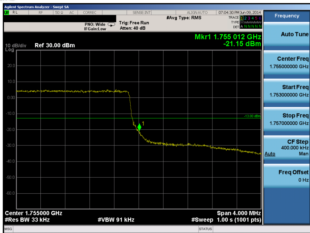
Plot 6-171. Upper Band Edge Plot (Band 4 – 3.0MHz QPSK – RB Size 15)
