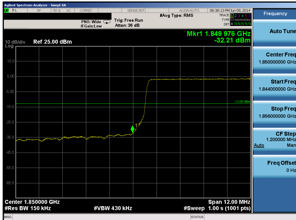
Plot 6-205. Lower Band Edge Plot (Band 2 – 15.0MHz QPSK – RB Size 75)
