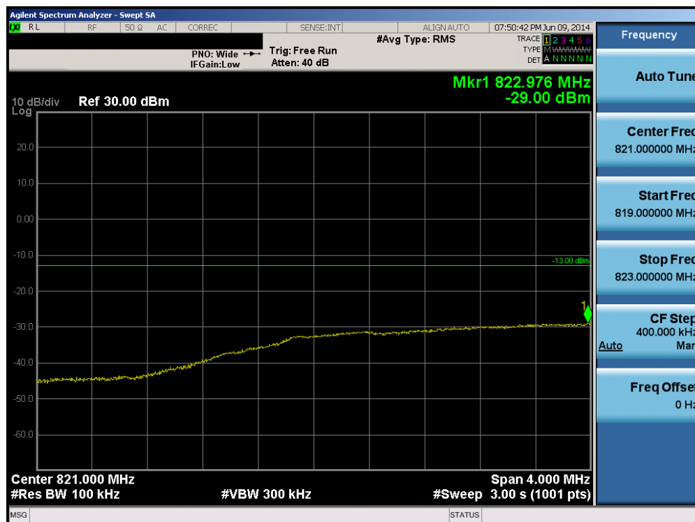
Plot 6-160. Lower Extended Band Edge Plot (Band 5 – 5.0MHz QPSK – RB Size 25)
