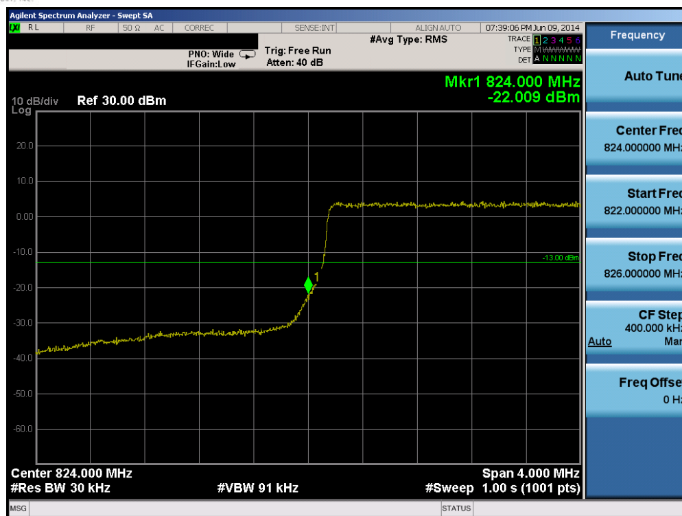
Plot 6-155. Lower Band Edge Plot (Band 5 – 3.0MHz QPSK – RB Size 15)
