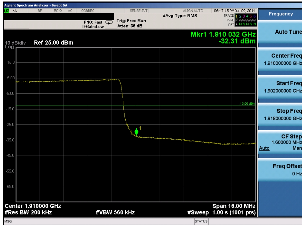
Plot 6-211. Upper Band Edge Plot (Band 2 – 20.0MHz QPSK – RB Size 100)
