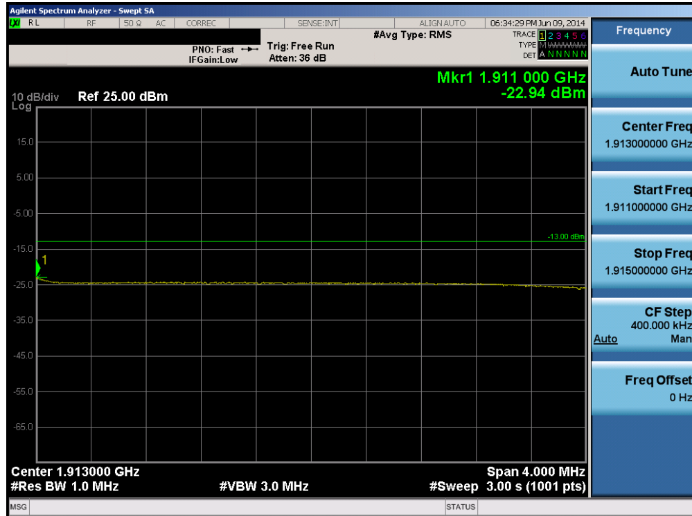
Plot 6-204. Upper Extended Band Edge Plot (Band 2 – 10.0MHz QPSK – RB Size 50)
