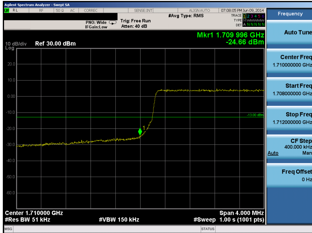
Plot 6-173. Lower Band Edge Plot (Band 4 – 5.0MHz QPSK – RB Size 25)
