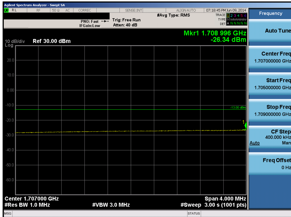
Plot 6-182. Lower Extended Band Edge Plot (Band 4 – 15.0MHz QPSK – RB Size 75)
