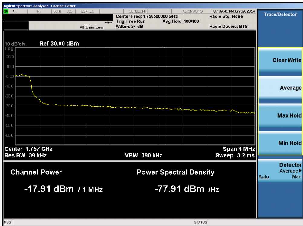
Plot 6-176. Upper Extended Band Edge Plot (Band 4 – 5.0MHz QPSK – RB Size 25)
