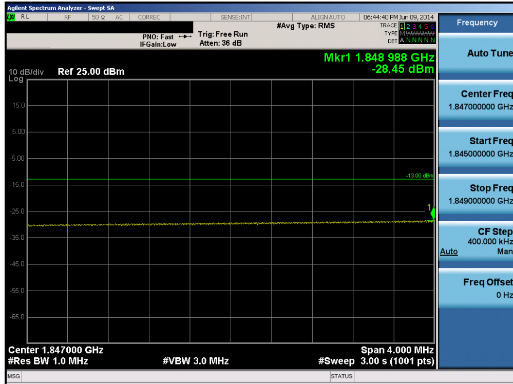
Plot 6-210. Lower Extended Band Edge Plot (Band 2 – 20.0MHz QPSK – RB Size 100)
