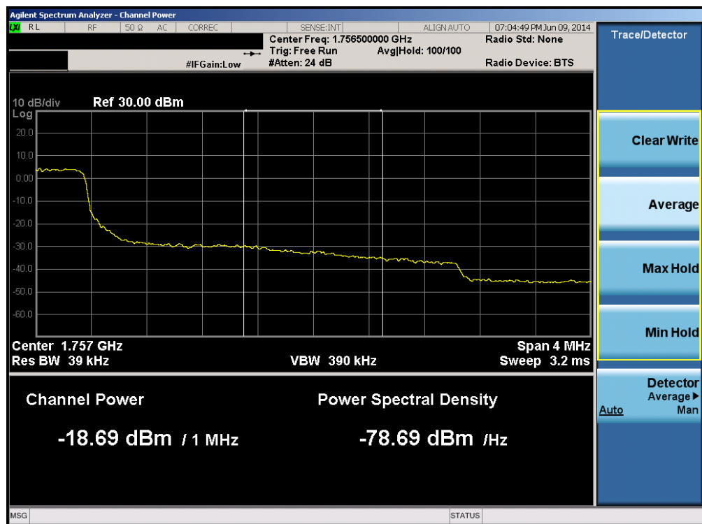
Plot 6-172. Upper Extended Band Edge Plot (Band 4 – 3.0MHz QPSK – RB Size 15)
