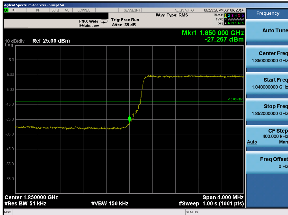
Plot 6-197. Lower Band Edge Plot (Band 2 – 5.0MHz QPSK – RB Size 25)
