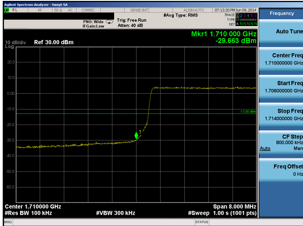
Plot 6-177. Lower Band Edge Plot (Band 4 – 10.0MHz QPSK – RB Size 50)
