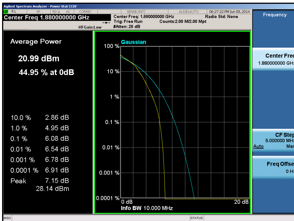
Plot 6-232. PAR Plot (Band 2 – 10.0MHz 16-QAM – RB Size 50)
