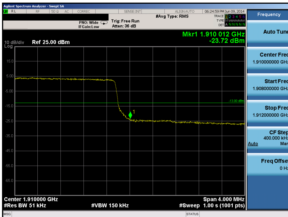
Plot 6-199. Upper Band Edge Plot (Band 2 – 5.0MHz QPSK – RB Size 25)
