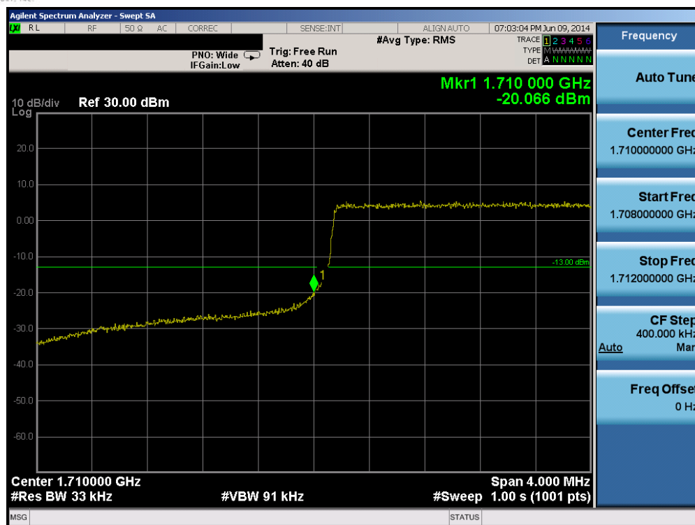
Plot 6-169. Lower Band Edge Plot (Band 4 – 3.0MHz QPSK – RB Size 15)
