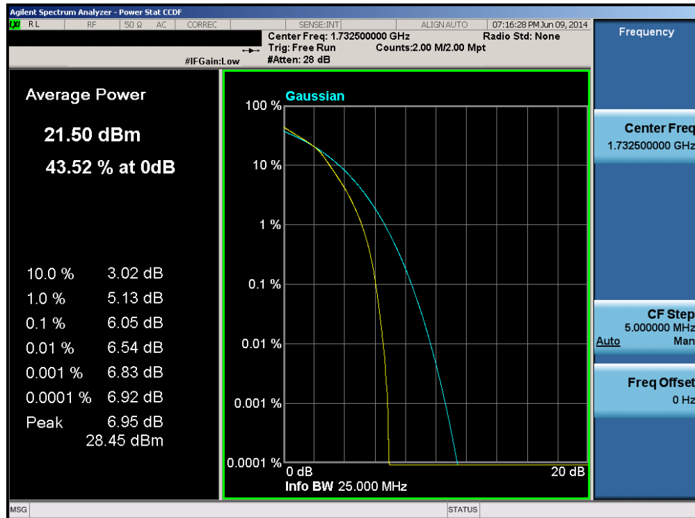
Plot 6-222. PAR Plot (Band 4 – 15.0MHz 16-QAM – RB Size 75)
