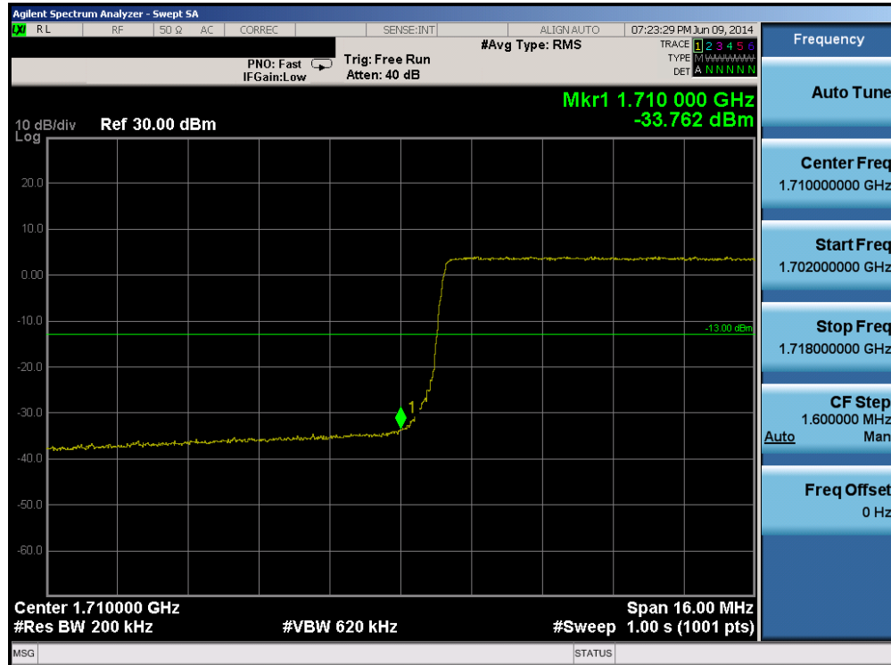
Plot 6-185. Lower Band Edge Plot (Band 4 – 20.0MHz QPSK – RB Size 100)
