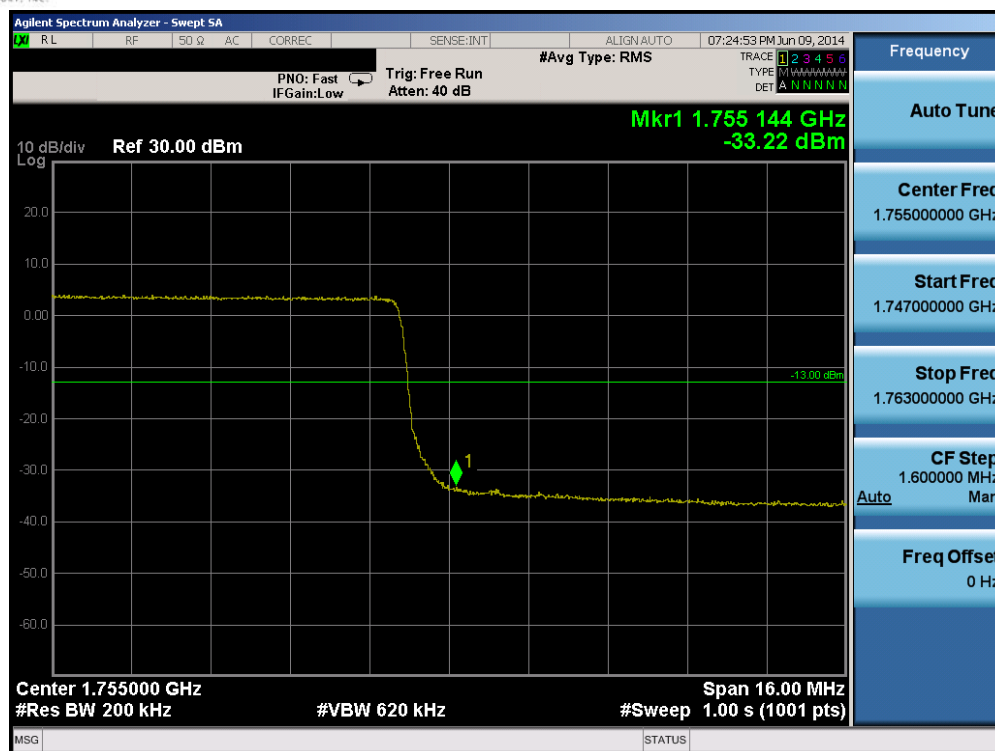
Plot 6-187. Upper Band Edge Plot (Band 4 – 20.0MHz QPSK – RB Size 100)
