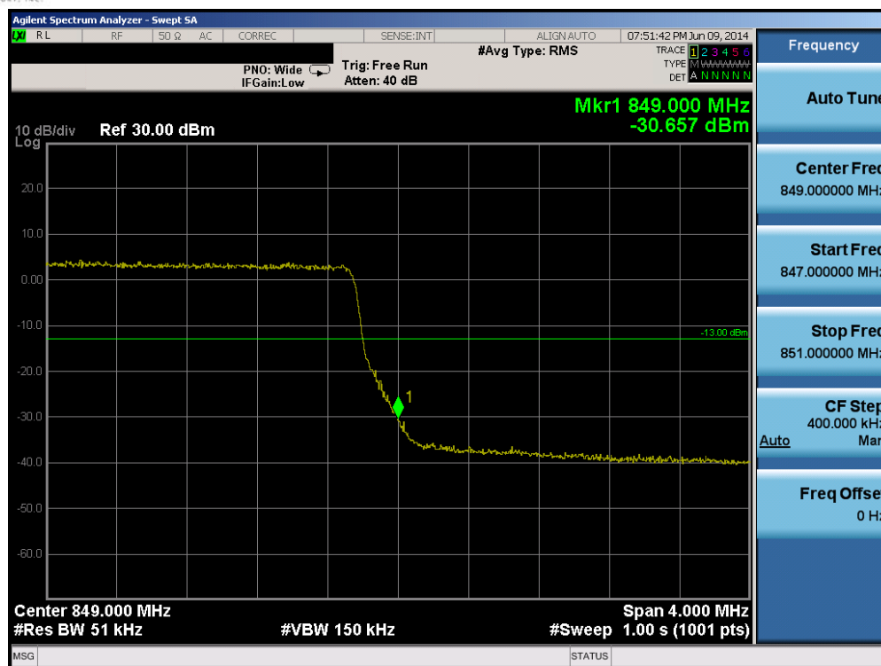
Plot 6-161. Upper Band Edge Plot (Band 5 – 5.0MHz QPSK – RB Size 25)
