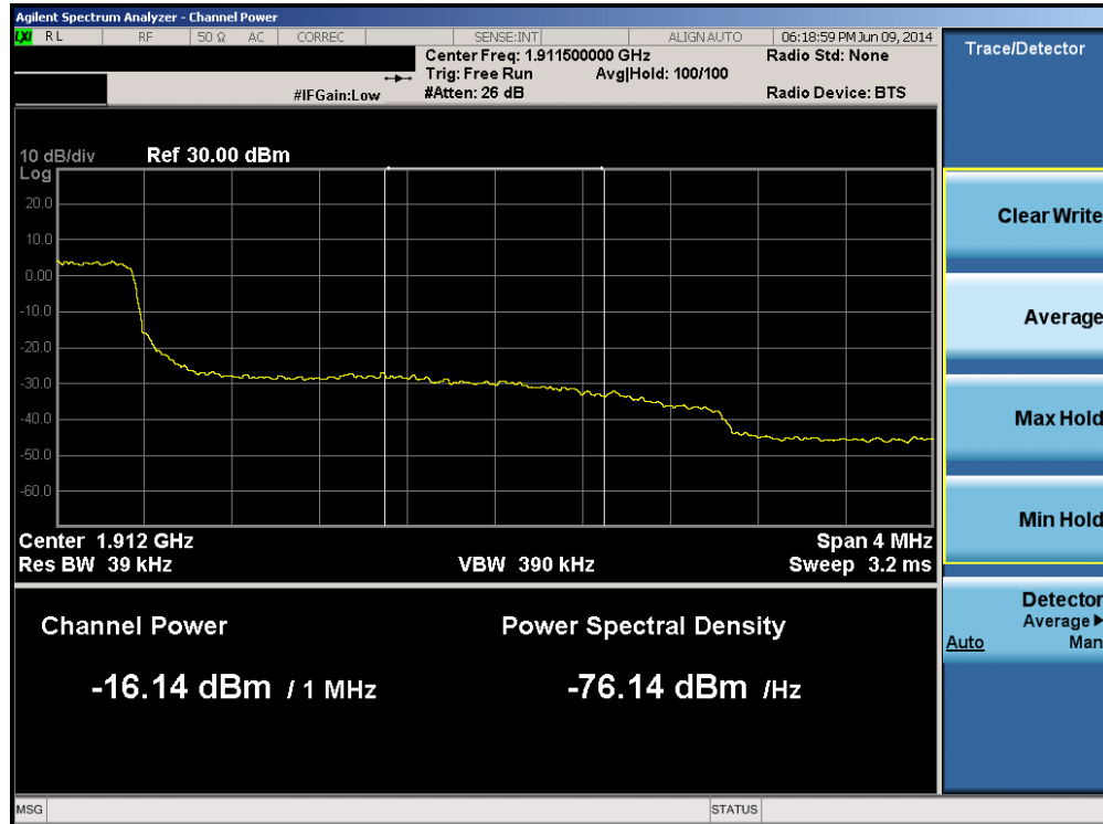
Plot 6-196. Upper Extended Band Edge Plot (Band 2 – 3.0MHz QPSK – RB Size 15)
