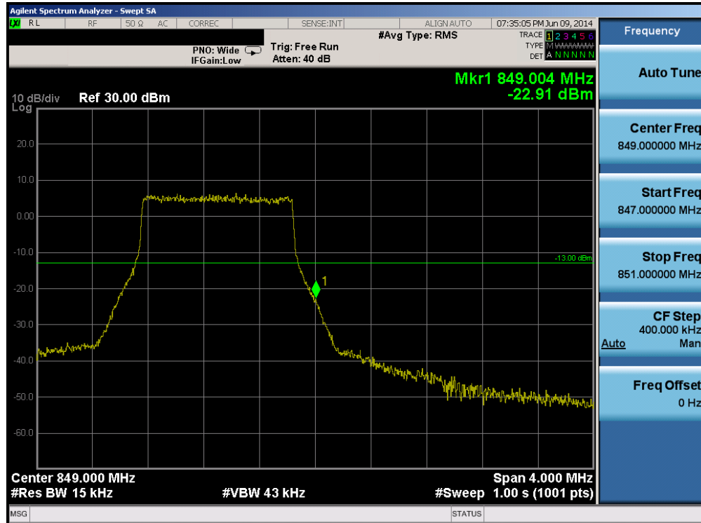
Plot 6-153. Upper Band Edge Plot (Band 5 – 1.4MHz QPSK – RB Size 6)
