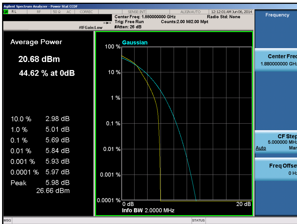
Plot 6-226. PAR Plot (Band 2 – 1.4MHz 16-QAM – RB Size 6)
