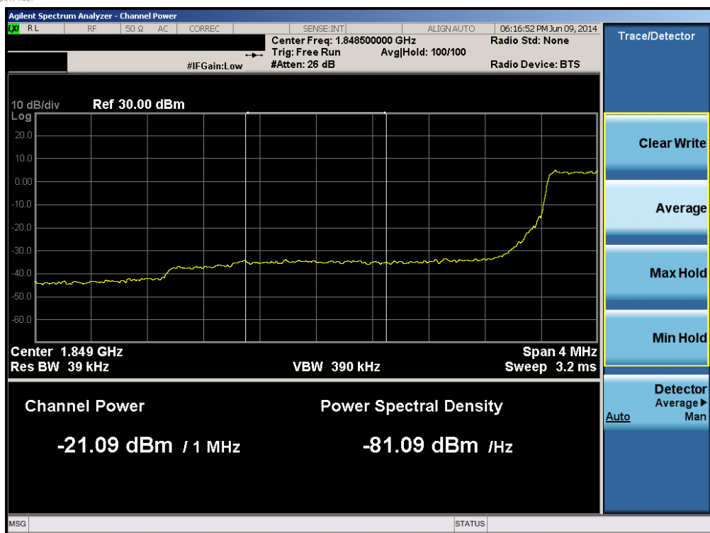
Plot 6-194. Lower Extended Band Edge Plot (Band 2 – 3.0MHz QPSK – RB Size 15)
