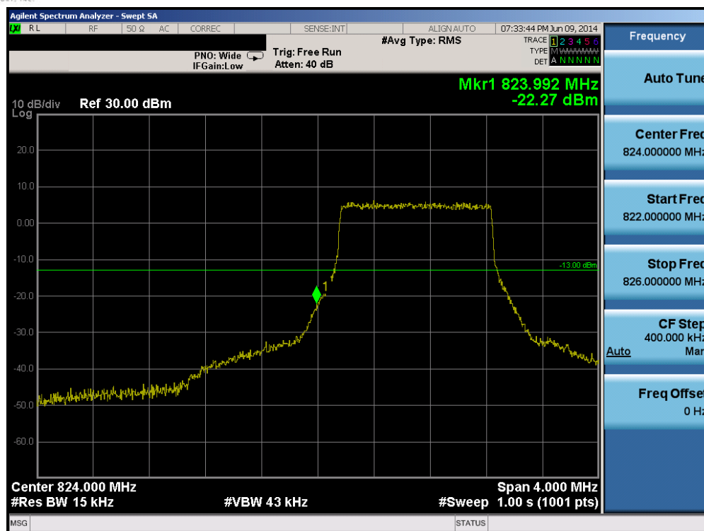
Plot 6-151. Lower Band Edge Plot (Band 5 – 1.4MHz QPSK – RB Size 6)
