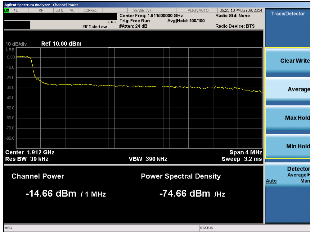
Plot 6-200. Upper Extended Band Edge Plot (Band 2 – 5.0MHz QPSK – RB Size 25)
