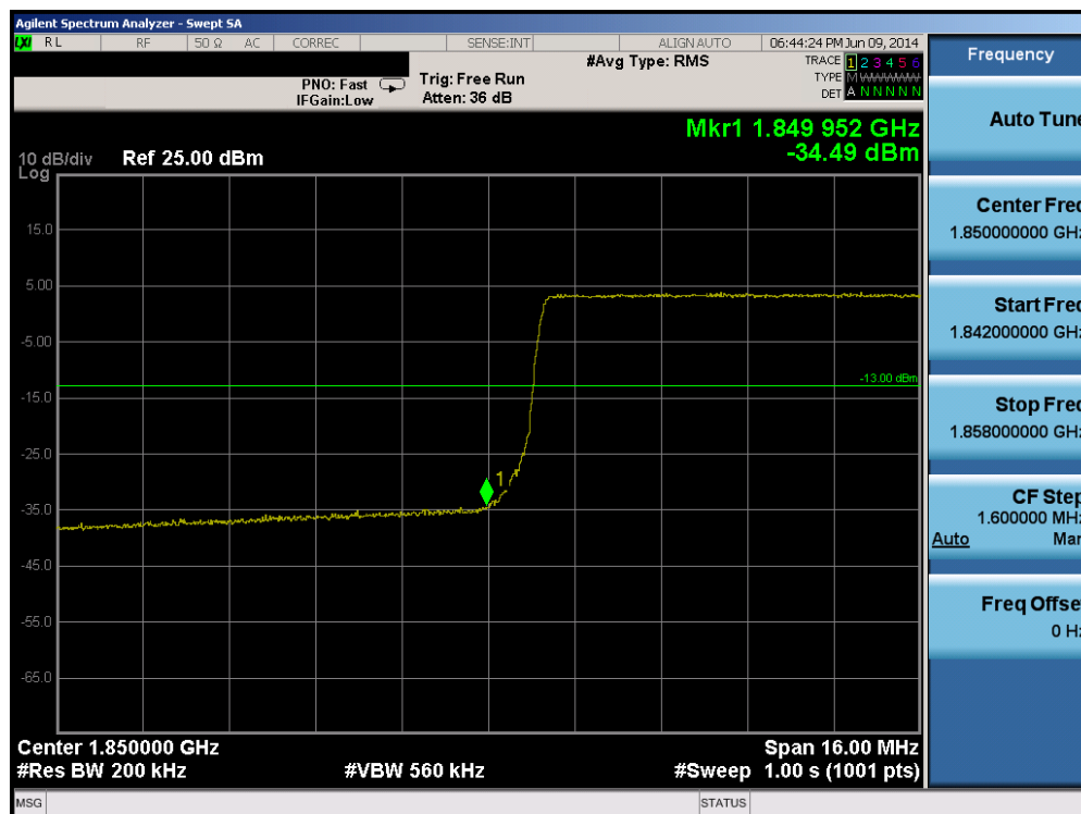
Plot 6-209. Lower Band Edge Plot (Band 2 – 20.0MHz QPSK – RB Size 100)
