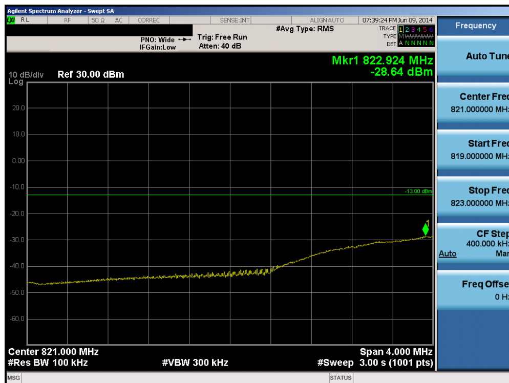
Plot 6-156. Lower Extended Band Edge Plot (Band 5 – 3.0MHz QPSK – RB Size 15)
