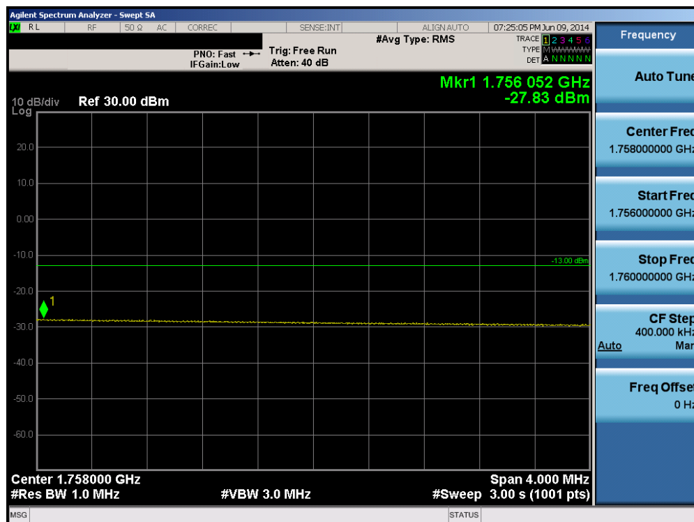
Plot 6-188. Upper Extended Band Edge Plot (Band 4 – 20.0MHz QPSK – RB Size 100)
