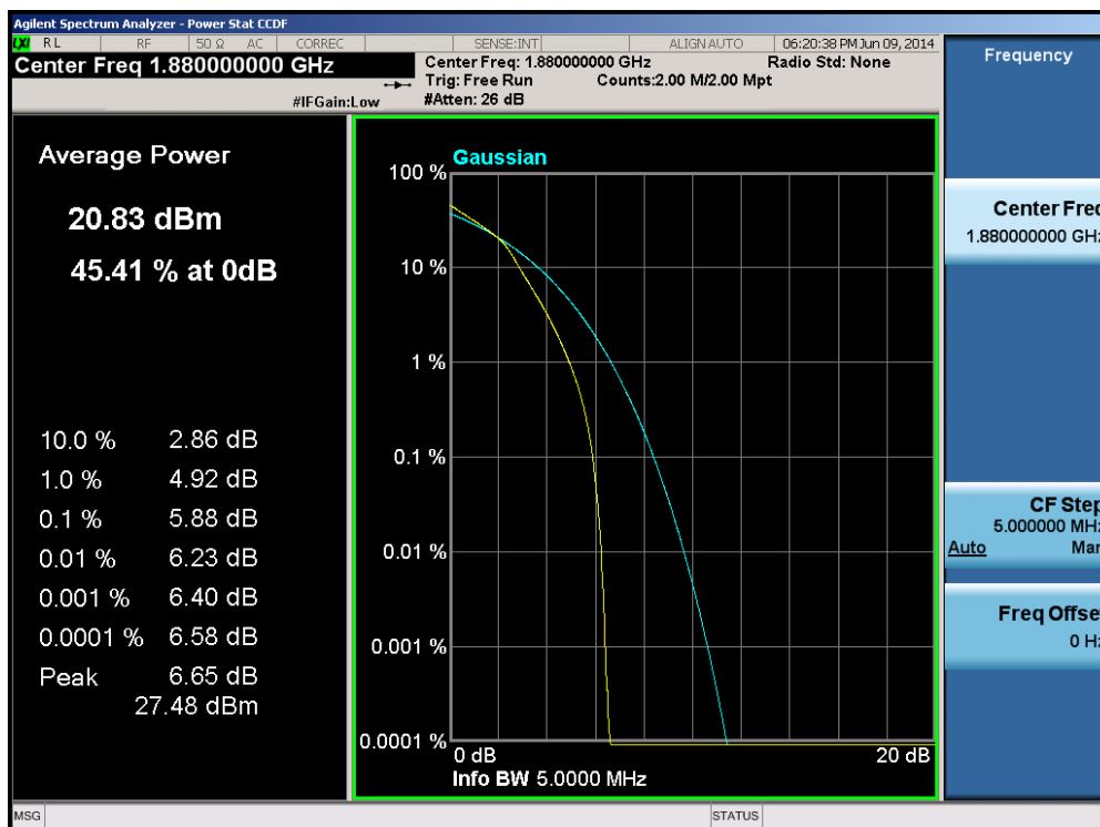
Plot 6-230. PAR Plot (Band 2 – 5.0MHz 16-QAM – RB Size 25)
