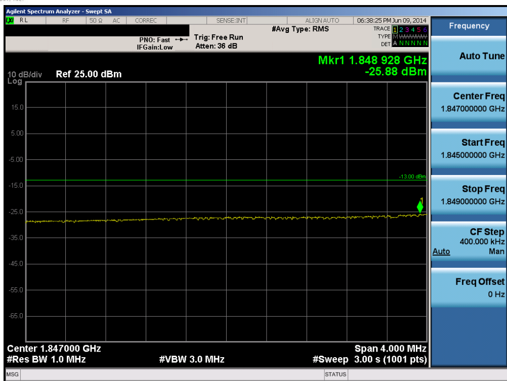
Plot 6-206. Lower Extended Band Edge Plot (Band 2 – 15.0MHz QPSK – RB Size 75)
