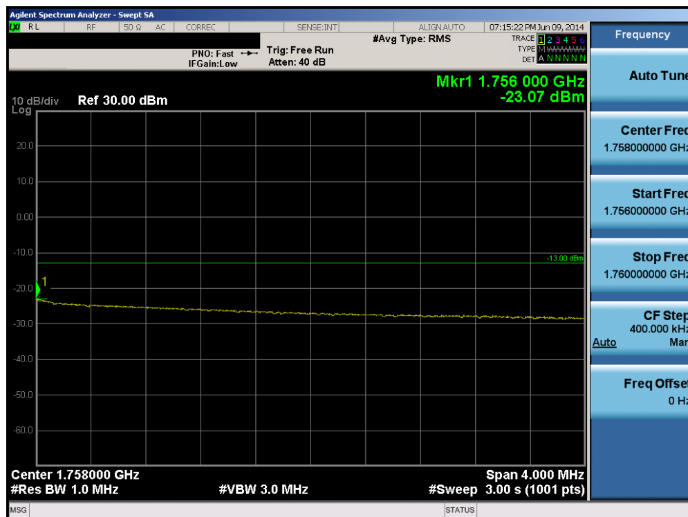
Plot 6-180. Upper Extended Band Edge Plot (Band 4 – 10.0MHz QPSK – RB Size 50)
