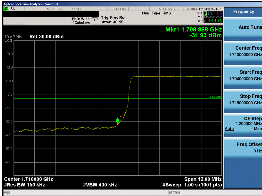
Plot 6-181. Lower Band Edge Plot (Band 4 – 15.0MHz QPSK – RB Size 75)
