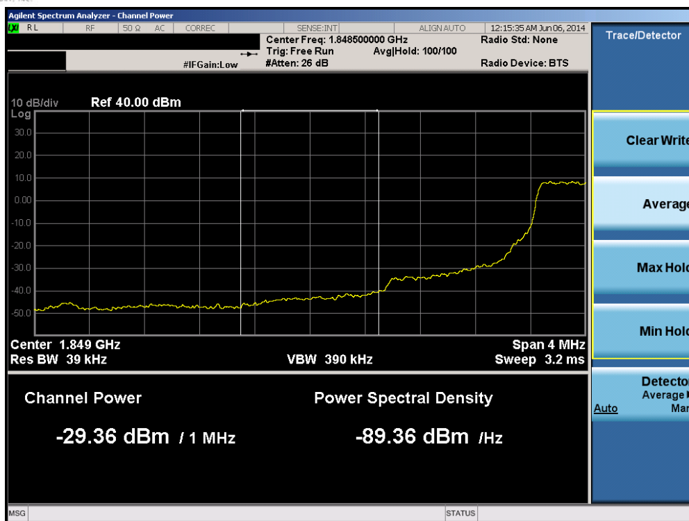
Plot 6-190. Lower Extended Band Edge Plot (Band 2 – 1.4MHz QPSK – RB Size 6)
