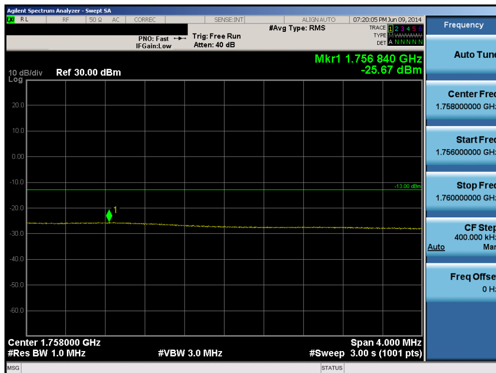
Plot 6-184. Upper Extended Band Edge Plot (Band 4 – 15.0MHz QPSK – RB Size 75)
