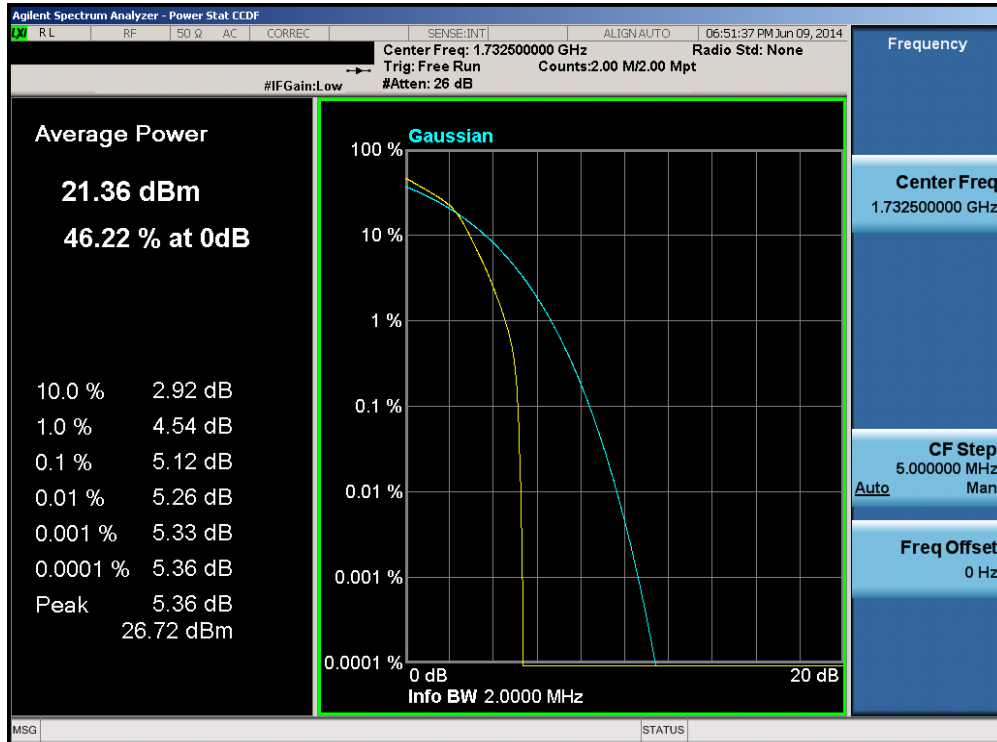
Plot 6-214. PAR Plot (Band 4 – 1.4MHz 16-QAM – RB Size 6)
