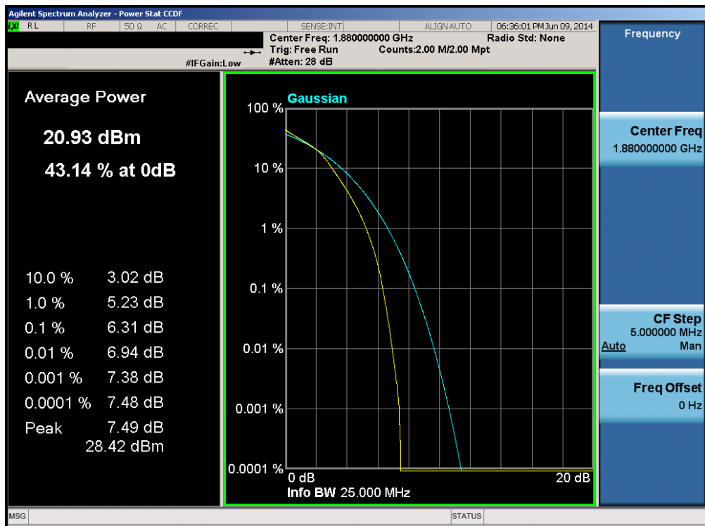
Plot 6-234. PAR Plot (Band 2 – 15.0MHz 16-QAM – RB Size 75)
