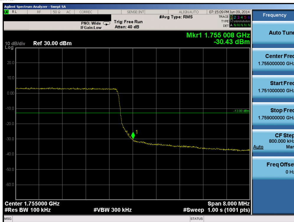
Plot 6-179. Upper Band Edge Plot (Band 4 – 10.0MHz QPSK – RB Size 50)
