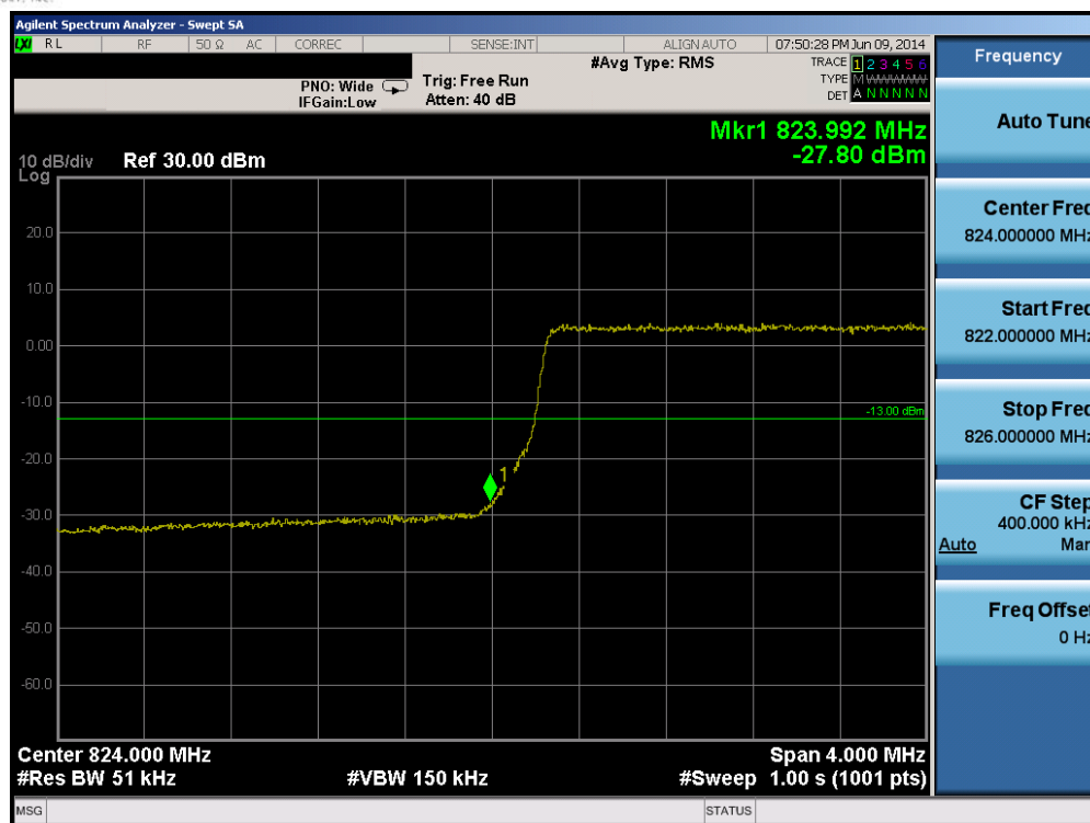
Plot 6-159. Lower Band Edge Plot (Band 5 – 5.0MHz QPSK – RB Size 25)
