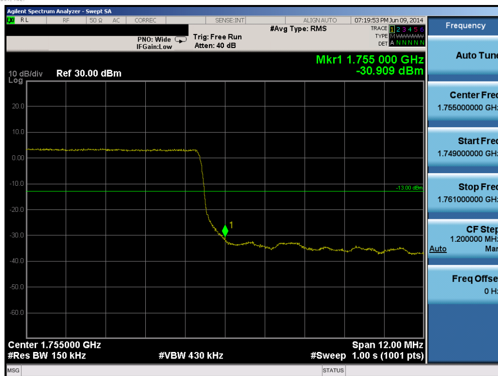
Plot 6-183. Upper Band Edge Plot (Band 4 – 15.0MHz QPSK – RB Size 75)
