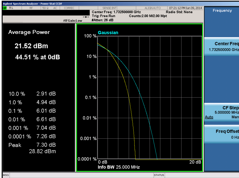
Plot 6-224. PAR Plot (Band 4 – 20.0MHz 16-QAM – RB Size 100)
