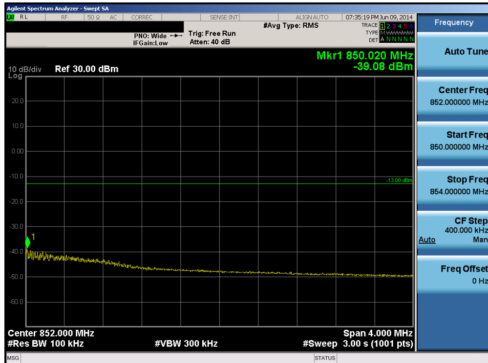
Plot 6-154. Upper Extended Band Edge Plot (Band 5 – 1.4MHz QPSK – RB Size 6)
