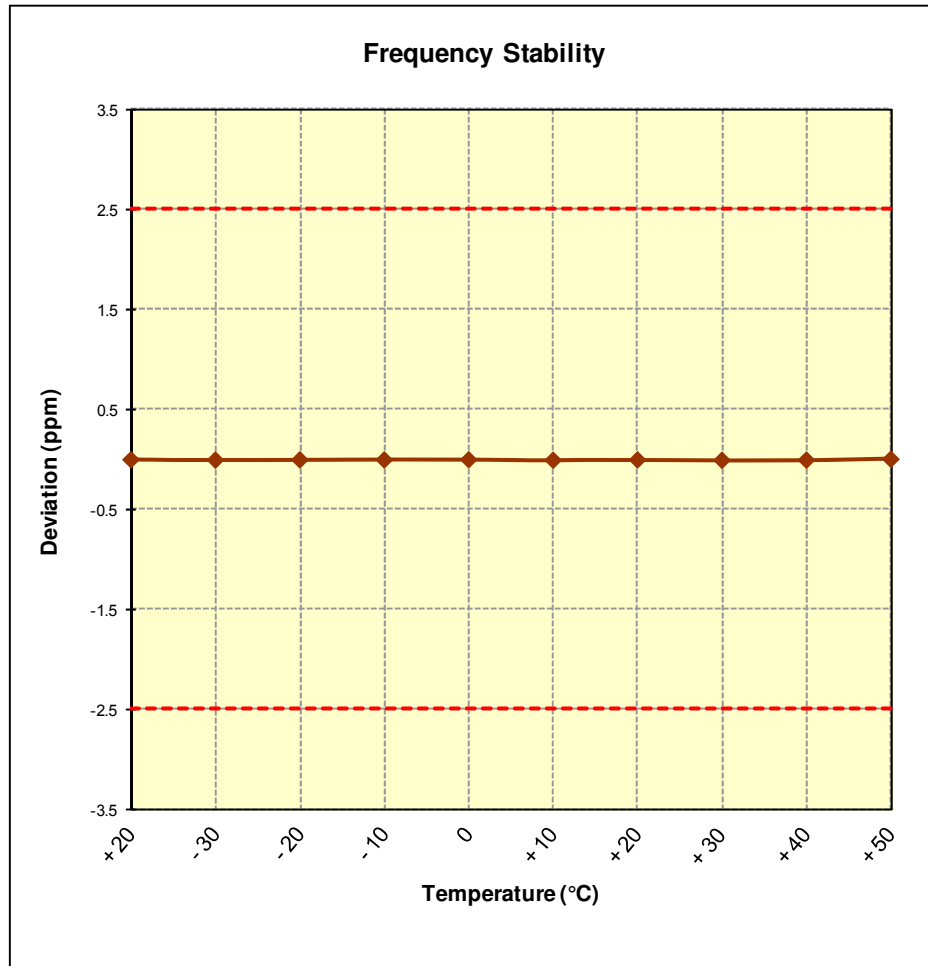
Figure 6-6. Frequency Stability Graph (Band 5)
