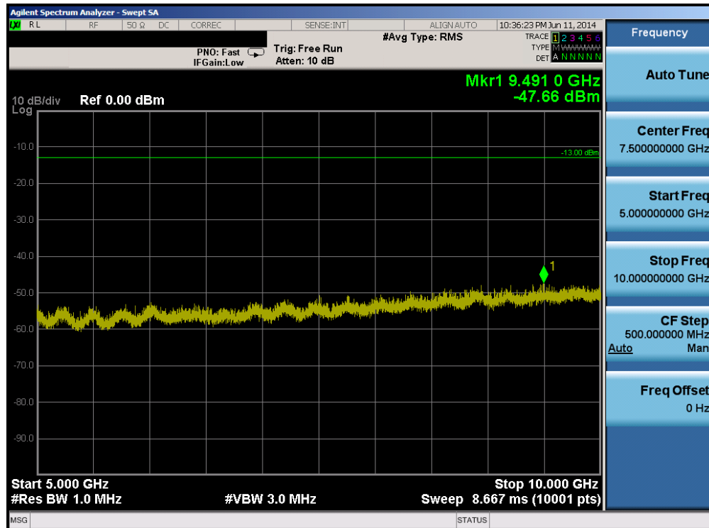
Plot 6-12. Conducted Spurious Plot (Band 5 – 5.0MHz QPSK – RB Size 1, RB Offset 0 – Mid Channel)
