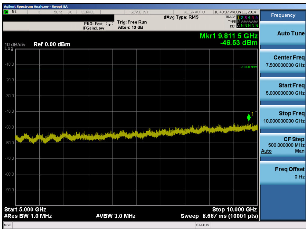
Plot 6-14. Conducted Spurious Plot (Band 5 – 5.0MHz QPSK – RB Size 1, RB Offset 0 – High Channel)
