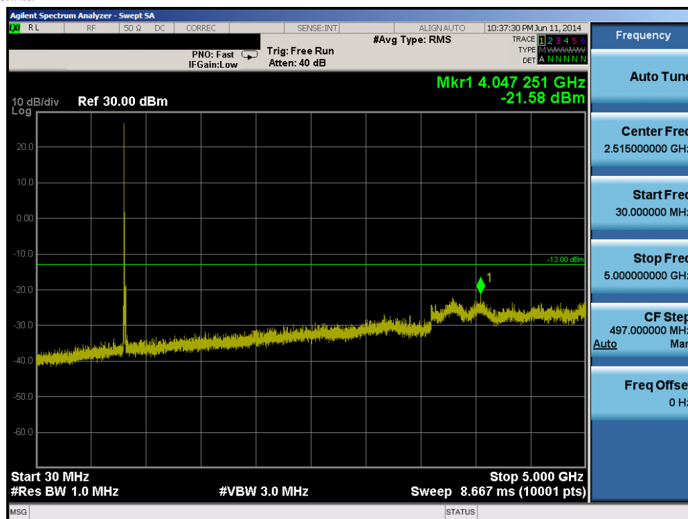
Plot 6-9. Conducted Spurious Plot (Band 5 – 5.0MHz QPSK – RB Size 1, RB Offset 0 – Low Channel)
