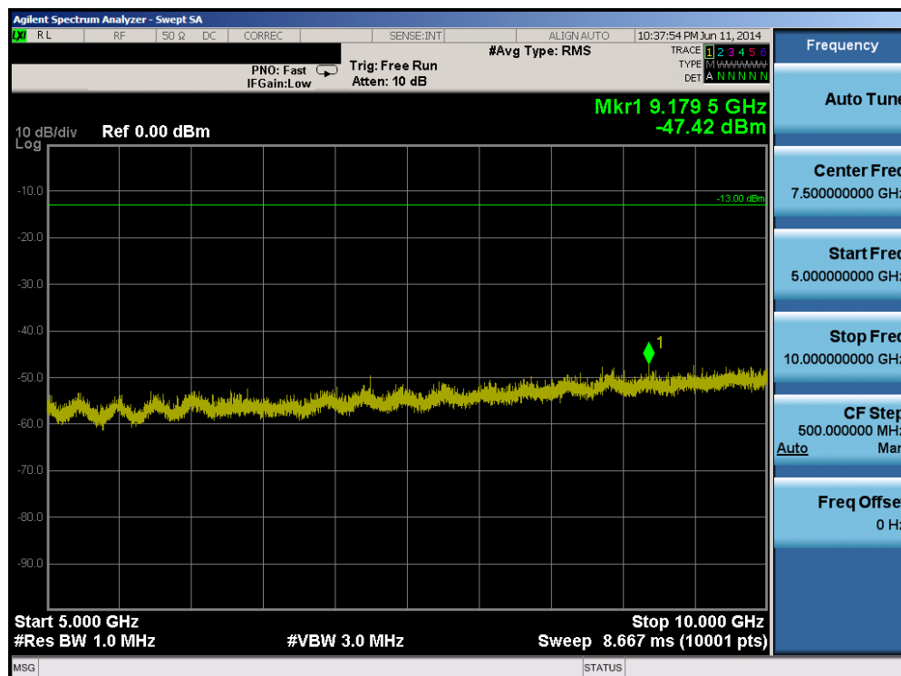
Plot 6-10. Conducted Spurious Plot (Band 5 – 5.0MHz QPSK – RB Size 1, RB Offset 0 – Low Channel)
