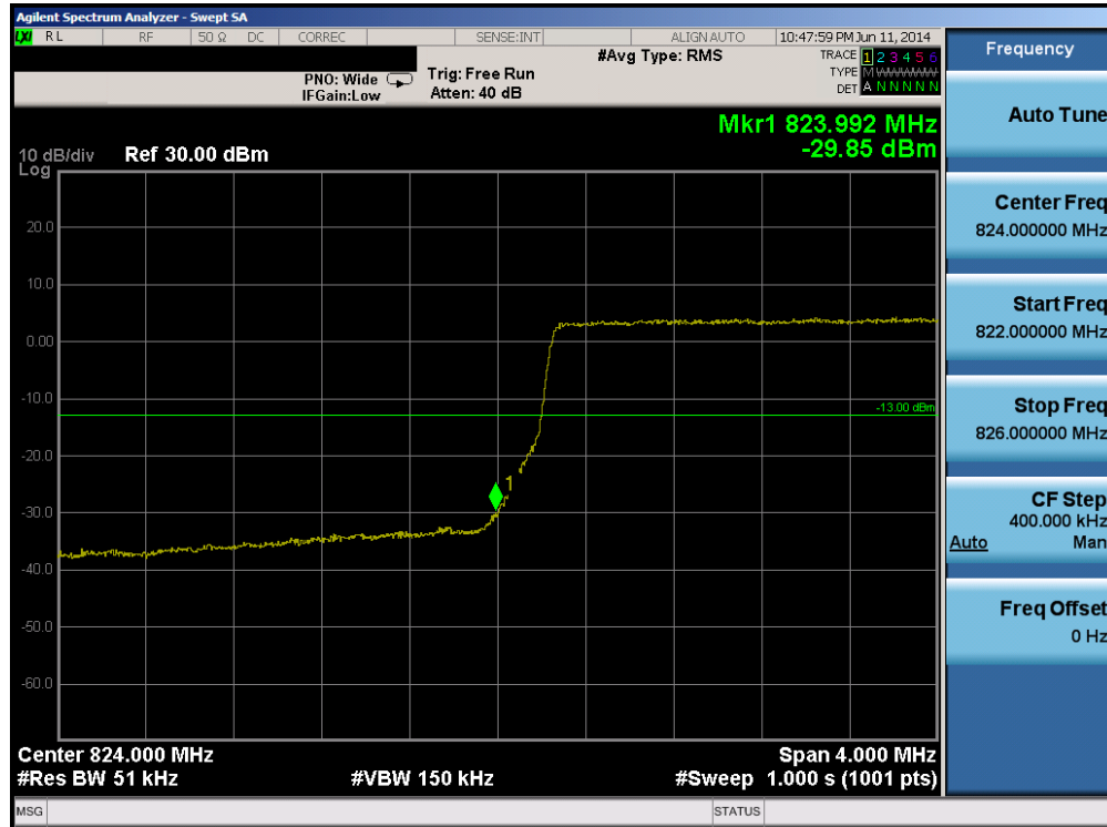
Plot 6-23. Lower Band Edge Plot (Band 5 – 5.0MHz QPSK – RB Size 25)
