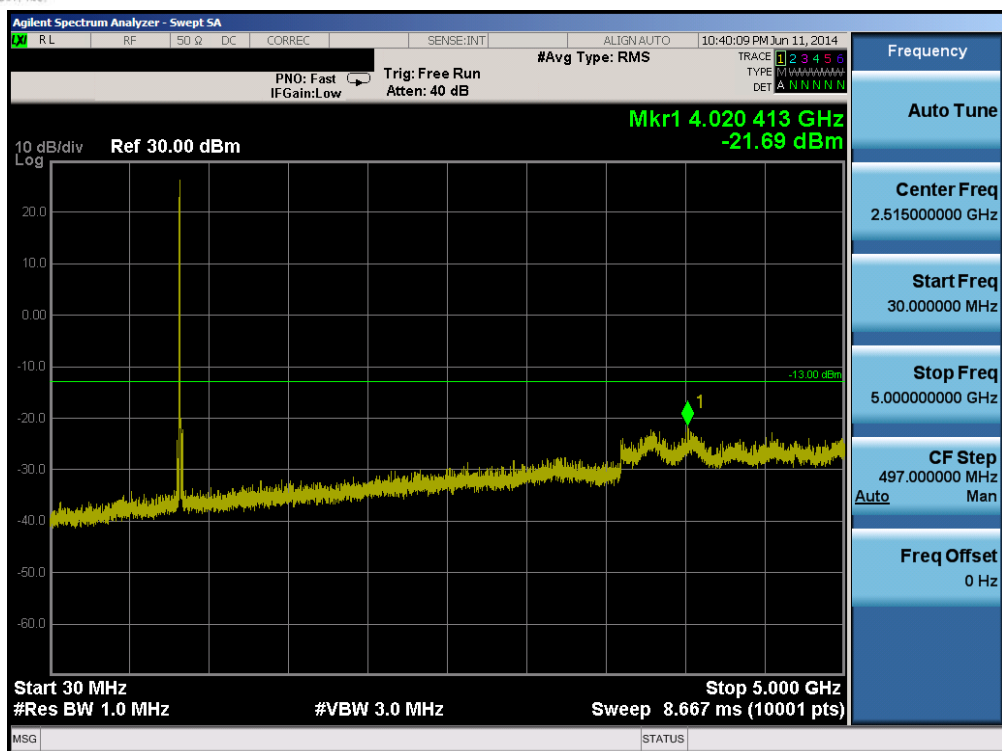
Plot 6-13. Conducted Spurious Plot (Band 5 – 5.0MHz QPSK – RB Size 1, RB Offset 0 – High Channel)
