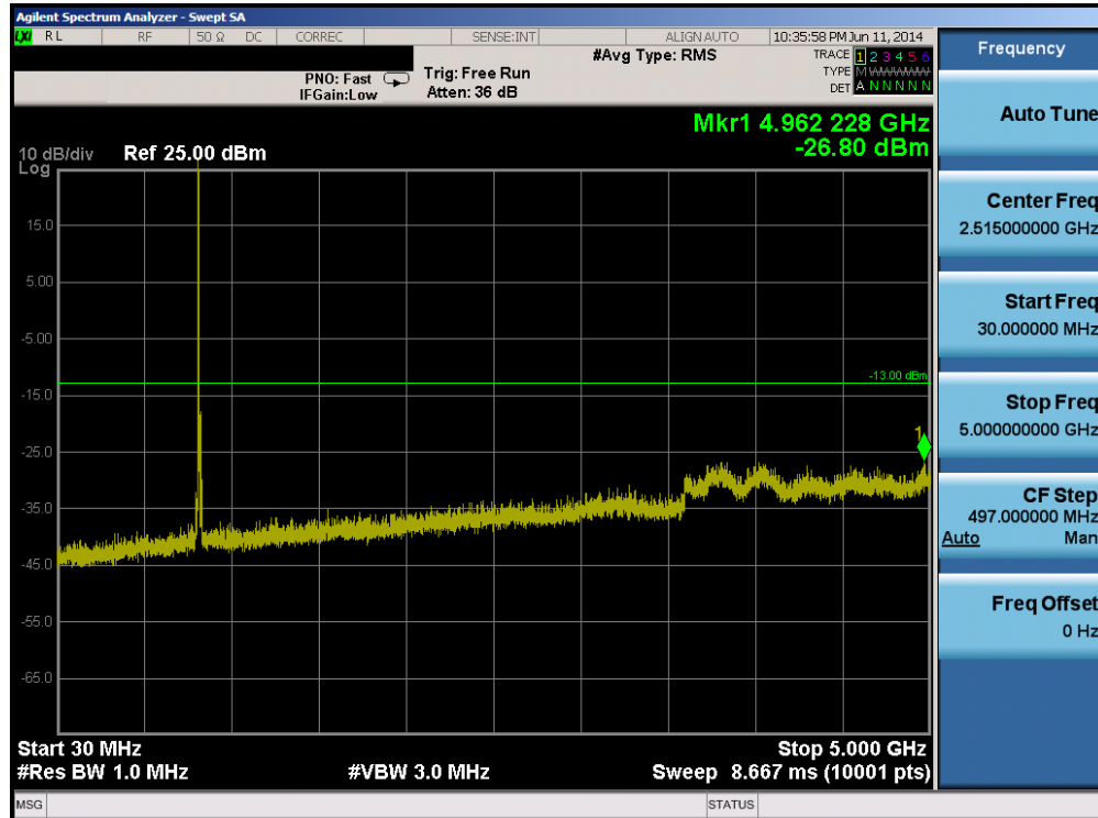
Plot 6-11. Conducted Spurious Plot (Band 5 – 5.0MHz QPSK – RB Size 1, RB Offset 0 – Mid Channel)
