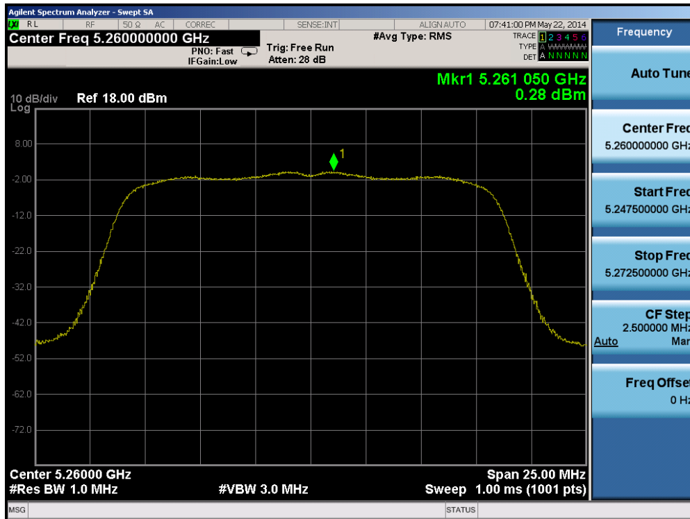
Plot 6-37. Peak Power Spectral Density Plot (802.11a (UNII Band 2A) – Ch. 52)
