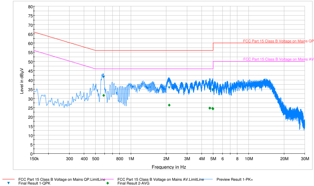
Plot 6-72. Line Conducted Plot with 802.11a UNII Band 1 (N)
