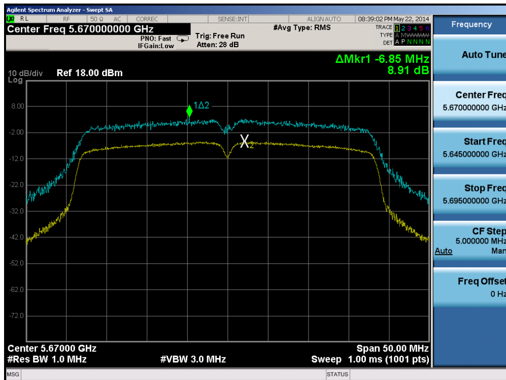
Plot 6-56. Peak Excursion Ratio Plot (40MHz BW 802.11n (UNII Band 2C) – Ch. 134)
