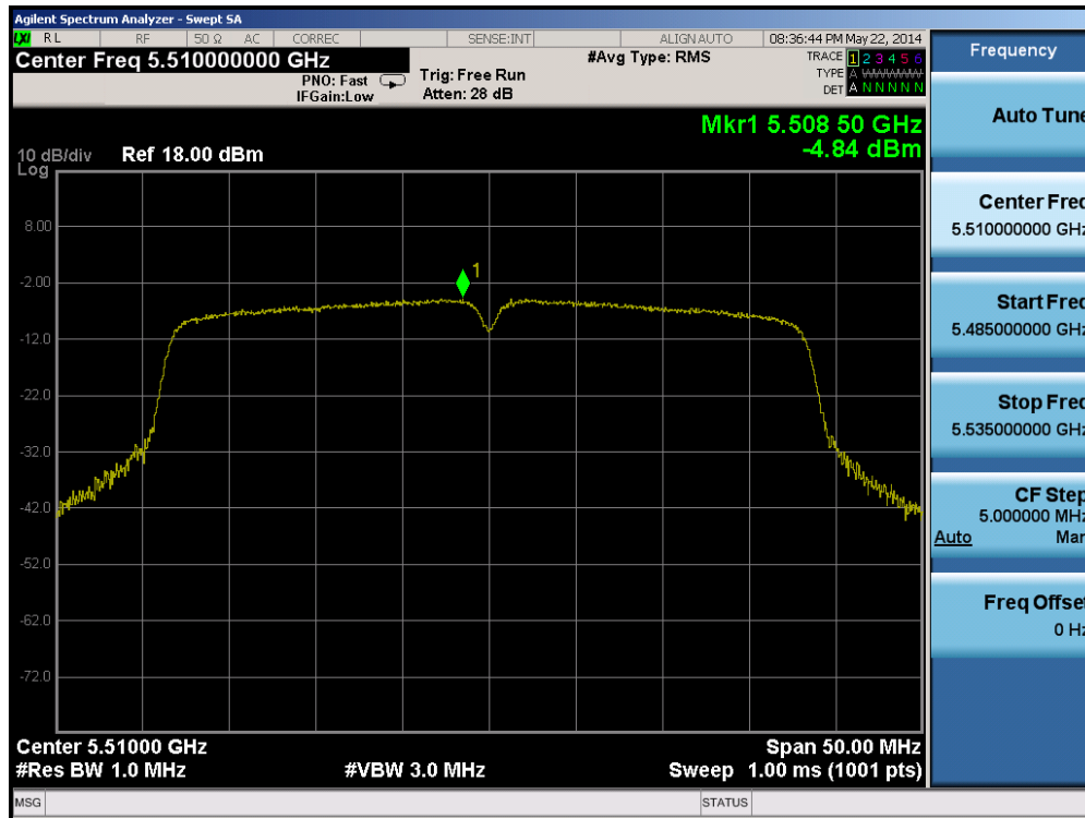
Plot 6-51. Peak Power Spectral Density Plot (40MHz BW 802.11n (UNII Band 2C) – Ch. 102)
