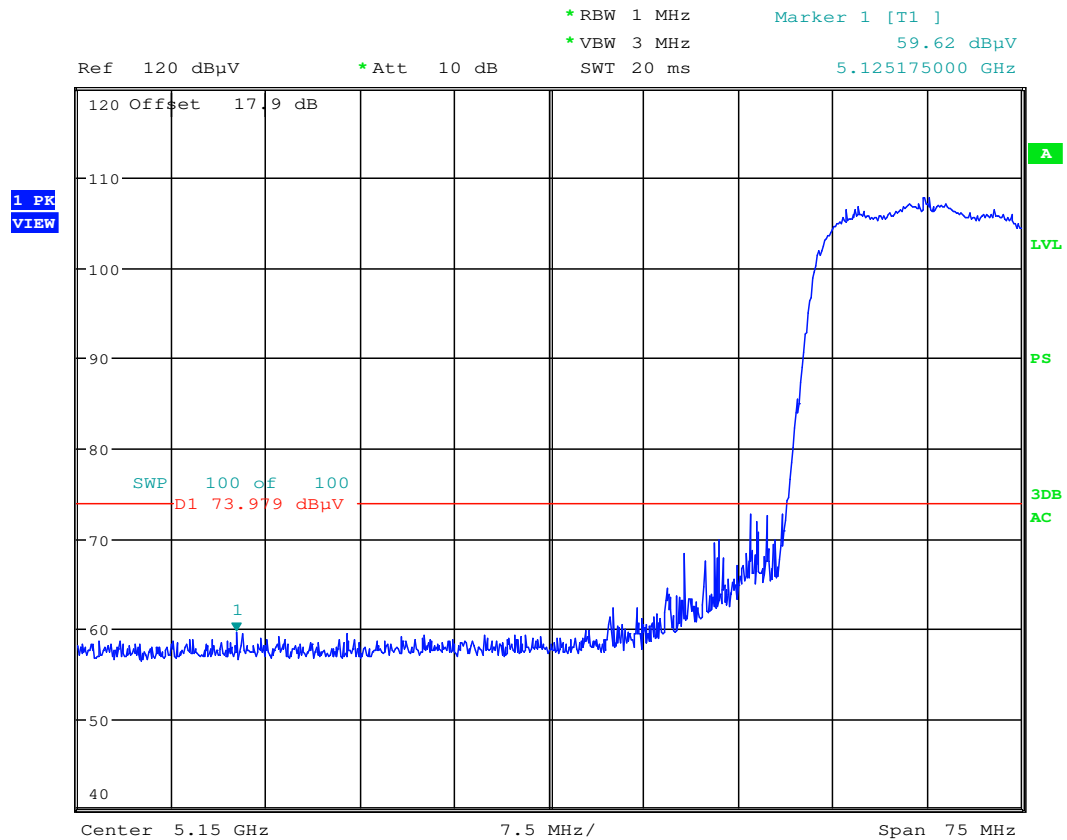
Plot 6-58. Radiated Restricted Lower Band Edge Plot (Peak – UNII Band 1)
