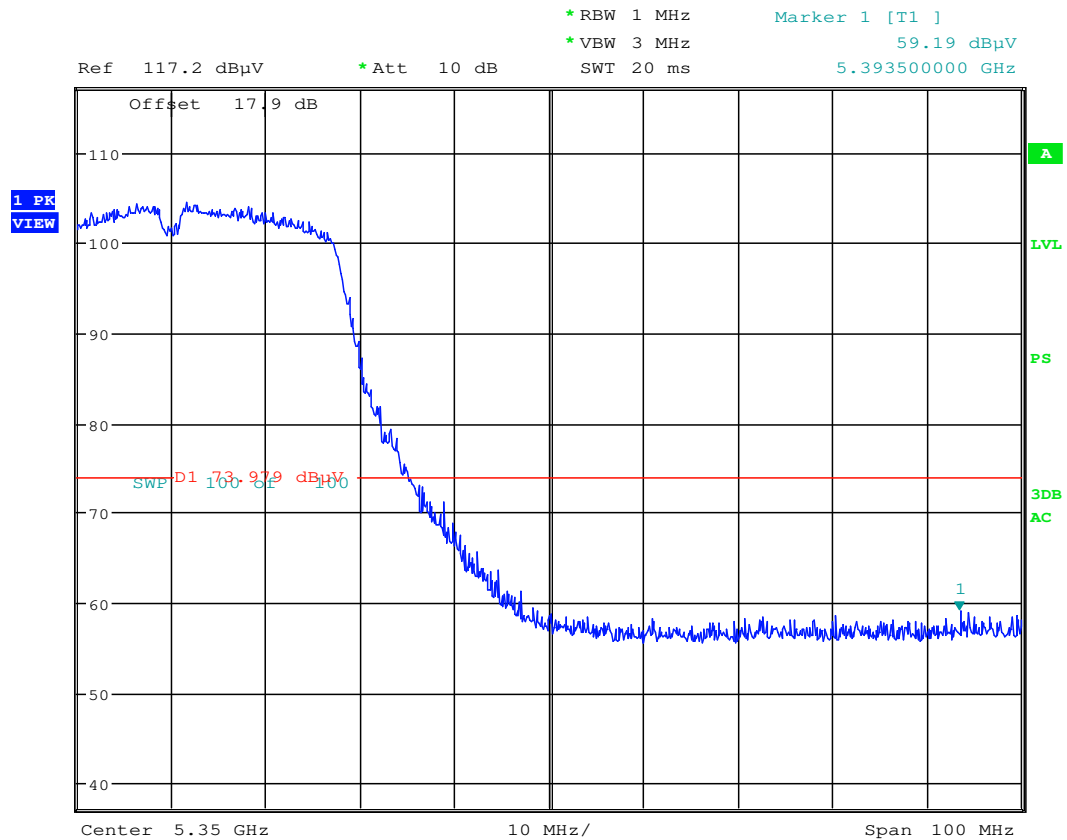
Plot 6-67. Radiated Restricted Upper Band Edge Plot (Peak – UNII Band 2A)
