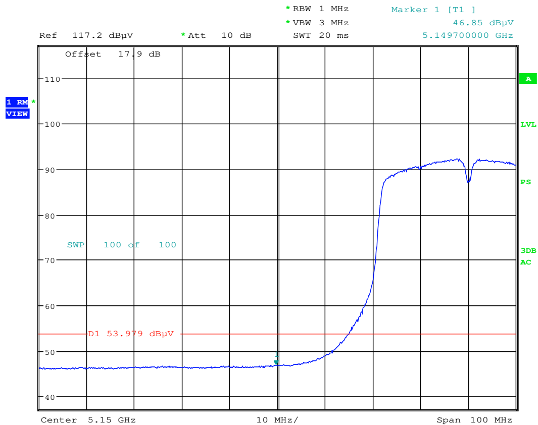
Plot 6-64. Radiated Restricted Lower Band Edge Plot (Average – UNII Band 1)
