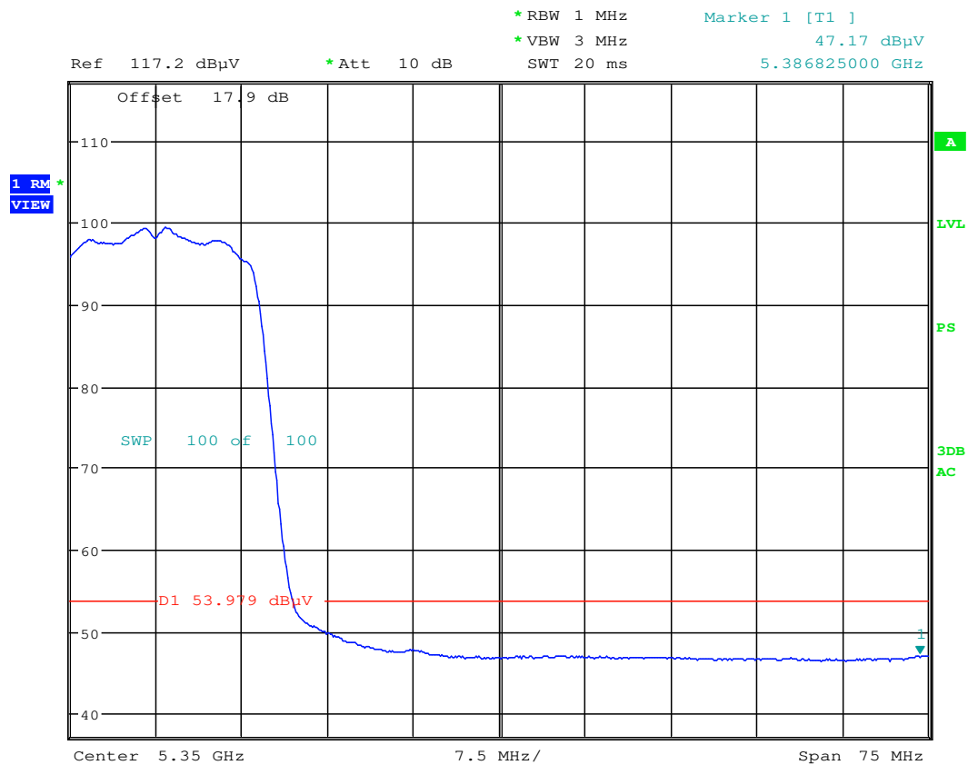
Plot 6-59. Radiated Restricted Upper Band Edge Plot (Average – UNII Band 2A)
