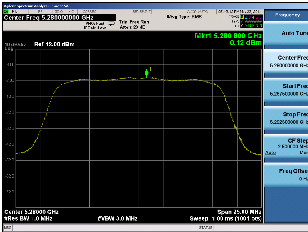
Plot 6-38. Peak Power Spectral Density Plot (802.11a (UNII Band 2A) – Ch. 56)
