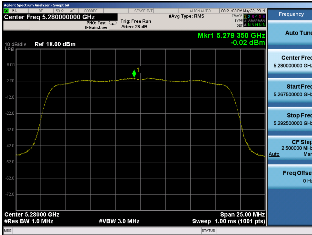
Plot 6-41. Peak Power Spectral Density Plot (20MHz BW 802.11n (UNII Band 2A) – Ch. 56)
