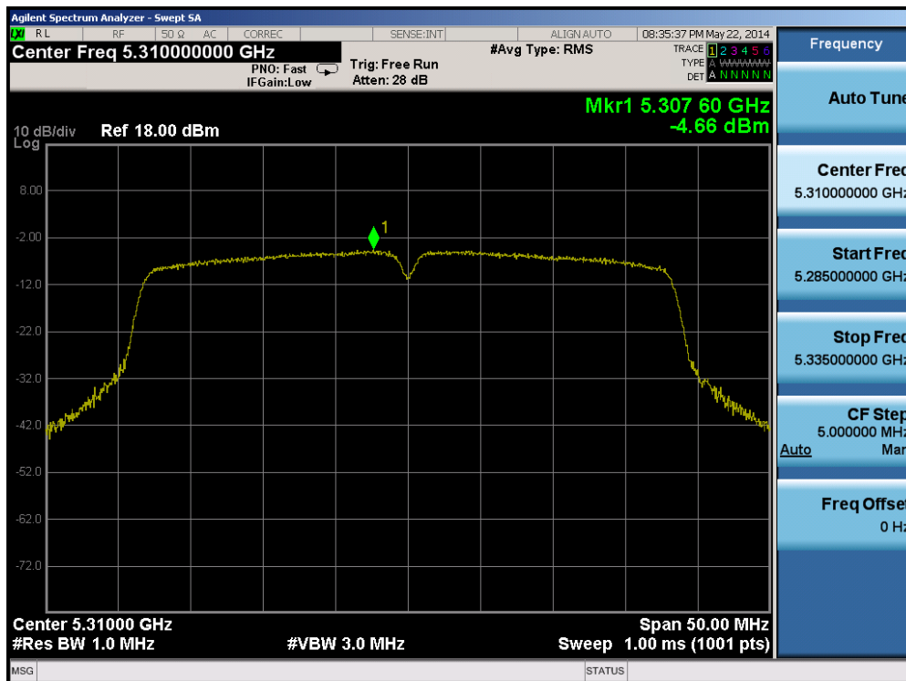
Plot 6-44. Peak Power Spectral Density Plot (40MHz BW 802.11n (UNII Band 2A) – Ch. 62)
