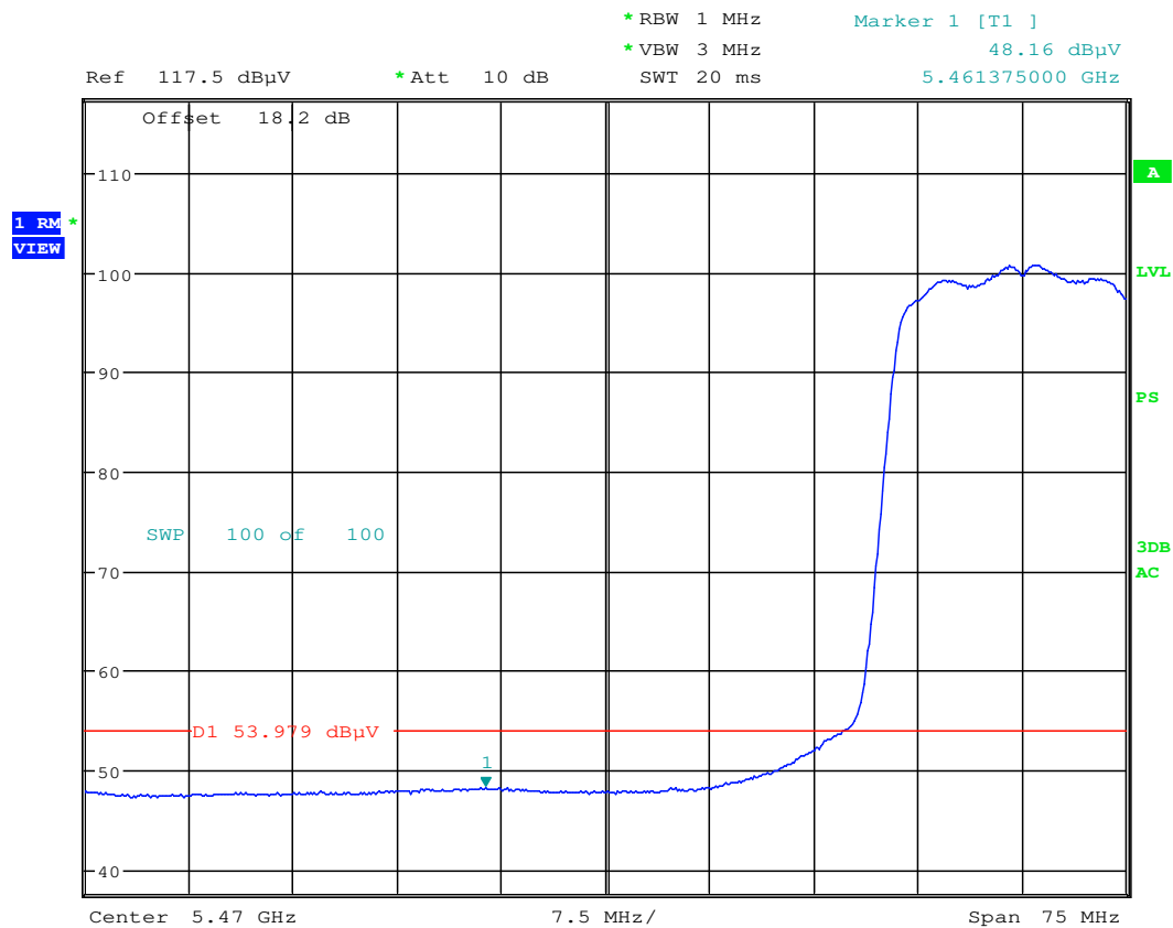
Plot 6-68. Radiated Restricted Lower Band Edge Plot (Average – UNII Band 2C)
