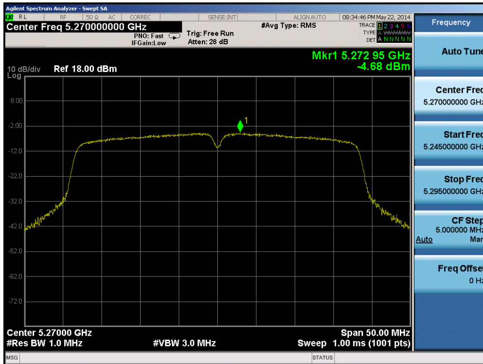
Plot 6-43. Peak Power Spectral Density Plot (40MHz BW 802.11n (UNII Band 2A) – Ch. 54)
