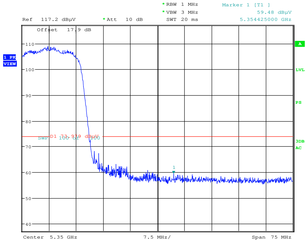
Plot 6-60. Radiated Restricted Upper Band Edge Plot (Peak – UNII Band 2A)
