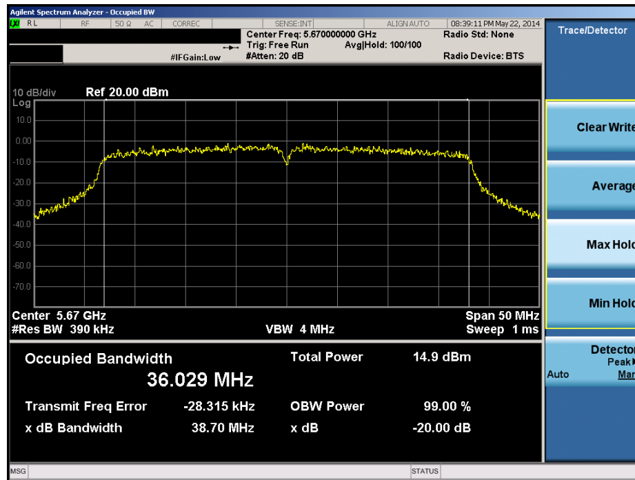
Plot 6-28. 20dB Bandwidth Plot (40MHz BW 802.11n (UNII Band 2C) – Ch. 134)
