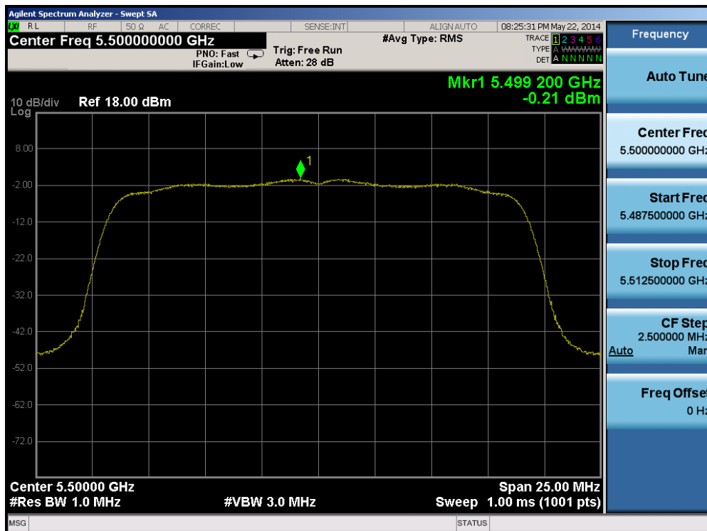
Plot 6-48. Peak Power Spectral Density Plot (20MHz BW 802.11n (UNII Band 2C) – Ch. 100)
