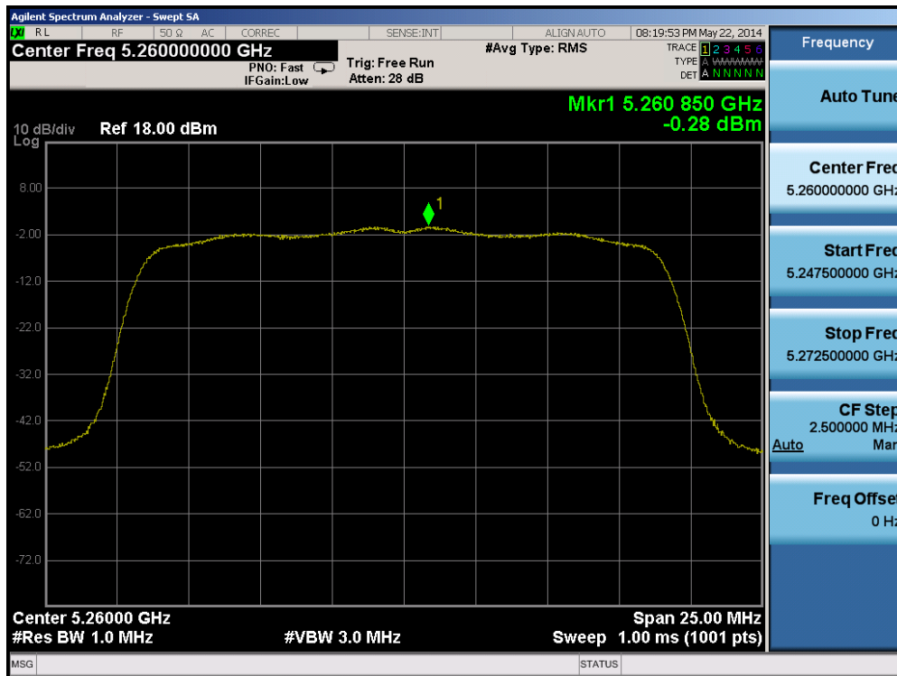
Plot 6-40. Peak Power Spectral Density Plot (20MHz BW 802.11n (UNII Band 2A) – Ch. 52)
