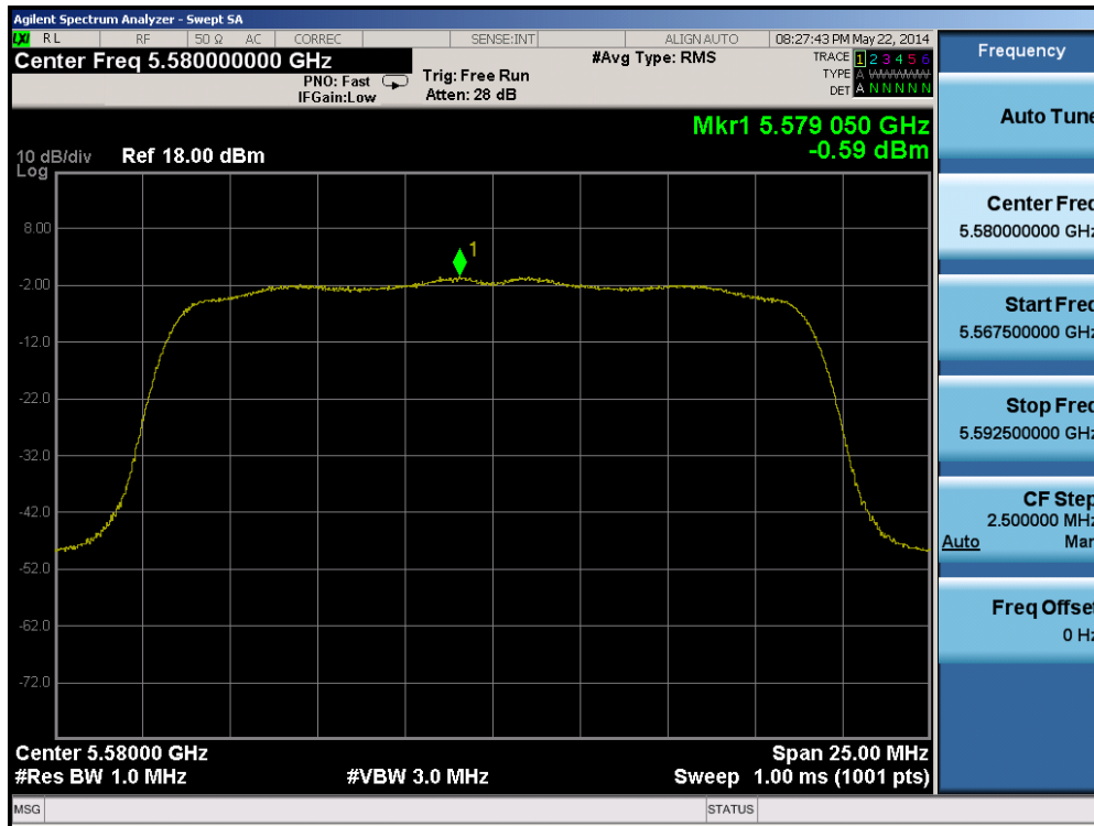
Plot 6-49. Peak Power Spectral Density Plot (20MHz BW 802.11n (UNII Band 2C) – Ch. 116)
