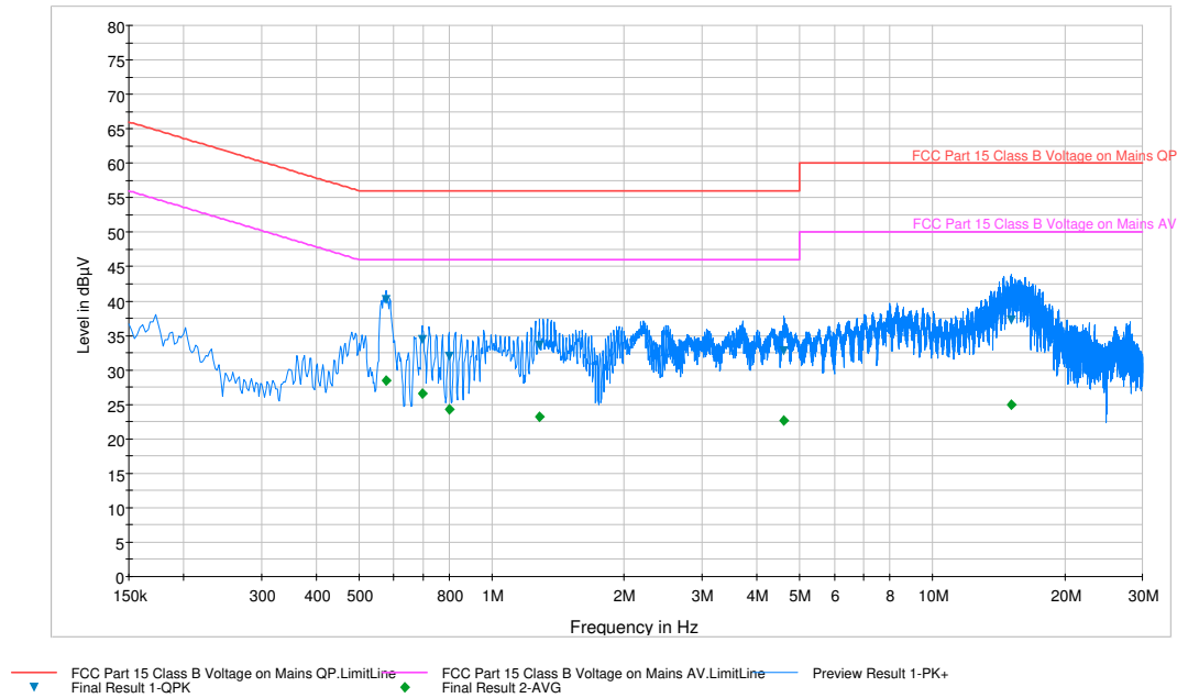
Plot 6-75. Line Conducted Plot with 802.11a UNII Band 2C (L1)
