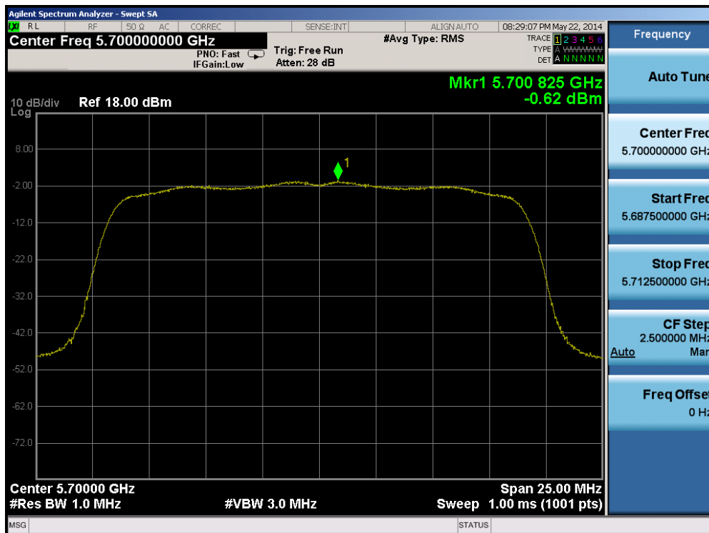
Plot 6-50. Peak Power Spectral Density Plot (20MHz BW 802.11a/n (UNII Band 2C) – Ch. 140)
