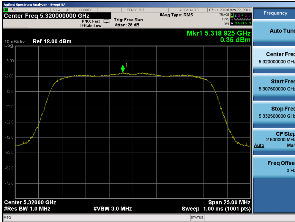
Plot 6-39. Peak Power Spectral Density Plot (802.11a (UNII Band 2A) – Ch. 64)
