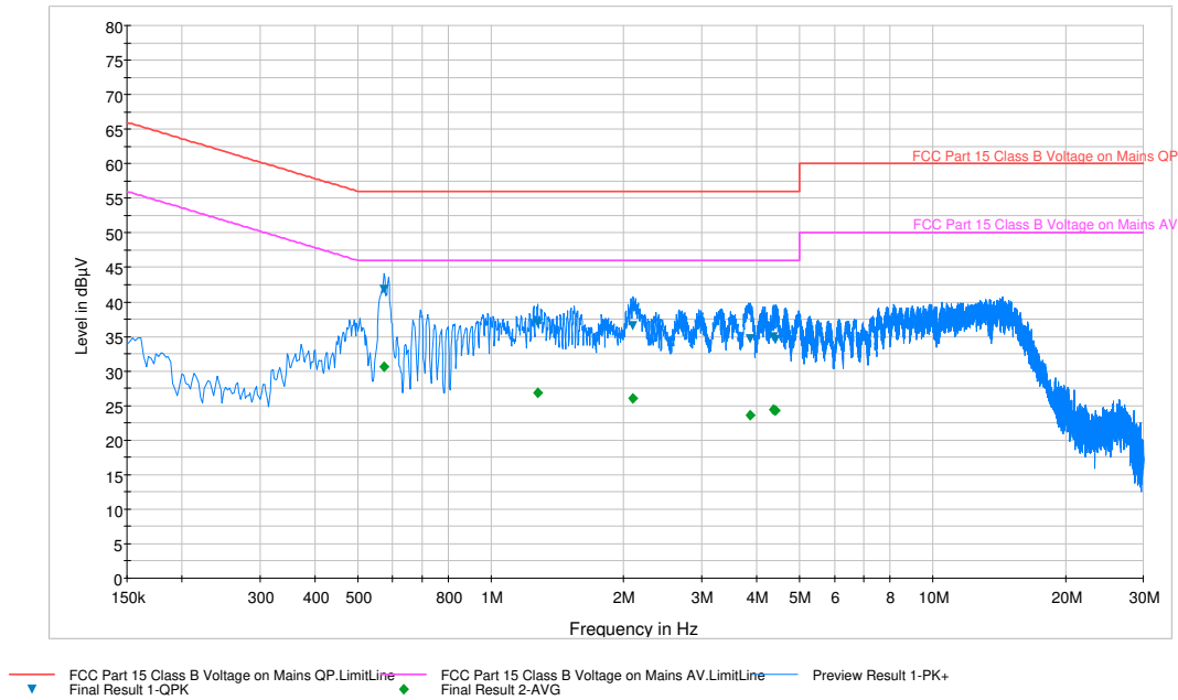
Plot 6-76. Line Conducted Plot with 802.11a UNII Band 2C (N)
