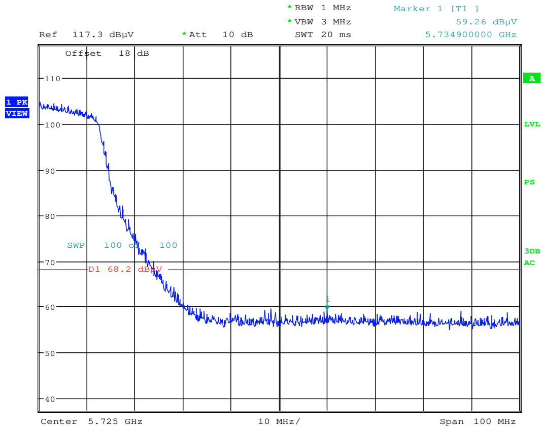
Plot 6-70. Radiated Upper Band Edge Plot (Peak – UNII Band 2C)
