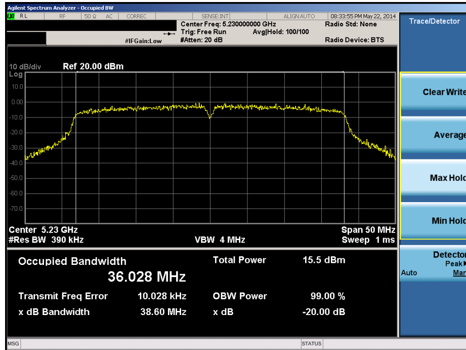
Plot 6-27. 20dB Bandwidth Plot (40MHz BW 802.11n (UNII Band 1) – Ch. 46)
