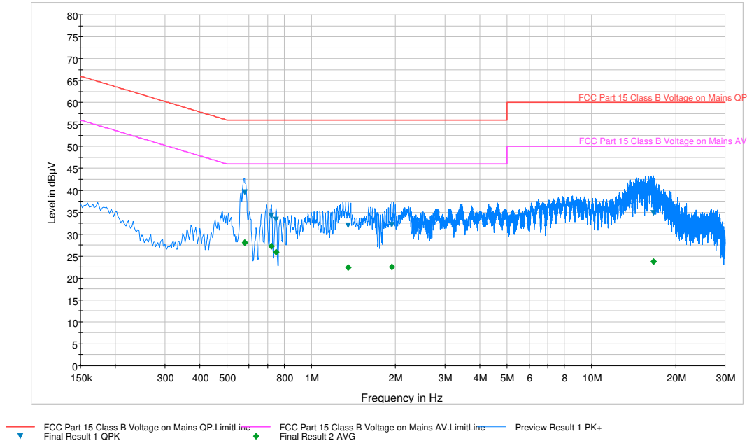
Plot 6-73. Line Conducted Plot with 802.11a UNII Band 2A (L1)
