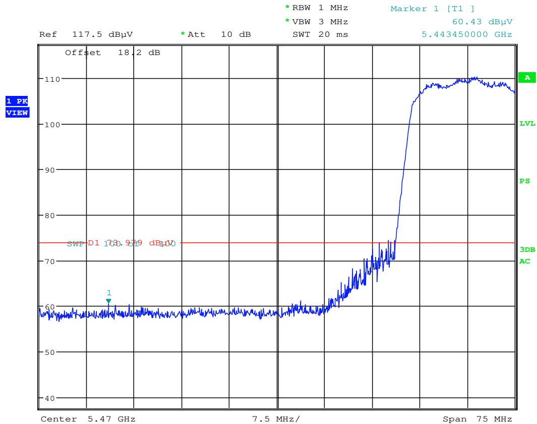
Plot 6-62. Radiated Restricted Lower Band Edge Plot (Peak – UNII Band 2C)
