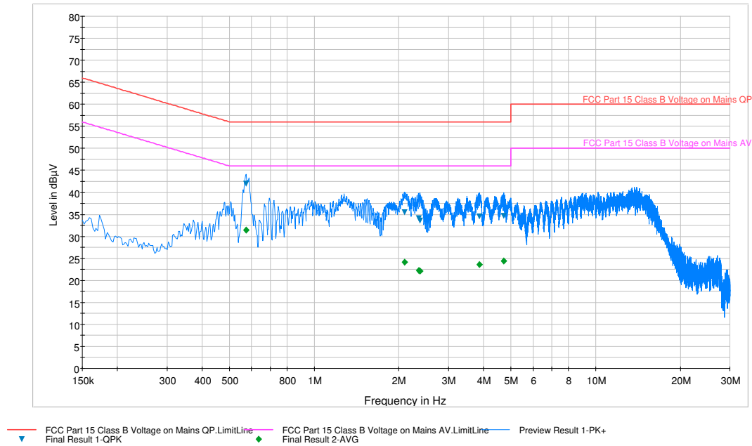
Plot 6-74. Line Conducted Plot with 802.11a UNII Band 2A (N)
