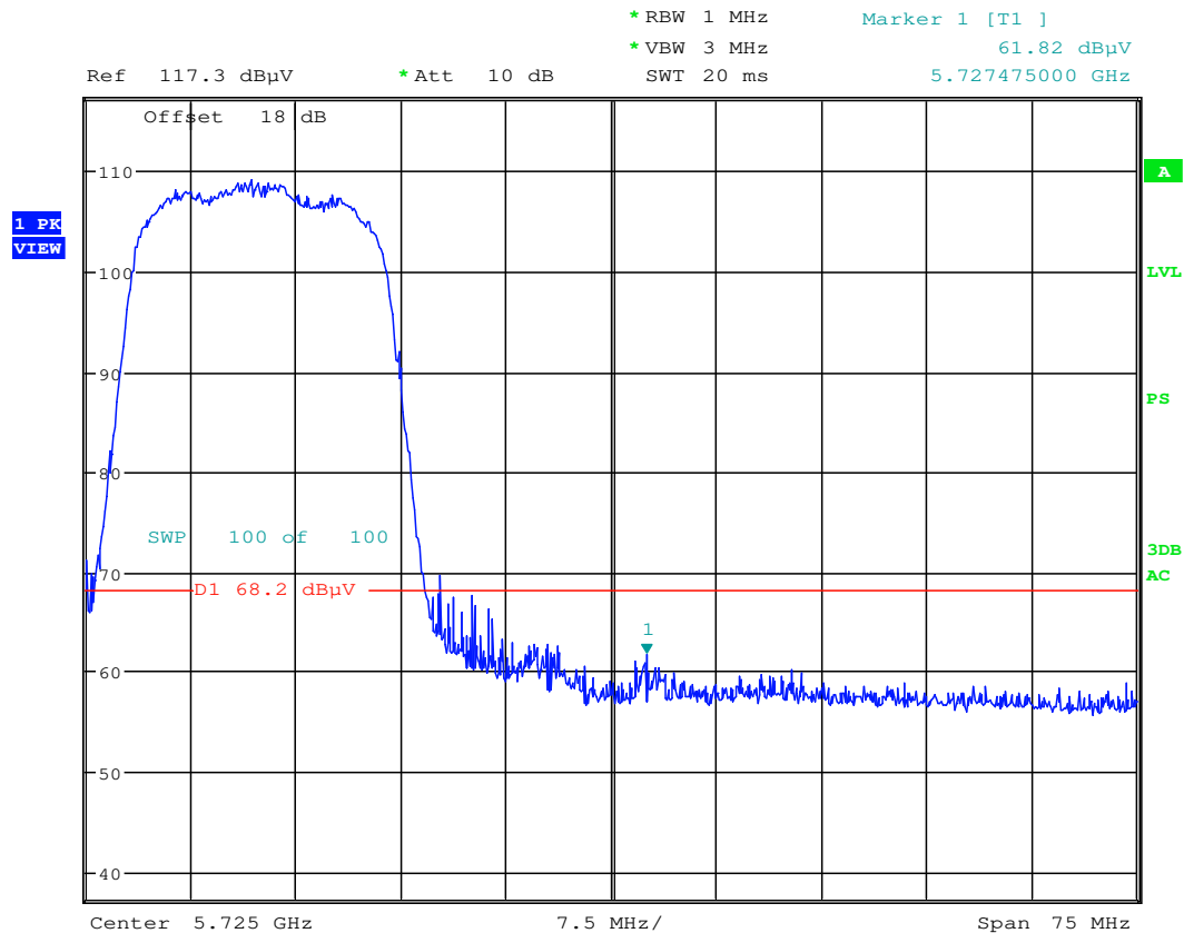
Plot 6-63. Radiated Upper Band Edge Plot (Peak – UNII Band 2C)
