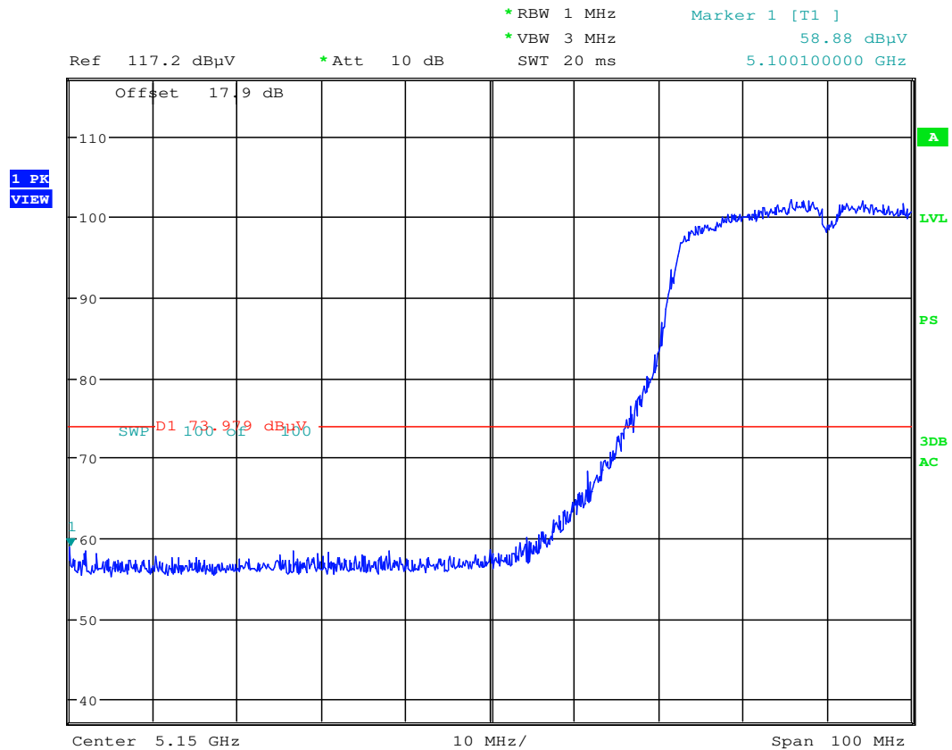
Plot 6-65. Radiated Restricted Lower Band Edge Plot (Peak – UNII Band 1)
