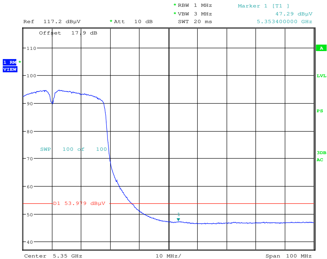
Plot 6-66. Radiated Restricted Upper Band Edge Plot (Average – UNII Band 2A)
