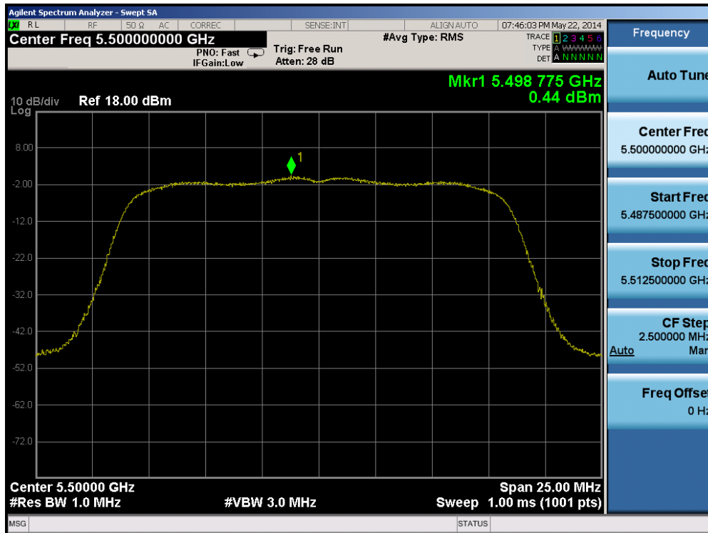
Plot 6-45. Peak Power Spectral Density Plot (802.11a (UNII Band 2C) – Ch. 100)
