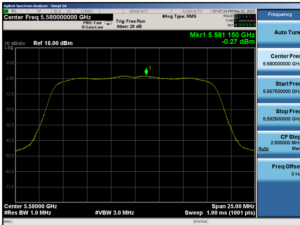
Plot 6-46. Peak Power Spectral Density Plot (802.11a (UNII Band 2C) – Ch. 116)
