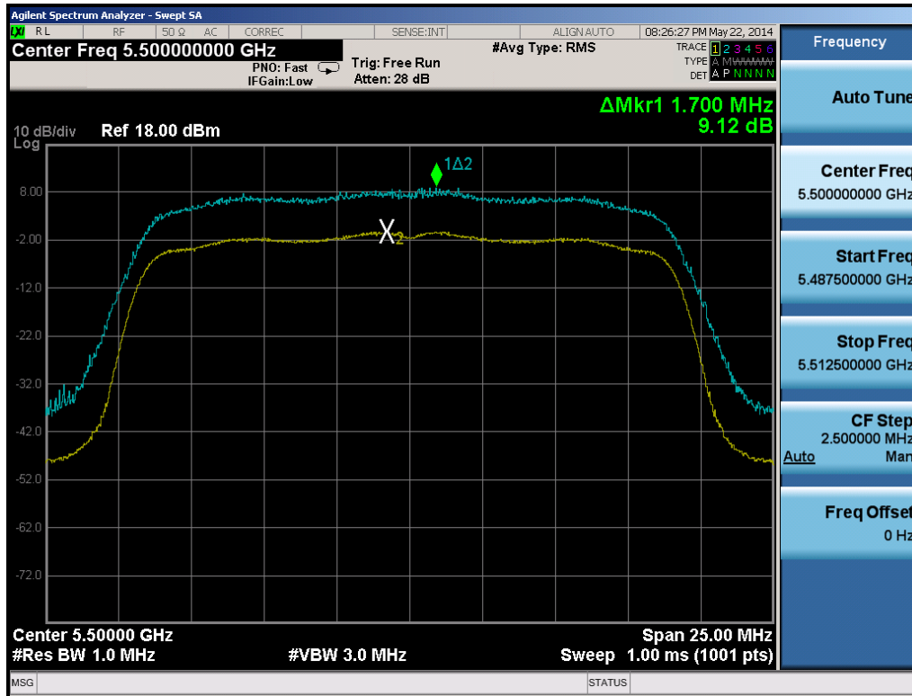
Plot 6-55. Peak Excursion Ratio Plot (20MHz BW 802.11n (UNII Band 2C) – Ch. 100)
