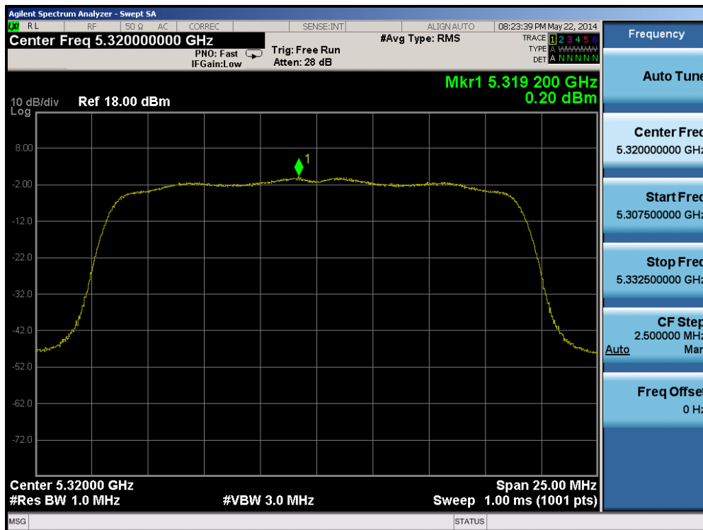
Plot 6-42. Peak Power Spectral Density Plot (20MHz BW 802.11n (UNII Band 2A) – Ch. 64)
