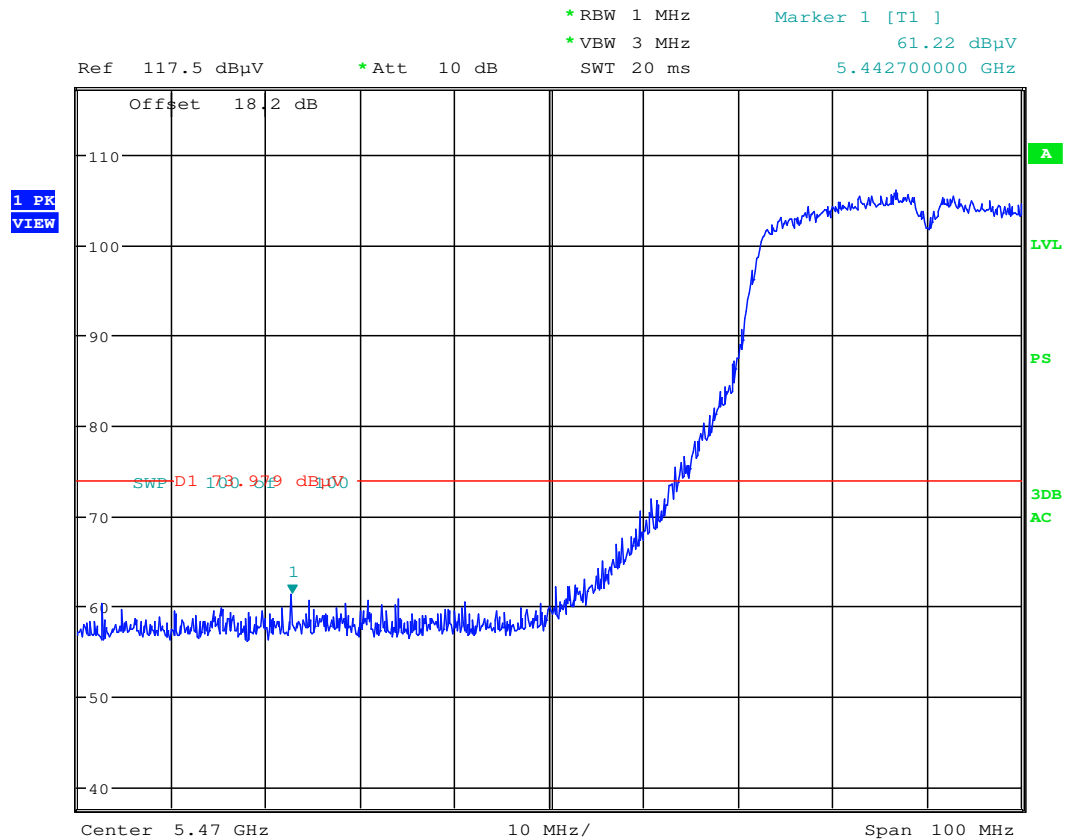
Plot 6-69. Radiated Restricted Lower Band Edge Plot (Peak – UNII Band 2C)
