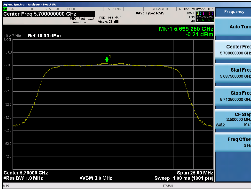
Plot 6-47. Peak Power Spectral Density Plot (802.11a (UNII Band 2C) – Ch. 140)
