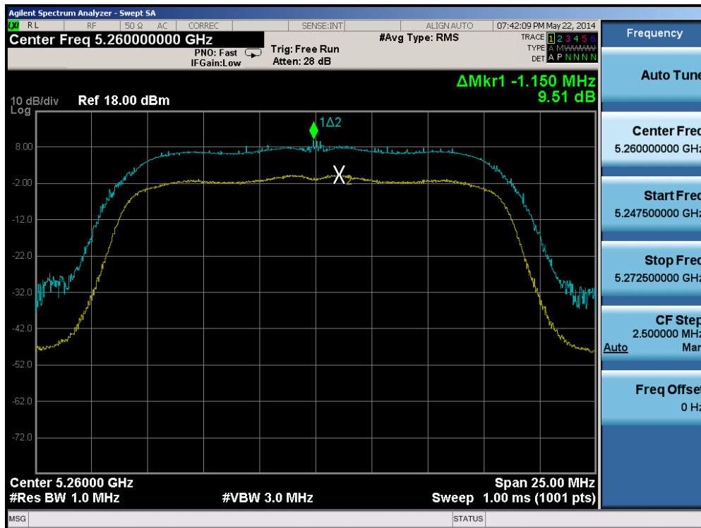
Plot 6-54. Peak Excursion Ratio Plot (802.11a (UNII Band 2A) – Ch. 52)
