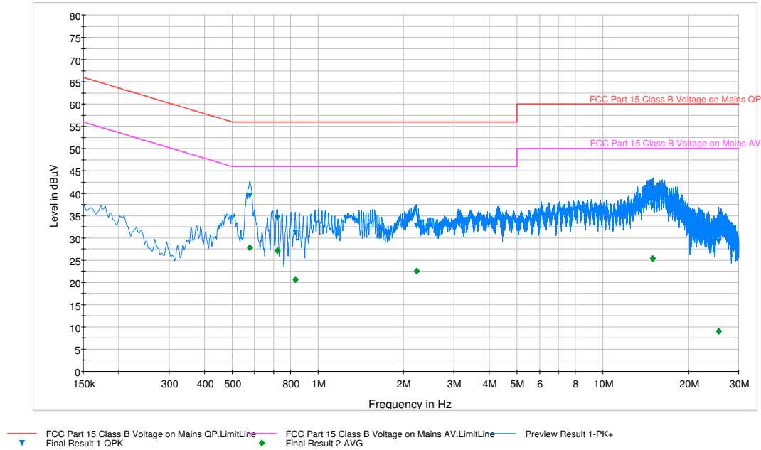
Plot 6-71. Line Conducted Plot with 802.11a UNII Band 1 (L1)
