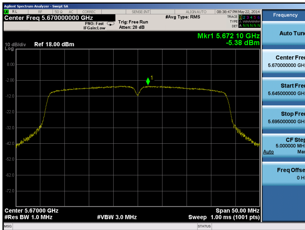
Plot 6-53. Peak Power Spectral Density Plot (40MHz BW 802.11n (UNII Band 2C) – Ch. 134)
