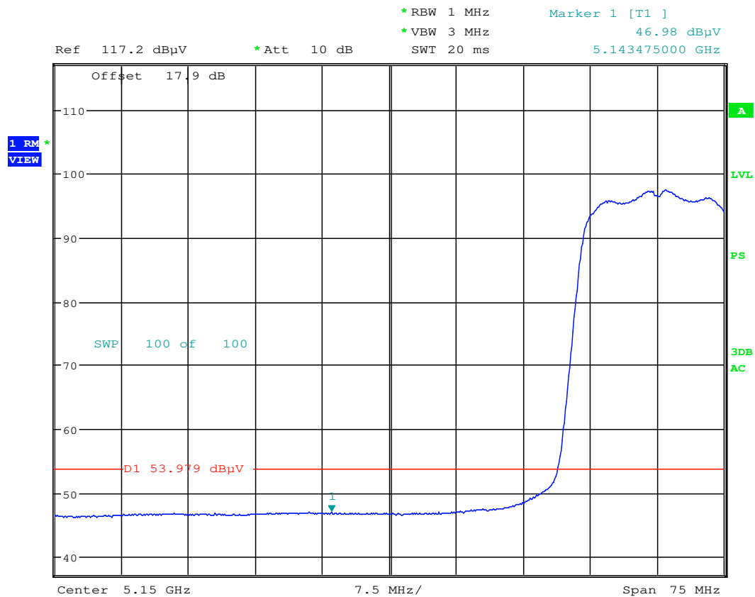
Plot 6-57. Radiated Restricted Lower Band Edge Plot (Average – UNII Band 1)
