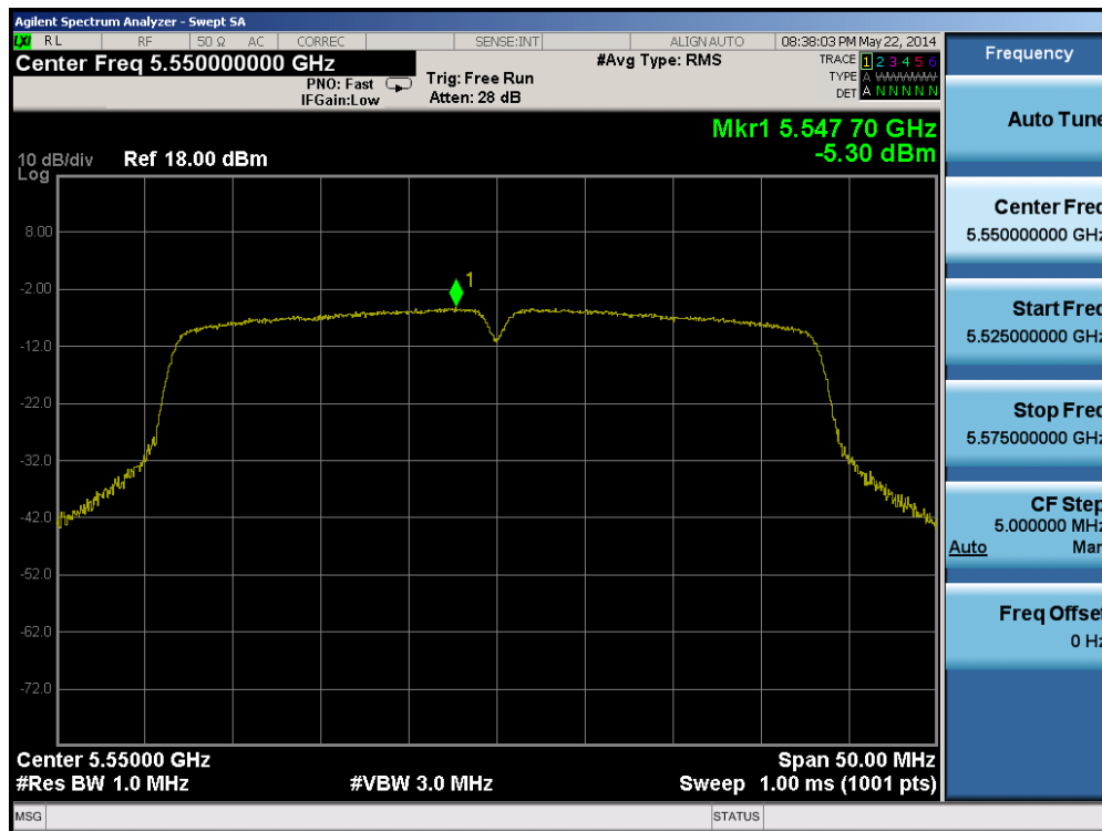
Plot 6-52. Peak Power Spectral Density Plot (40MHz BW 802.11n (UNII Band 2C) – Ch. 110)
