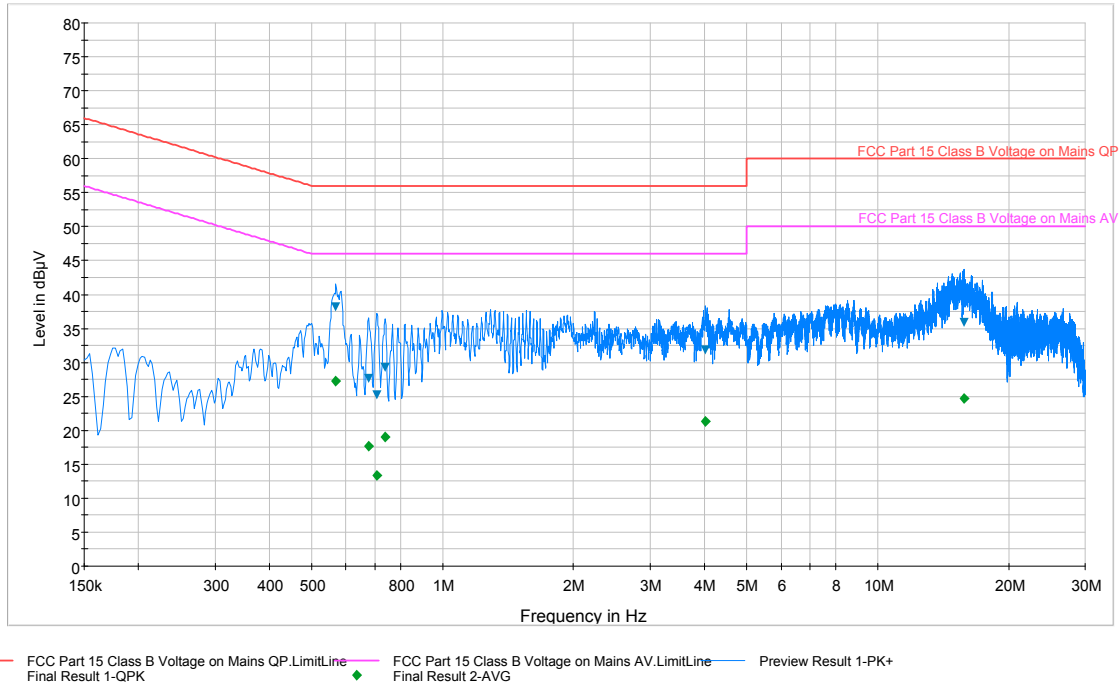
Plot 6-63. Line Conducted Plot with 802.11b (L1)
