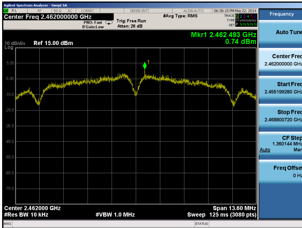
Plot 6-20. Power Spectral Density Plot (802.11b – Ch. 11)
