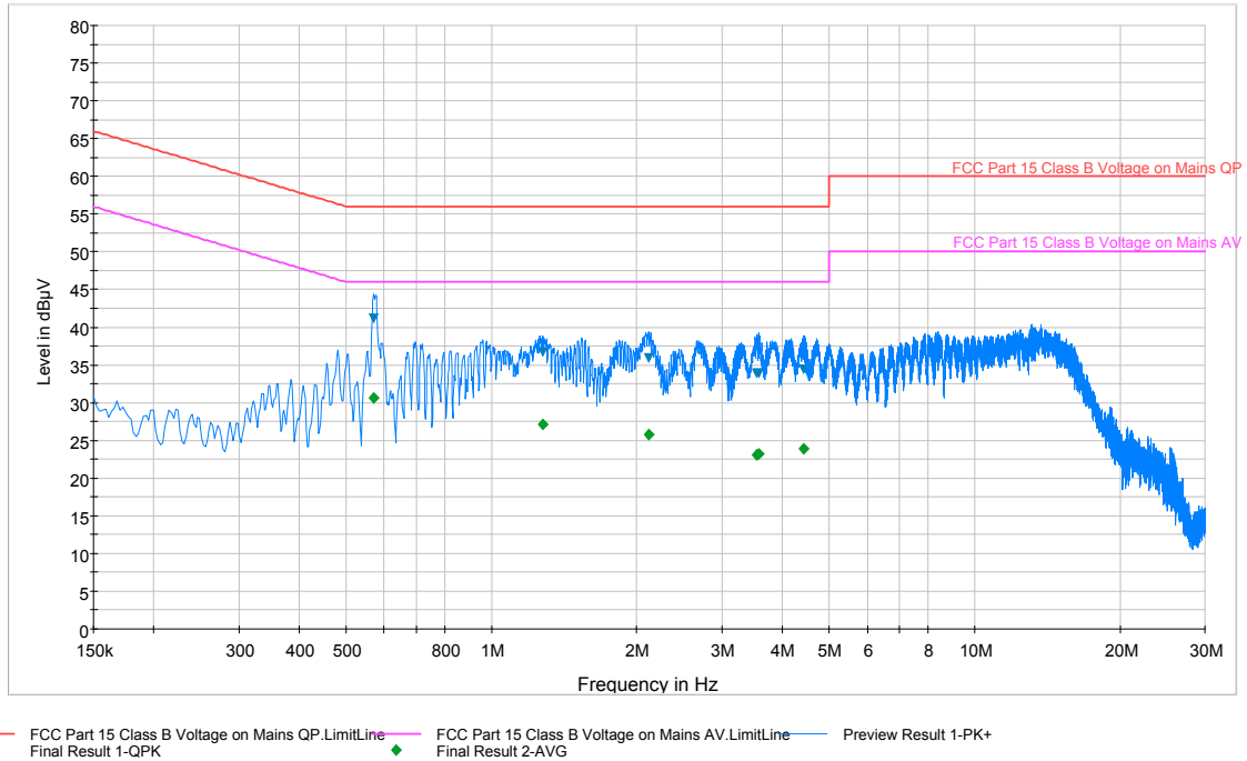
Plot 6-64. Line Conducted Plot with 802.11b (N)
