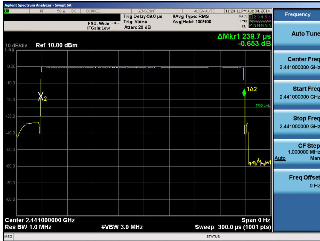
Plot 6-1. Pulse Width Measurement
