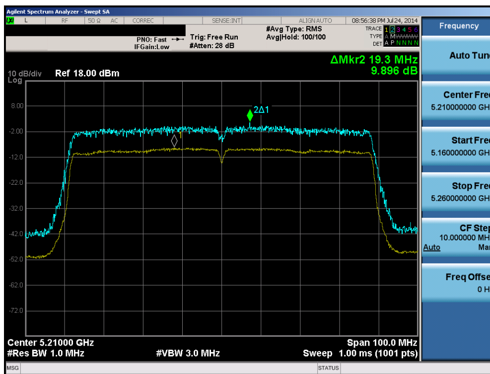
Plot 6-125. Peak Excursion Ratio Plot (80MHz BW 802.11ac (UNII Band 1) – Ch. 42)
