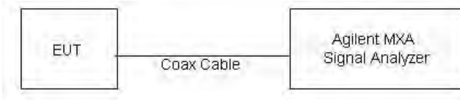
Figure 9-6 Power Measurement Setup for Bandwidths > 50 MHz
