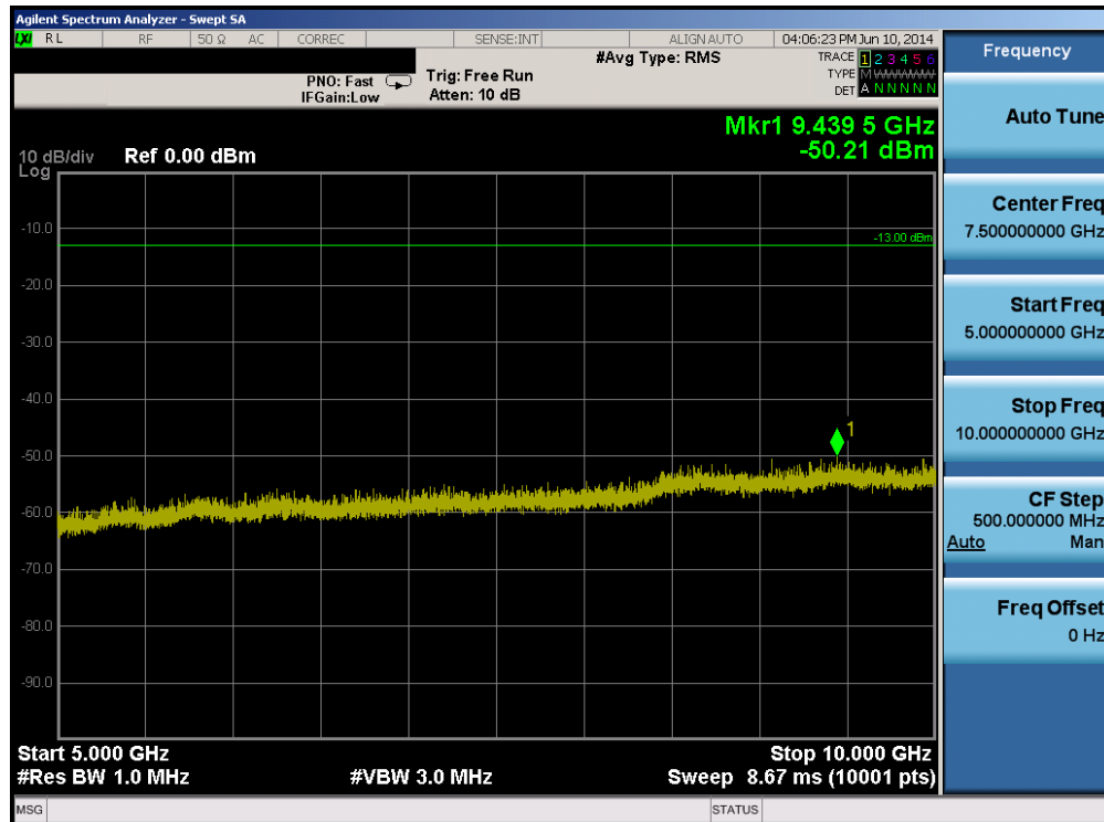
Plot 6-24. Conducted Spurious Plot (Band 5 – 5.0MHz QPSK – RB Size 1, RB Offset 0 – Mid Channel)
