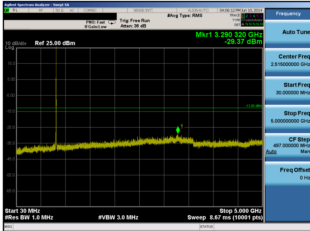
Plot 6-23. Conducted Spurious Plot (Band 5 – 5.0MHz QPSK – RB Size 1, RB Offset 0 – Mid Channel)
