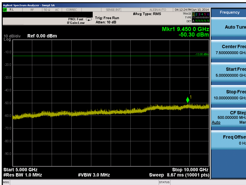
Plot 6-26. Conducted Spurious Plot (Band 5 – 5.0MHz QPSK – RB Size 1, RB Offset 0 – High Channel)
