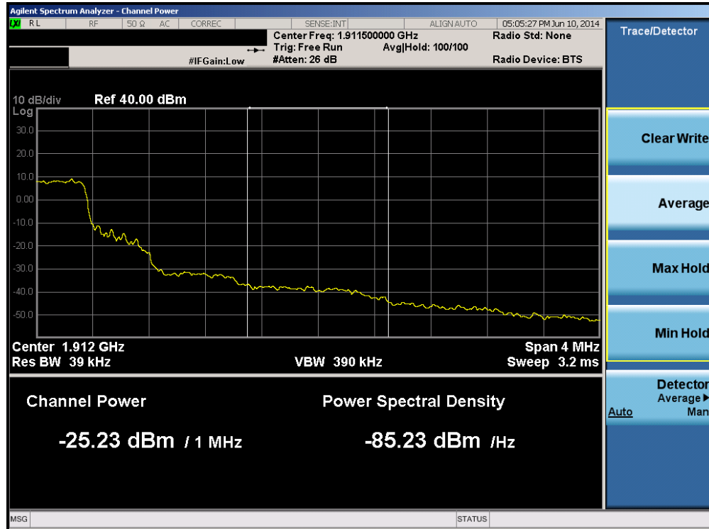
Plot 6-50. Upper Extended Band Edge Plot (Band 2 – 1.4MHz QPSK – RB Size 6)
