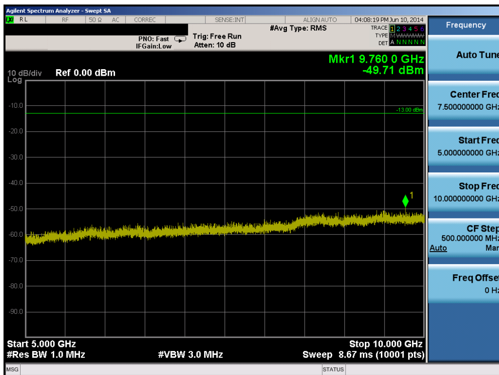
Plot 6-22. Conducted Spurious Plot (Band 5 – 5.0MHz QPSK – RB Size 1, RB Offset 0 – Low Channel)
