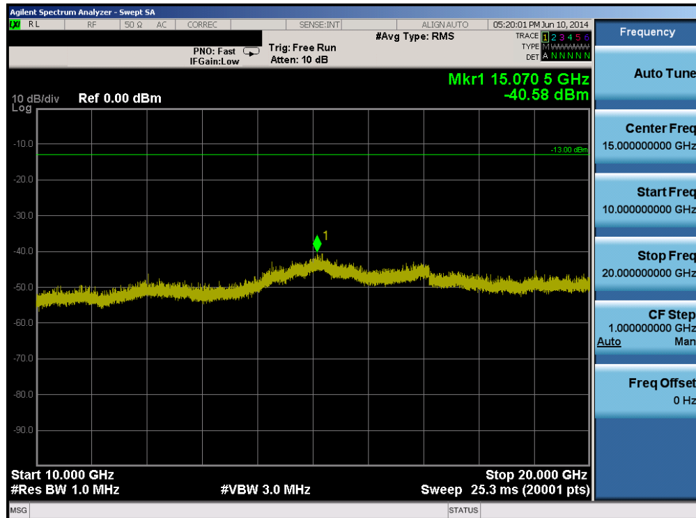
Plot 6-32. Conducted Spurious Plot (Band 2 – 10.0MHz QPSK – RB Size 1, RB Offset 0 – High Channel)
