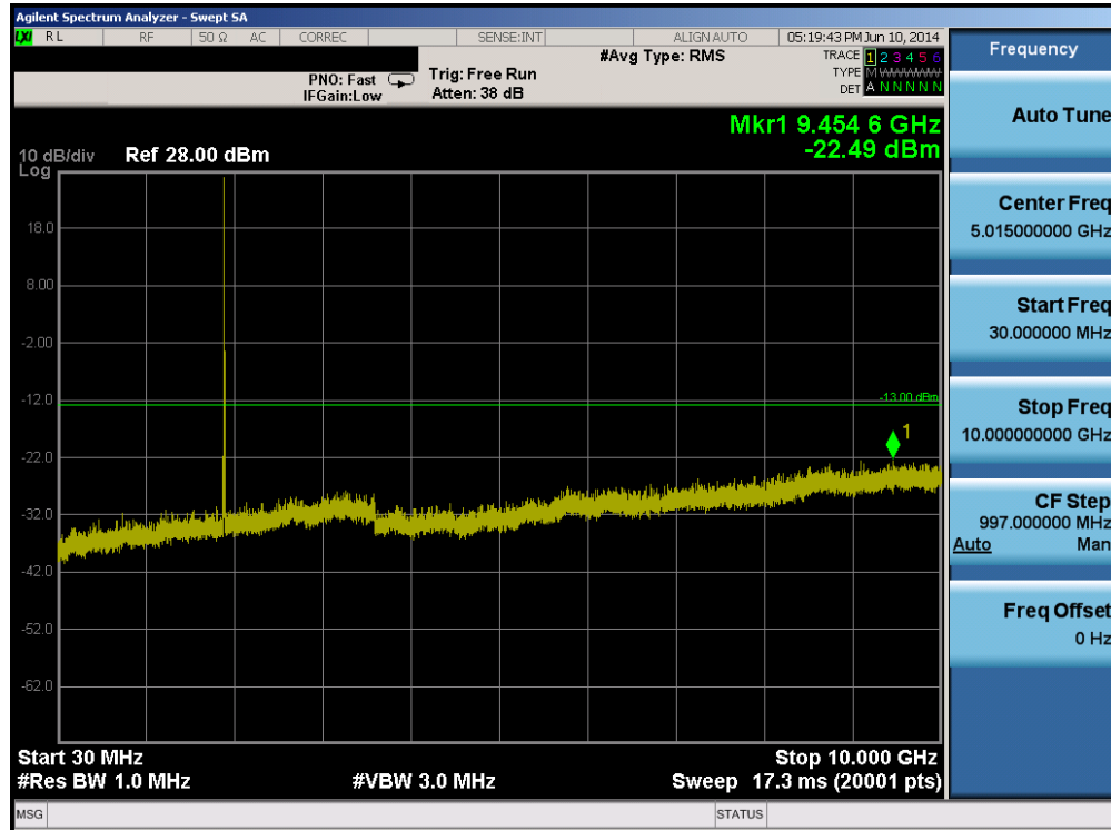
Plot 6-31. Conducted Spurious Plot (Band 2 – 10.0MHz QPSK – RB Size 1, RB Offset 0 – High Channel)
