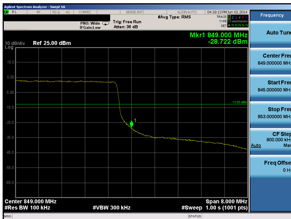
Plot 6-46. Upper Band Edge Plot (Band 5 – 10.0MHz QPSK – RB Size 50)
