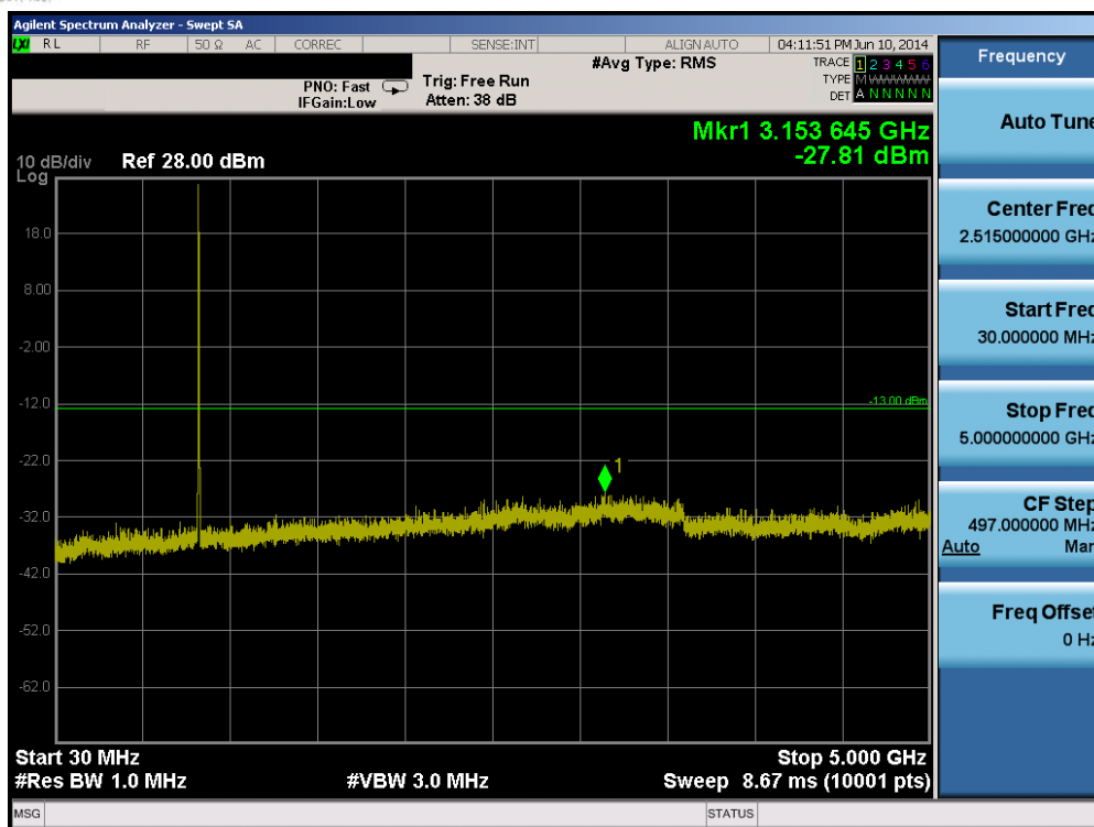
Plot 6-25. Conducted Spurious Plot (Band 5 – 5.0MHz QPSK – RB Size 1, RB Offset 0 – High Channel)
