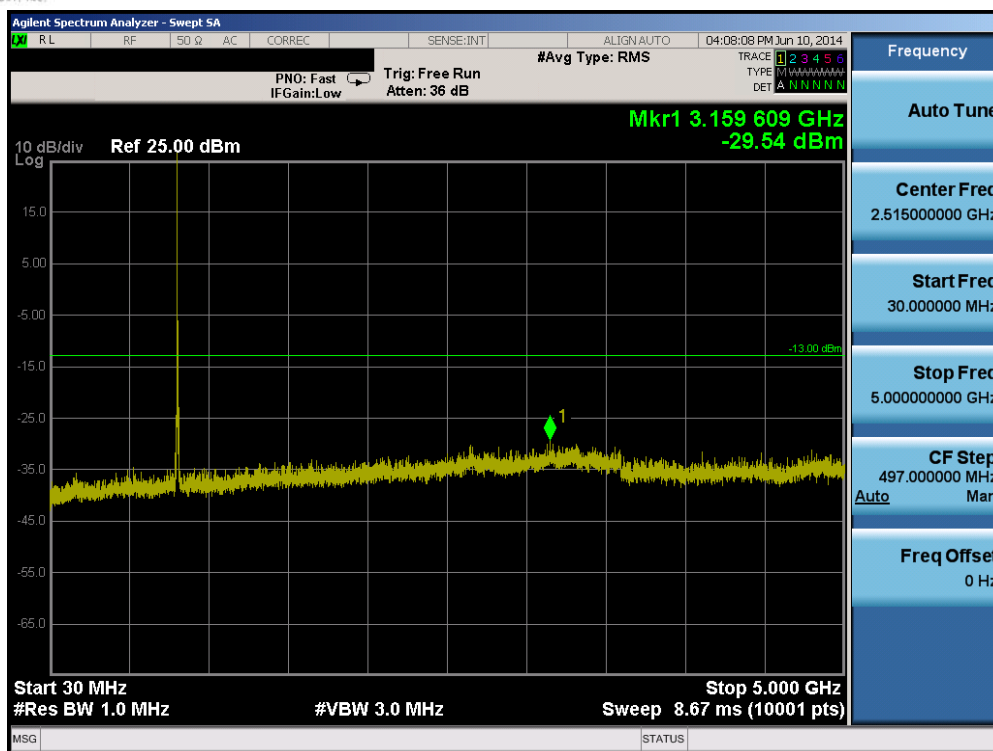
Plot 6-21. Conducted Spurious Plot (Band 5 – 5.0MHz QPSK – RB Size 1, RB Offset 0 – Low Channel)
