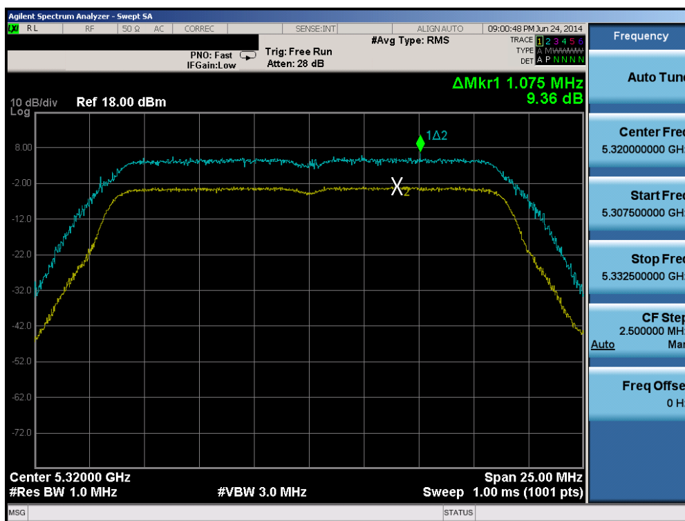
Plot 6-125. Peak Excursion Ratio Plot (20MHz BW 802.11n (UNII Band 2A) – Ch. 64)
