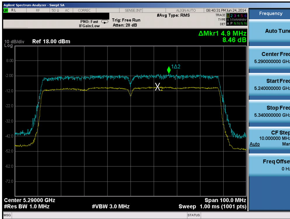
Plot 6-130. Peak Excursion Ratio Plot (80MHz BW 802.11ac (UNII Band 2A) – Ch. 58)
