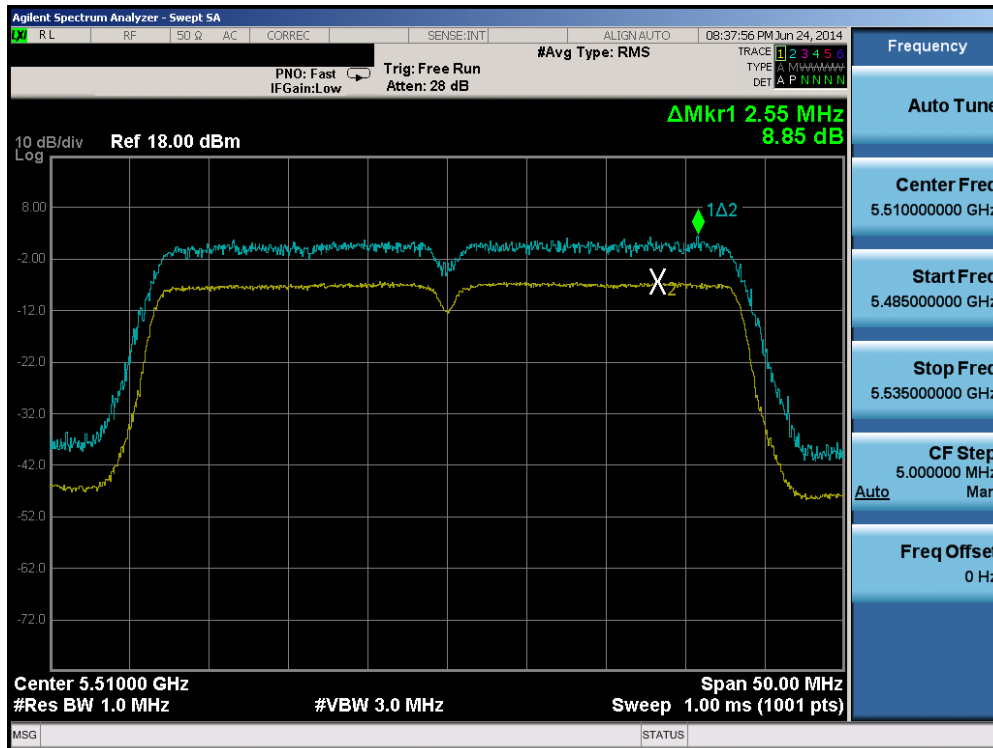
Plot 6-132. Peak Excursion Ratio Plot (40MHz BW 802.11n (UNII Band 2C) – Ch. 102)
