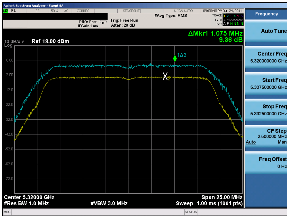
Plot 6-125. Peak Excursion Ratio Plot (20MHz BW 802.11n (UNII Band 2A) – Ch. 64)
