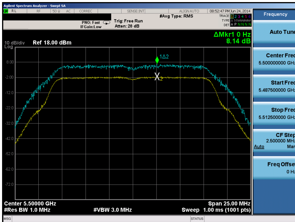
Plot 6-127. Peak Excursion Ratio Plot (802.11a (UNII Band 2C) – Ch. 100)
