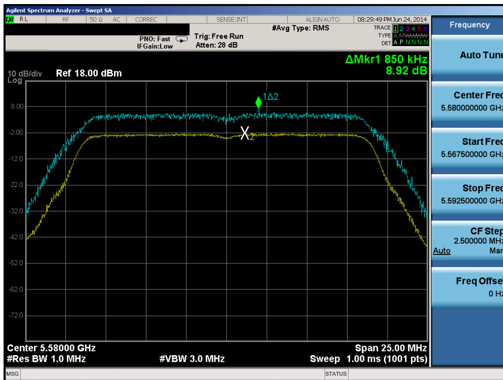
Plot 6-131. Peak Excursion Ratio Plot (20MHz BW 802.11n (UNII Band 2C) – Ch. 116)
