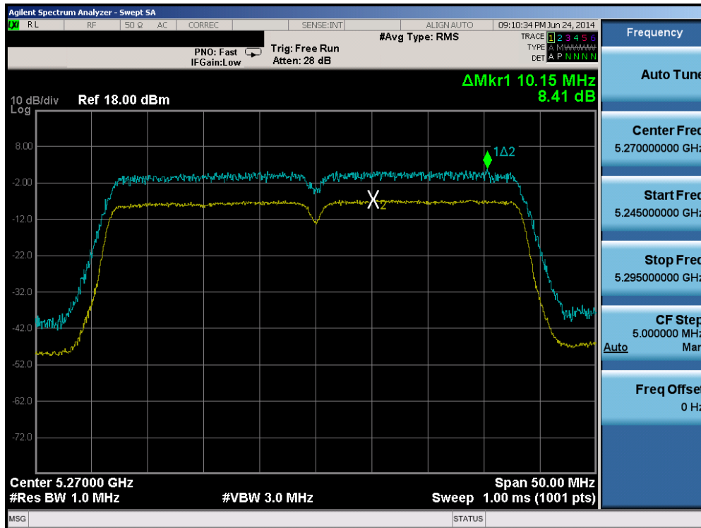
Plot 6-126. Peak Excursion Ratio Plot (40MHz BW 802.11n (UNII Band 2A) – Ch. 54)
