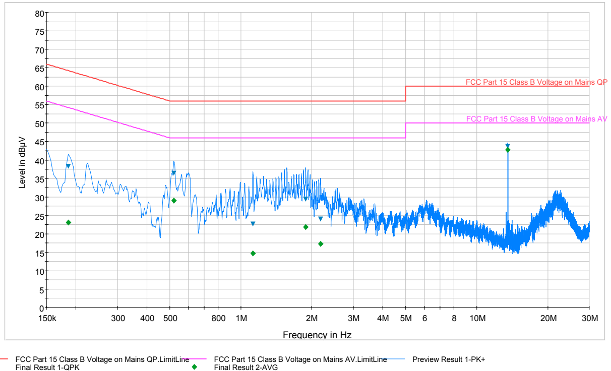
Plot 8-1. Line-Conducted Test Plot (L1)
