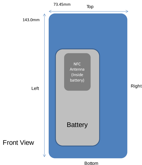
Figure 1-2 NFC Antenna Locations
