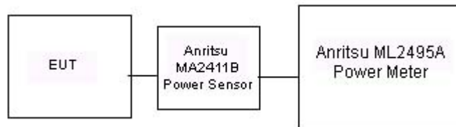
Figure 9-8 Power Measurement Setup for Bandwidths < 50 MHz
