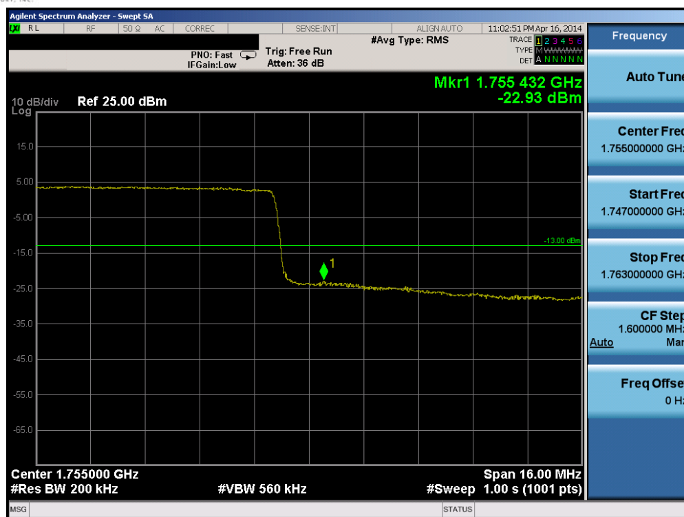
Plot 6-191. Upper Band Edge Plot (Band 4 - 20.0MHz QPSK - RB Size 100)
