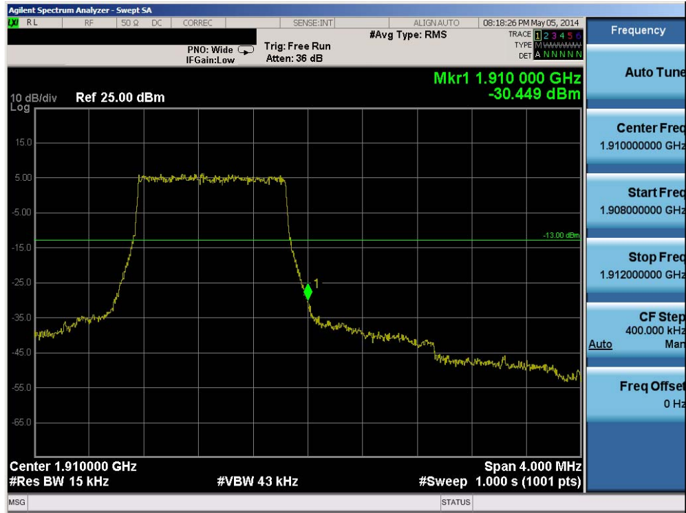
Plot 6-195. Upper Band Edge Plot (Band 2 – 1.4MHz QPSK – RB Size 6)
