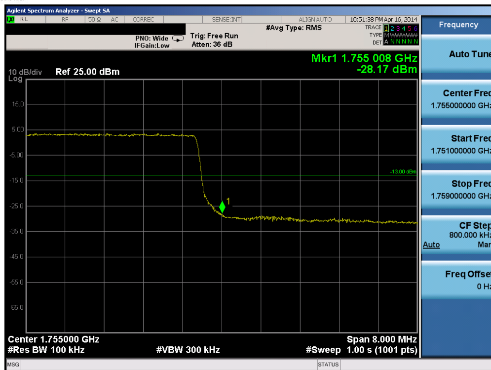
Plot 6-183. Upper Band Edge Plot (Band 4 - 10.0MHz QPSK - RB Size 50)
