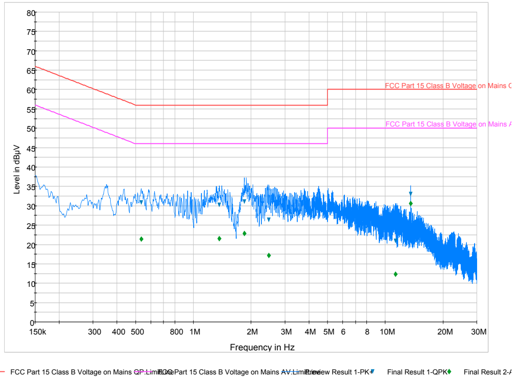
Plot 8-1. Line-Conducted Test Plot (L1)
