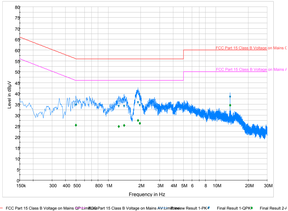
Plot 8-2. Line-Conducted Test Plot (N)
