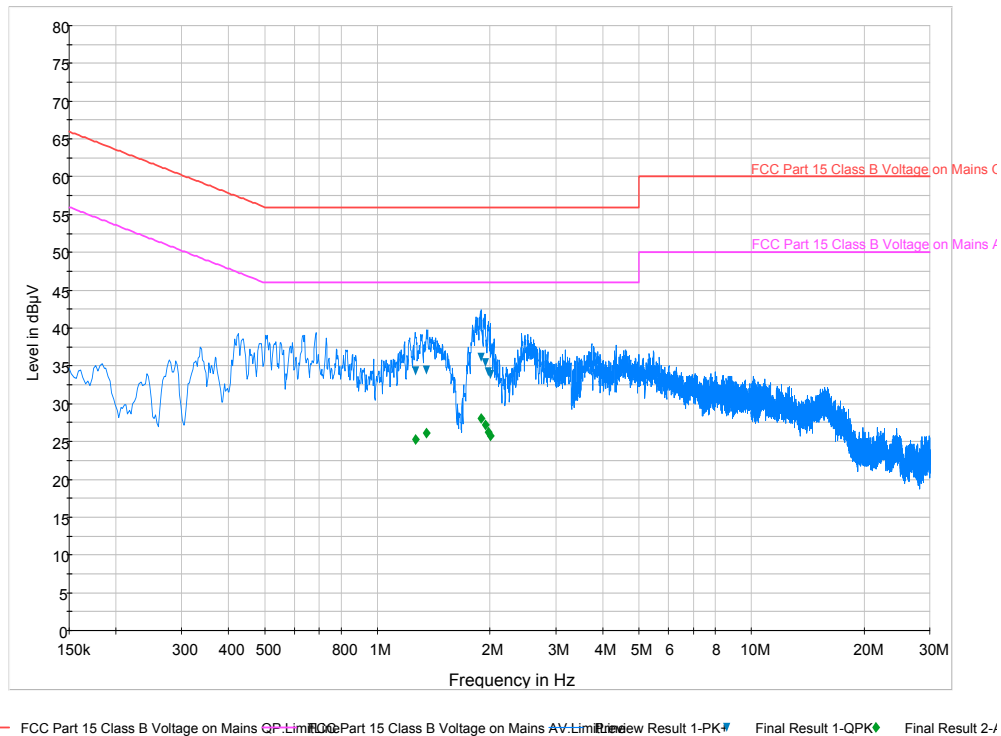
Plot 6-7. Line-Conducted Test Plot (N)
