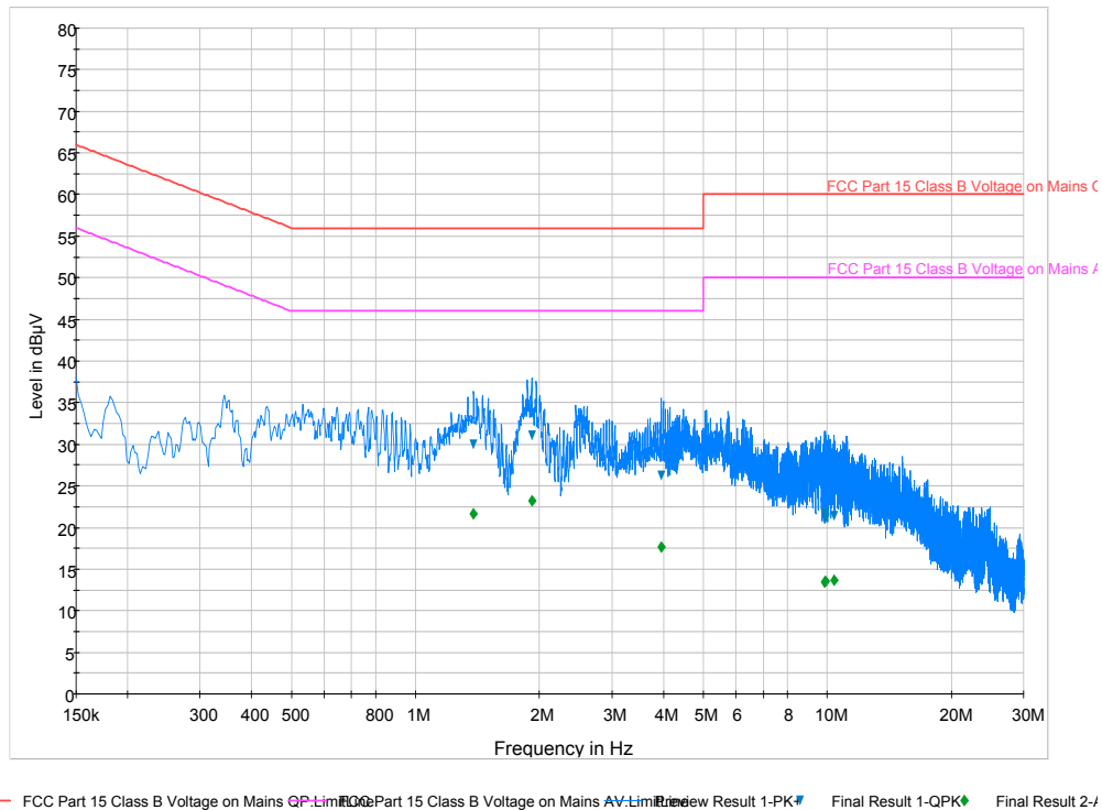
Plot 6-6. Line-Conducted Test Plot (L1)
