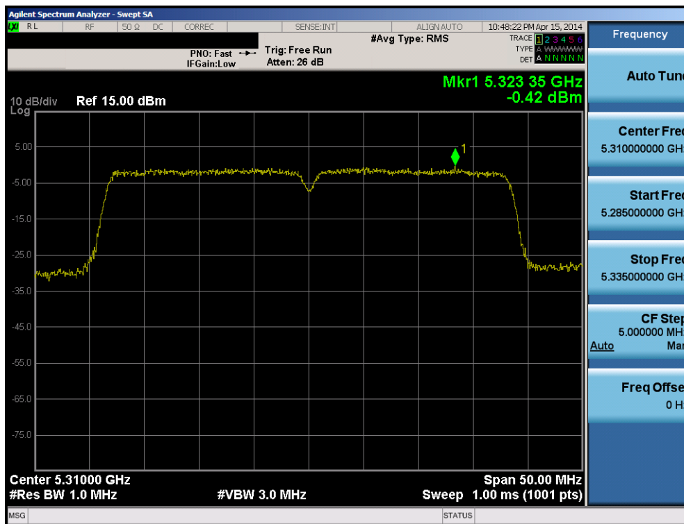
Plot 6-113. Peak Power Spectral Density Plot (40MHz BW 802.11n (UNII Band 2A) – Ch. 62)
