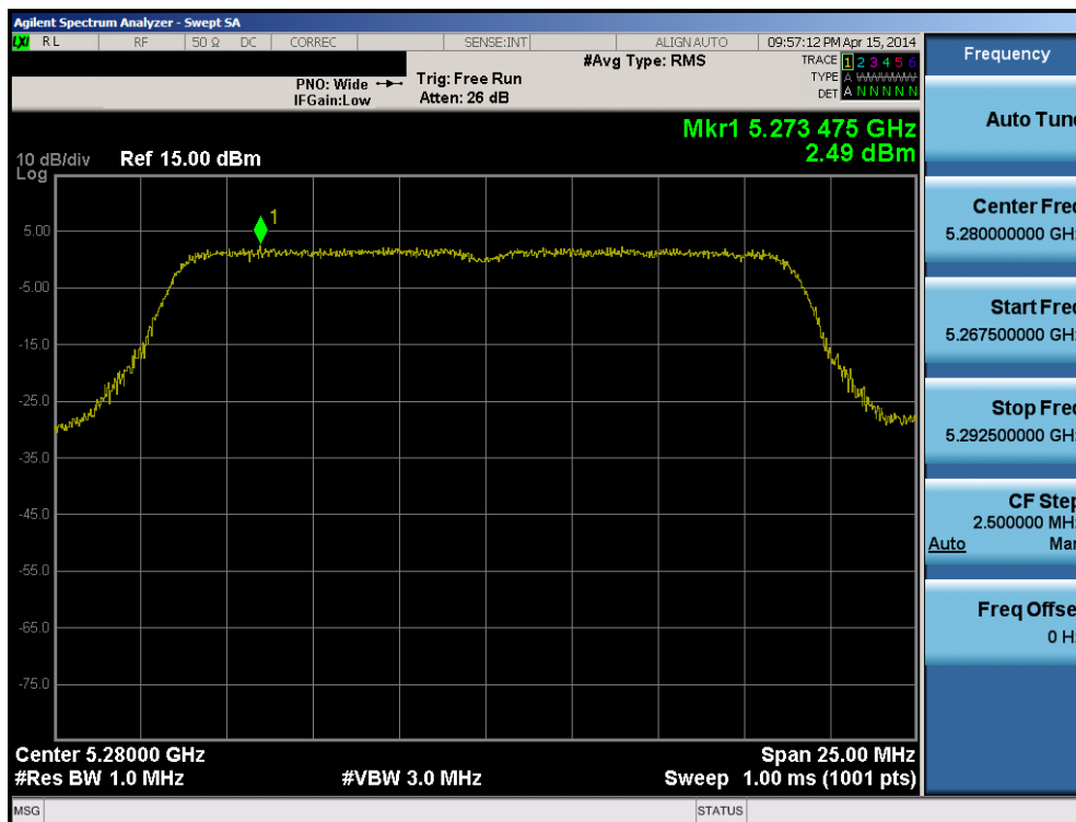
Plot 6-82. Peak Power Spectral Density Plot (20MHz BW 802.11n (UNII Band 2A) – Ch. 56)
