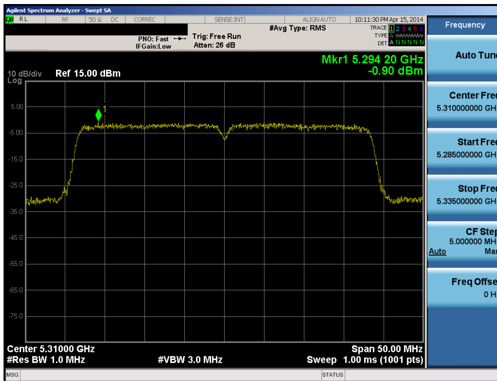
Plot 6-85. Peak Power Spectral Density Plot (40MHz BW 802.11n (UNII Band 2A) – Ch. 62)
