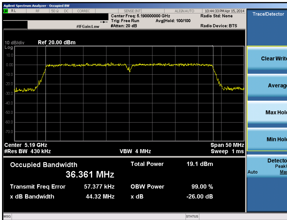
Plot 6-41. 26dB Bandwidth Plot (40MHz BW 802.11n (UNII Band 1) – Ch. 38)
