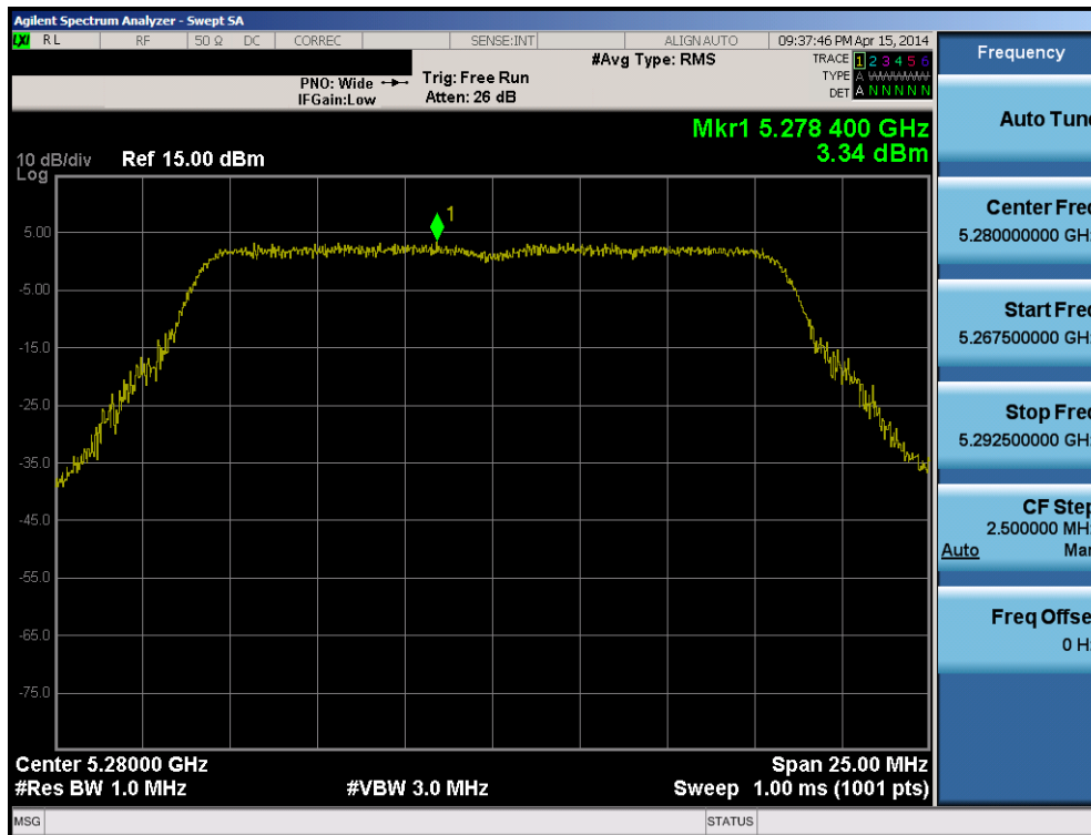
Plot 6-79. Peak Power Spectral Density Plot (802.11a (UNII Band 2A) – Ch. 56)
