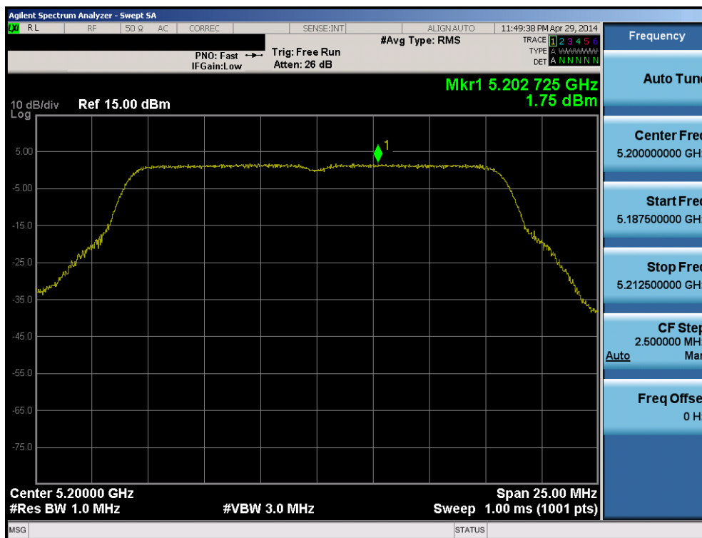
Plot 6-98. Peak Power Spectral Density Plot (802.11a (UNII Band 1) – Ch. 40)
