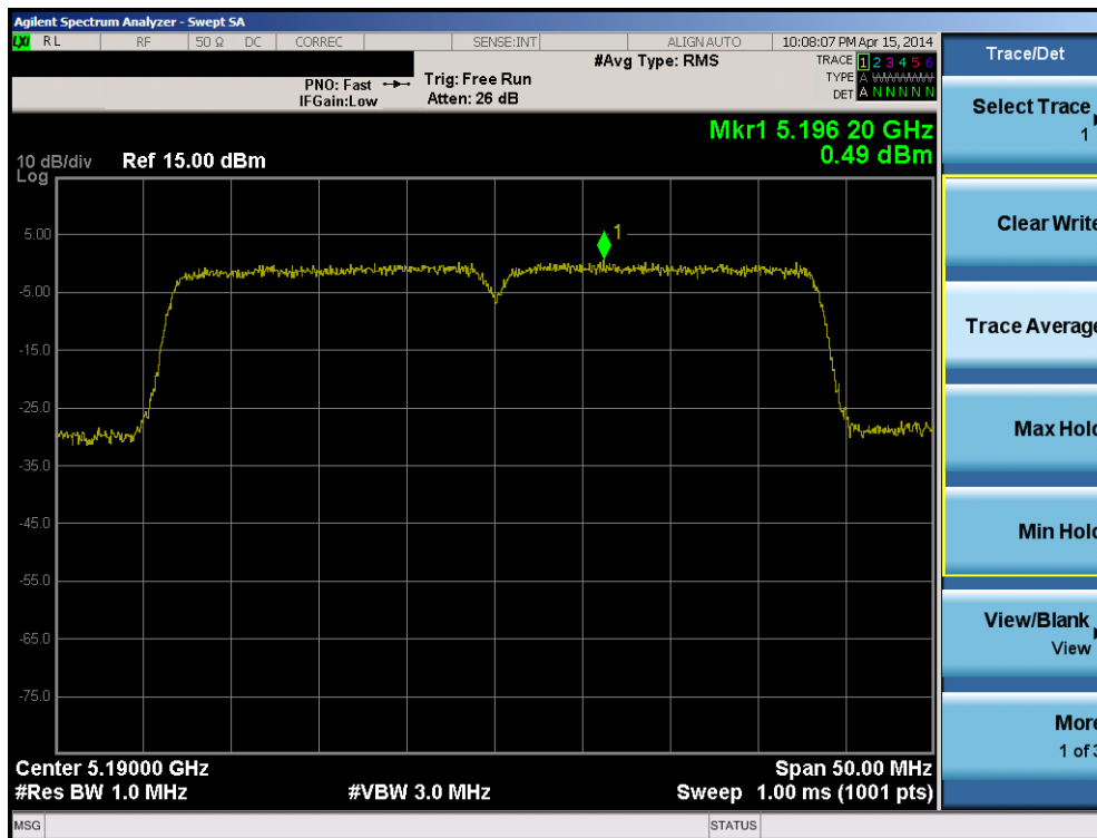
Plot 6-75. Peak Power Spectral Density Plot (40MHz BW 802.11n (UNII Band 1) – Ch. 38)
