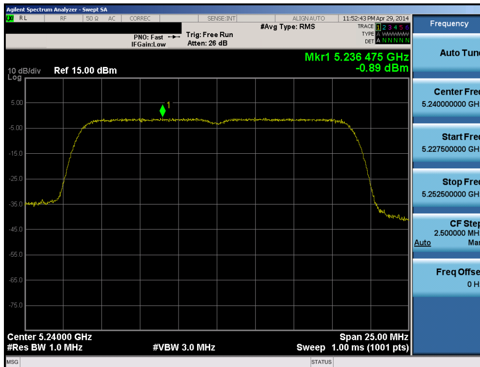
Plot 6-102. Peak Power Spectral Density Plot (20MHz BW 802.11n (UNII Band 1) – Ch. 48)
