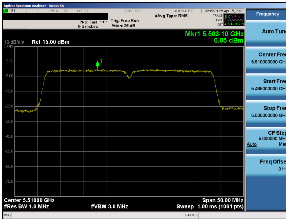
Plot 6-121. Peak Power Spectral Density Plot (40MHz BW 802.11n (UNII Band 2C) – Ch. 102)
