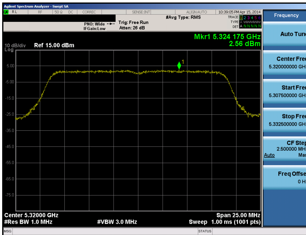
Plot 6-111. Peak Power Spectral Density Plot (20MHz BW 802.11n (UNII Band 2A) – Ch. 64)
