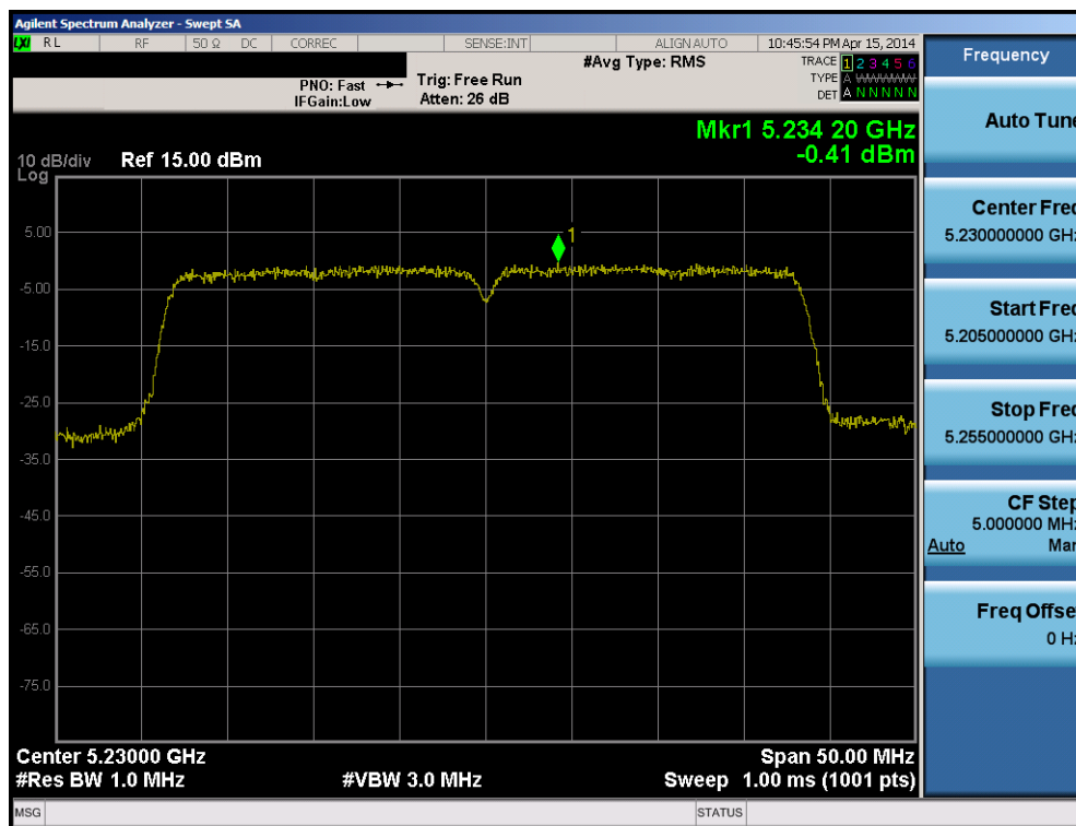
Plot 6-104. Peak Power Spectral Density Plot (40MHz BW 802.11n (UNII Band 1) – Ch. 46)
