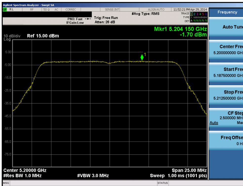
Plot 6-101. Peak Power Spectral Density Plot (20MHz BW 802.11n (UNII Band 1) – Ch. 40)
