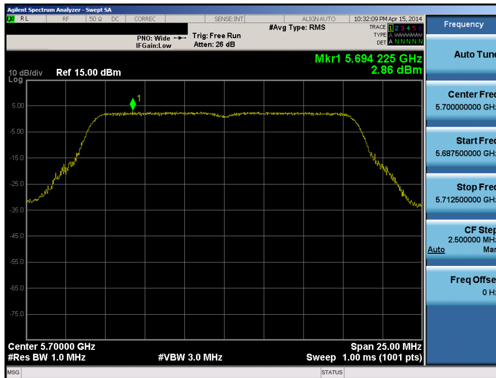
Plot 6-117. Peak Power Spectral Density Plot (802.11a (UNII Band 2C) – Ch. 140)
