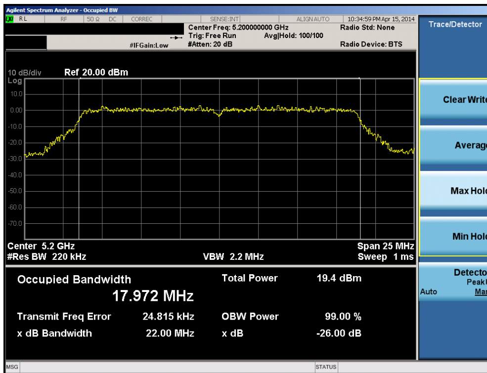
Plot 6-39. 26dB Bandwidth Plot (20MHz BW 802.11n (UNII Band 1) – Ch. 40)
