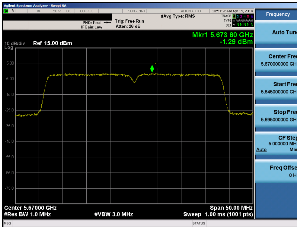
Plot 6-123. Peak Power Spectral Density Plot (40MHz BW 802.11n (UNII Band 2C) – Ch. 134)
