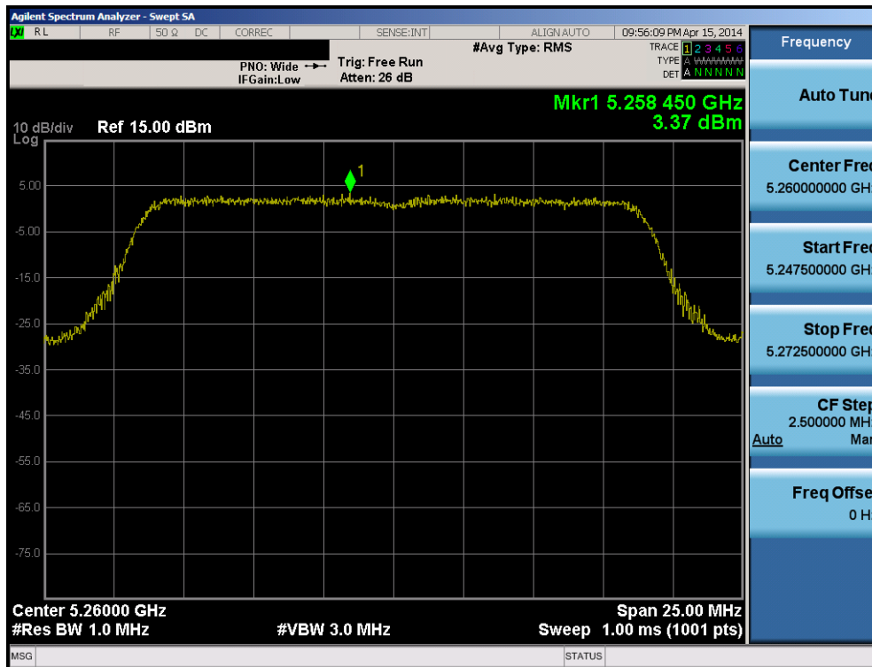
Plot 6-81. Peak Power Spectral Density Plot (20MHz BW 802.11n (UNII Band 2A) – Ch. 52)
