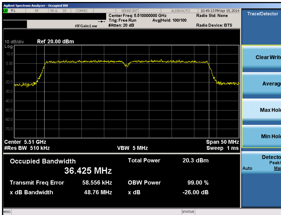
Plot 6-59. 26dB Bandwidth Plot (40MHz BW 802.11n (UNII Band 2C) – Ch. 102)
