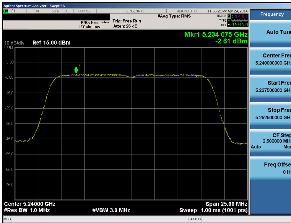
Plot 6-71. Peak Power Spectral Density Plot (802.11a (UNII Band 1) – Ch. 48)
