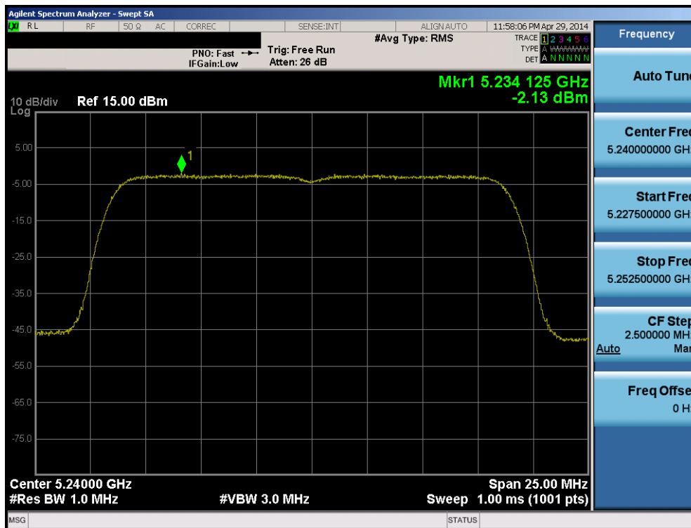
Plot 6-74. Peak Power Spectral Density Plot (20MHz BW 802.11n (UNII Band 1) – Ch. 48)
