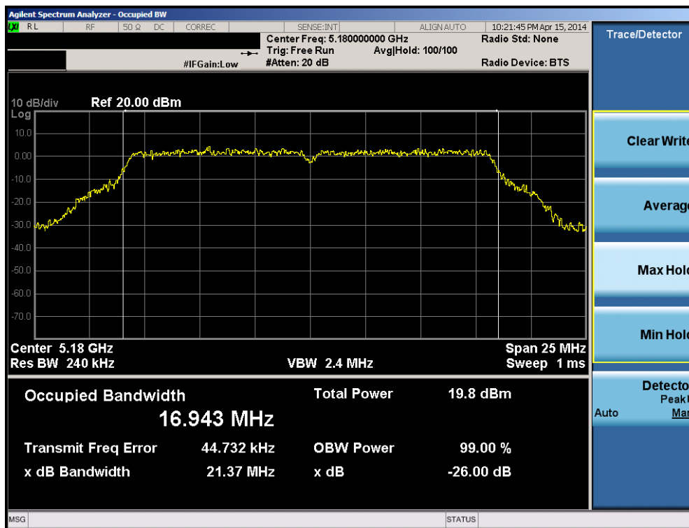
Plot 6-35. 26dB Bandwidth Plot (802.11a (UNII Band 1) – Ch. 36)
