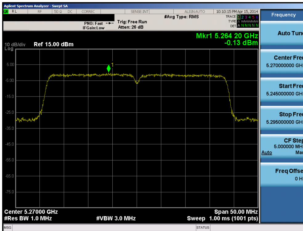
Plot 6-84. Peak Power Spectral Density Plot (40MHz BW 802.11n (UNII Band 2A) – Ch. 54)
