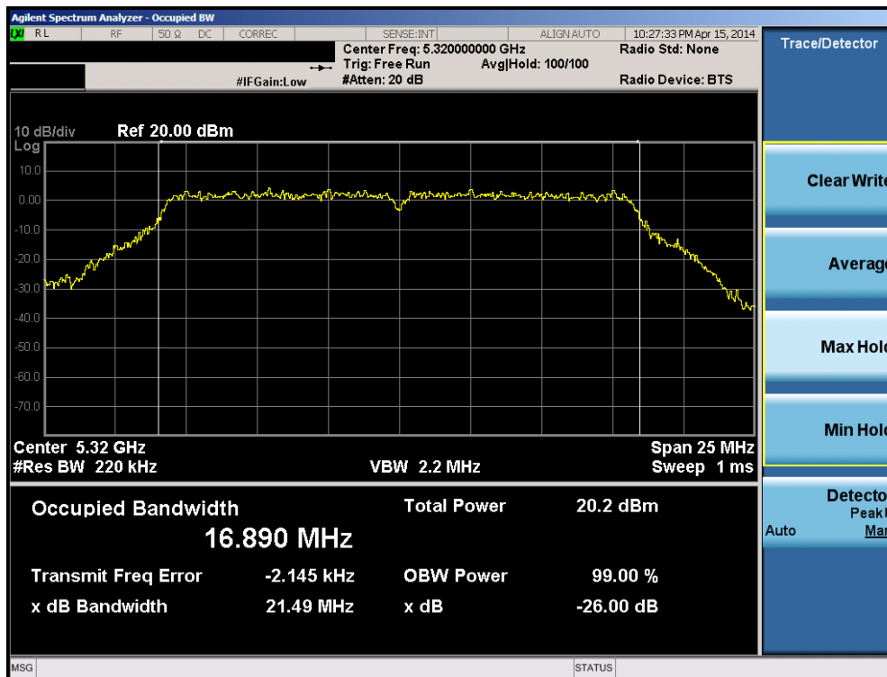
Plot 6-46. 26dB Bandwidth Plot (802.11a (UNII Band 2A) – Ch. 64)
