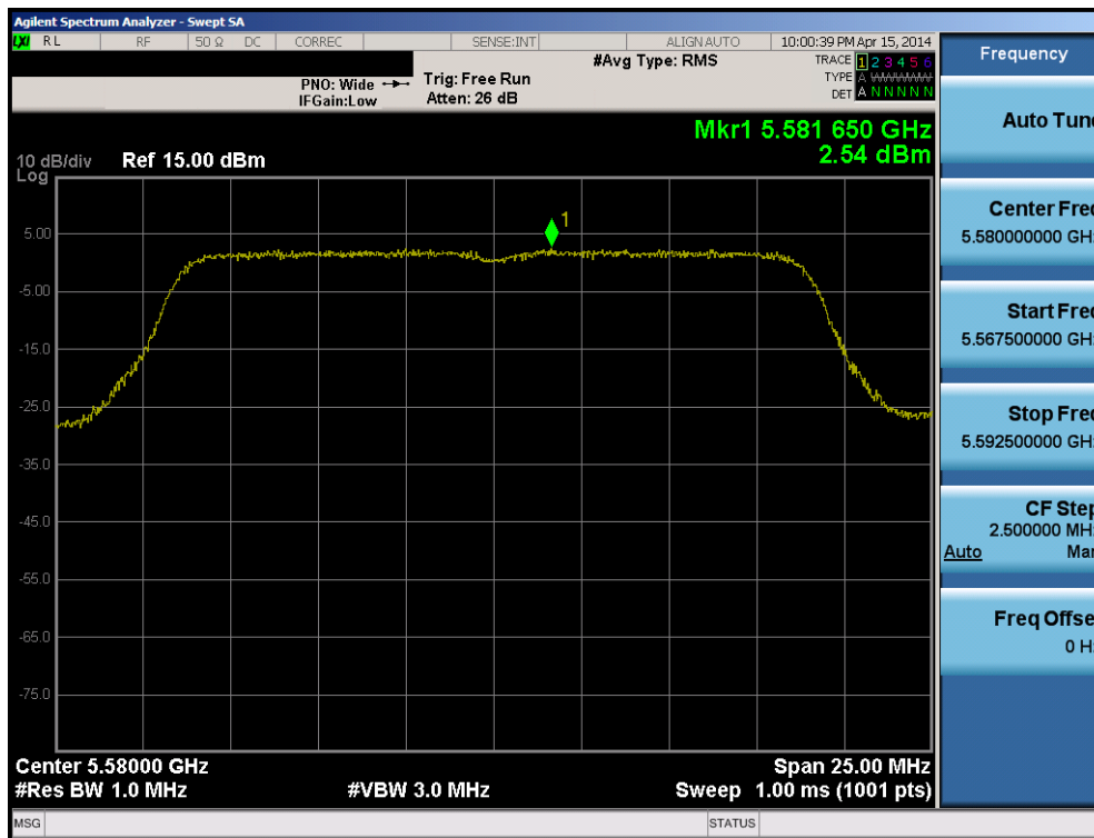
Plot 6-91. Peak Power Spectral Density Plot (20MHz BW 802.11n (UNII Band 2C) – Ch. 116)
