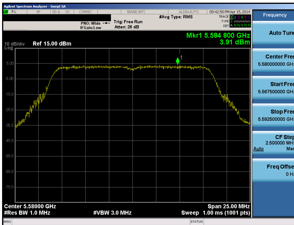
Plot 6-88. Peak Power Spectral Density Plot (802.11a (UNII Band 2C) – Ch. 116)
