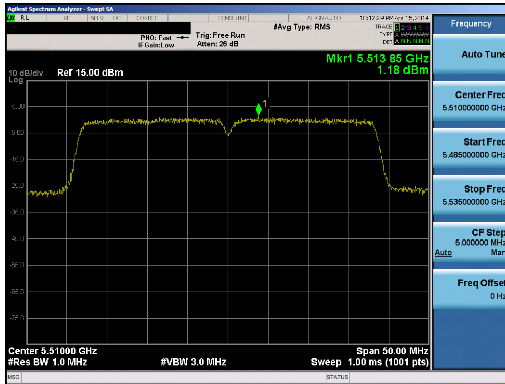
Plot 6-93. Peak Power Spectral Density Plot (40MHz BW 802.11n (UNII Band 2C) – Ch. 102)
