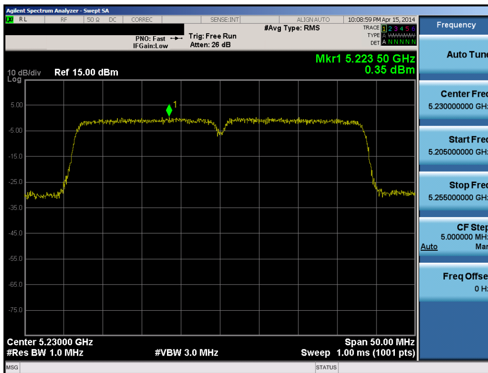
Plot 6-76. Peak Power Spectral Density Plot (40MHz BW 802.11n (UNII Band 1) – Ch. 46)
