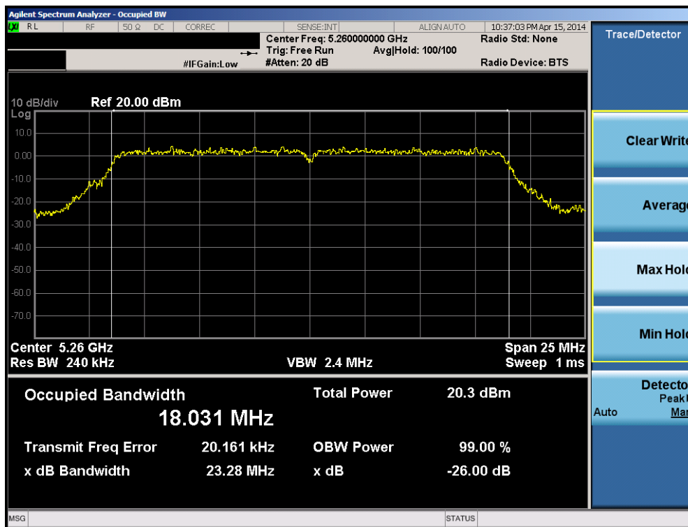
Plot 6-47. 26dB Bandwidth Plot (20MHz BW 802.11n (UNII Band 2A) – Ch. 52)
