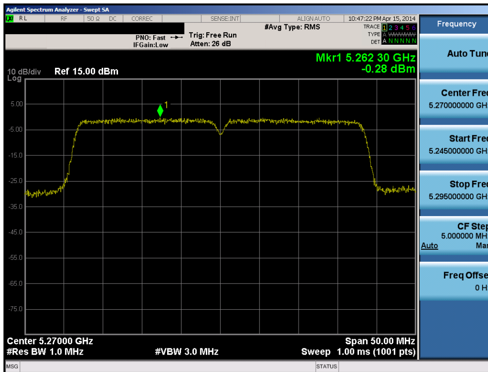
Plot 6-112. Peak Power Spectral Density Plot (40MHz BW 802.11n (UNII Band 2A) – Ch. 54)
