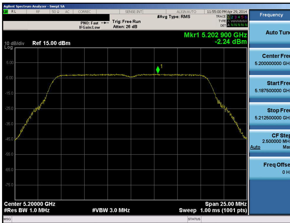
Plot 6-70. Peak Power Spectral Density Plot (802.11a (UNII Band 1) – Ch. 40)
