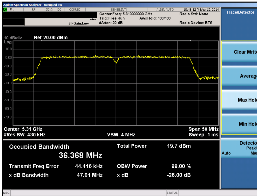
Plot 6-51. 26dB Bandwidth Plot (40MHz BW 802.11n (UNII Band 2A) – Ch. 62)
