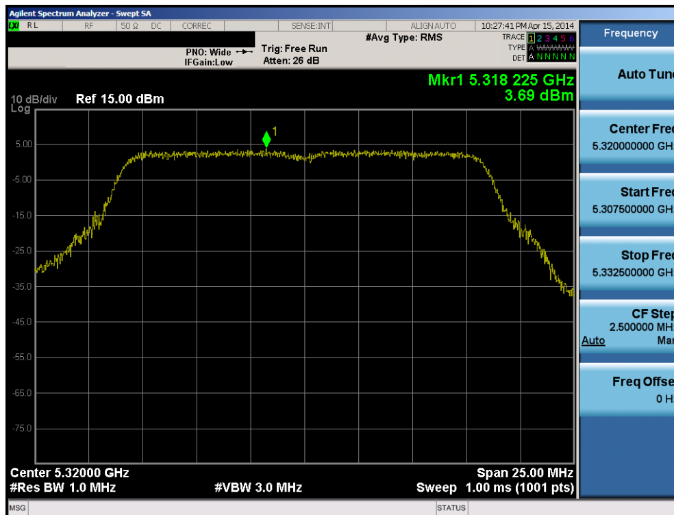
Plot 6-108. Peak Power Spectral Density Plot (802.11a (UNII Band 2A) – Ch. 64)
