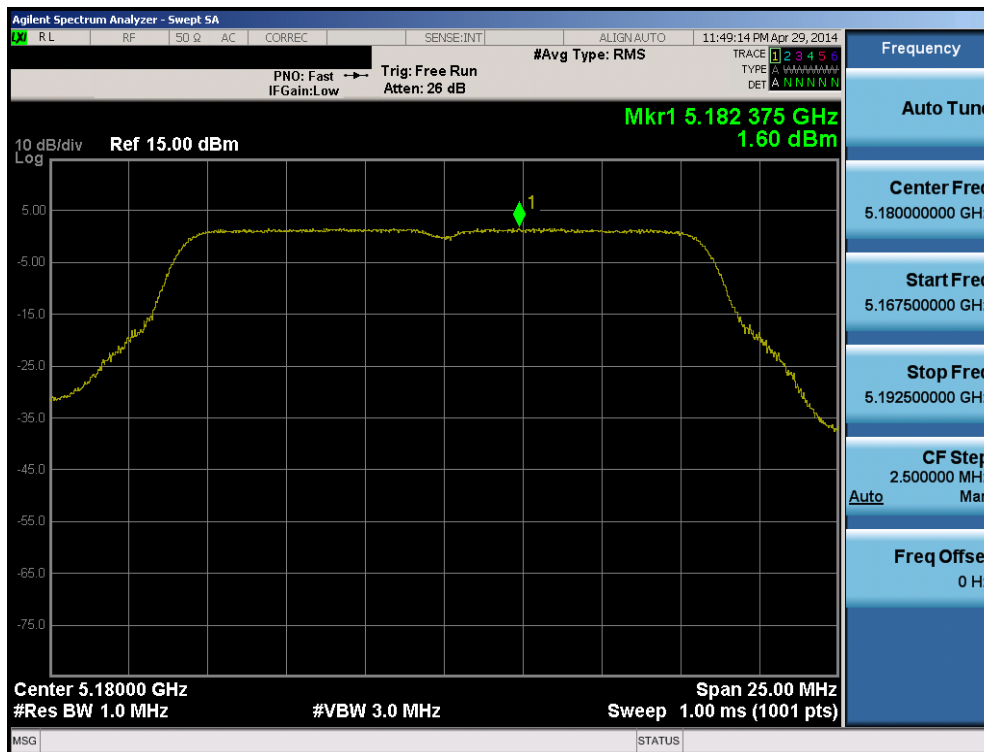
Plot 6-97. Peak Power Spectral Density Plot (802.11a (UNII Band 1) – Ch. 36)
