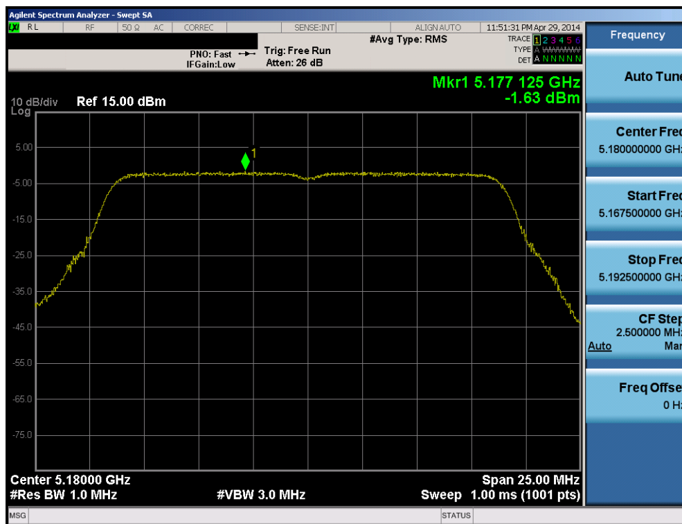
Plot 6-100. Peak Power Spectral Density Plot (20MHz BW 802.11n (UNII Band 1) – Ch. 36)
