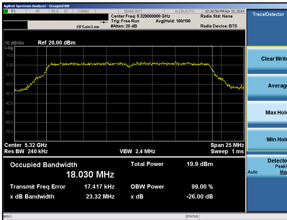
Plot 6-49. 26dB Bandwidth Plot (20MHz BW 802.11n (UNII Band 2A) – Ch. 64)
