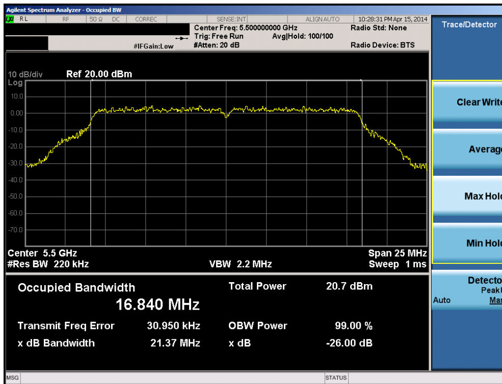
Plot 6-53. 26dB Bandwidth Plot (802.11a (UNII Band 2C) – Ch. 100)
