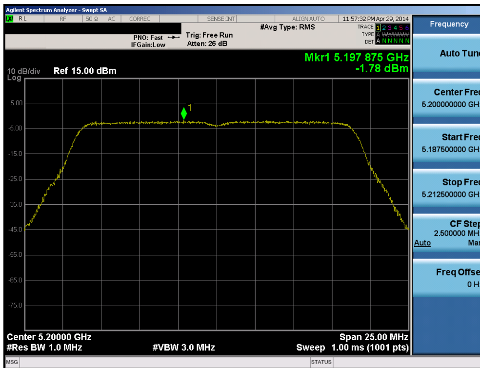
Plot 6-73. Peak Power Spectral Density Plot (20MHz BW 802.11n (UNII Band 1) – Ch. 40)
