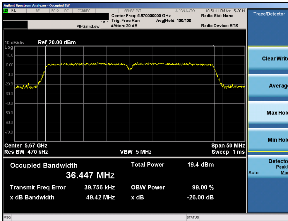
Plot 6-61. 26dB Bandwidth Plot (40MHz BW 802.11n (UNII Band 2C) – Ch. 134)
