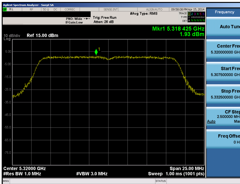
Plot 6-83. Peak Power Spectral Density Plot (20MHz BW 802.11n (UNII Band 2A) – Ch. 64)
