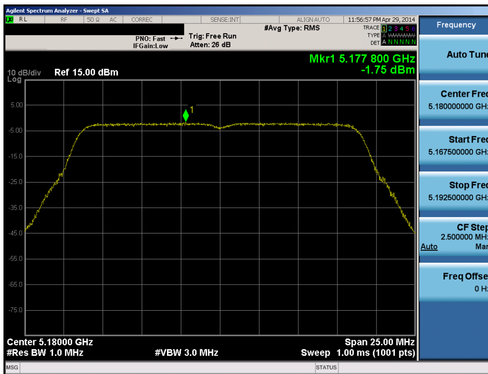
Plot 6-72. Peak Power Spectral Density Plot (20MHz BW 802.11n (UNII Band 1) – Ch. 36)
