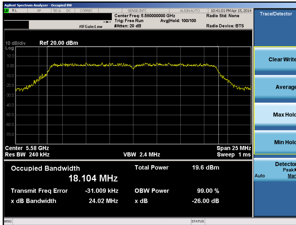
Plot 6-57. 26dB Bandwidth Plot (20MHz BW 802.11n (UNII Band 2C) – Ch. 116)
