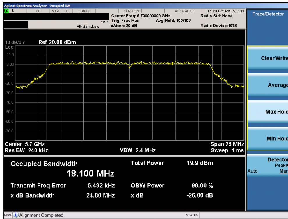
Plot 6-58. 26dB Bandwidth Plot (20MHz BW 802.11n (UNII Band 2C) – Ch. 140)
