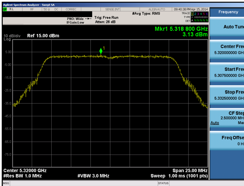
Plot 6-80. Peak Power Spectral Density Plot (802.11a (UNII Band 2A) – Ch. 64)
