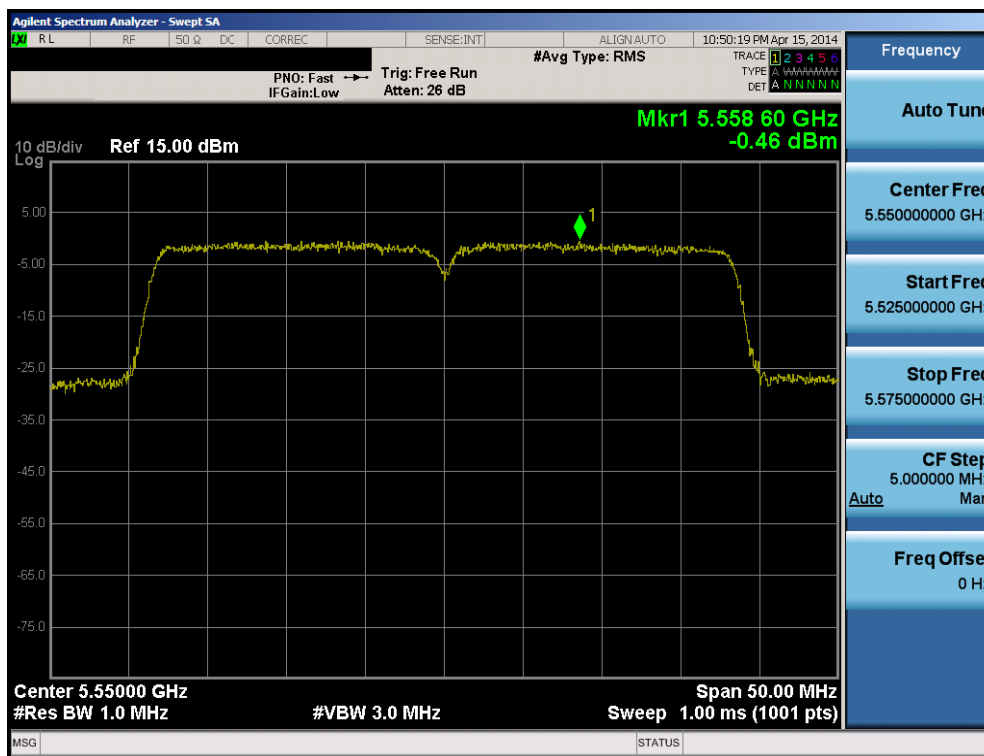
Plot 6-122. Peak Power Spectral Density Plot (40MHz BW 802.11n (UNII Band 2C) – Ch. 110)
