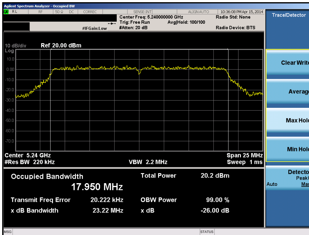
Plot 6-40. 26dB Bandwidth Plot (20MHz BW 802.11n (UNII Band 1) – Ch. 48)
