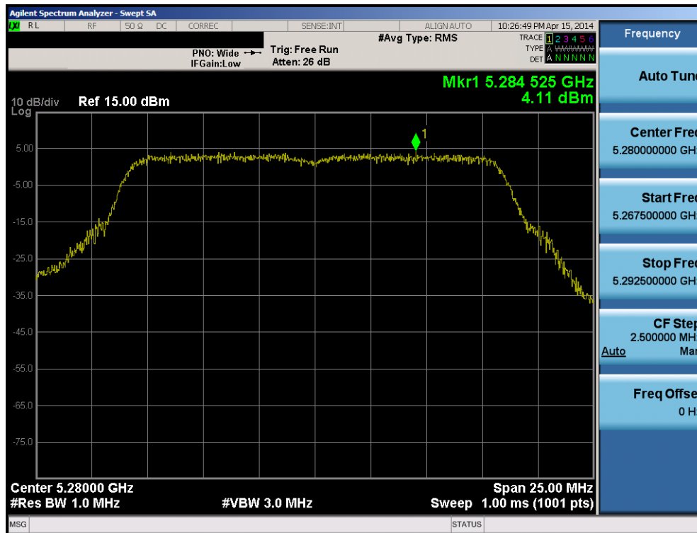
Plot 6-107. Peak Power Spectral Density Plot (802.11a (UNII Band 2A) – Ch. 56)
