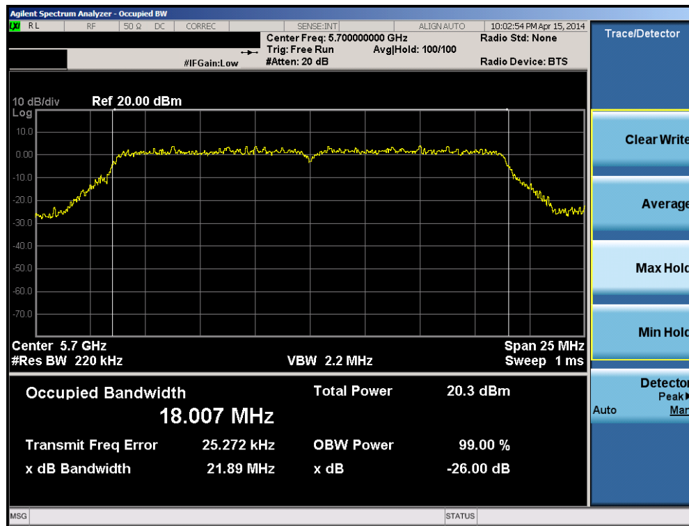
Plot 6-24. 26dB Bandwidth Plot (20MHz BW 802.11n (UNII Band 2C) – Ch. 140)
