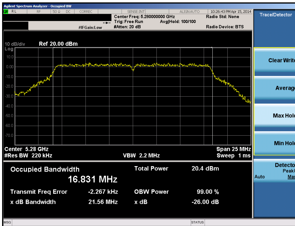
Plot 6-45. 26dB Bandwidth Plot (802.11a (UNII Band 2A) – Ch. 56)
