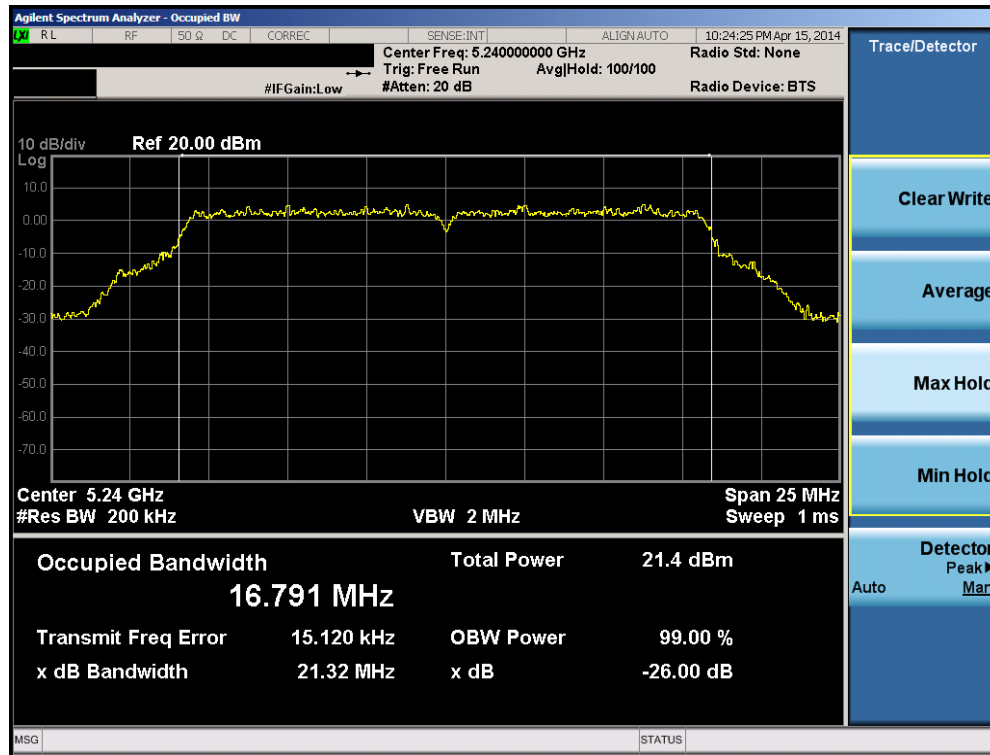
Plot 6-37. 26dB Bandwidth Plot (802.11a (UNII Band 1) – Ch. 48)
