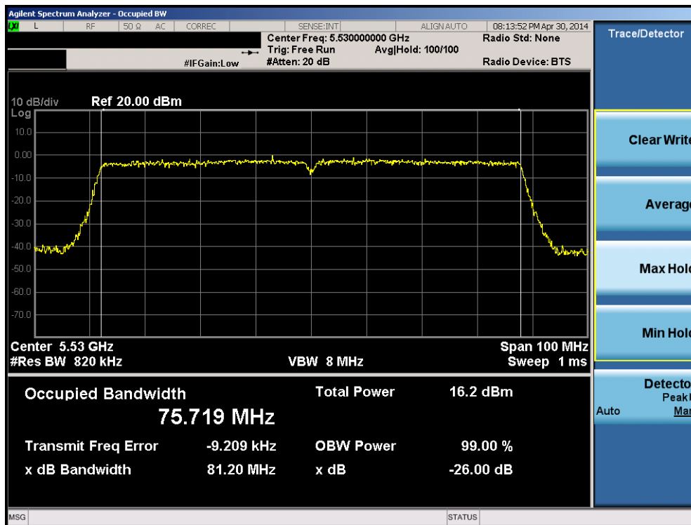
Plot 6-62. 26dB Bandwidth Plot (80MHz BW 802.11ac (UNII Band 2C) – Ch. 106)
