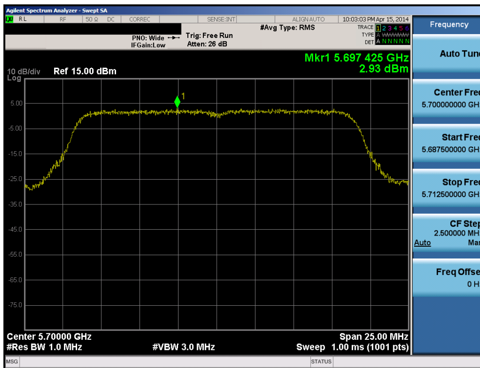
Plot 6-92. Peak Power Spectral Density Plot (20MHz BW 802.11n (UNII Band 2C) – Ch. 140)
