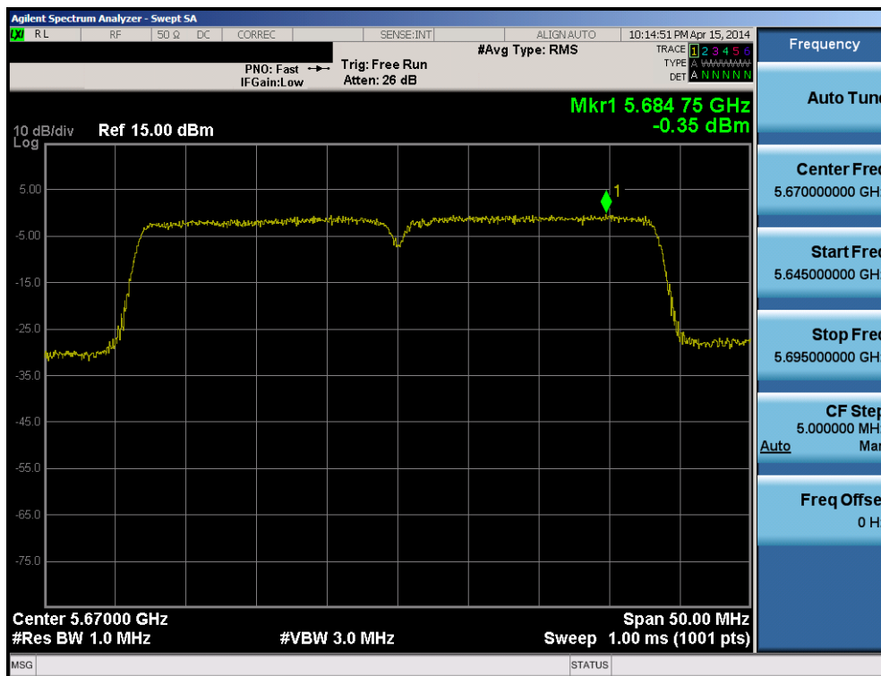
Plot 6-95. Peak Power Spectral Density Plot (40MHz BW 802.11n (UNII Band 2C) – Ch. 134)
