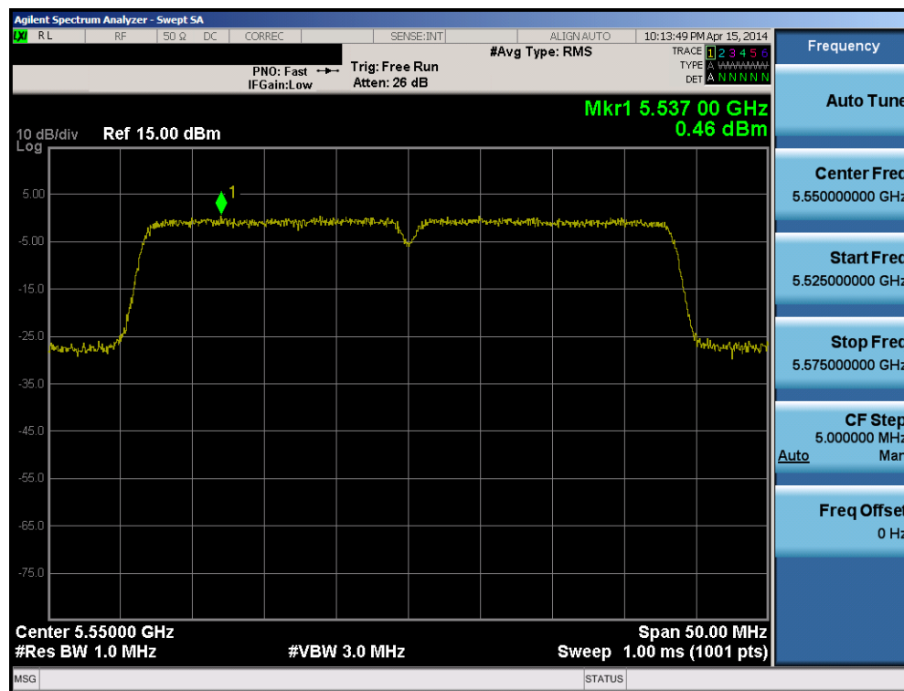
Plot 6-94. Peak Power Spectral Density Plot (40MHz BW 802.11n (UNII Band 2C) – Ch. 110)
