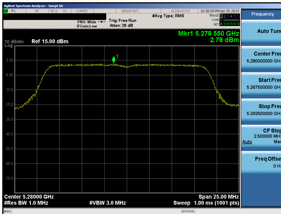
Plot 6-110. Peak Power Spectral Density Plot (20MHz BW 802.11n (UNII Band 2A) – Ch. 56)
