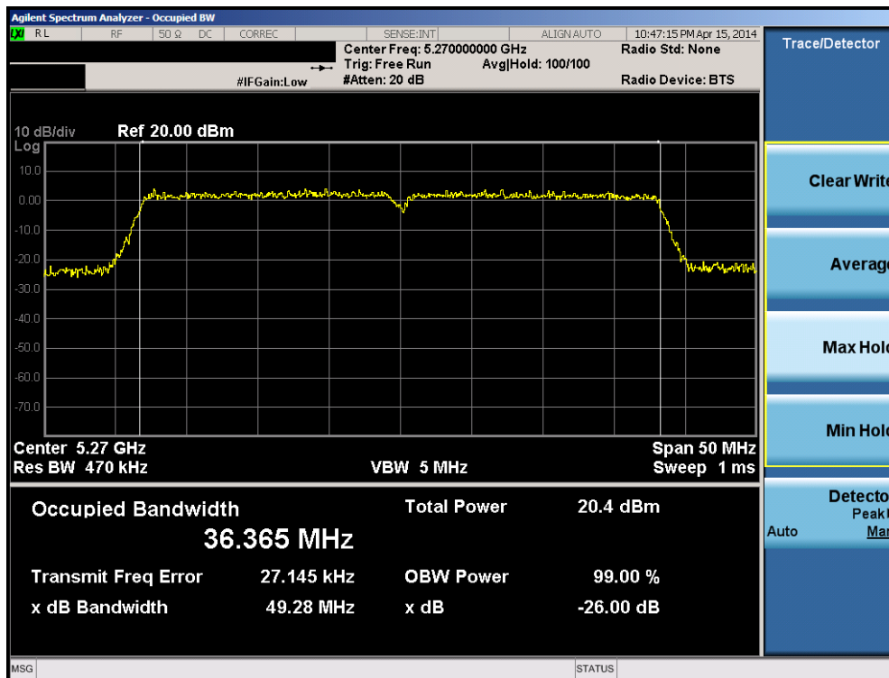
Plot 6-50. 26dB Bandwidth Plot (40MHz BW 802.11n (UNII Band 2A) – Ch. 54)
