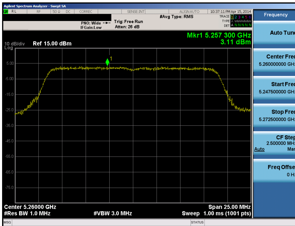
Plot 6-109. Peak Power Spectral Density Plot (20MHz BW 802.11n (UNII Band 2A) – Ch. 52)
