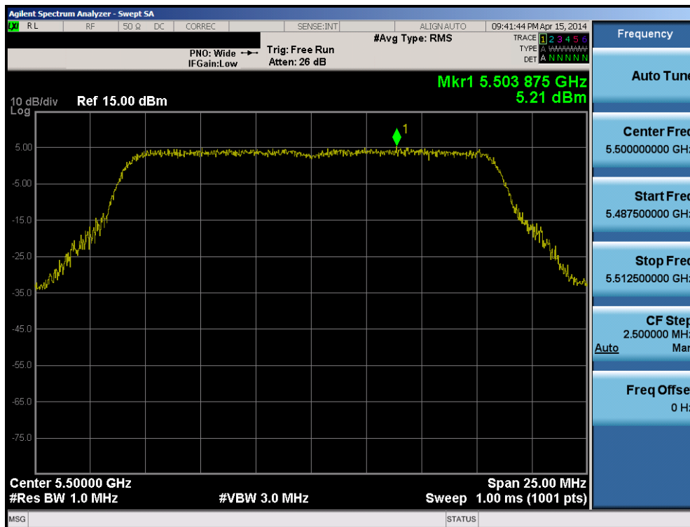
Plot 6-87. Peak Power Spectral Density Plot (802.11a (UNII Band 2C) – Ch. 100)
