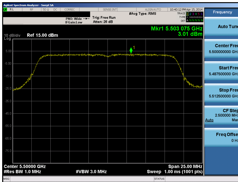
Plot 6-118. Peak Power Spectral Density Plot (20MHz BW 802.11n (UNII Band 2C) – Ch. 100)
