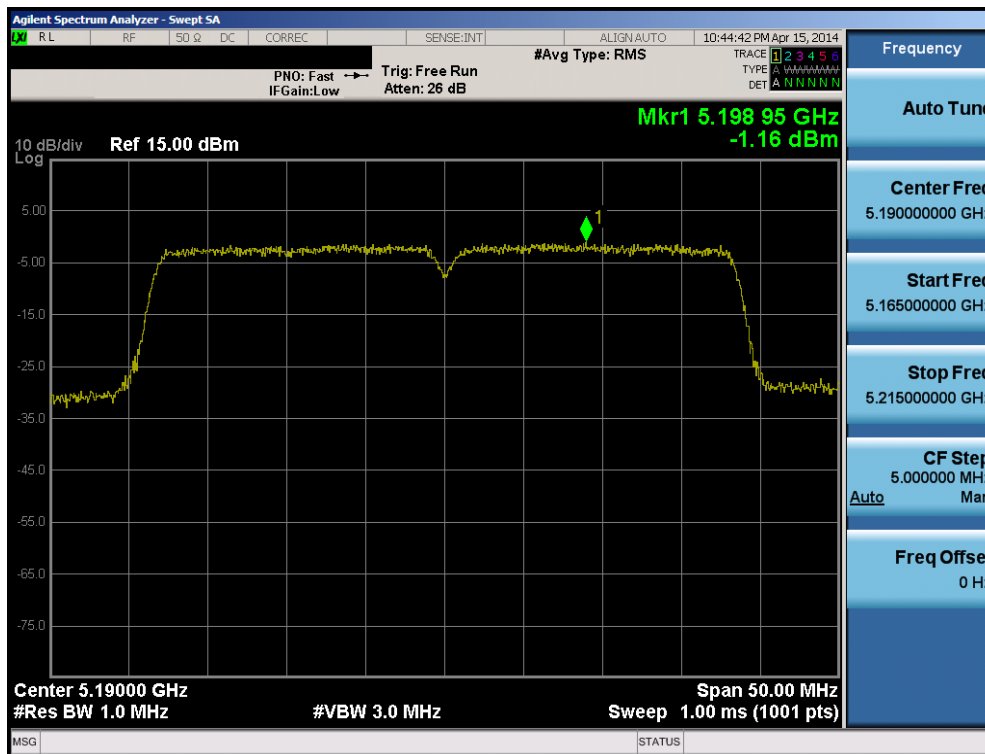
Plot 6-103. Peak Power Spectral Density Plot (40MHz BW 802.11n (UNII Band 1) – Ch. 38)
