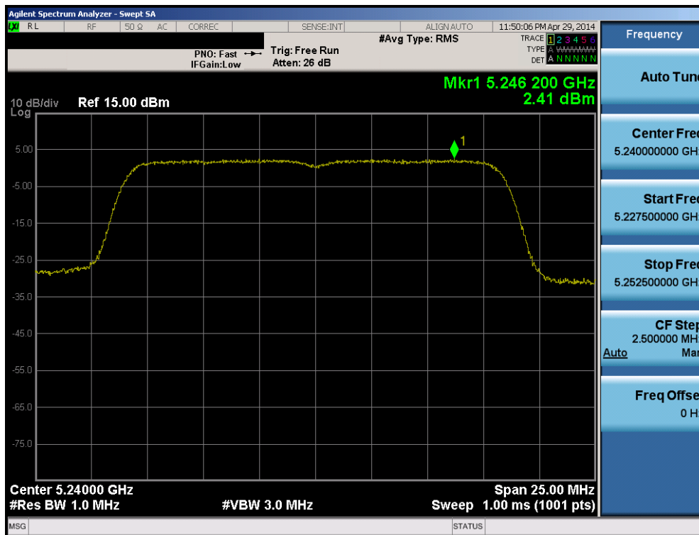
Plot 6-99. Peak Power Spectral Density Plot (802.11a (UNII Band 1) – Ch. 48)
