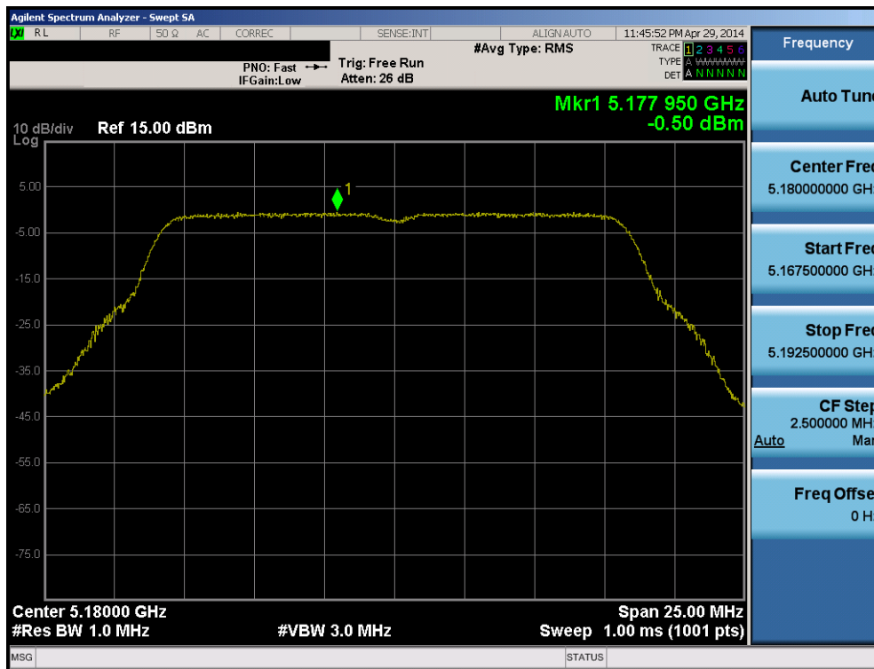
Plot 6-69. Peak Power Spectral Density Plot (802.11a (UNII Band 1) – Ch. 36)
