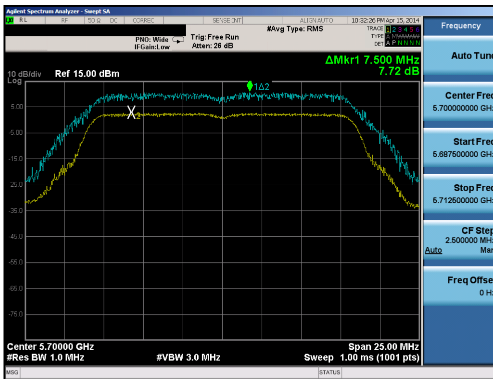
Plot 6-129. Peak Excursion Ratio Plot (802.11a (UNII Band 2C) – Ch. 140)
