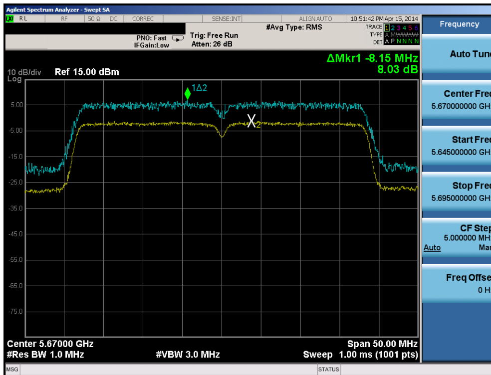
Plot 6-131. Peak Excursion Ratio Plot (40MHz BW 802.11n (UNII Band 2C) – Ch. 134)
