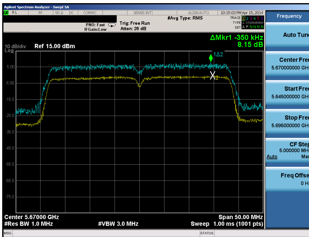
Plot 6-127. Peak Excursion Ratio Plot (40MHz BW 802.11n (UNII Band 2C) – Ch. 134)
