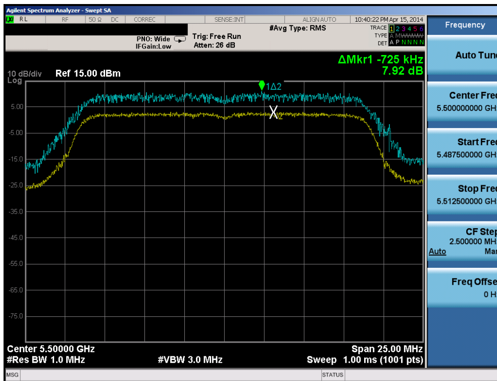
Plot 6-130. Peak Excursion Ratio Plot (20MHz BW 802.11n (UNII Band 2C) – Ch. 100)
