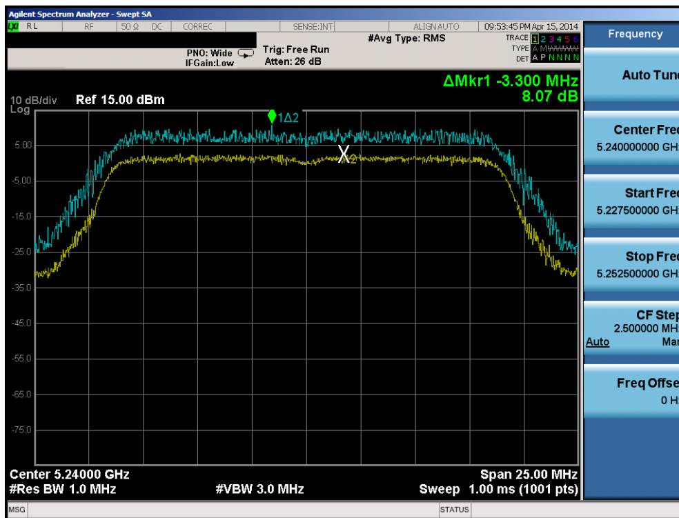
Plot 6-126. Peak Excursion Ratio Plot (802.11n (UNII Band 1) – Ch. 48)
