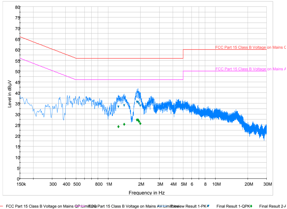
Plot 6-140. Line Conducted Plot with 802.11a (N)
