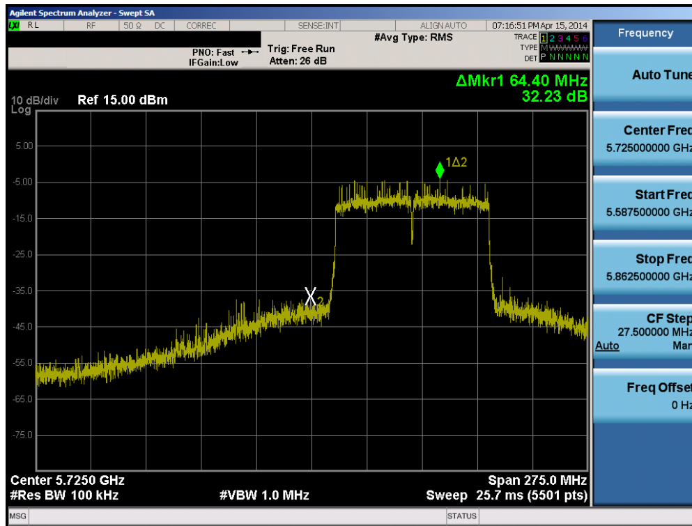
Plot 6-85. Band Edge Plot (80MHz BW 802.11ac (5.8GHz) – Ch. 155)
