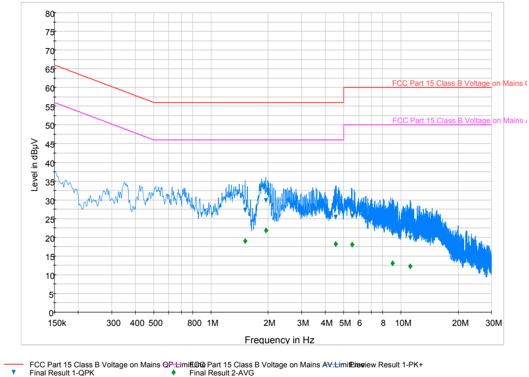
Plot 6-139. Line Conducted Plot with 802.11a (L1)
