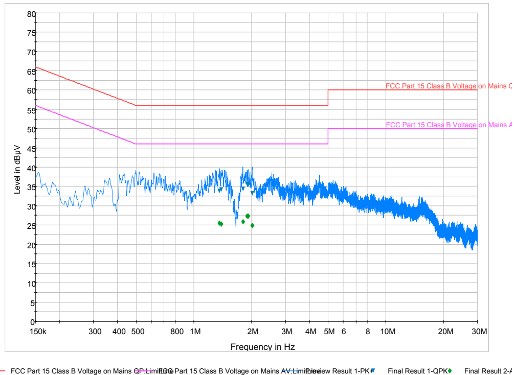
Plot 6-138. Line Conducted Plot with 802.11b (N)
