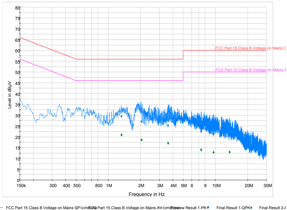
Plot 6-137. Line Conducted Plot with 802.11b (L1)
