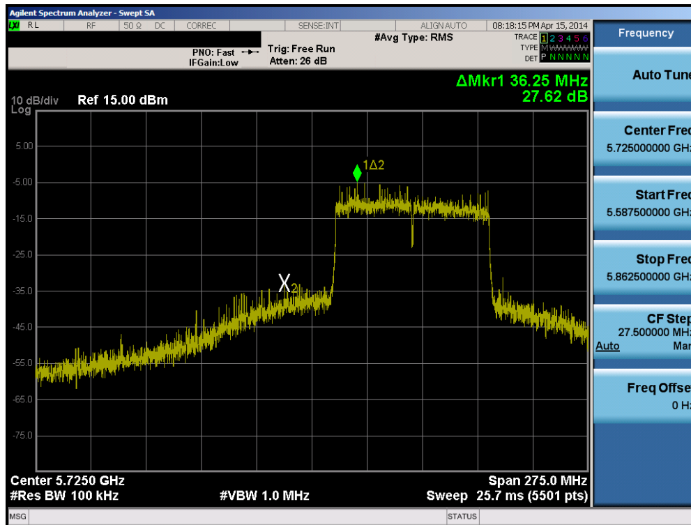
Plot 6-99. Band Edge Plot (80MHz BW 802.11ac (5.8GHz) – Ch. 155)
