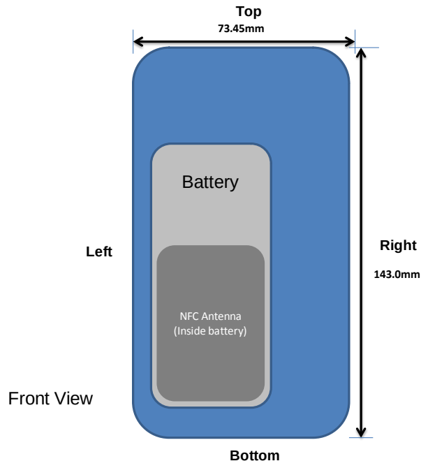
Figure 1-2 NFC Antenna Locations
