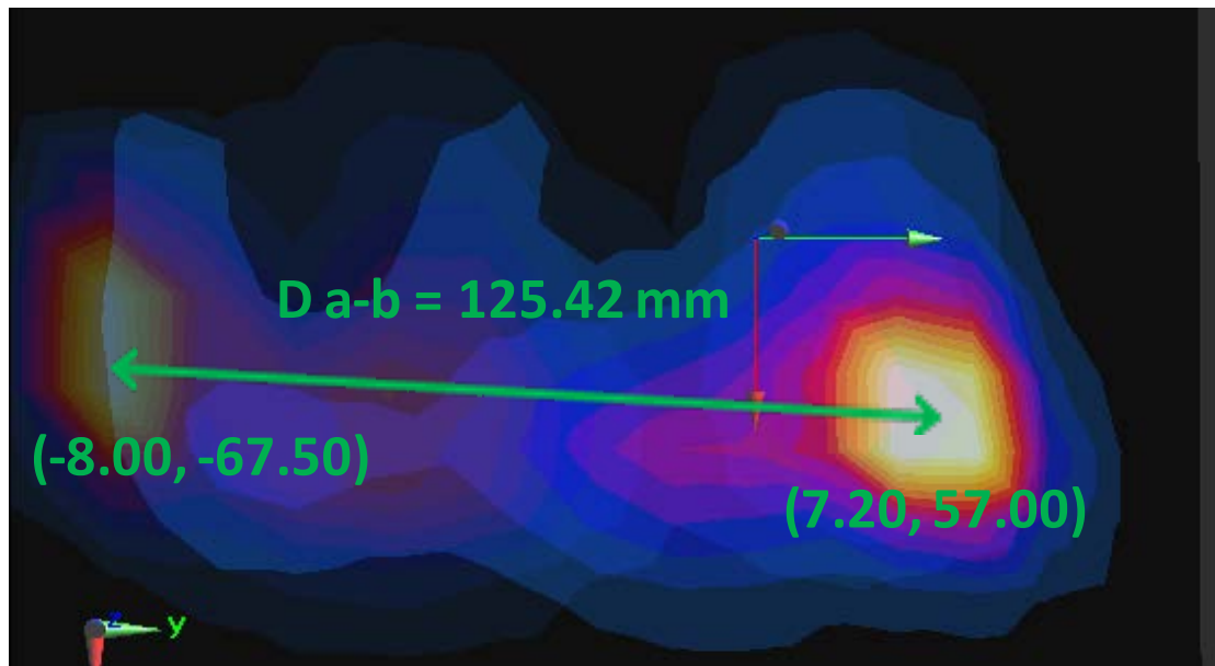
Figure 12-1 Peak SAR Locations of LTE band 2 and 2.4 GHz WLAN Ant. 2 Back Side at 10 mm
