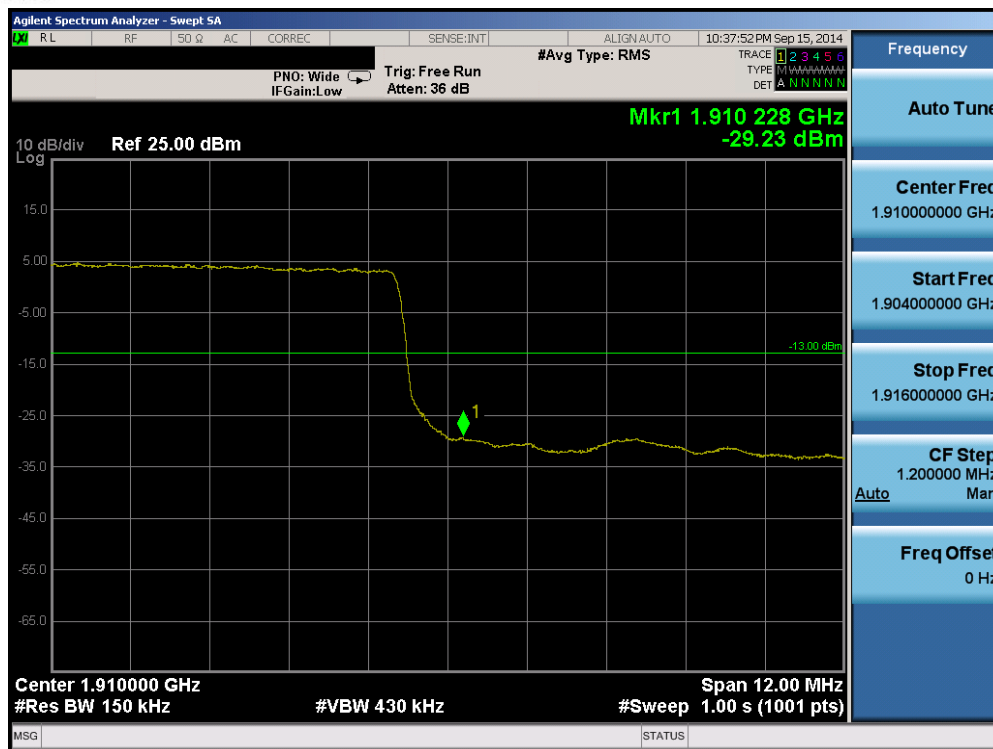
Plot 6-65. Upper Band Edge Plot (Band 2 – 15.0MHz QPSK – RB Size 75)
