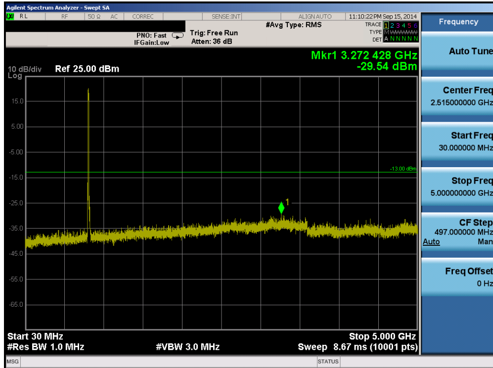
Plot 6-21. Conducted Spurious Plot (Band 5 – 10.0MHz QPSK – RB Size 1, RB Offset 0– Low Channel)
