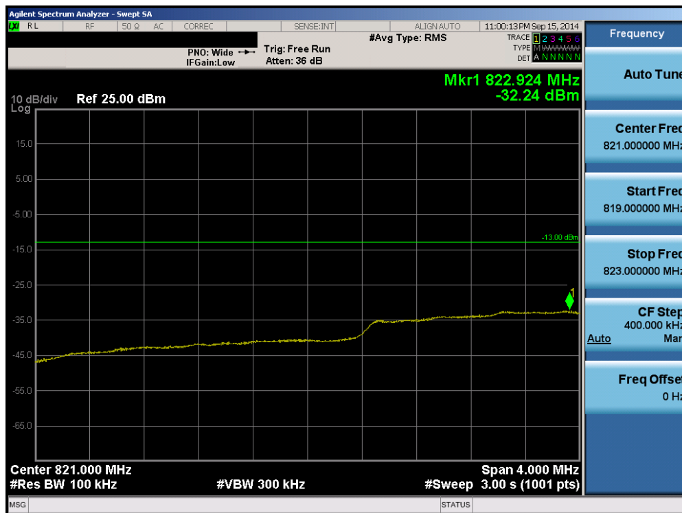
Plot 6-38. Lower Extended Band Edge Plot (Band 5 – 3.0MHz QPSK – RB Size 15)
