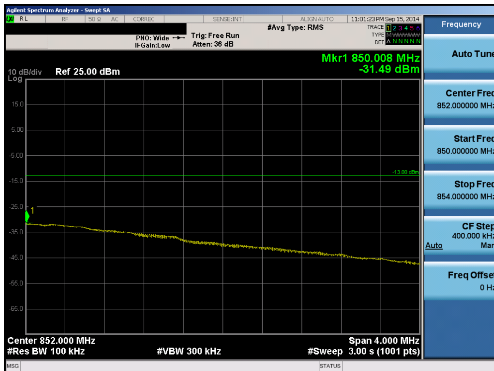
Plot 6-40. Upper Extended Band Edge Plot (Band 5 - Band 5 - 3.0MHz QPSK - RB Size 15)
