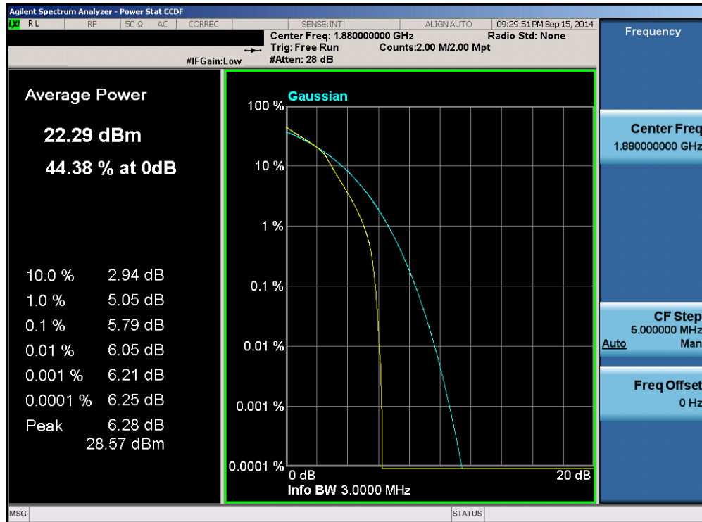
Plot 6-74. PAR Plot (Band 2 – 3.0MHz 16-QAM – RB Size 15)
