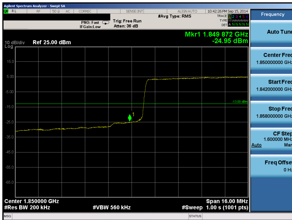
Plot 6-67. Lower Band Edge Plot (Band 2 – 20.0MHz QPSK – RB Size 100)
