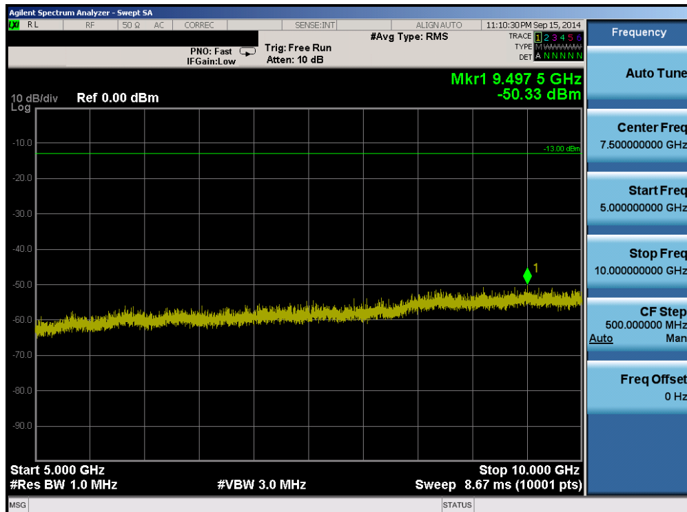
Plot 6-22. Conducted Spurious Plot (Band 5 – 10.0MHz QPSK – RB Size 1, RB Offset 0 – Low Channel)
