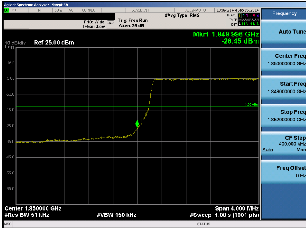
Plot 6-55. Lower Band Edge Plot (Band 2 – 5.0MHz QPSK – RB Size 25)
