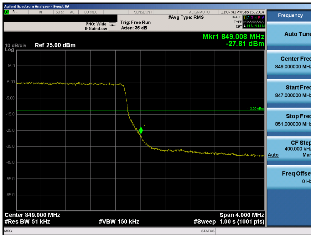
Plot 6-43. Upper Band Edge Plot (Band 5 - 5.0MHz QPSK - RB Size 25)
