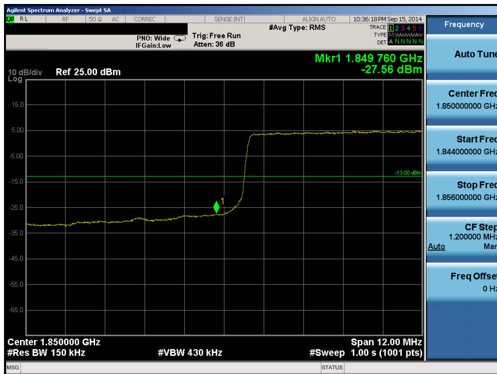
Plot 6-63. Lower Band Edge Plot (Band 2 – 15.0MHz QPSK – RB Size 75)
