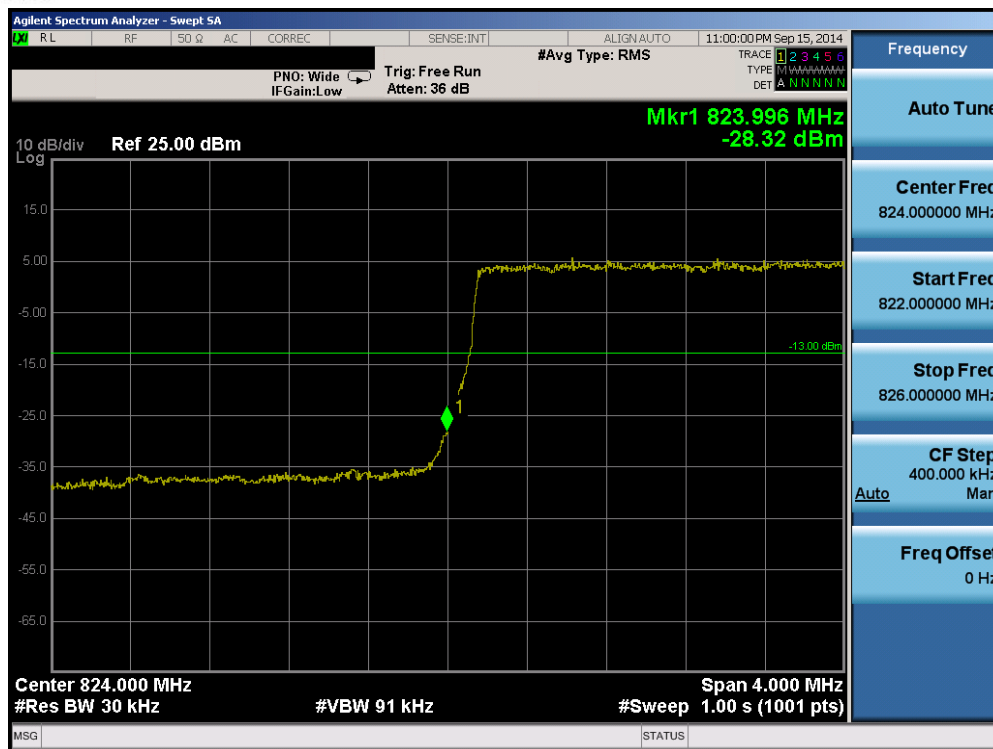
Plot 6-37. Lower Band Edge Plot (Band 5 – 3.0MHz QPSK – RB Size 15)
