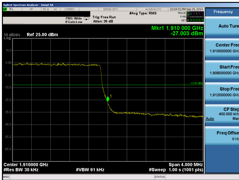
Plot 6-53. Upper Band Edge Plot (Band 2 – 3.0MHz QPSK – RB Size 15)
