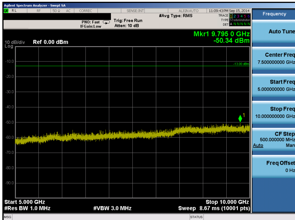
Plot 6-24. Conducted Spurious Plot (Band 5 – 10.0MHz QPSK – RB Size 1, RB Offset 0 – Mid Channel)
