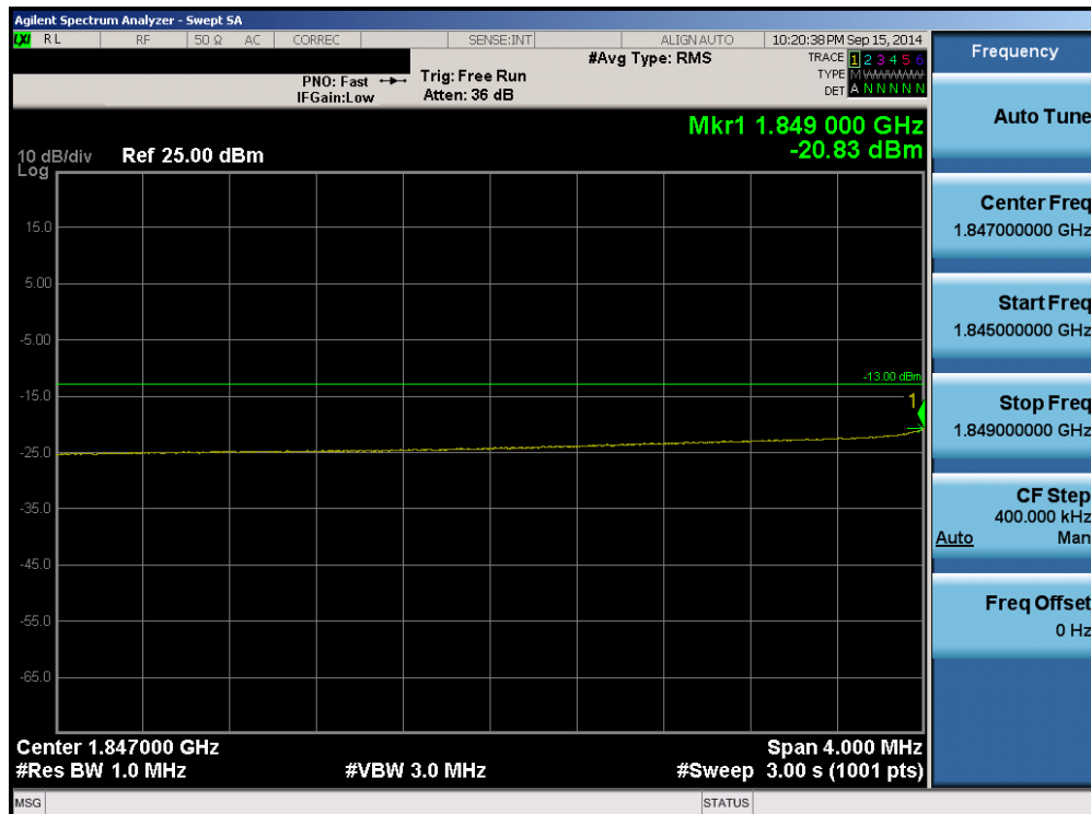
Plot 6-60. Lower Extended Band Edge Plot (Band 2 – 10.0MHz QPSK – RB Size 50)
