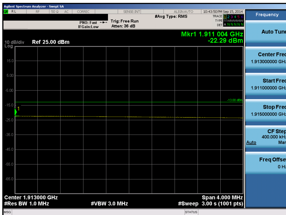
Plot 6-70. Upper Extended Band Edge Plot (Band 2 – 20.0MHz QPSK – RB Size 100)
