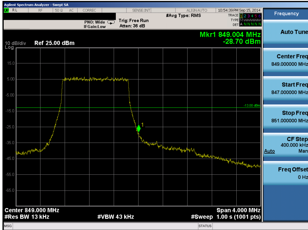
Plot 6-35. Upper Band Edge Plot (Band 5 – 1.4MHz QPSK – RB Size 6)
