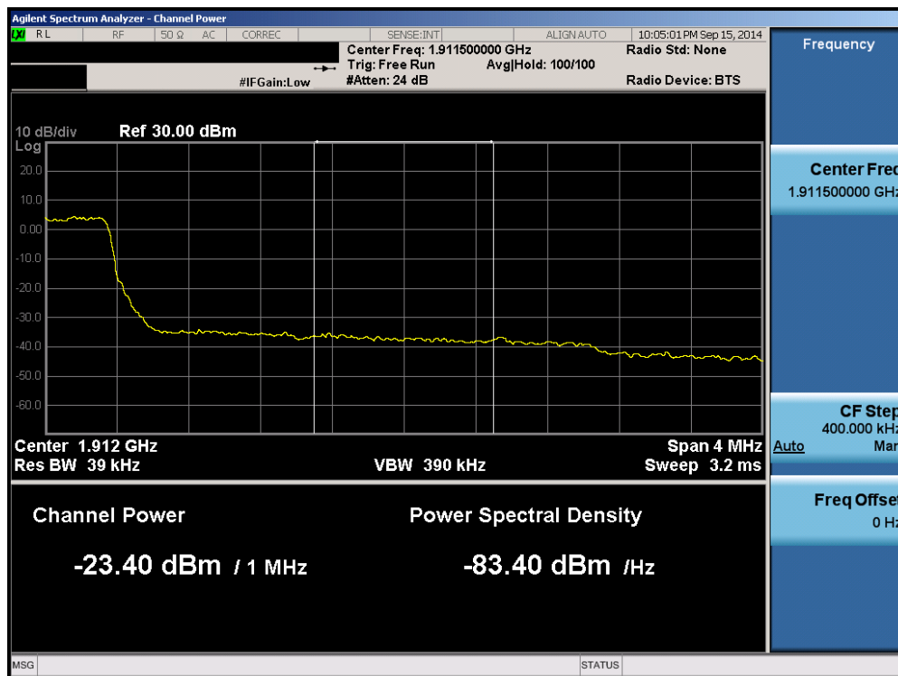
Plot 6-54. Upper Extended Band Edge Plot (Band 2 – 3.0MHz QPSK – RB Size 15)
