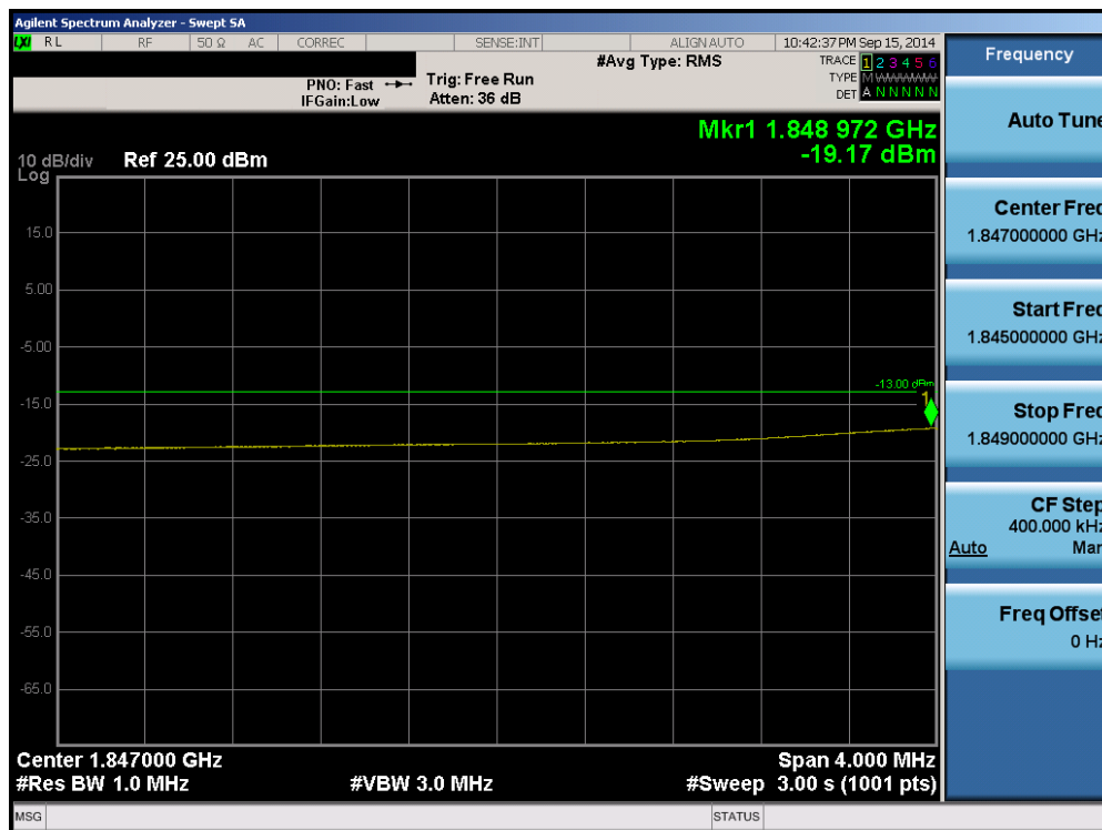
Plot 6-68. Lower Extended Band Edge Plot (Band 2 – 20.0MHz QPSK – RB Size 100)
