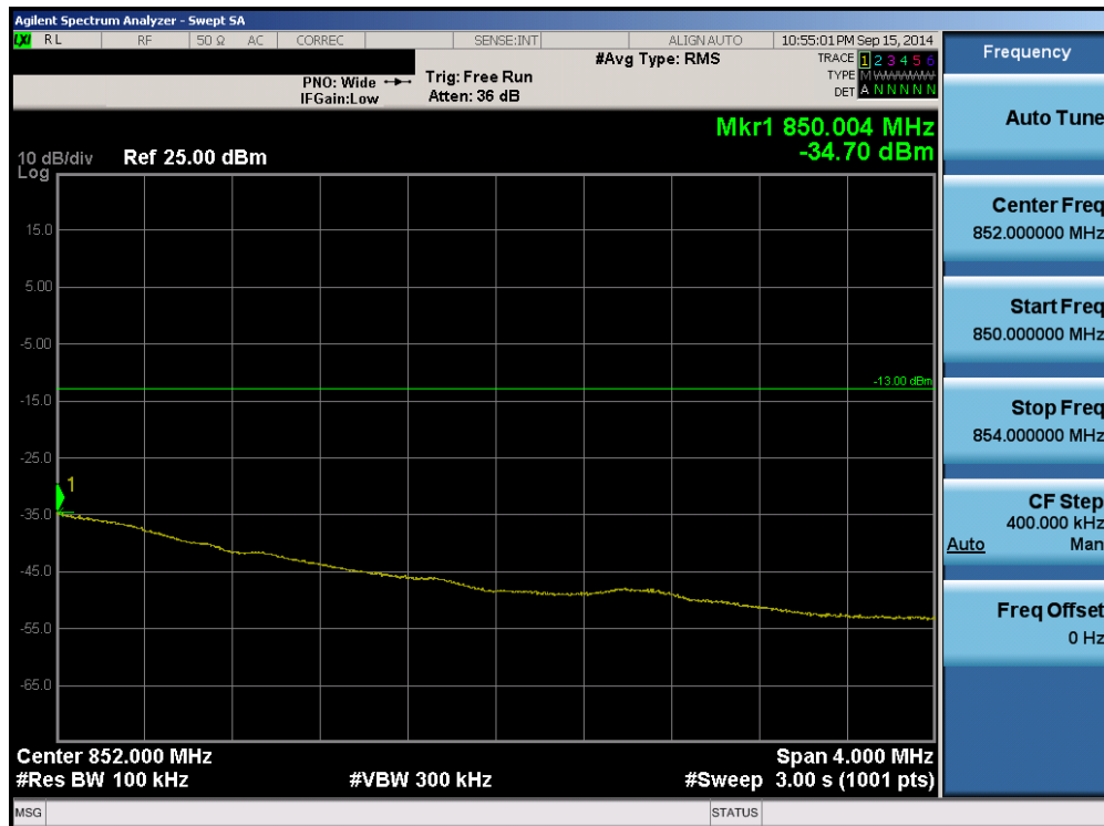
Plot 6-36. Upper Extended Band Edge Plot (Band 5 – 1.4MHz QPSK – RB Size 6)
