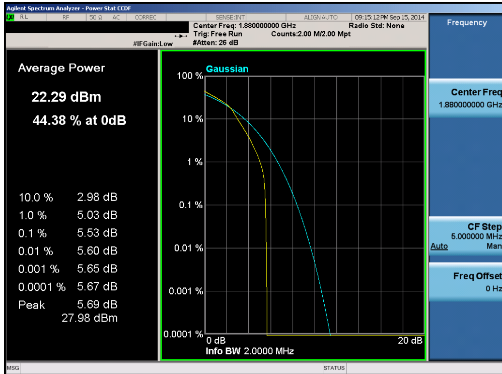
Plot 6-72. PAR Plot (Band 2 – 1.4MHz 16-QAM – RB Size 6)
