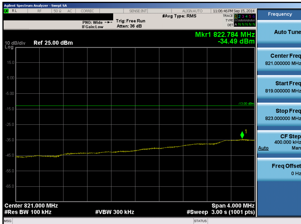
Plot 6-42. Lower Extended Band Edge Plot (Band 5 - 5.0MHz QPSK - RB Size 25)
