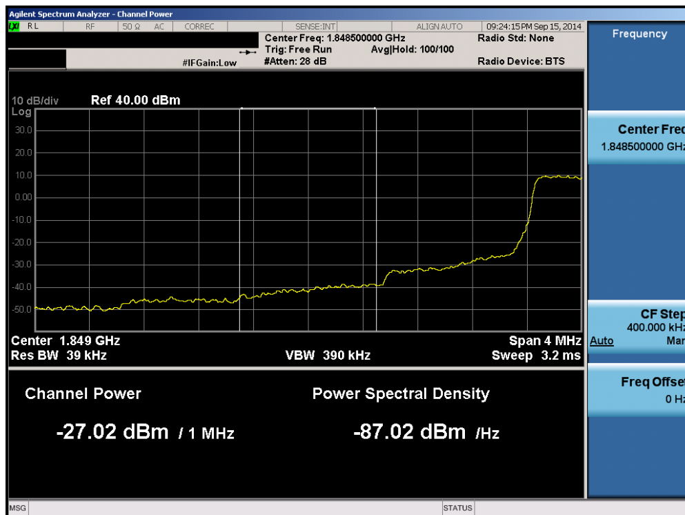
Plot 6-48. Lower Extended Band Edge Plot (Band 2 – 1.4MHz QPSK – RB Size 6)
