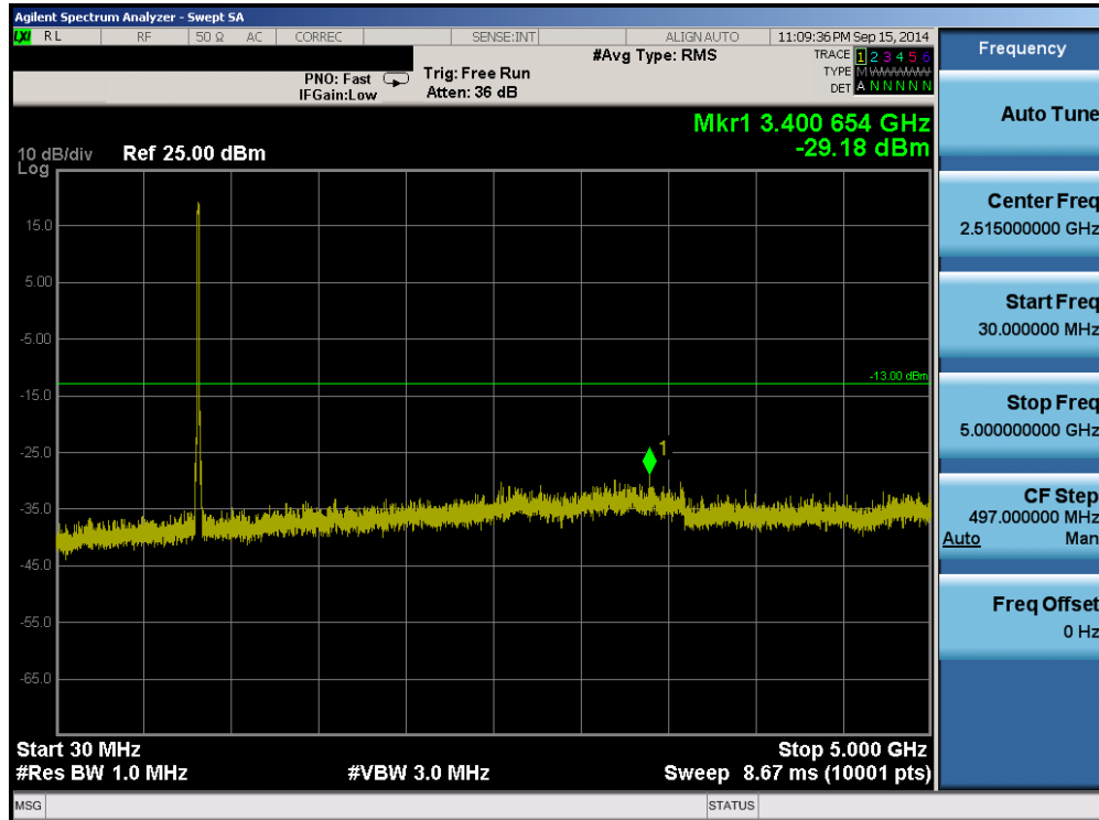
Plot 6-23. Conducted Spurious Plot (Band 5 – 10.0MHz QPSK – RB Size 1, RB Offset 0 – Mid Channel)
