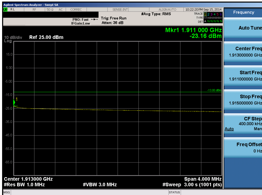
Plot 6-62. Upper Extended Band Edge Plot (Band 2 – 10.0MHz QPSK – RB Size 50)
