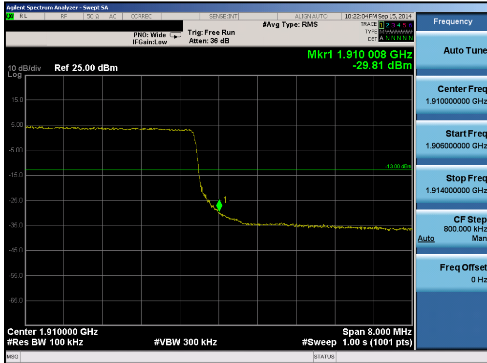
Plot 6-61. Upper Band Edge Plot (Band 2 – 10.0MHz QPSK – RB Size 50)
