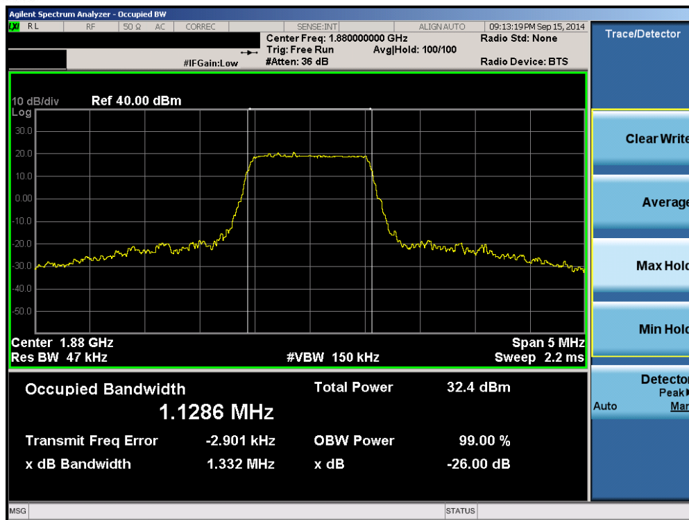
Plot 6-9. Occupied Bandwidth Plot (Band 2 – 1.4MHz QPSK – RB Size 6)
