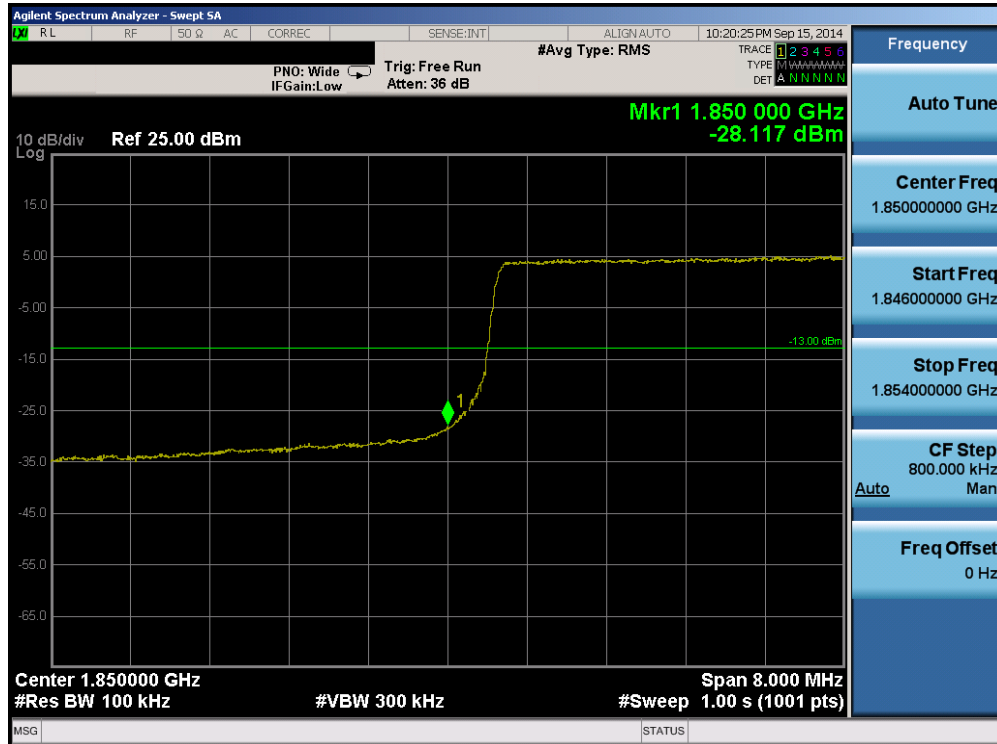
Plot 6-59. Lower Band Edge Plot (Band 2 – 10.0MHz QPSK – RB Size 50)
