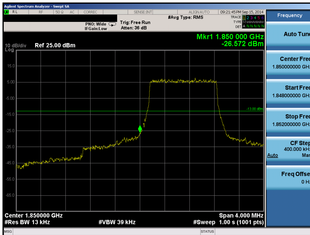
Plot 6-47. Lower Band Edge Plot (Band 2 – 1.4MHz QPSK – RB Size 6)
