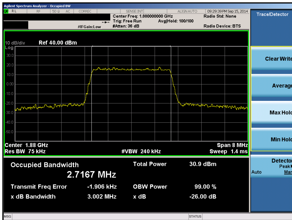
Plot 6-12. Occupied Bandwidth Plot (Band 2 – 3.0MHz 16-QAM – RB Size 15)
