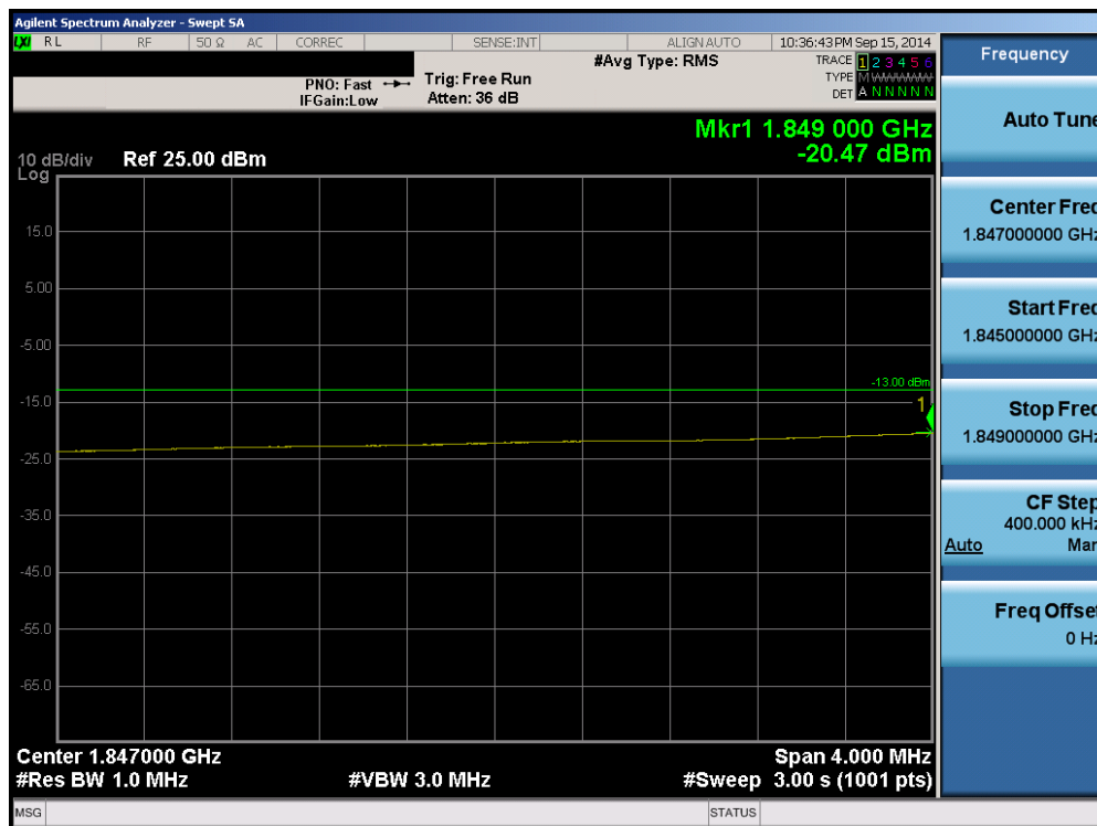
Plot 6-64. Lower Extended Band Edge Plot (Band 2 – 15.0MHz QPSK – RB Size 75)
