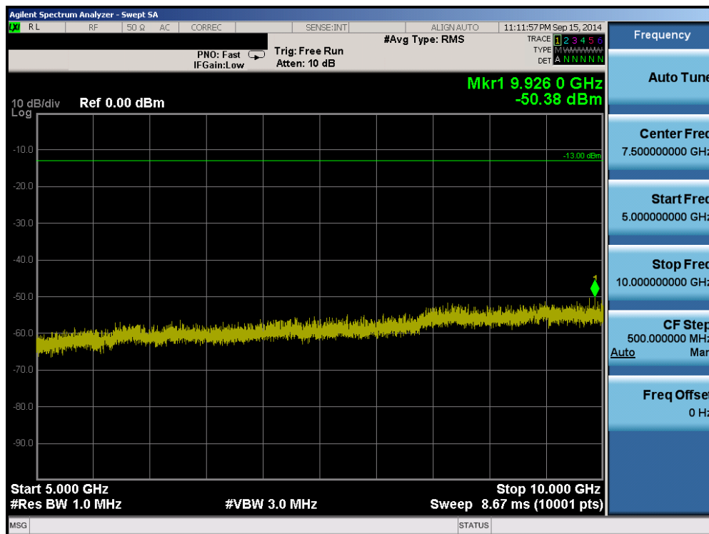
Plot 6-26. Conducted Spurious Plot (Band 5 – 10.0MHz QPSK – RB Size 1, RB Offset 0 – High Channel)
