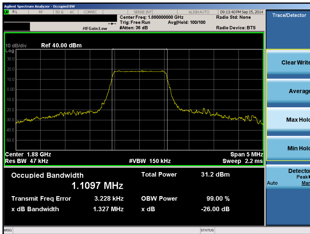
Plot 6-10. Occupied Bandwidth Plot (Band 2 – 1.4MHz 16-QAM – RB Size 6)
