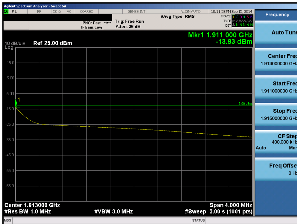
Plot 6-58. Upper Extended Band Edge Plot (Band 2 – 5.0MHz QPSK – RB Size 25)
