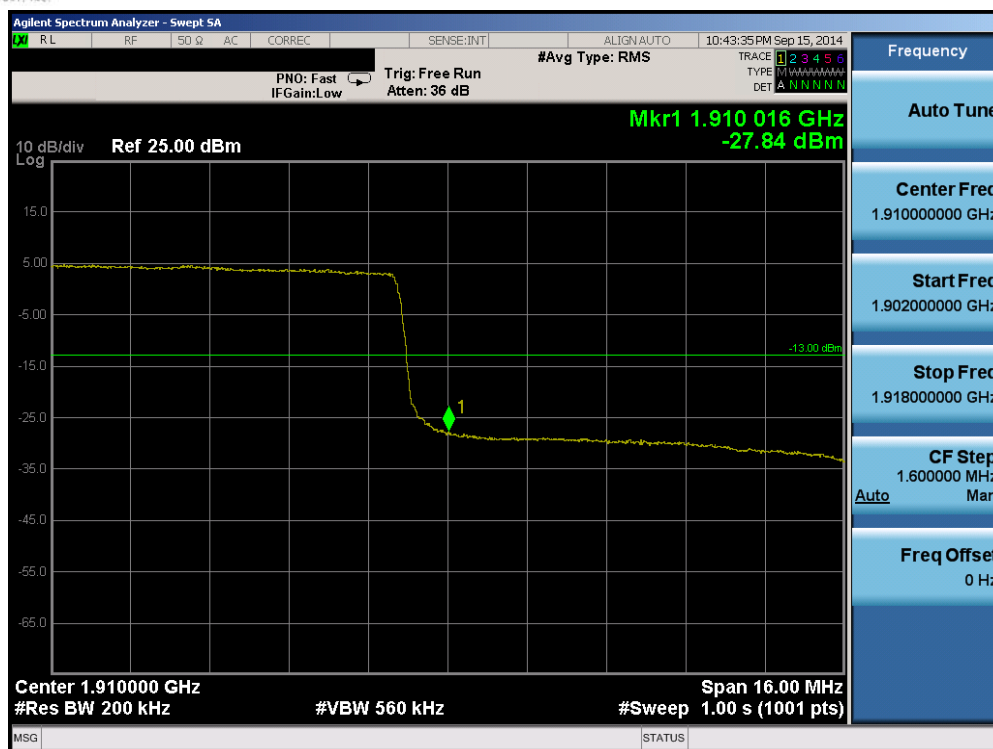
Plot 6-69. Upper Band Edge Plot (Band 2 – 20.0MHz QPSK – RB Size 100)
