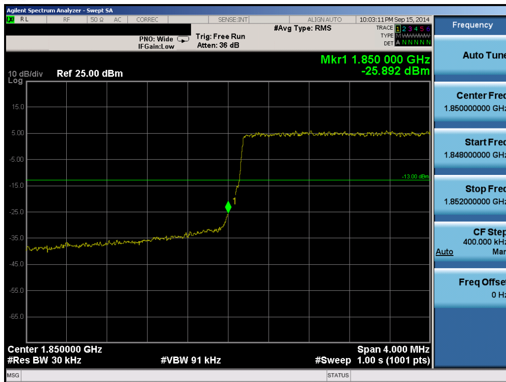
Plot 6-51. Lower Band Edge Plot (Band 2 – 3.0MHz QPSK – RB Size 15)
