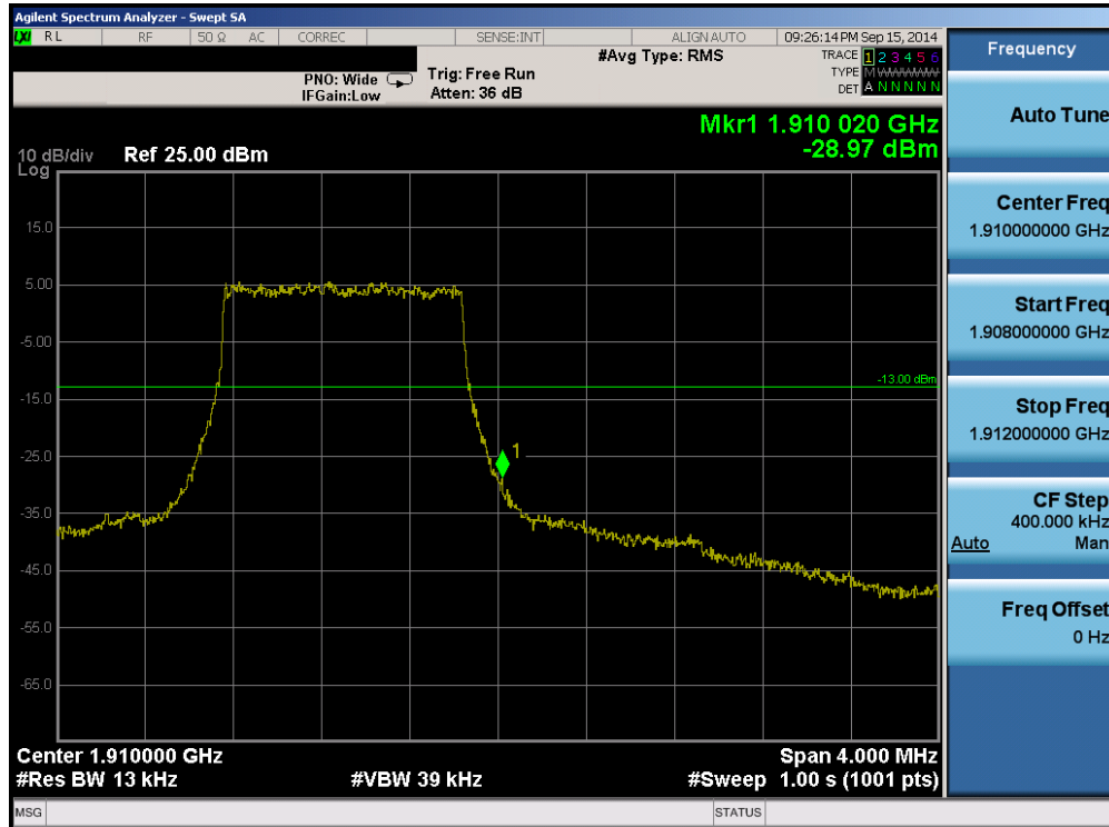
Plot 6-49. Upper Band Edge Plot (Band 2 – 1.4MHz QPSK – RB Size 6)
