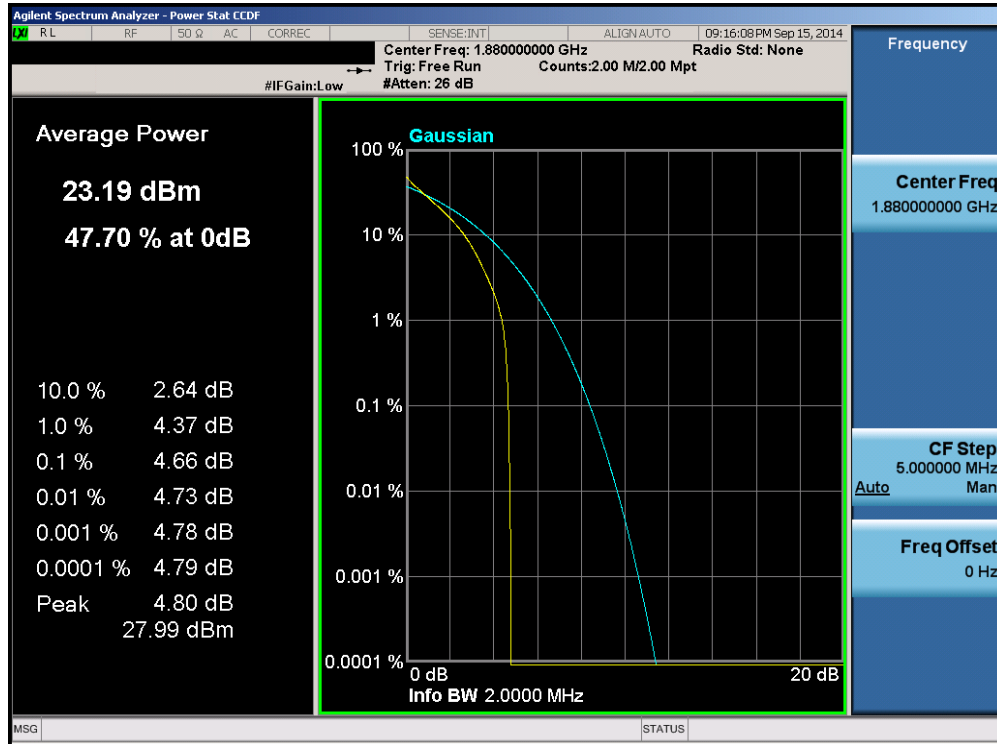
Plot 6-71. PAR Plot (Band 2 – 1.4MHz QPSK – RB Size 6)
