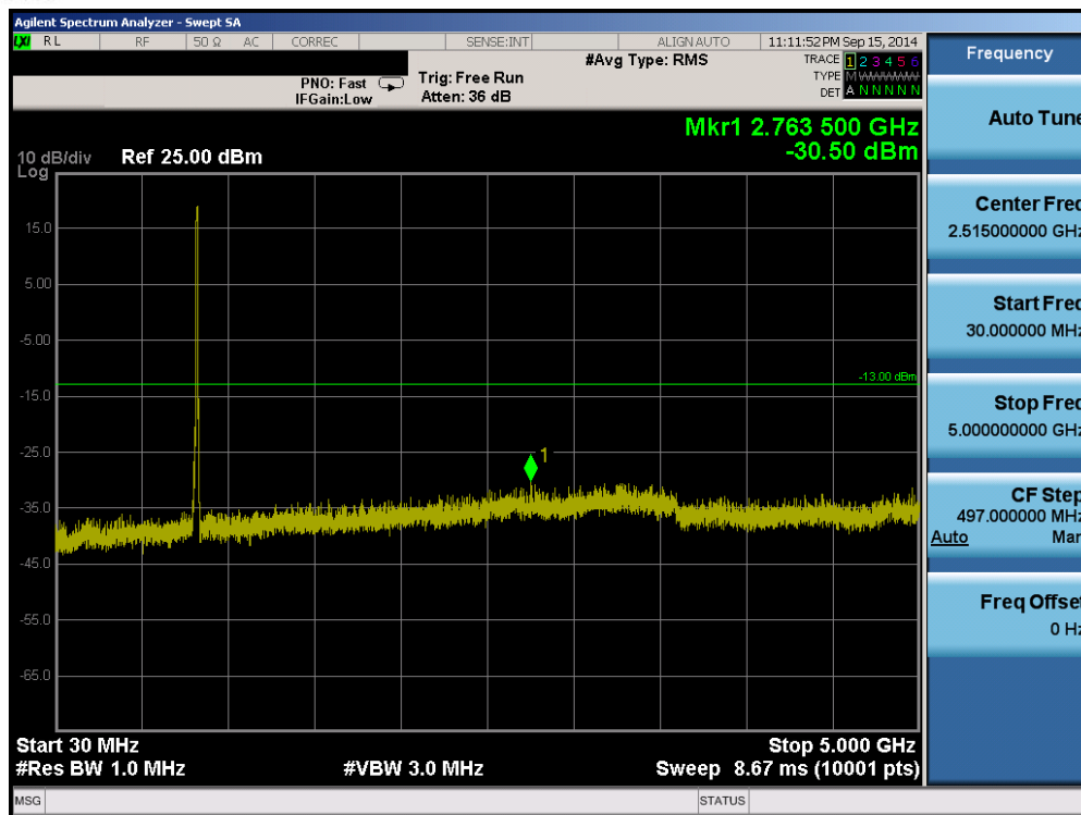
Plot 6-25. Conducted Spurious Plot (Band 5 – 10.0MHz QPSK – RB Size 1, RB Offset 0 – High Channel)
