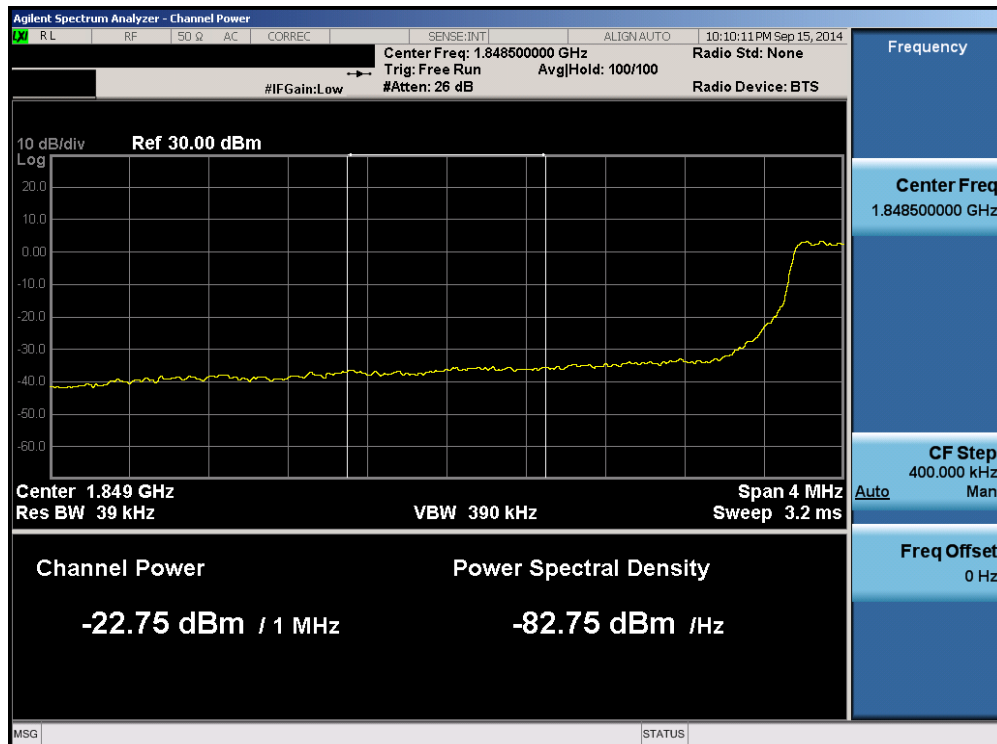
Plot 6-56. Lower Extended Band Edge Plot (Band 2 – 5.0MHz QPSK – RB Size 25)
