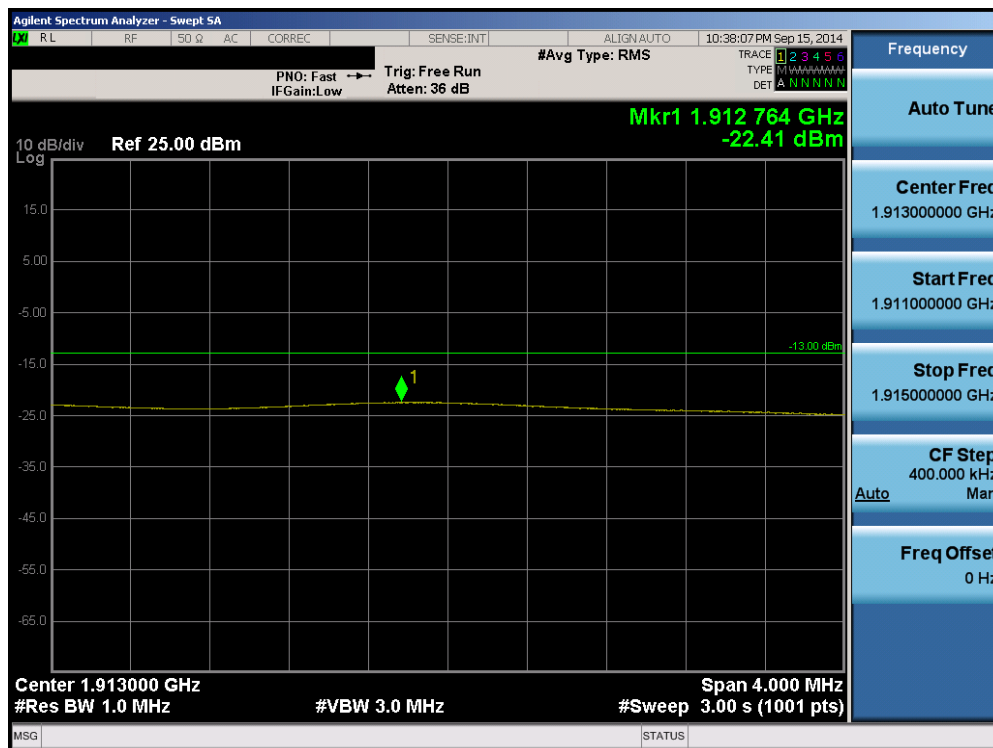
Plot 6-66. Upper Extended Band Edge Plot (Band 2 – 15.0MHz QPSK – RB Size 75)
