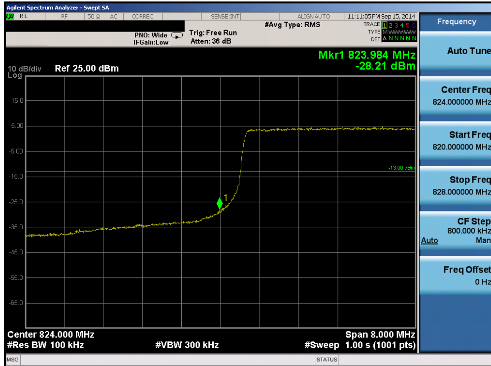
Plot 6-45. Lower Band Edge Plot (Band 5 – 10.0MHz QPSK – RB Size 50)
