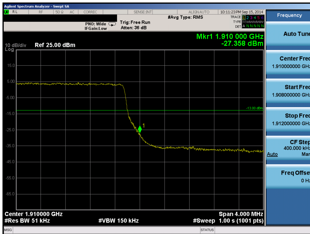
Plot 6-57. Upper Band Edge Plot (Band 2 – 5.0MHz QPSK – RB Size 25)
