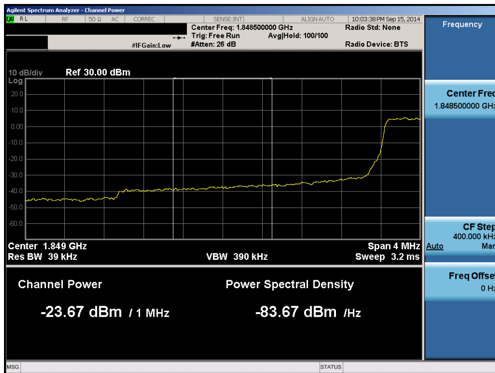
Plot 6-52. Lower Extended Band Edge Plot (Band 2 – 3.0MHz QPSK – RB Size 15)
