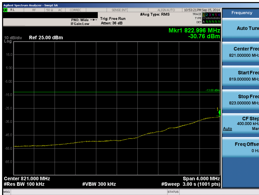
Plot 6-34. Lower Extended Band Edge Plot (Band 5 – 1.4MHz QPSK – RB Size 6)
