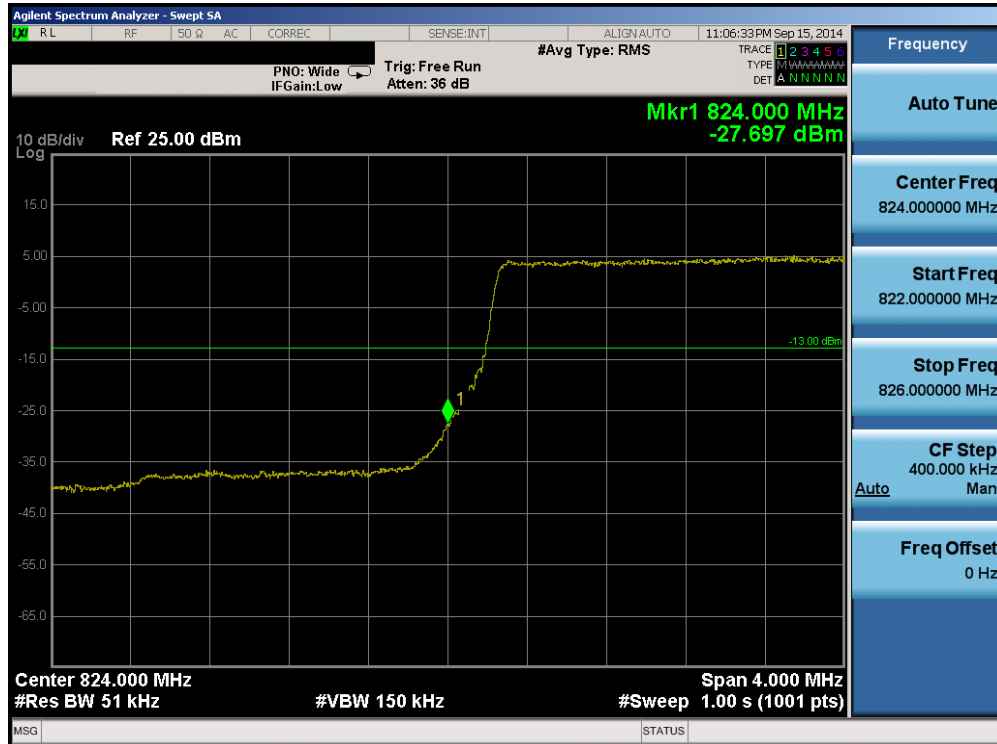
Plot 6-41. Lower Band Edge Plot (Band 5 - 5.0MHz QPSK - RB Size 25)
