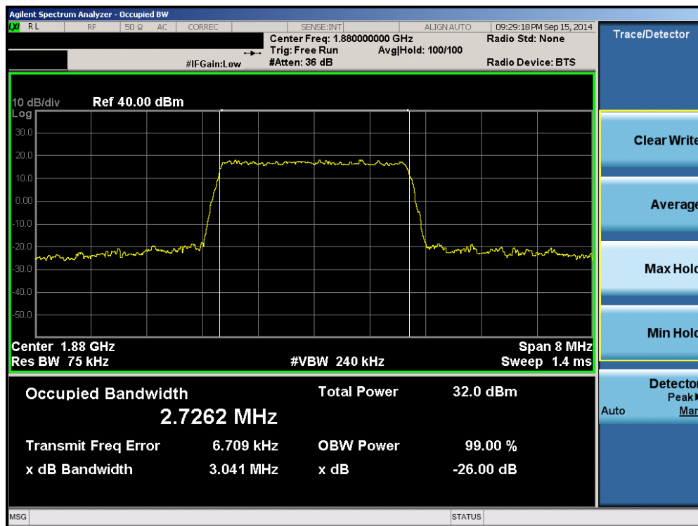
Plot 6-11. Occupied Bandwidth Plot (Band 2 – 3.0MHz QPSK – RB Size 15)
