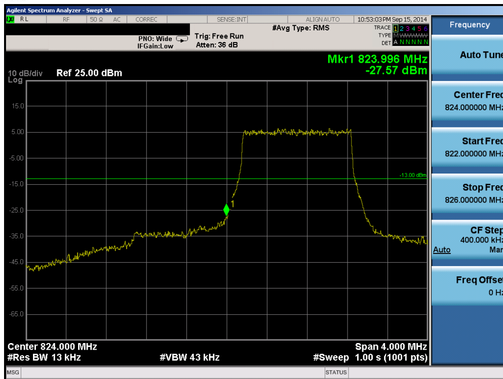
Plot 6-33. Lower Band Edge Plot (Band 5 – 1.4MHz QPSK – RB Size 6)
