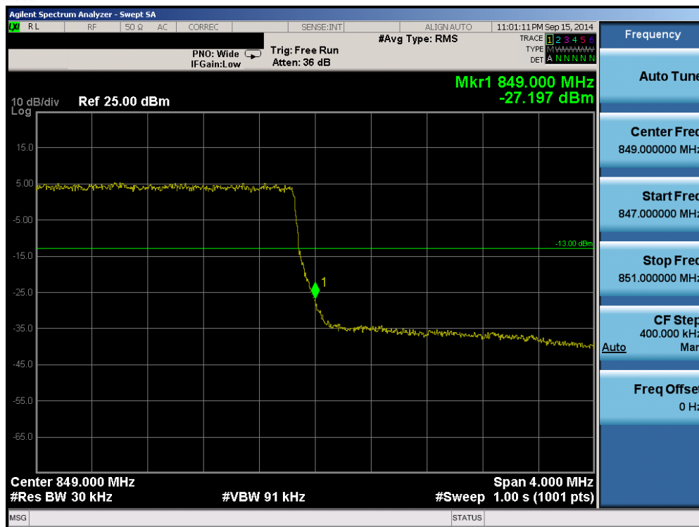
Plot 6-39. Upper Band Edge Plot (Band 5 - 3.0MHz QPSK - RB Size 15)
