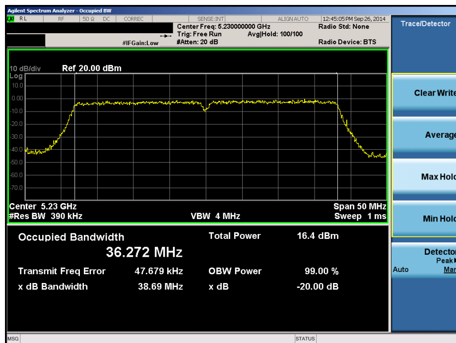
Plot 6-61. 20dB Bandwidth Plot (40MHz BW 802.11n (UNII Band 1) – Ch. 46)
