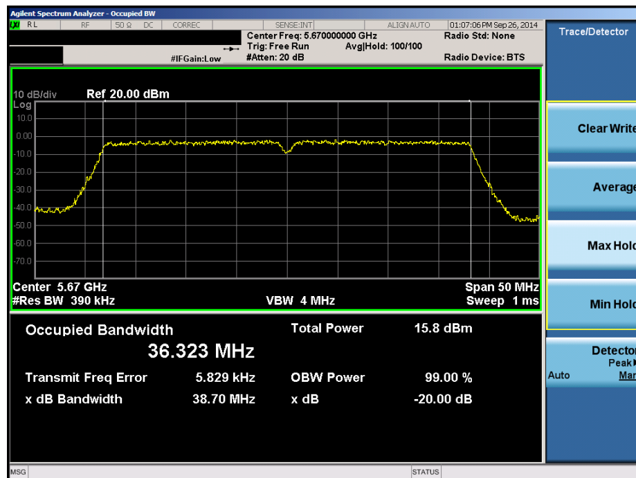
Plot 6-62. 20dB Bandwidth Plot (40MHz BW 802.11n (UNII Band 2C) – Ch. 134)
