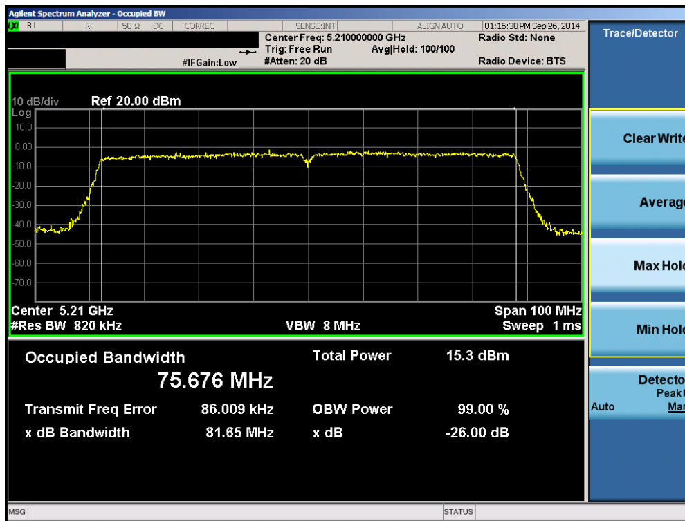
Plot 6-40. 26dB Bandwidth Plot (80MHz BW 802.11ac (UNII Band 1) – Ch. 42)
