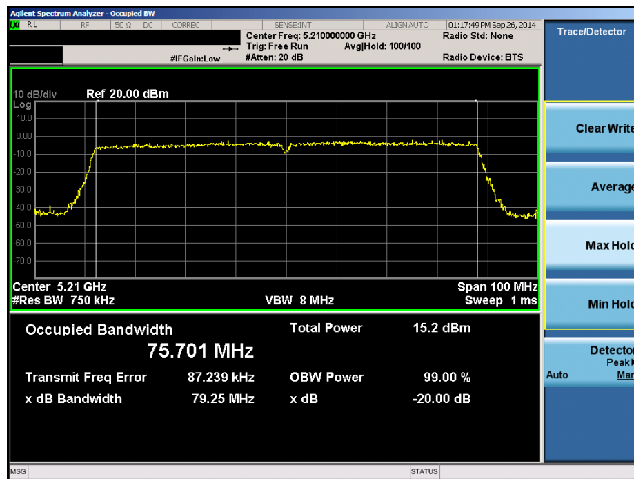
Plot 6-63. 20dB Bandwidth Plot (80MHz BW 802.11ac (UNII Band 1) – Ch. 42)
