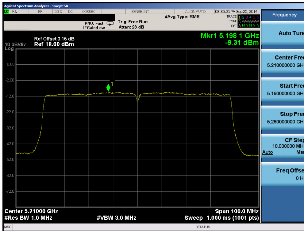
Plot 6-72. Peak Power Spectral Density Plot (80MHz BW 802.11ac (UNII Band 1) – Ch. 42)
