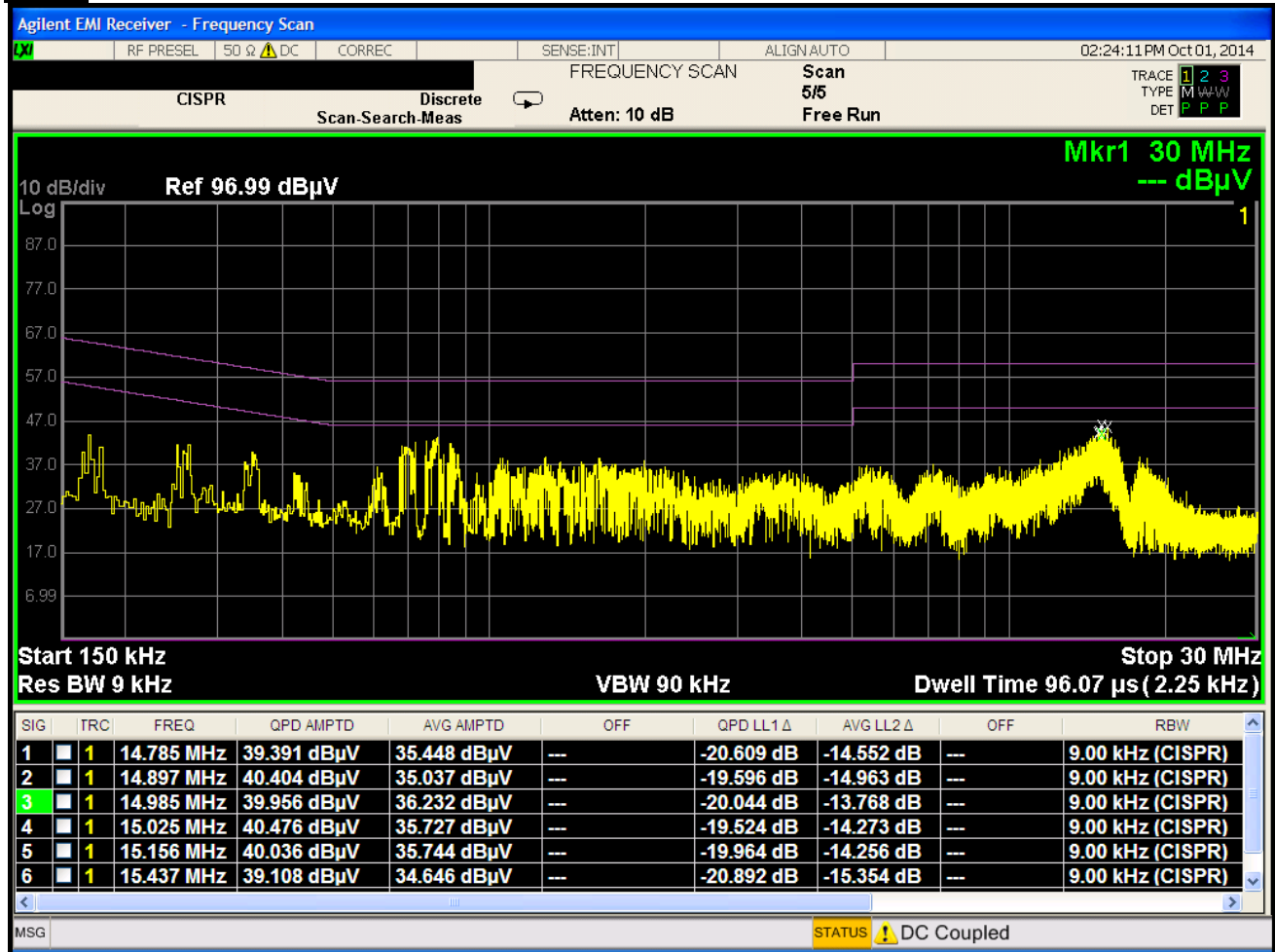
Plot 6-193. Line Conducted Plot with 802.11a UNII Band 2C (N)
