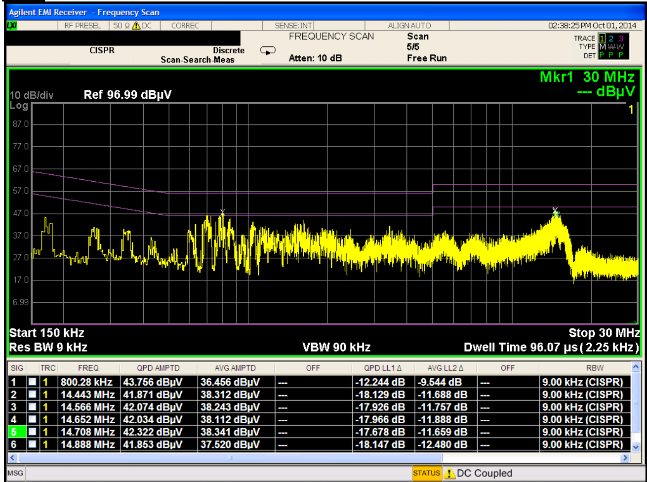
Plot 6-188. Line Conducted Plot with 802.11a UNII Band 1 (L1)
