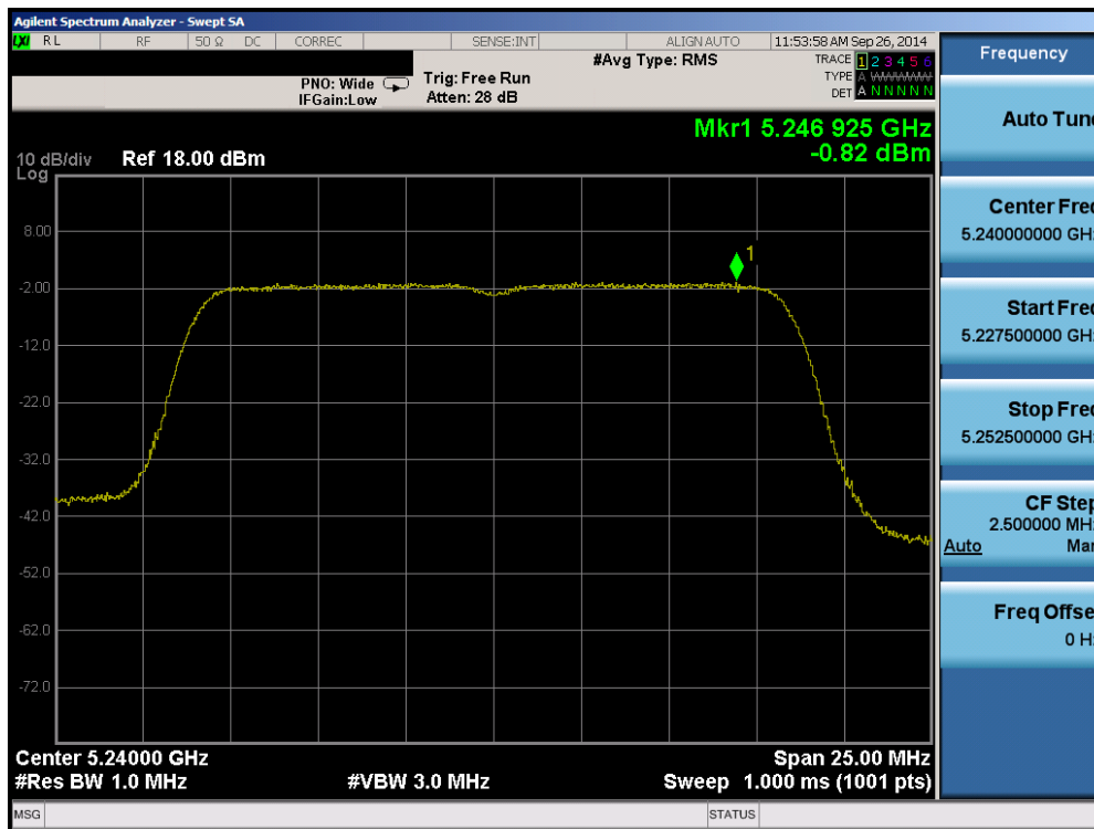
Plot 6-94. Peak Power Spectral Density Plot (802.11a (UNII Band 1) – Ch. 48)
