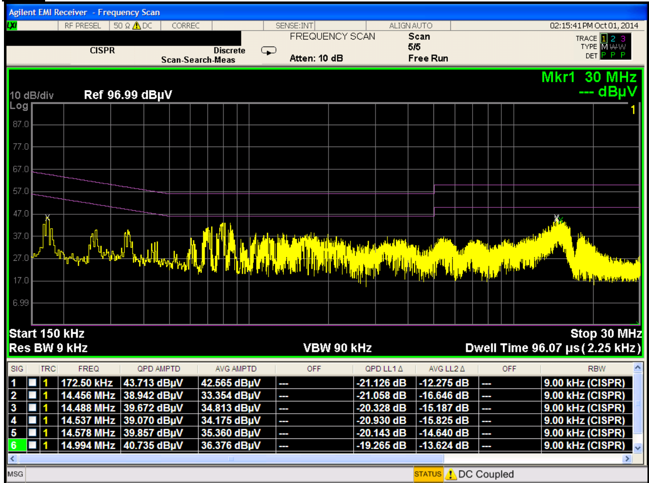
Plot 6-189. Line Conducted Plot with 802.11a UNII Band 1 (N)
