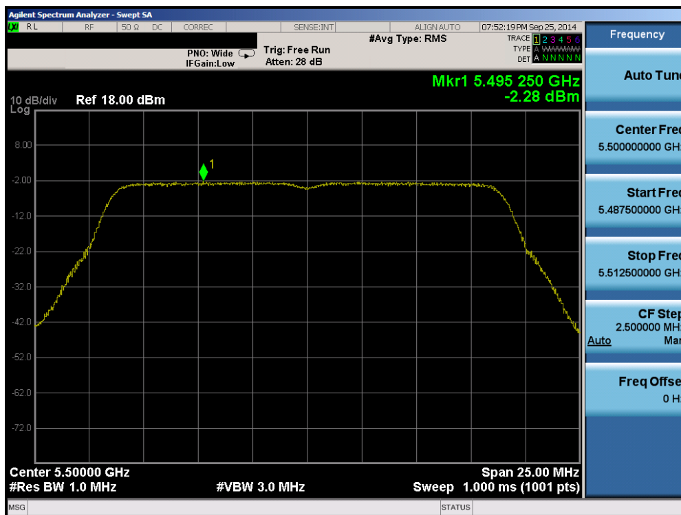
Plot 6-85. Peak Power Spectral Density Plot (20MHz BW 802.11n (UNII Band 2C) – Ch. 100)
