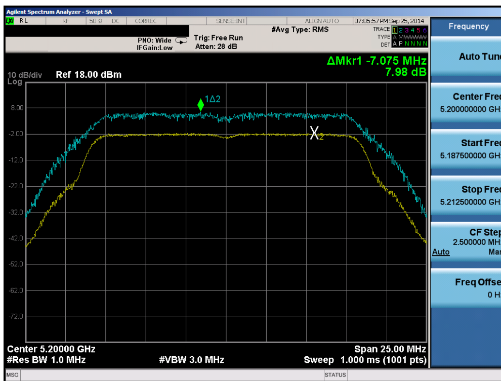
Plot 6-120. Peak Excursion Ratio Plot (802.11a (UNII Band 1) – Ch. 40)
