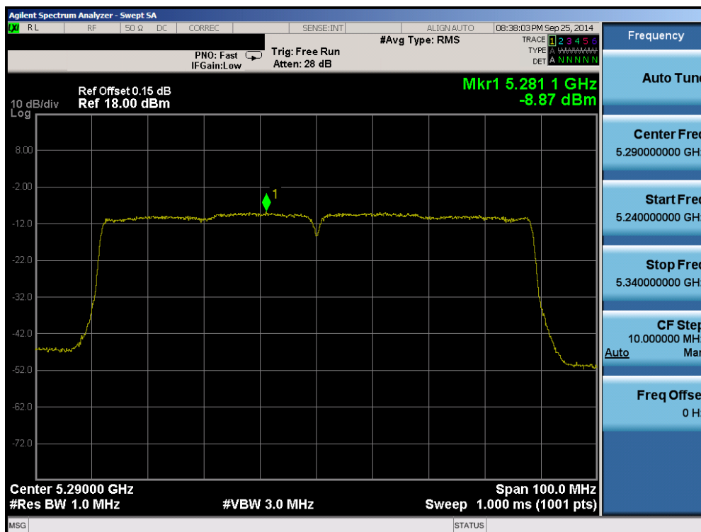
Plot 6-81. Peak Power Spectral Density Plot (80MHz BW 802.11ac (UNII Band 2A) – Ch. 58)
