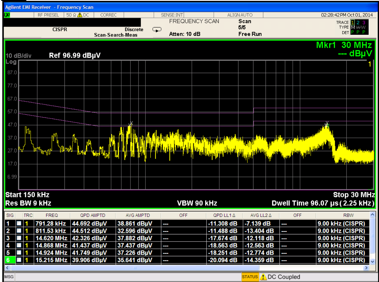
Plot 6-192. Line Conducted Plot with 802.11a UNII Band 2C (L1)
