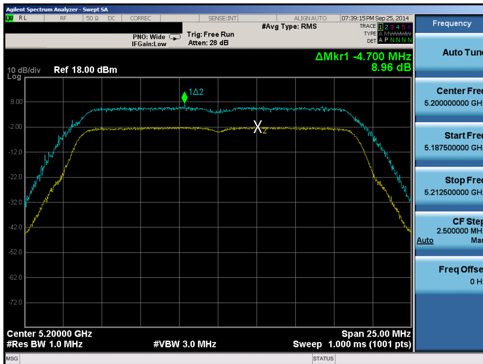
Plot 6-121. Peak Excursion Ratio Plot (20MHz BW 802.11n (UNII Band 1) – Ch. 40)
