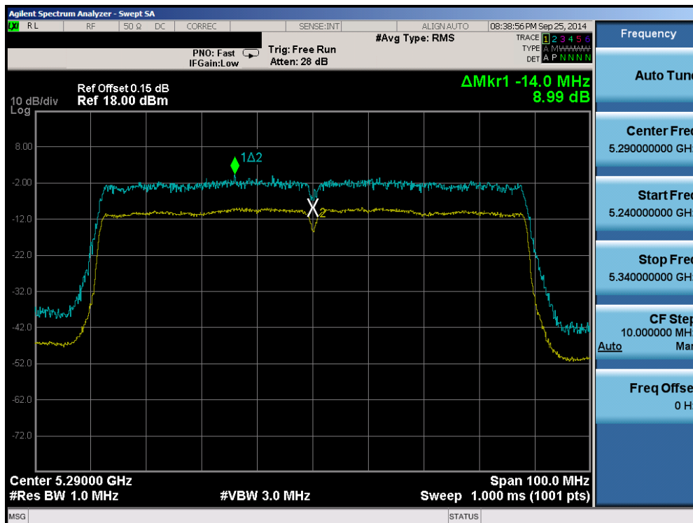
Plot 6-122. Peak Excursion Ratio Plot (80MHz BW 802.11ac (UNII Band 2A) – Ch. 58)
