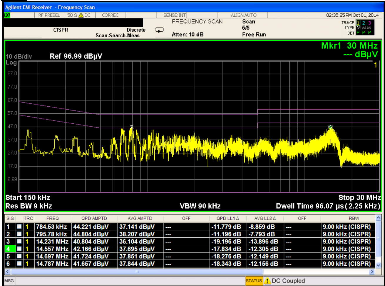
Plot 6-190. Line Conducted Plot with 802.11a UNII Band 2A (L1)
