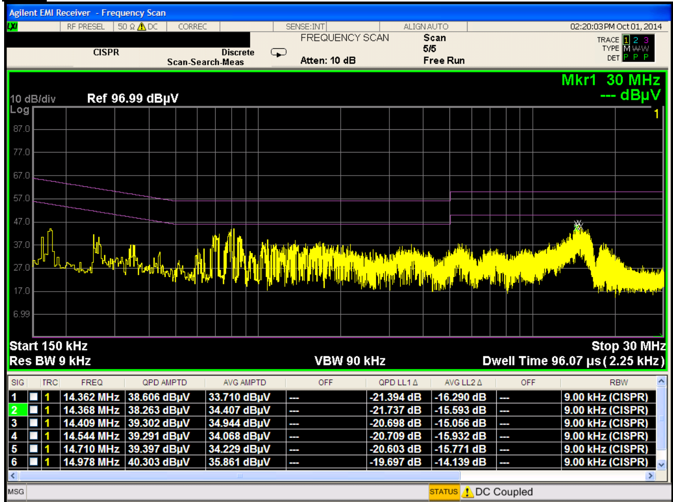
Plot 6-191. Line Conducted Plot with 802.11a UNII Band 2A (N)
