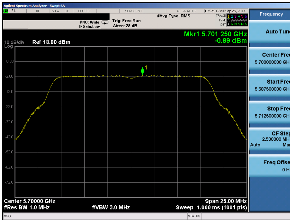
Plot 6-84. Peak Power Spectral Density Plot (802.11a (UNII Band 2C) – Ch. 140)
