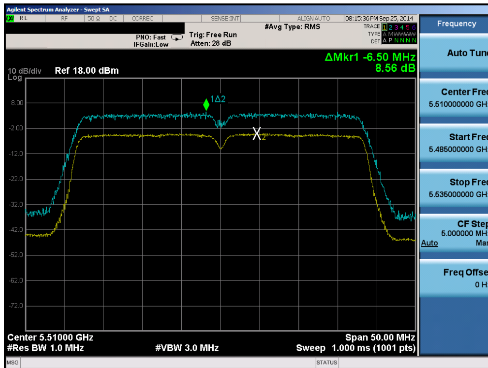
Plot 6-123. Peak Excursion Ratio Plot (40MHz BW 802.11n (UNII Band 2C) – Ch. 102)
