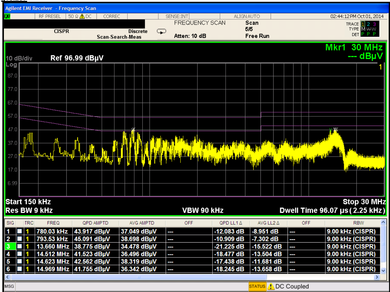
Plot 6-137. Line Conducted Plot with 802.11a (L1)
