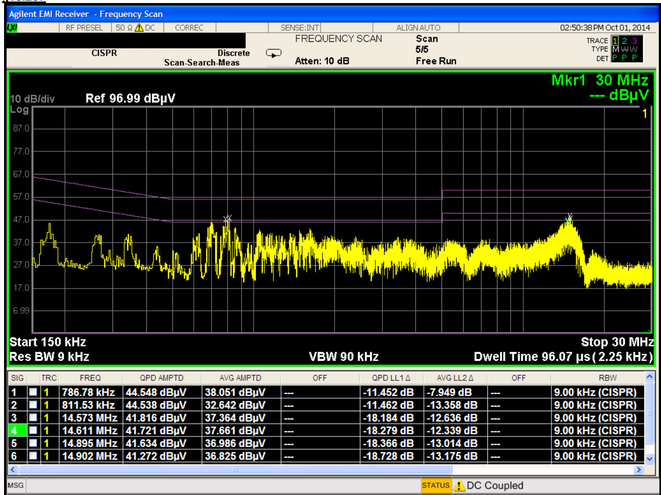
Plot 6-135. Line Conducted Plot with 802.11b (L1)
