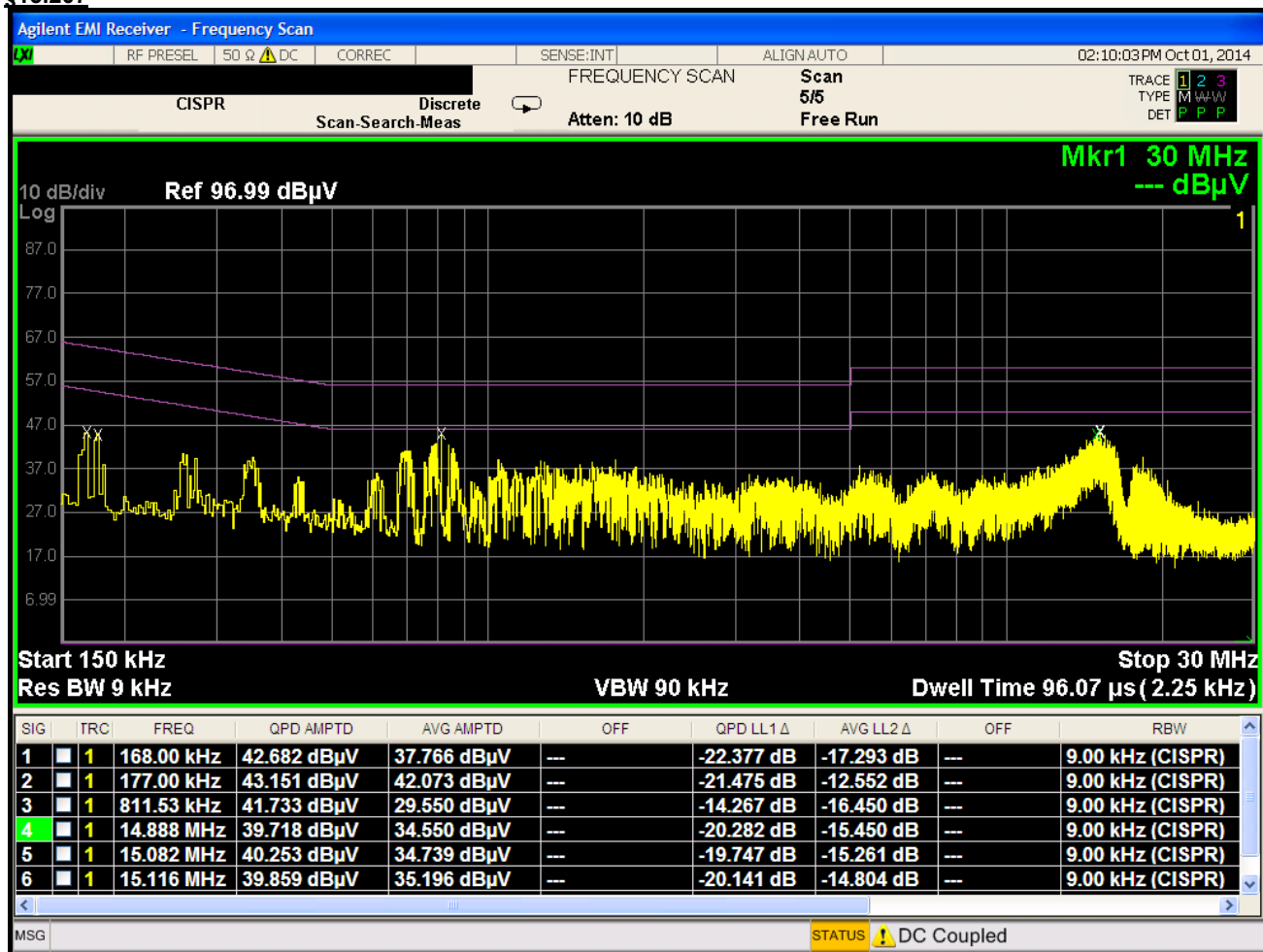
Plot 6-138. Line Conducted Plot with 802.11a (N)
