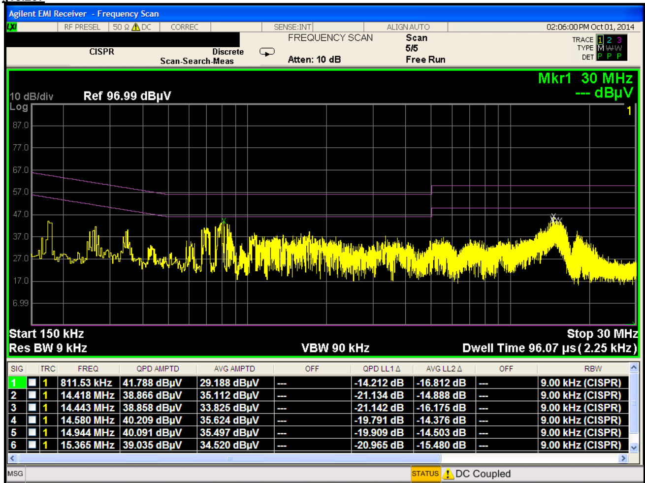
Plot 6-136. Line Conducted Plot with 802.11b (N)
