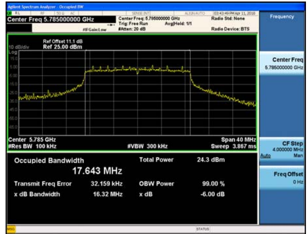
802.11n_HT20 UNII 3 BAND 6dB Bandwidth(CH.157)
