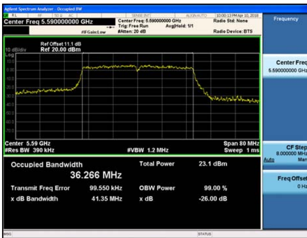
802.11n_HT40 UNII 2C BAND 26dB Bandwidth(CH 118)
