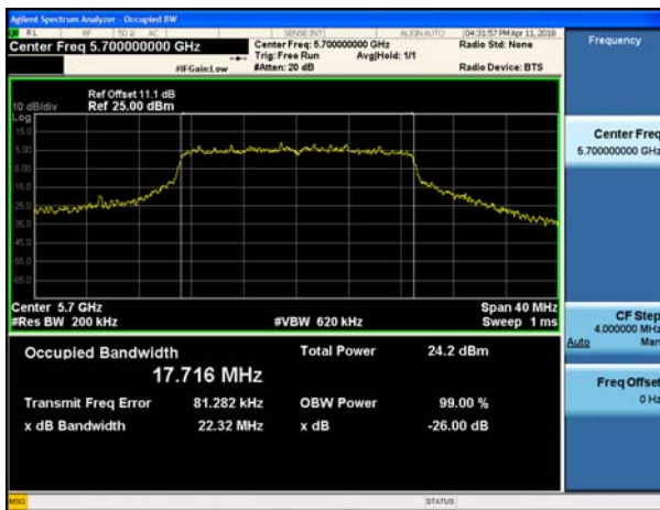
802.11ac_VHT20 UNII 2C BAND 26dB Bandwidth(CH 140)
