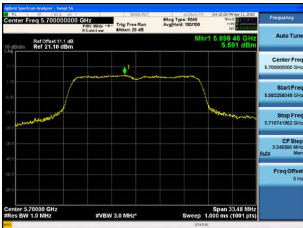
802.11ac_VHT20 UNII 2C BAND PSD CH 140
