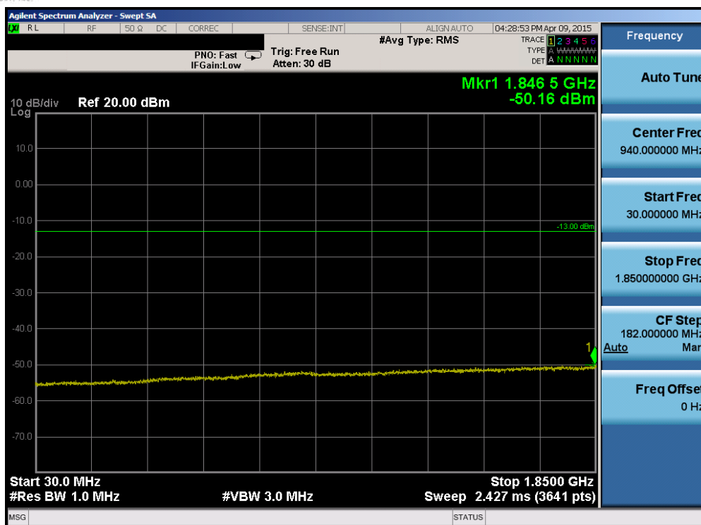
Plot 6-75. Conducted Spurious Plot (Band 2 – 1.4MHz QPSK – RB Size 1, RB Offset 0 – Mid Channel)
