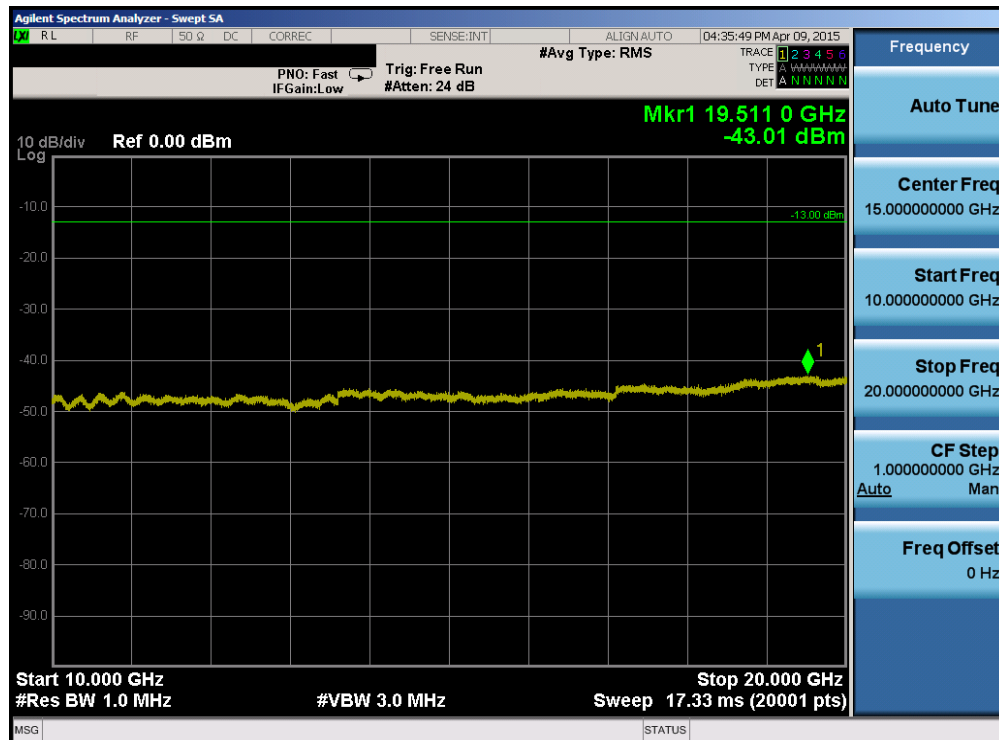
Plot 6-74. Conducted Spurious Plot (Band 2 – 1.4MHz QPSK – RB Size 1, RB Offset 0 – Low Channel)
