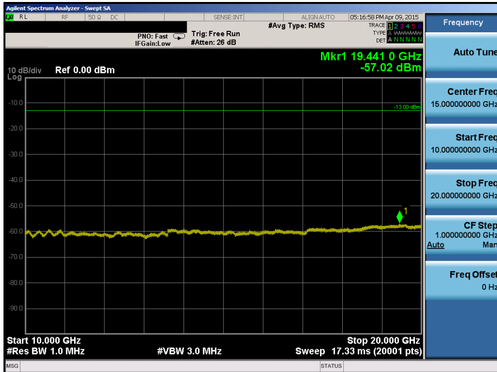
Plot 6-80. Conducted Spurious Plot (Band 2 – 1.4MHz QPSK – RB Size 1, RB Offset 0 – High Channel)
