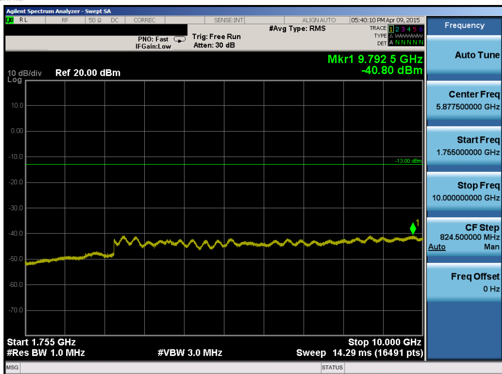
Plot 6-67. Conducted Spurious Plot (Band 4 – 1.4MHz QPSK – RB Size 1, RB Offset 0 – Mid Channel)
