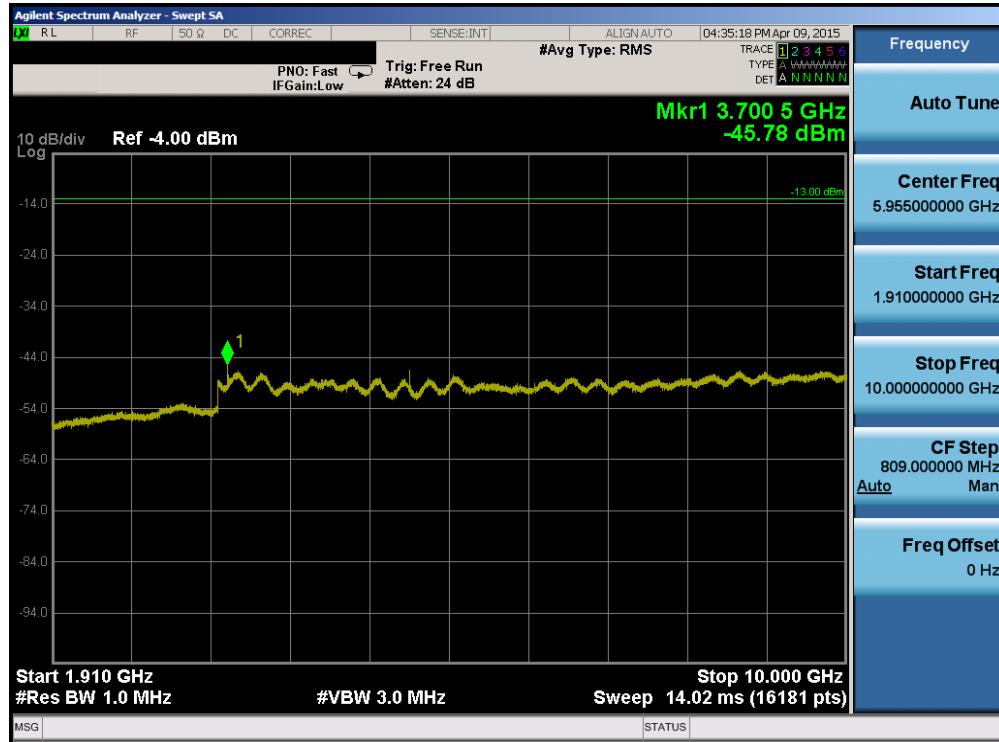
Plot 6-73. Conducted Spurious Plot (Band 2 – 1.4MHz QPSK – RB Size 1, RB Offset 0 – Low Channel)
