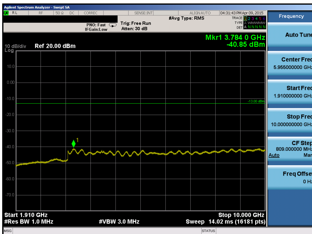
Plot 6-76. Conducted Spurious Plot (Band 2 – 1.4MHz QPSK – RB Size 1, RB Offset 0 – Mid Channel)
