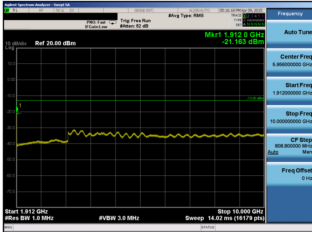
Plot 6-79. Conducted Spurious Plot (Band 2 – 1.4MHz QPSK – RB Size 1, RB Offset 0 – High Channel)
