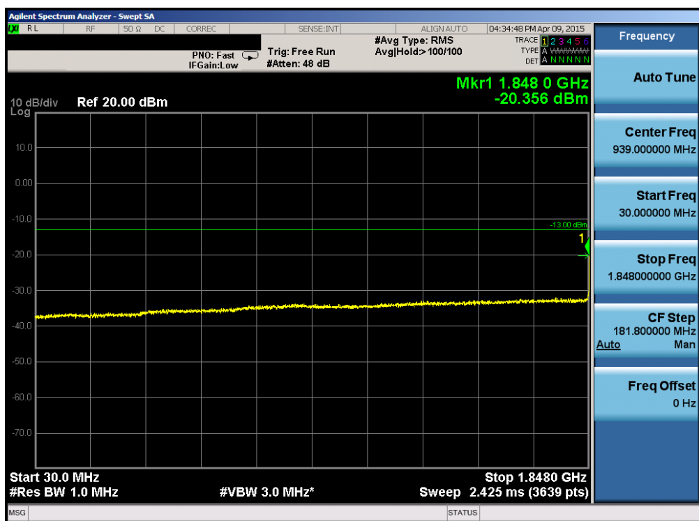
Plot 6-72. Conducted Spurious Plot (Band 2 – 1.4MHz QPSK – RB Size 1, RB Offset 0 – Low Channel)
