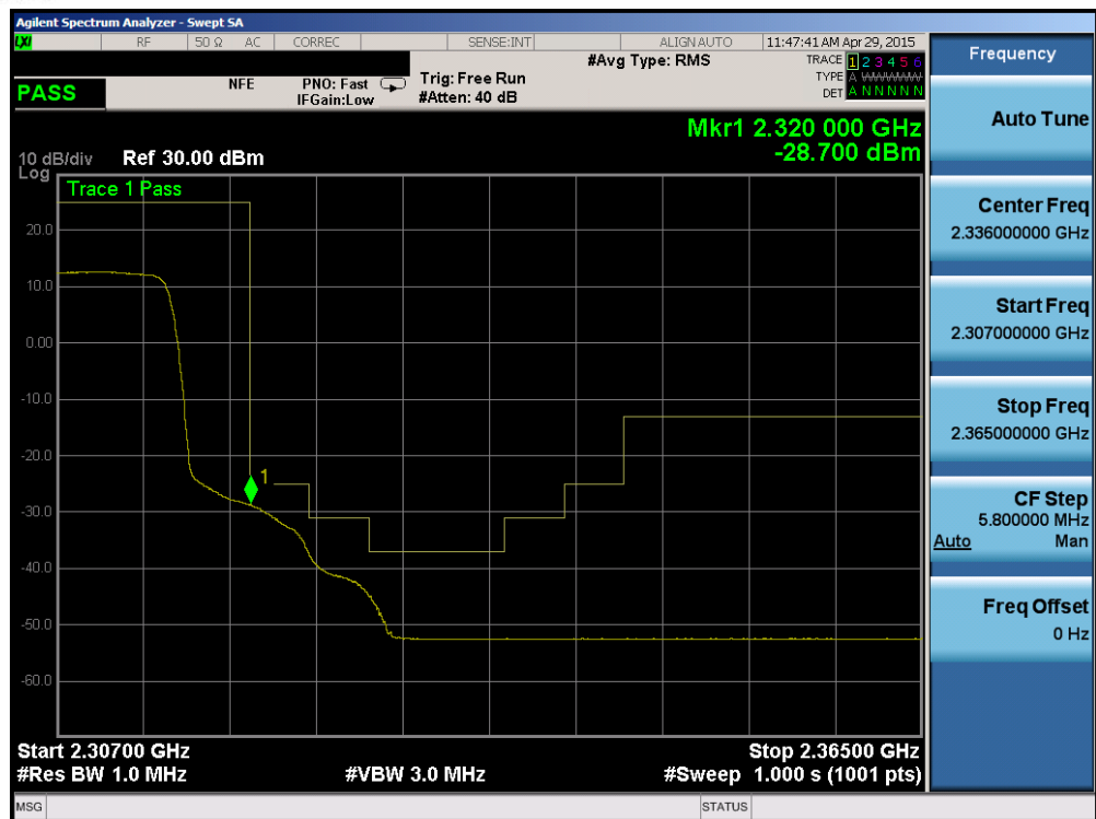
Plot 6-167. Upper Extended Band Edge Plot (Band 30 – 10MHz QPSK – RB Size 50)
