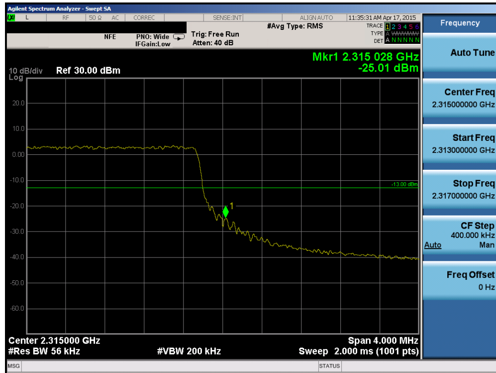
Plot 6-162. Upper Band Edge Plot (Band 30 – 5MHz QPSK – RB Size 25)
