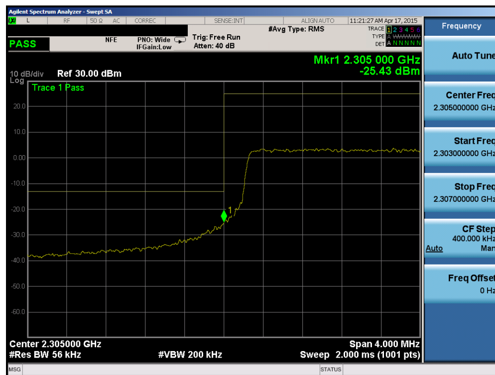
Plot 6-160. Lower Band Edge Plot (Band 30 – 5MHz QPSK – RB Size 25)
