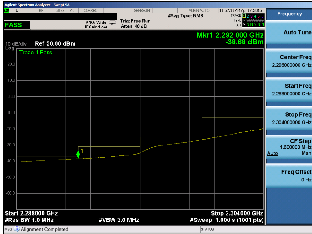
Plot 6-165. Lower Extended Band Edge Plot (Band 30 – 10MHz QPSK – RB Size 50)
