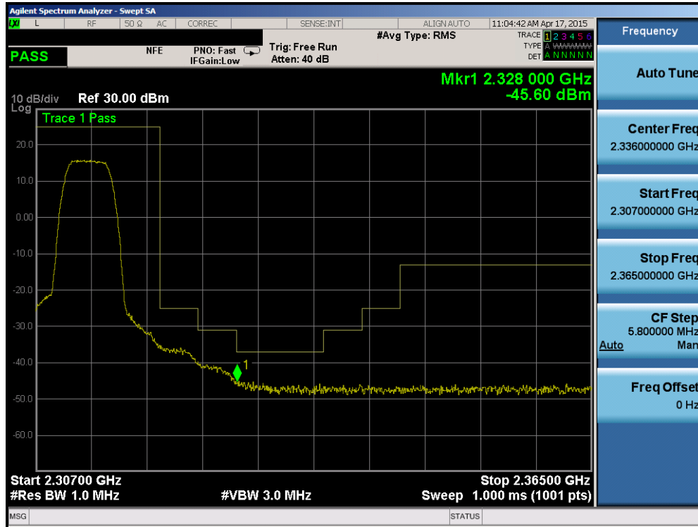
Plot 6-163. Upper Extended Band Edge Plot (Band 30 – 5MHz QPSK – RB Size 25)
