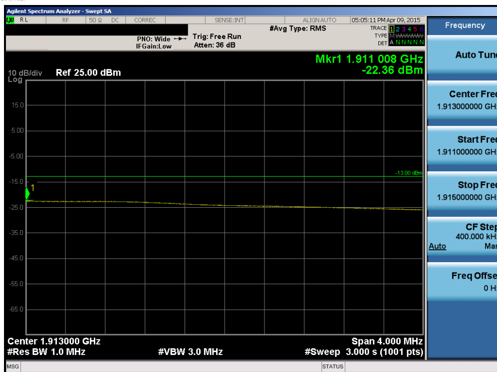
Plot 6-155. Upper Extended Band Edge Plot (Band 2 – 15.0MHz QPSK – RB Size 75)
