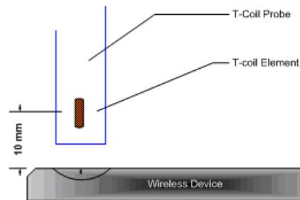
Figure 4-10 Measurement Distance
