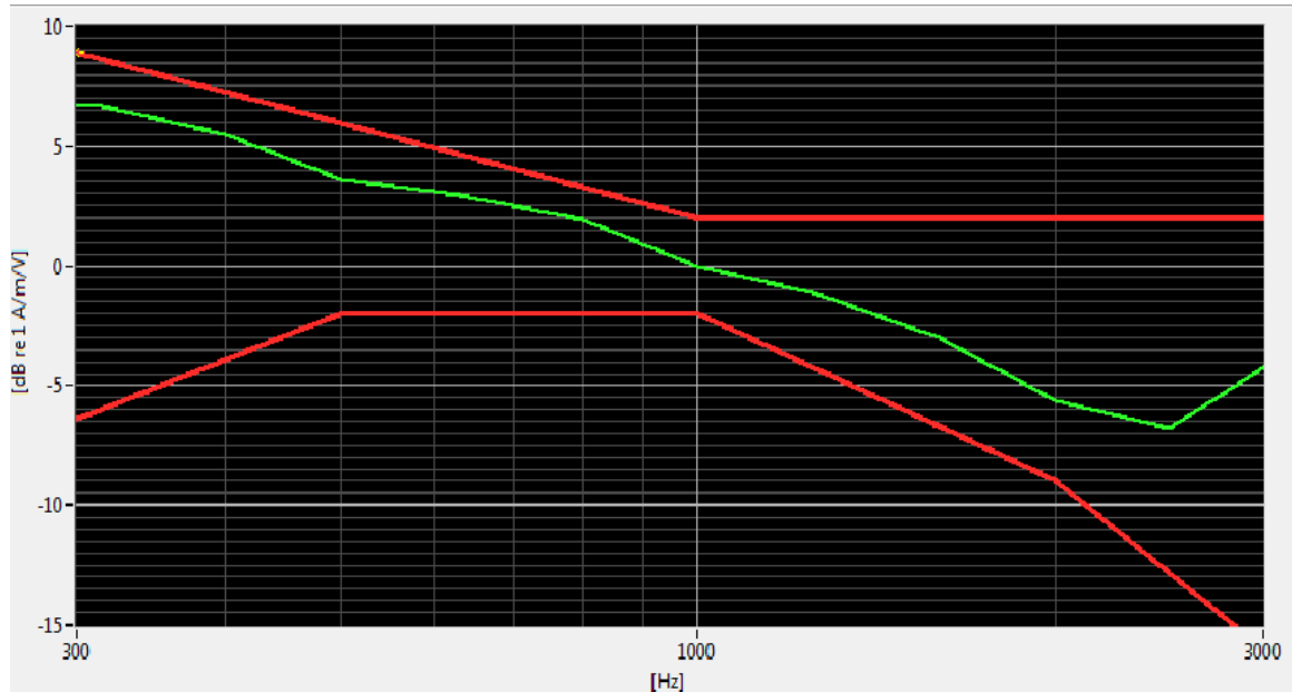
Figure 7-1 Axial Frequency Response
