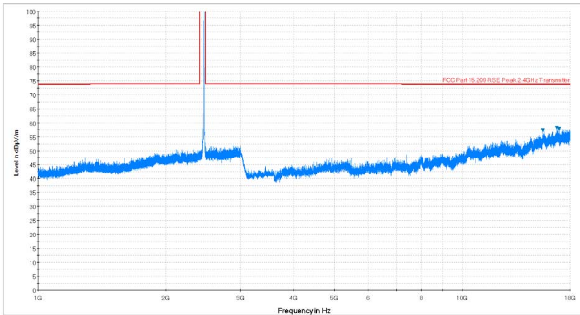
Plot 6-74. Radiated Spurious Plot above 1GHz (802.11b – Ch. 11, Ant. Pol. V)
