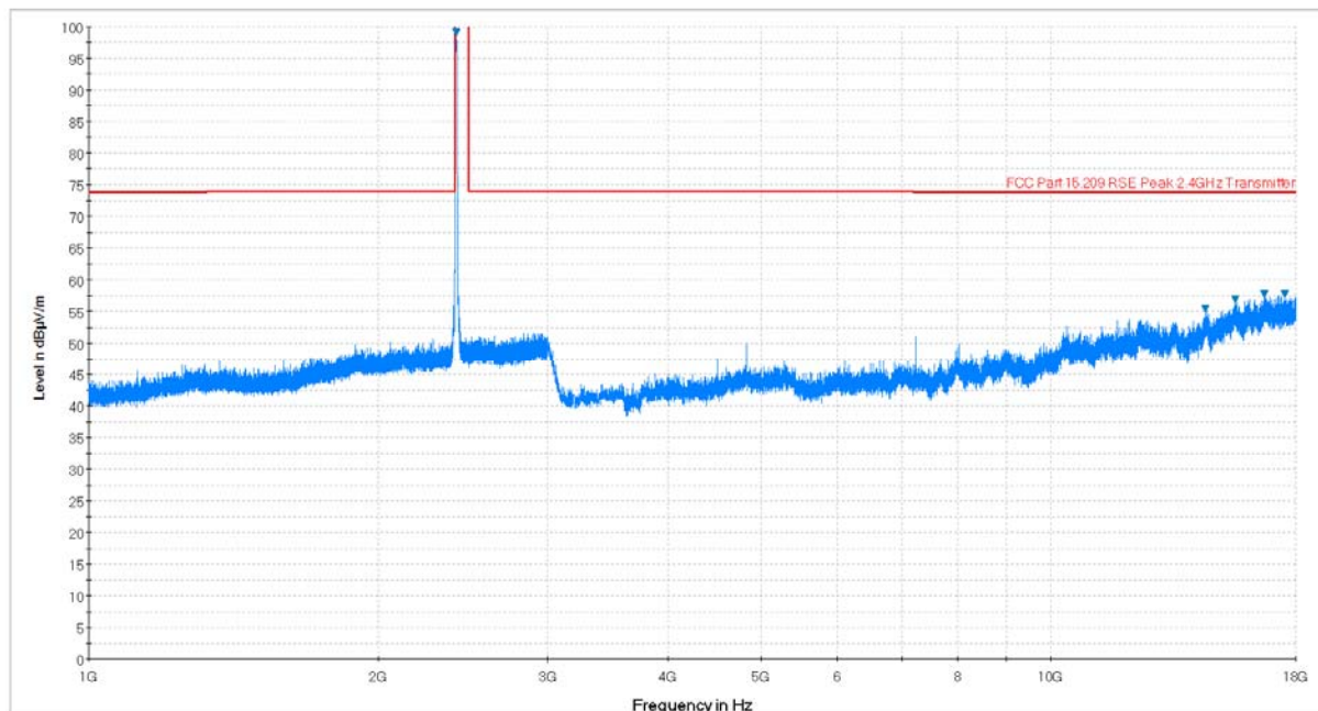
Plot 6-62. Radiated Spurious Plot above 1GHz (802.11b – Ch. 1, Ant. Pol. V)
