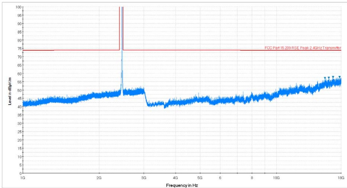
Plot 6-66. Radiated Spurious Plot above 1GHz (802.11b – Ch. 11, Ant. Pol. V)
