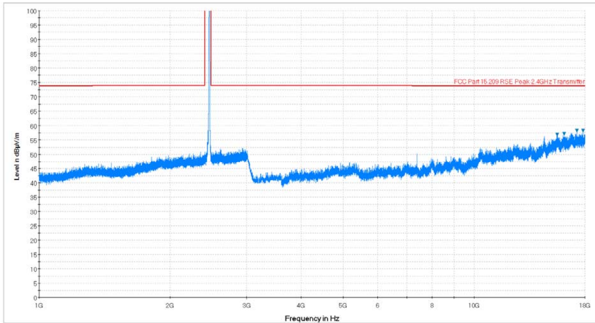
Plot 6-73. Radiated Spurious Plot above 1GHz (802.11b – Ch. 11, Ant. Pol. H)
