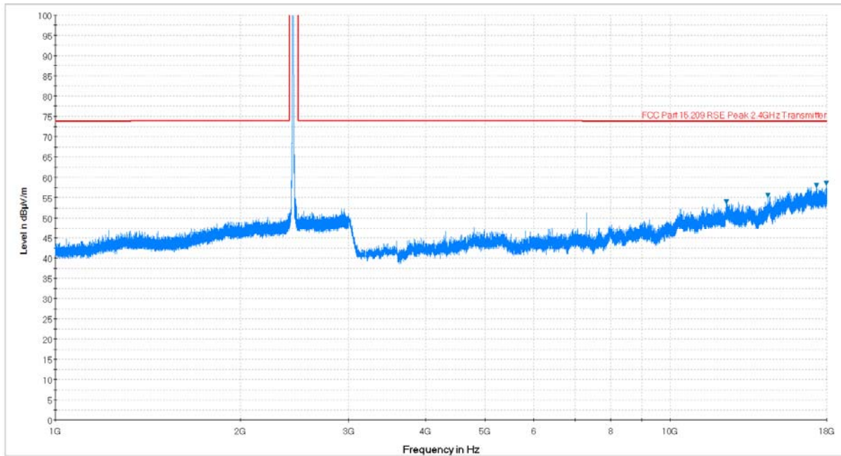
Plot 6-71. Radiated Spurious Plot above 1GHz (802.11b – Ch. 6, Ant. Pol. H)
