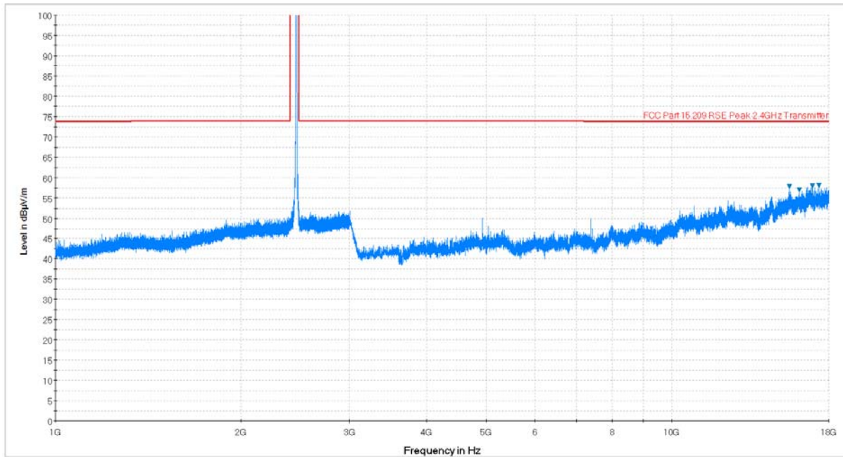
Plot 6-65. Radiated Spurious Plot above 1GHz (802.11b – Ch. 11, Ant. Pol. H)
