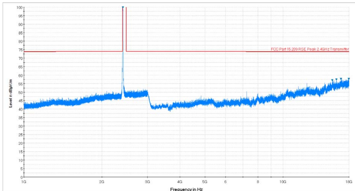
Plot 6-70. Radiated Spurious Plot above 1GHz (802.11b – Ch. 1, Ant. Pol. V)
