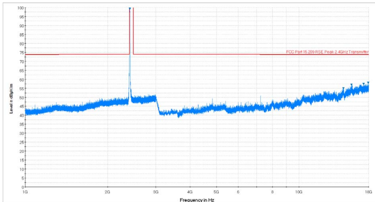
Plot 6-69. Radiated Spurious Plot above 1GHz (802.11b – Ch. 1, Ant. Pol. H)
