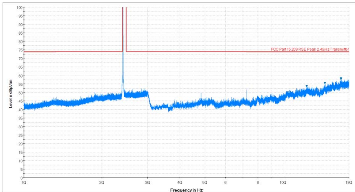
Plot 6-61. Radiated Spurious Plot above 1GHz (802.11b – Ch. 1, Ant. Pol. H)
