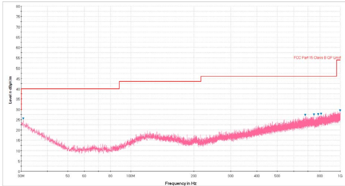
Plot 6-89. Radiated Spurious Plot below 1GHz (Pol. H)
