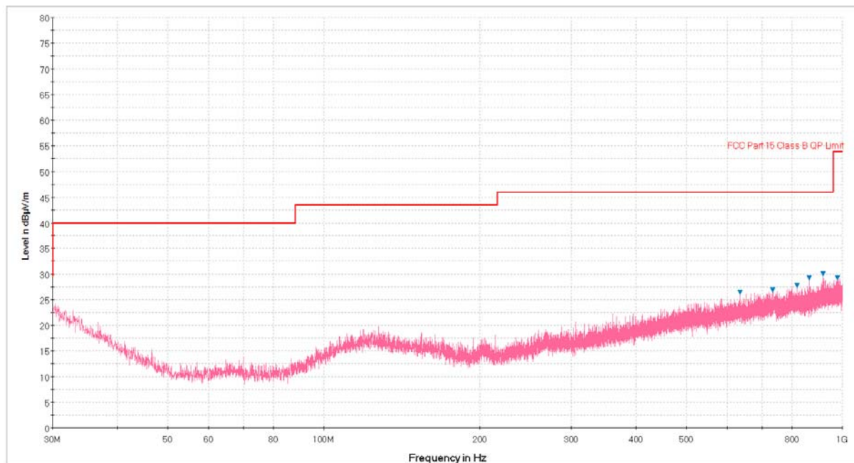
Plot 6-90. Radiated Spurious Plot below 1GHz (Pol. V)
