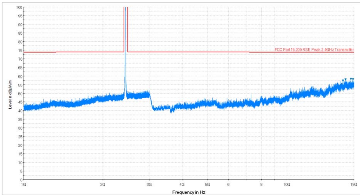
Plot 6-64. Radiated Spurious Plot above 1GHz (802.11b – Ch. 6, Ant. Pol. V)
