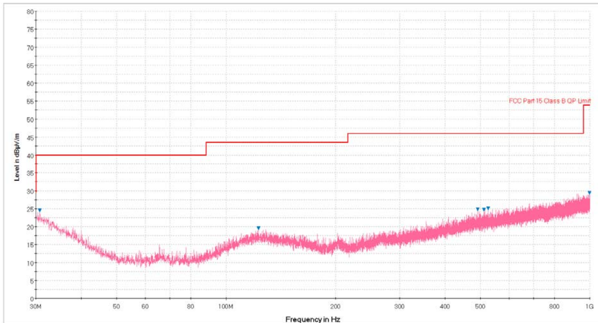
Plot 6-92. Radiated Spurious Plot below 1GHz (Pol. V)
