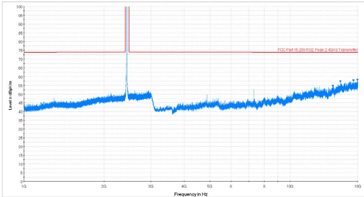
Plot 6-63. Radiated Spurious Plot above 1GHz (802.11b – Ch. 6, Ant. Pol. H)
