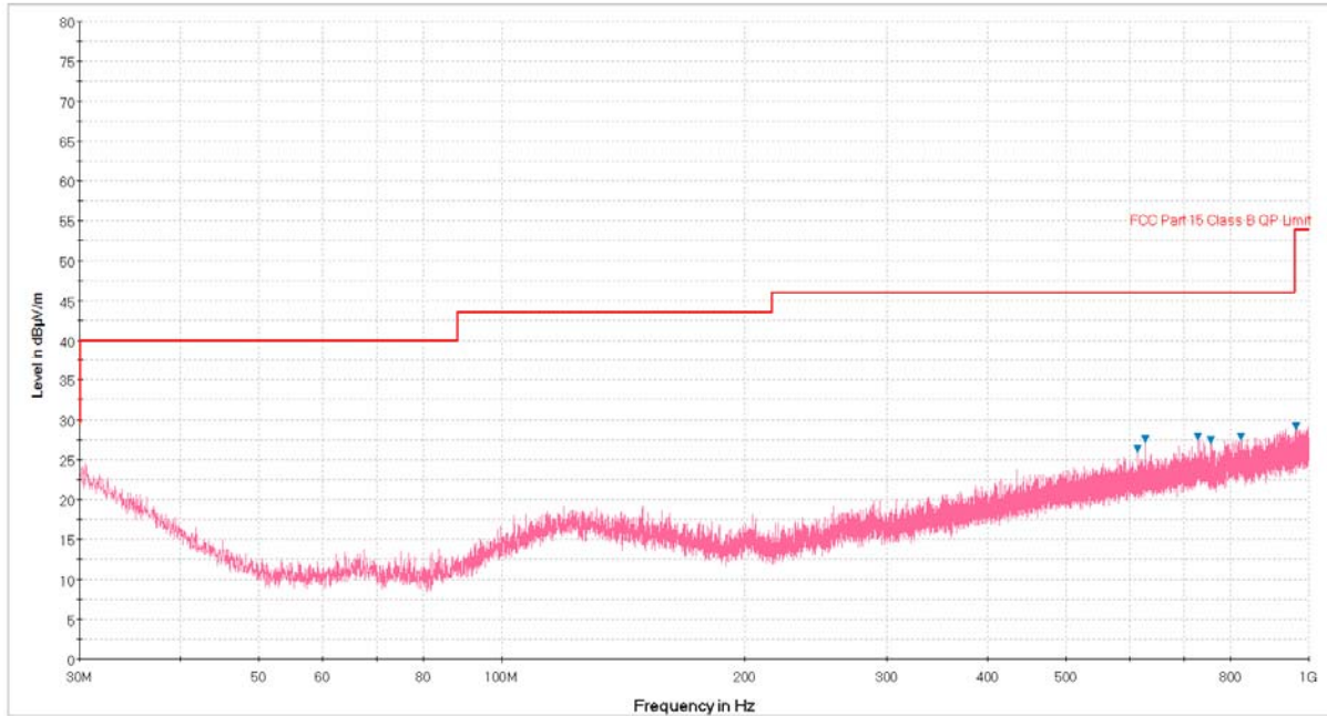
Plot 6-91. Radiated Spurious Plot below 1GHz (Pol. H)
