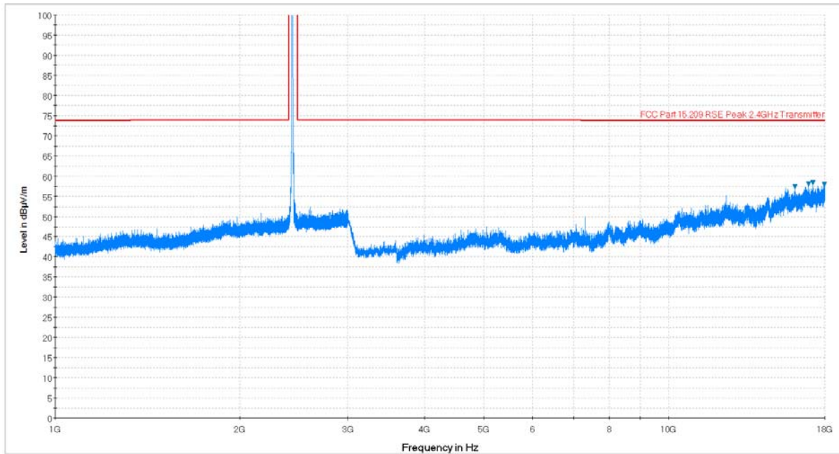
Plot 6-72. Radiated Spurious Plot above 1GHz (802.11b – Ch. 6, Ant. Pol. V)
