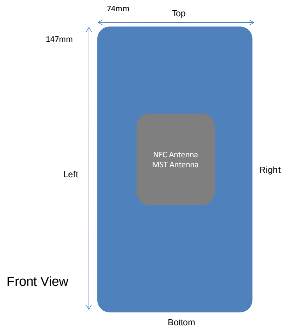
Figure F-2 NFC Antenna Locations
