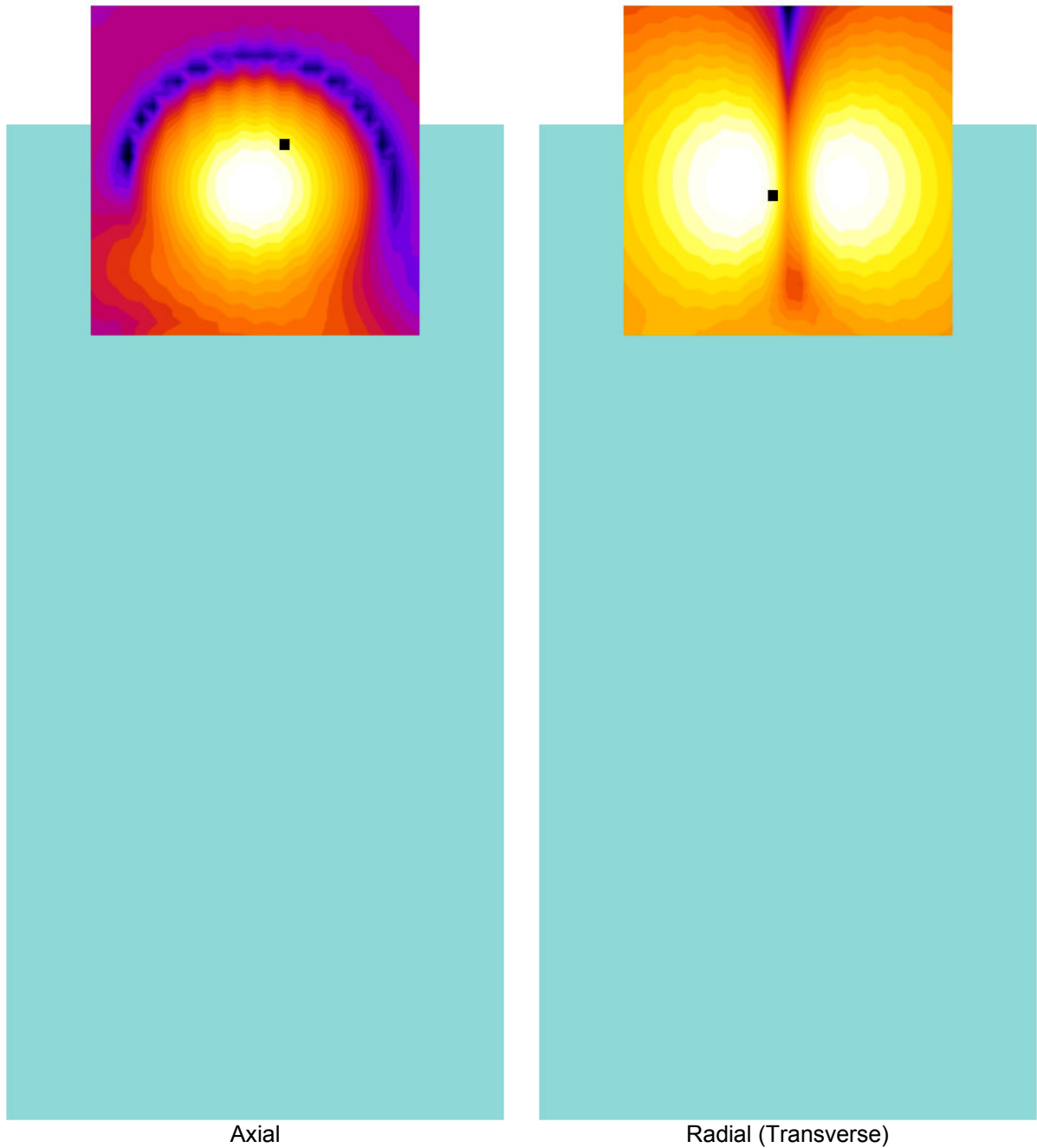
Figure 7-1 T-Coil Scan Overlay Magnetic Field Distributions
