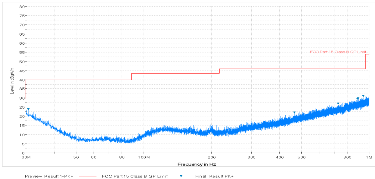
Plot 7-55. Radiated Spurious Plot below 1GHz (Pol. V)
