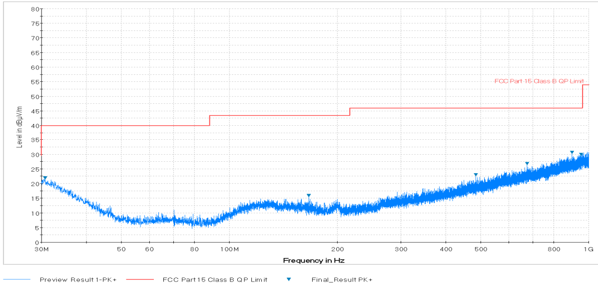
Plot 7-54. Radiated Spurious Plot below 1GHz (Pol. H)
