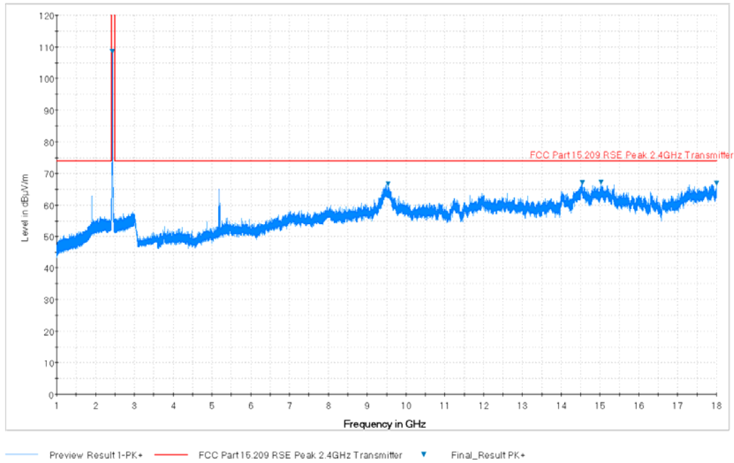
Plot 7-72. Radiated Spurious Plot above 1GHz (802.11b – Ch. 6, Ant. Pol. V)
