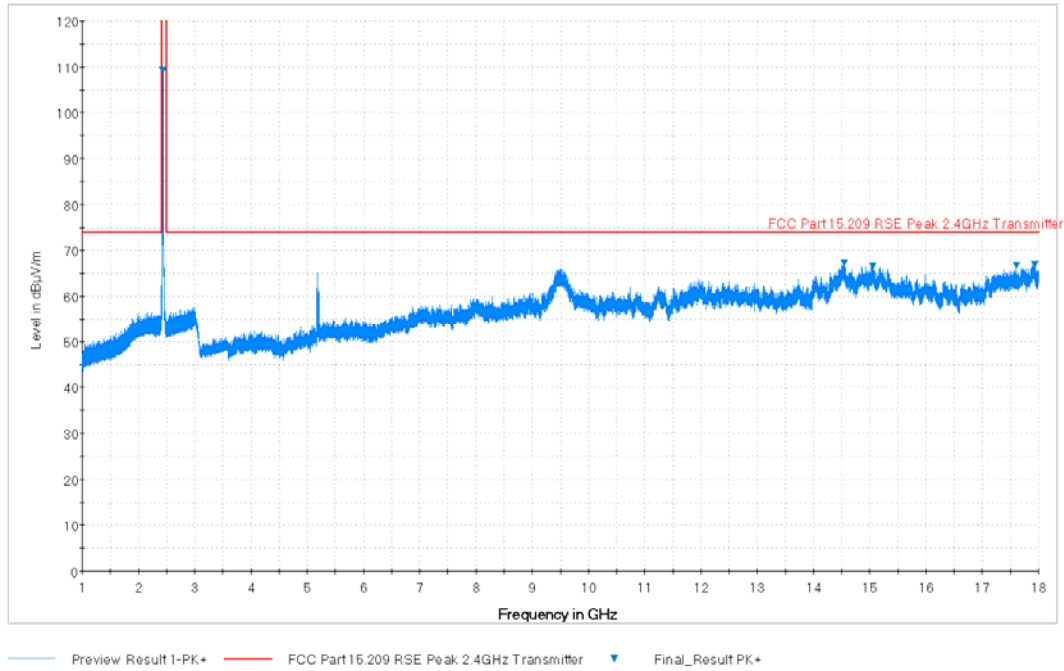
Plot 7-71. Radiated Spurious Plot above 1GHz (802.11b – Ch. 6, Ant. Pol. H)
