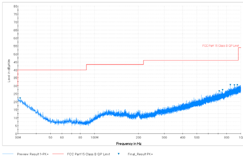
Plot 7-100. Radiated Spurious Plot below 1GHz (Pol. V)
