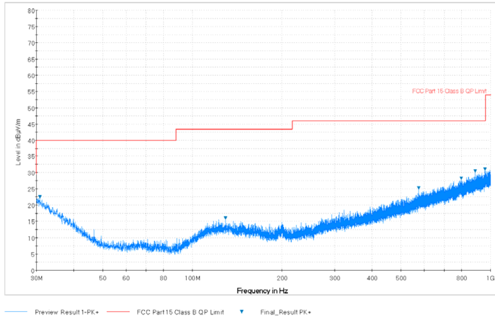
Plot 7-99. Radiated Spurious Plot below 1GHz (Pol. H)
