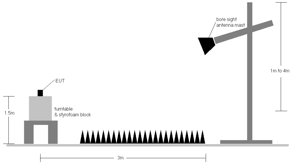
Figure 7-2. Radiated Test Setup
