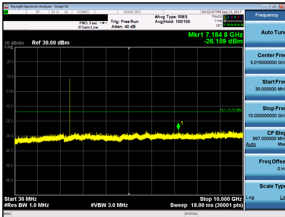
Plot 7-31. Conducted Spurious Plot (Bluetooth (LE), 2Mbps – Ch. 19)
