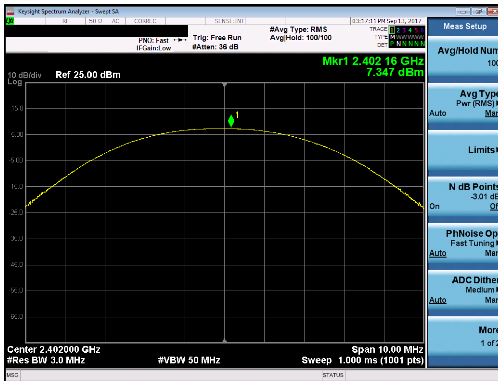
Plot 7-10. Peak Power Plot (Bluetooth (LE), 2Mbps - Ch. 0)
