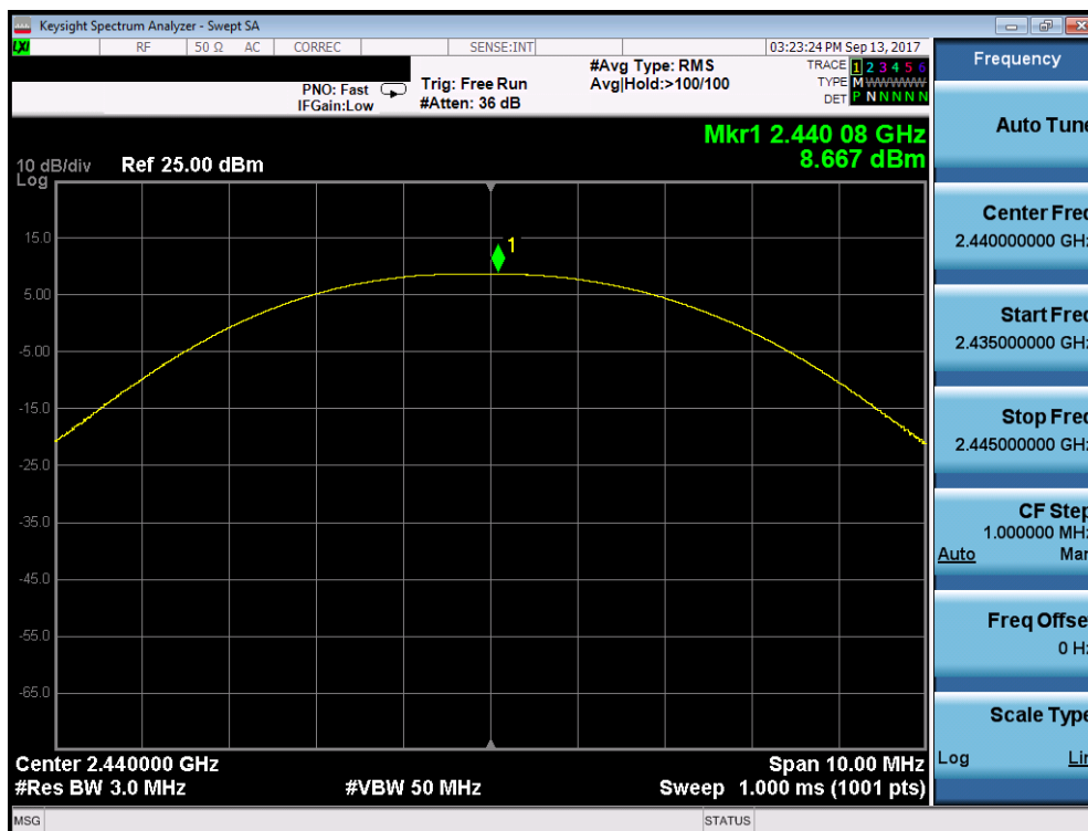
Plot 7-11. Peak Power Plot (Bluetooth (LE), 2Mbps - Ch. 19)
