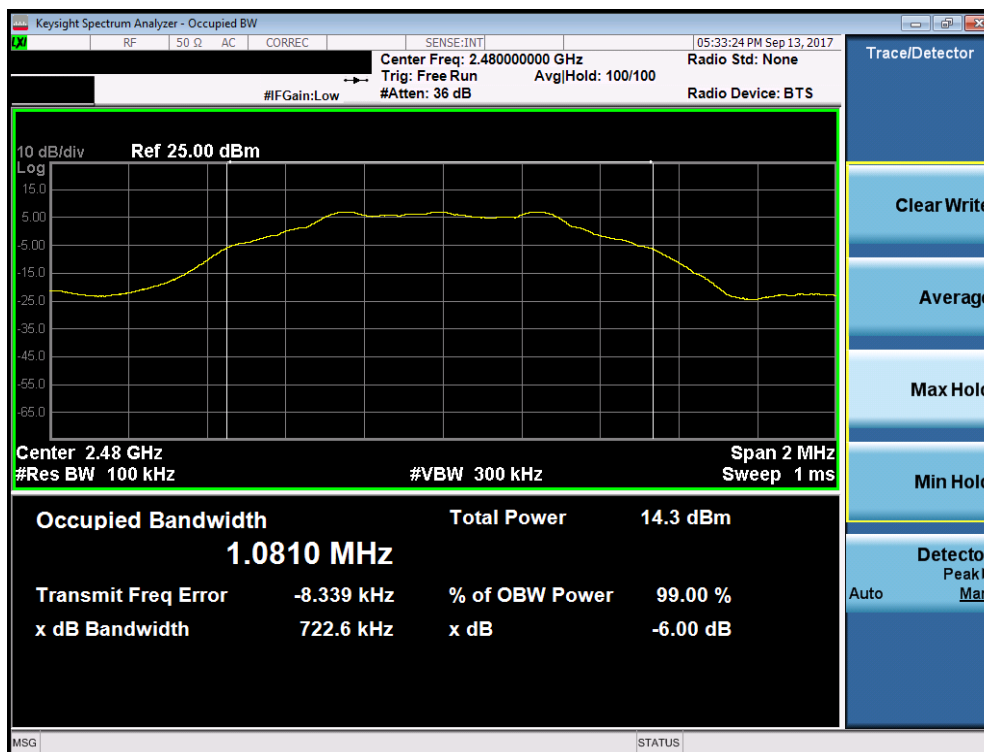
Plot 7-3. 6dB Bandwidth Plot (Bluetooth (LE), 1Mbps – Ch. 39)
