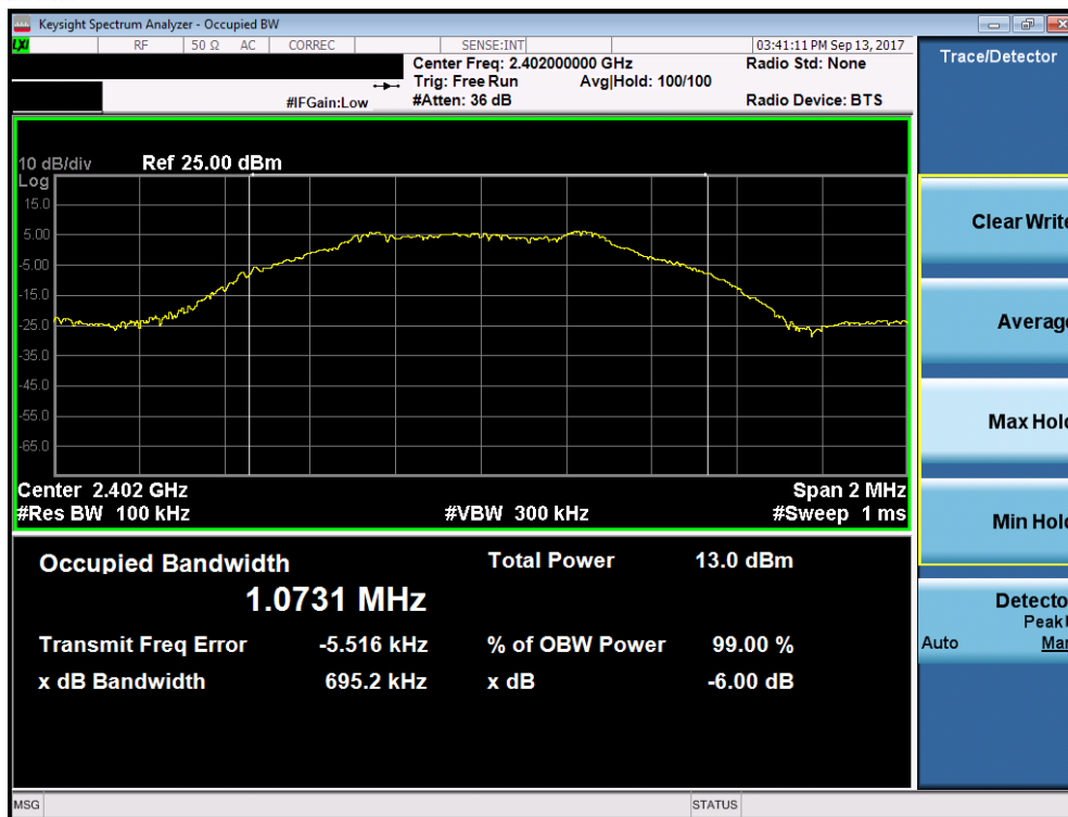
Plot 7-4. 6dB Bandwidth Plot (Bluetooth (LE), 2Mbps - Ch. 0)
