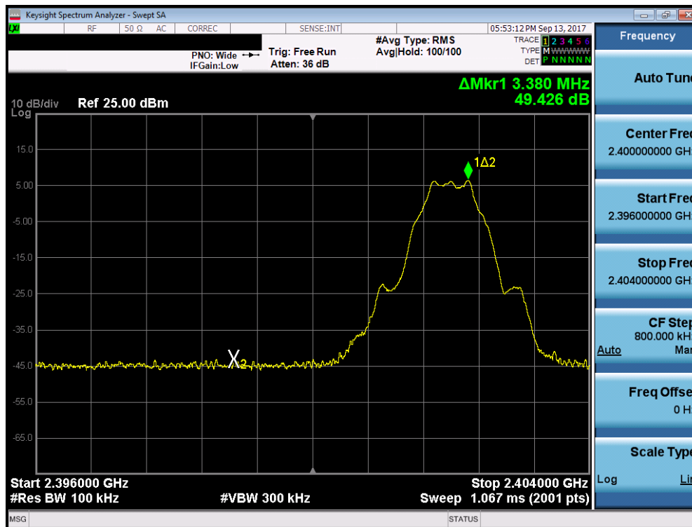
Plot 7-19. Band Edge Plot (Bluetooth (LE), 1Mbps - Ch. 0)
