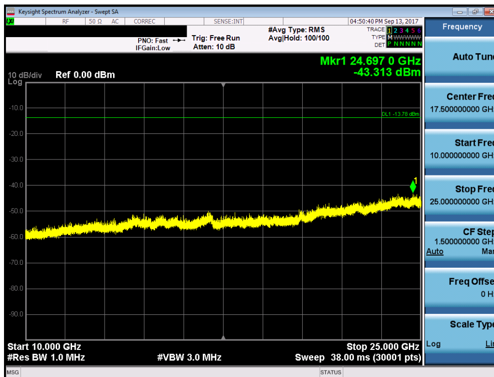
Plot 7-32. Conducted Spurious Plot (Bluetooth (LE), 2Mbps – Ch. 19)
