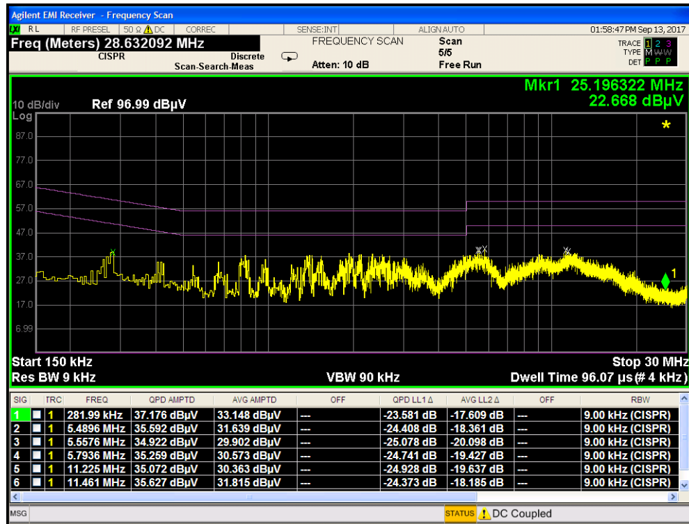
Plot 7-40. Line Conducted Plot with Bluetooth LE (N)
