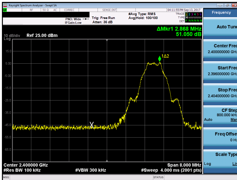
Plot 7-21. Band Edge Plot (Bluetooth (LE), 2Mbps - Ch. 0)
