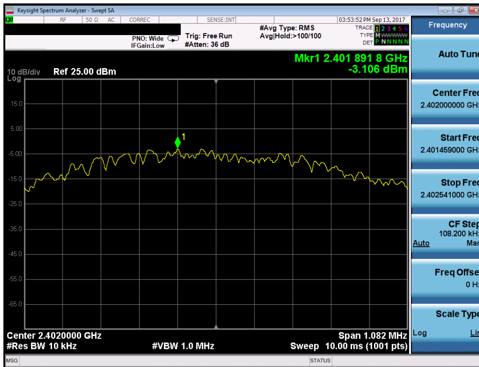
Plot 7-16. Power Spectral Density Plot (Bluetooth (LE), 2Mbps - Ch. 0)
