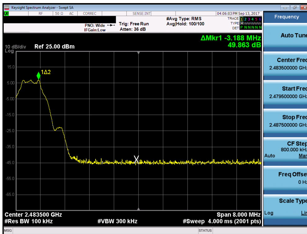
Plot 7-22. Band Edge Plot (Bluetooth (LE), 2Mbps - Ch. 39)
