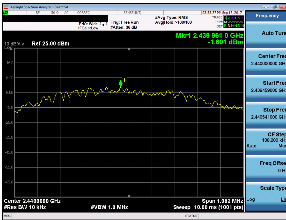
Plot 7-17. Power Spectral Density Plot (Bluetooth (LE), 2Mbps - Ch. 19)
