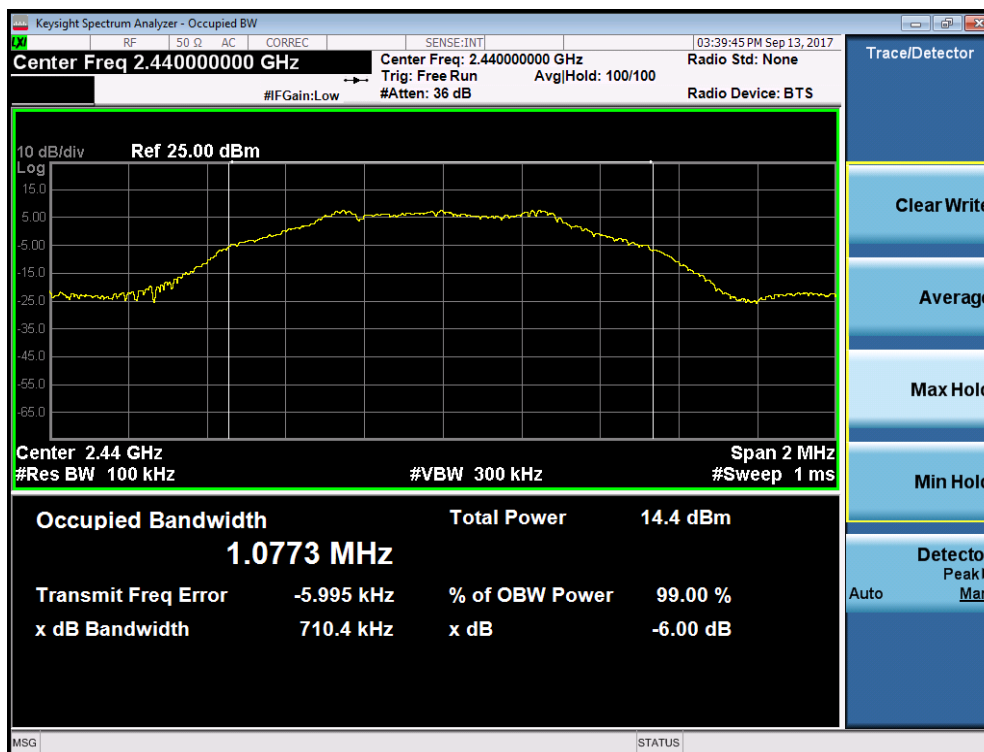
Plot 7-5. 6dB Bandwidth Plot (Bluetooth (LE), 2Mbps - Ch. 19)
