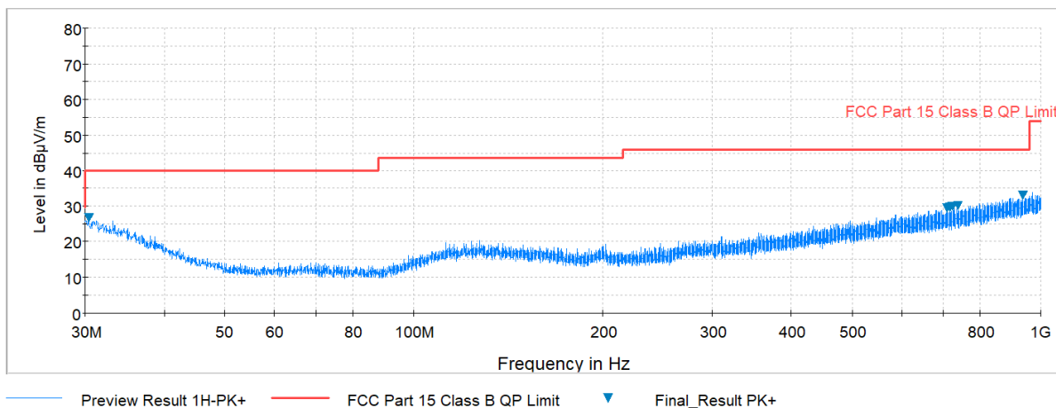
Plot 7-54. Radiated Spurious Plot below 1GHz (Pol. H)
