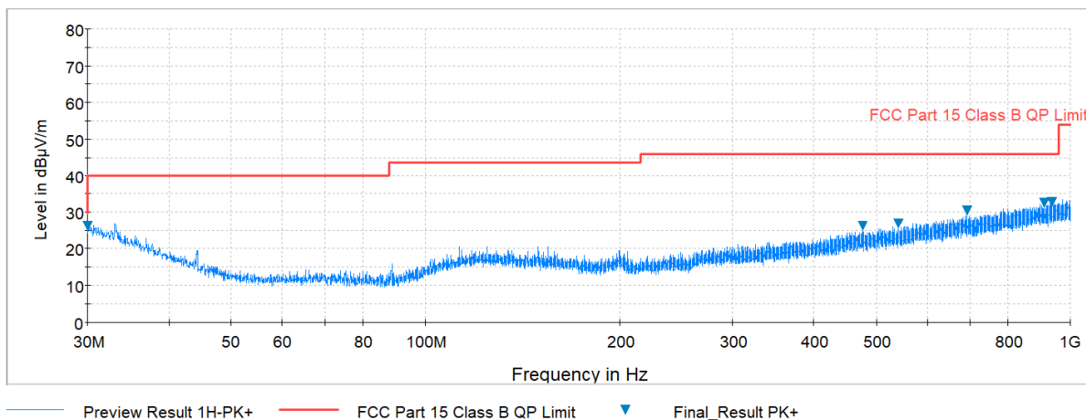
Plot 7-55. Radiated Spurious Plot below 1GHz (Pol. V)
