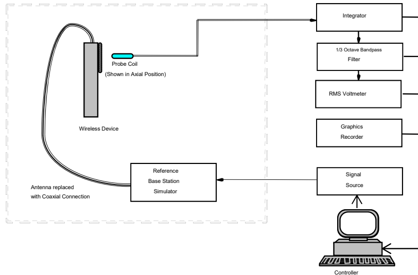
Figure 4-12 Audio Magnetic Field Test Setup
