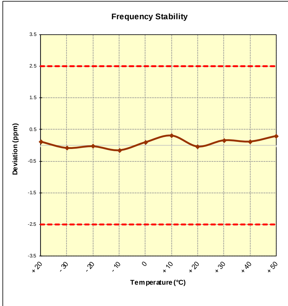
Figure 7-13. Frequency Stability Graph (Band 5/26)
