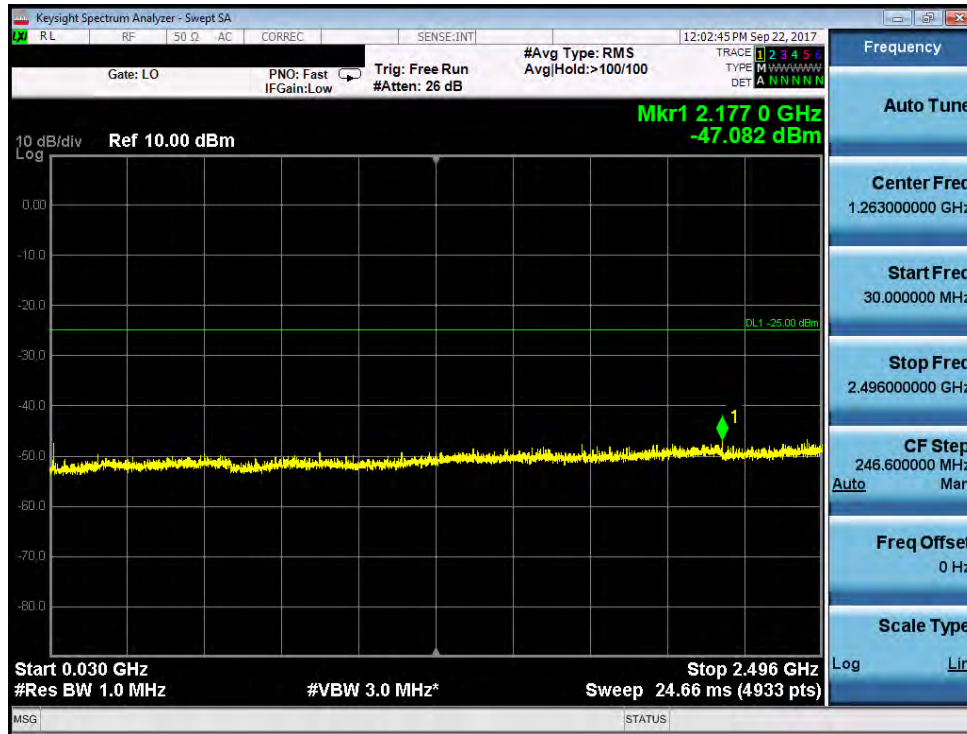
Plot 7-310. Conducted Spurious Plot (Band 41 – 20.0MHz QPSK – PCC 1/99 SCC 1/0 – Mid Channel)
