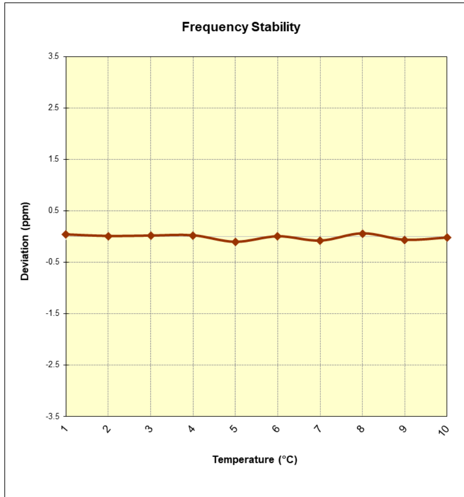
Figure 7-17. Frequency Stability Graph (Band 38/41)
