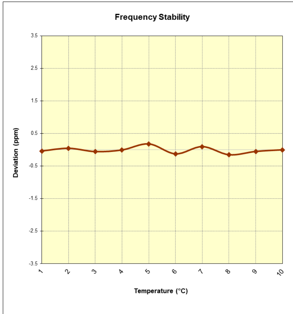
Figure 7-14. Frequency Stability Graph (Band 4/66)
