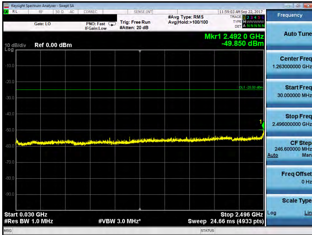
Plot 7-314. Conducted Spurious Plot (Band 41 – 20.0MHz QPSK – PCC 100/0 SCC 100/0 – Mid Channel)
