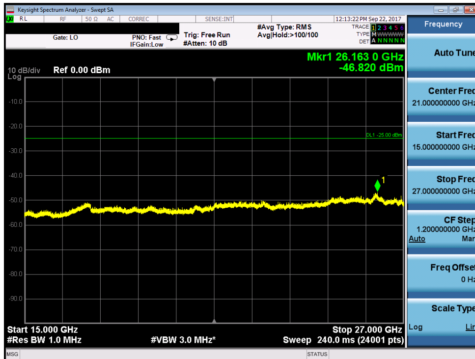
Plot 7-313. Conducted Spurious Plot (Band 41 – 20.0MHz QPSK – PCC 1/99 SCC 1/0 – Mid Channel)
