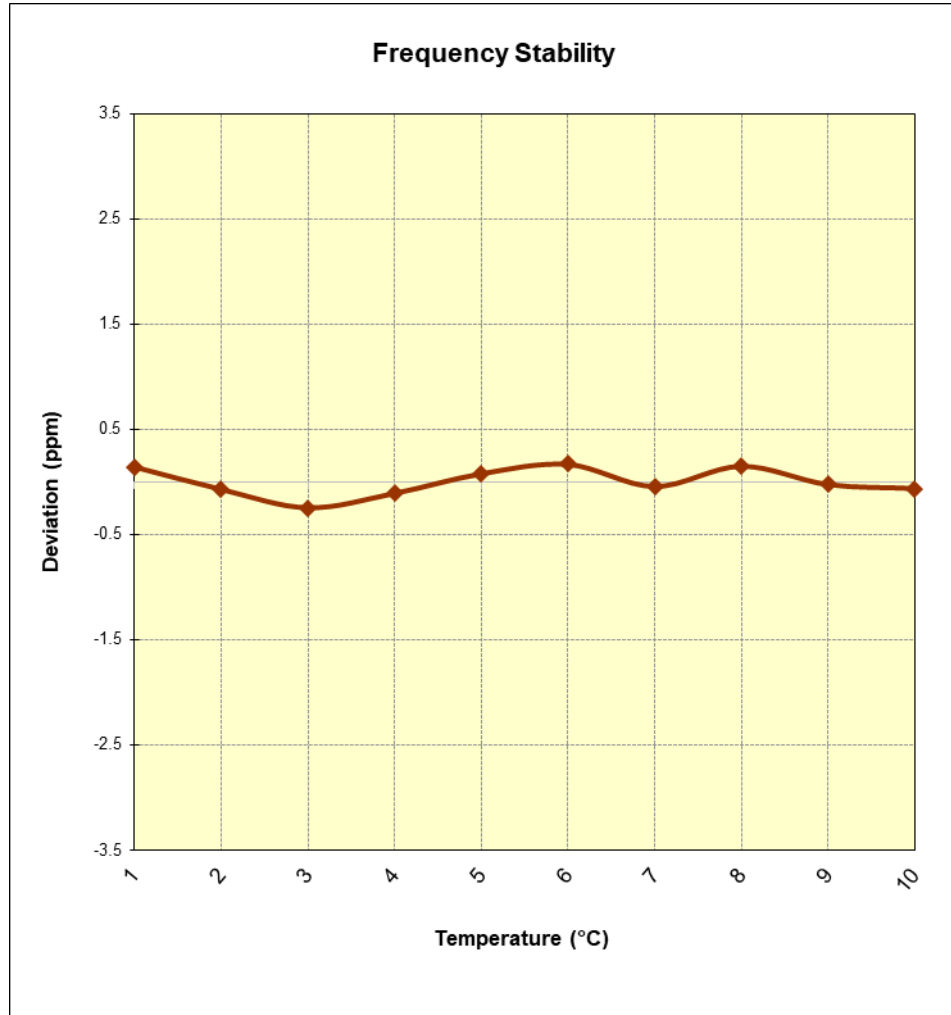
Figure 7-15. Frequency Stability Graph (Band 2/25)
