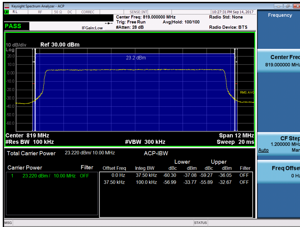
Plot 7-34. Channel Edge Plot (10MHz QPSK – RB Size 50)
