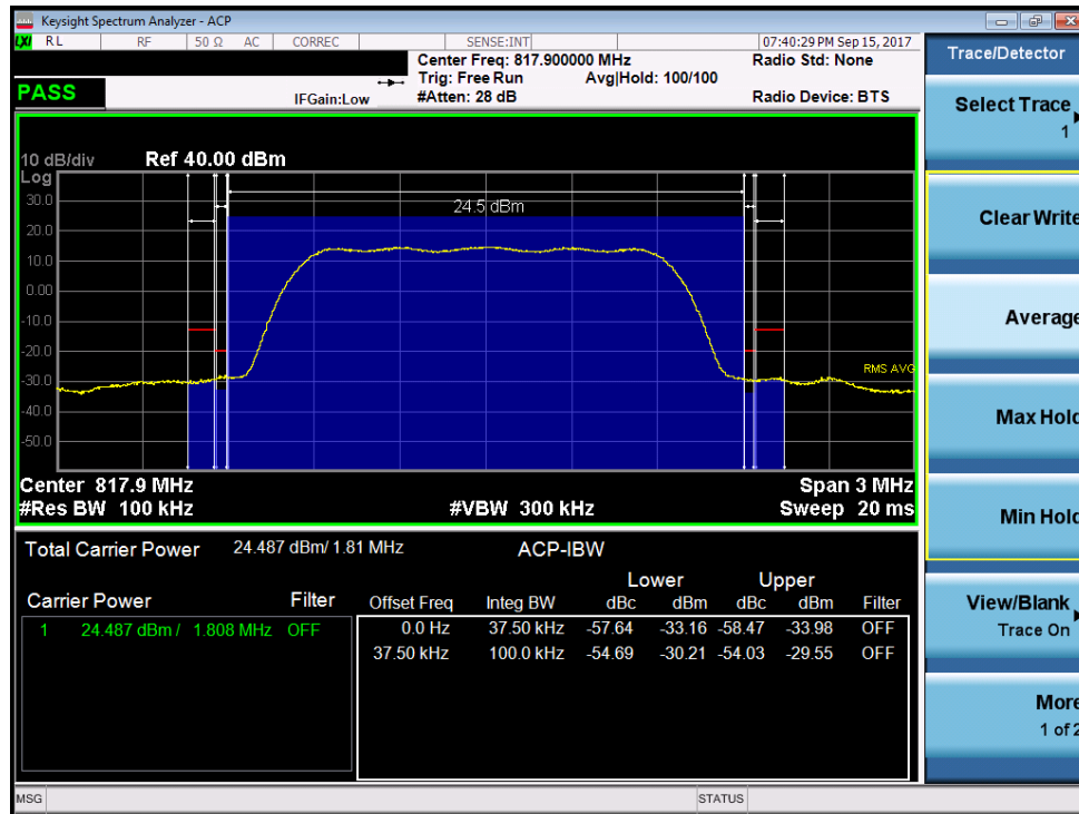
Plot 7-26. Channel Edge Plot (Ch. 476)
