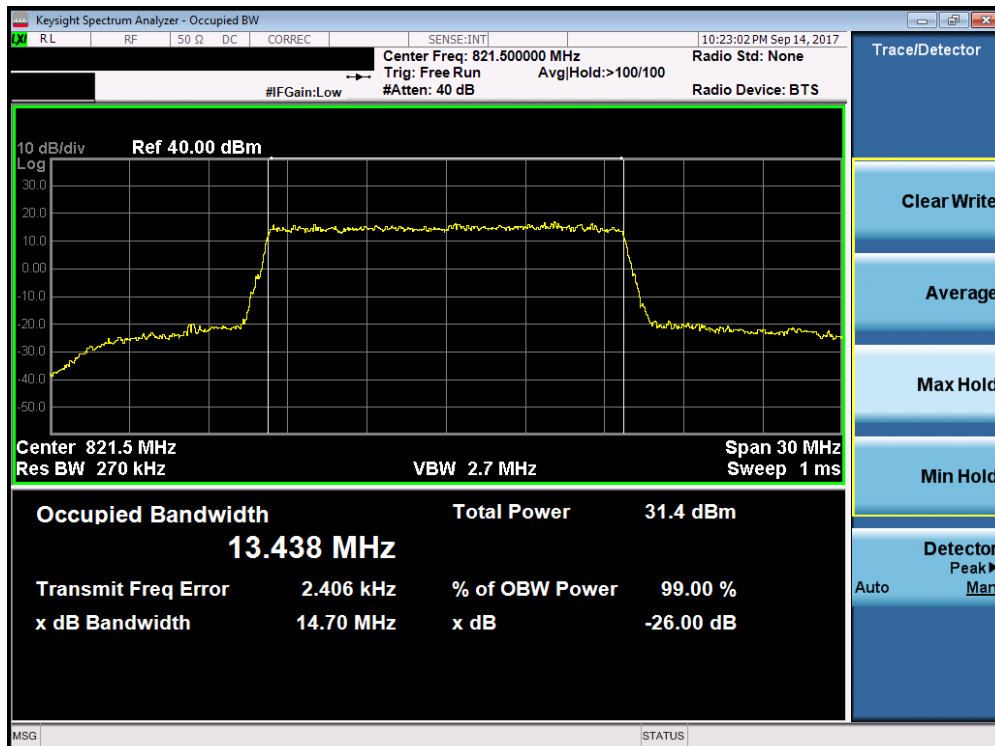
Plot 7-16. Occupied Bandwidth Plot (15MHz 16-QAM – RB Size 75)
