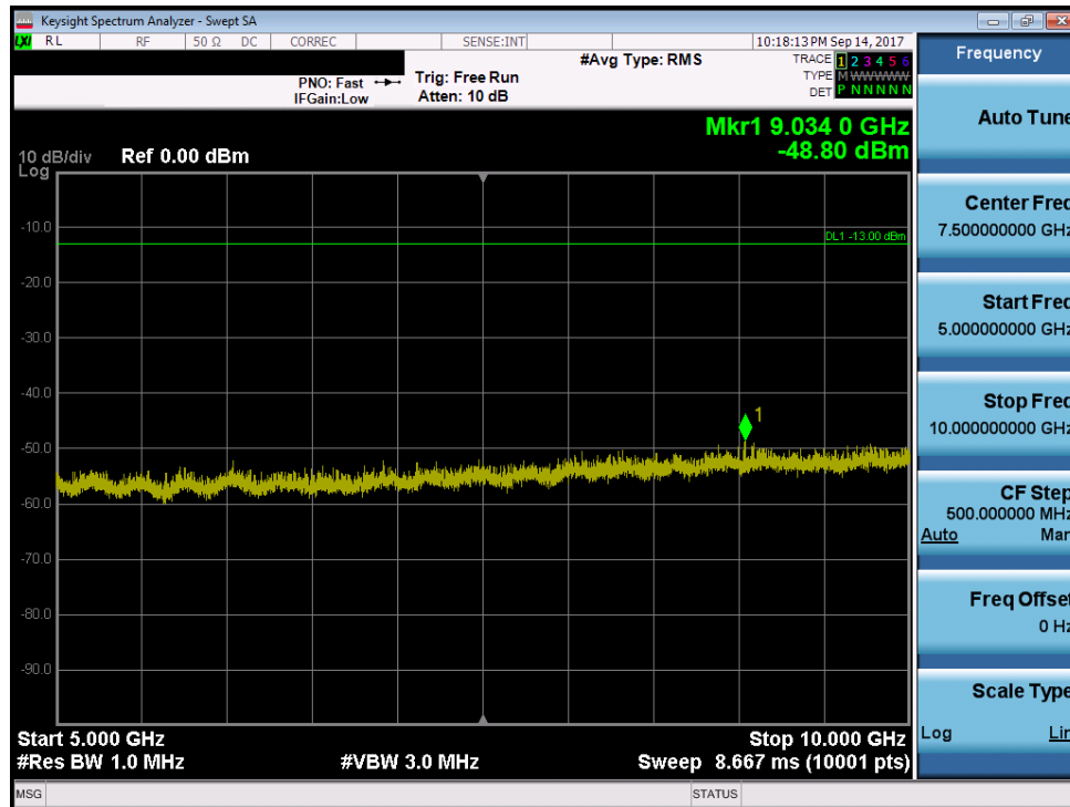
Plot 7-25. Conducted Spurious Plot (5 MHz QPSK – RB Size 1, RB Offset 0 – High Channel)
