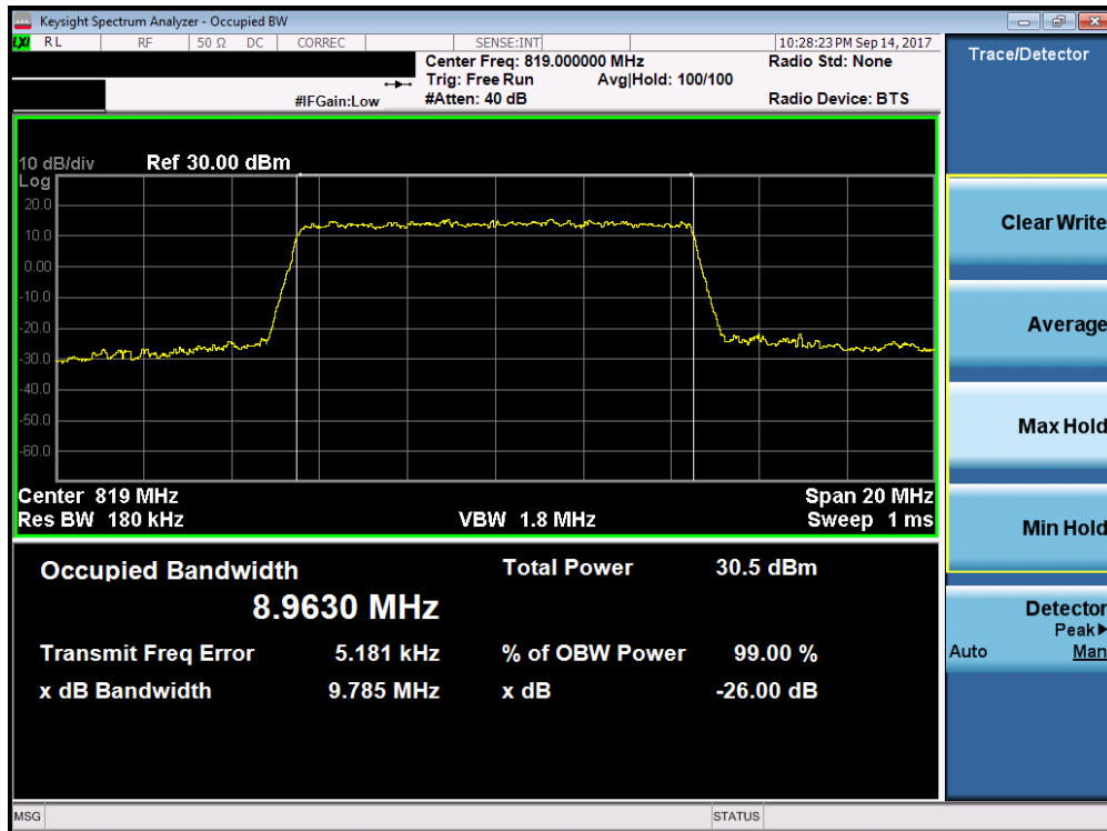
Plot 7-14. Occupied Bandwidth Plot (10MHz 64-QAM – RB Size 50)
