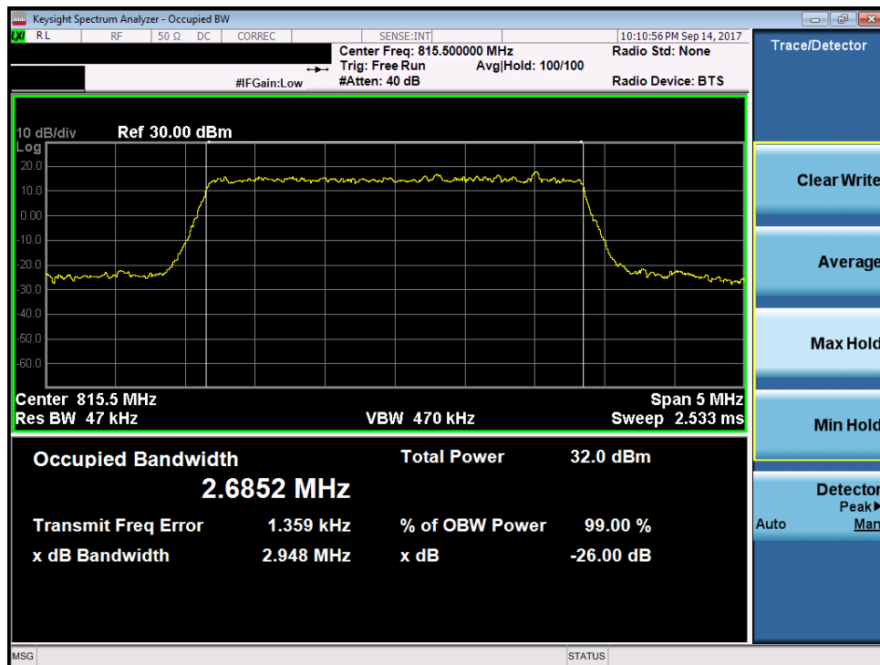
Plot 7-6. Occupied Bandwidth Plot (3MHz QPSK – RB Size 15– Low Channel)
