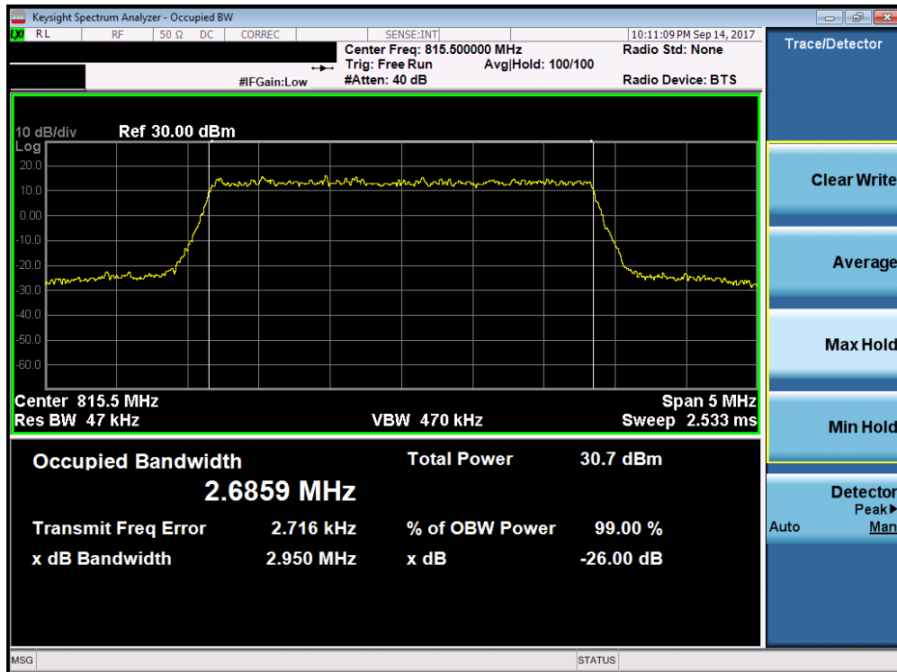
Plot 7-7. Occupied Bandwidth Plot (3MHz 16-QAM – RB Size 15– Low Channel)
