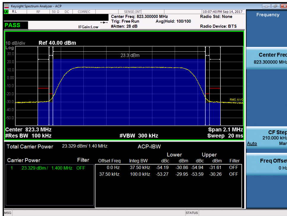
Plot 7-29. Channel Edge Plot (1.4MHz QPSK – RB Size 6 – High Channel)
