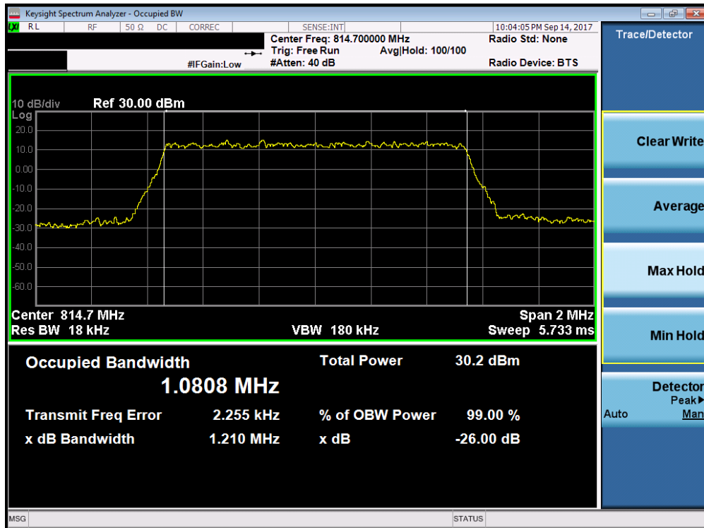
Plot 7-5. Occupied Bandwidth Plot (1.4MHz 64-QAM – RB Size 6– Low Channel)
