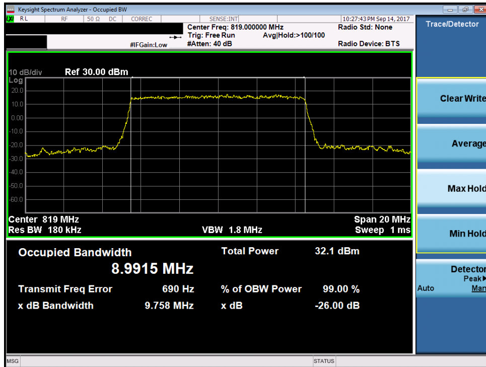
Plot 7-12. Occupied Bandwidth Plot (10MHz QPSK – RB Size 50)
