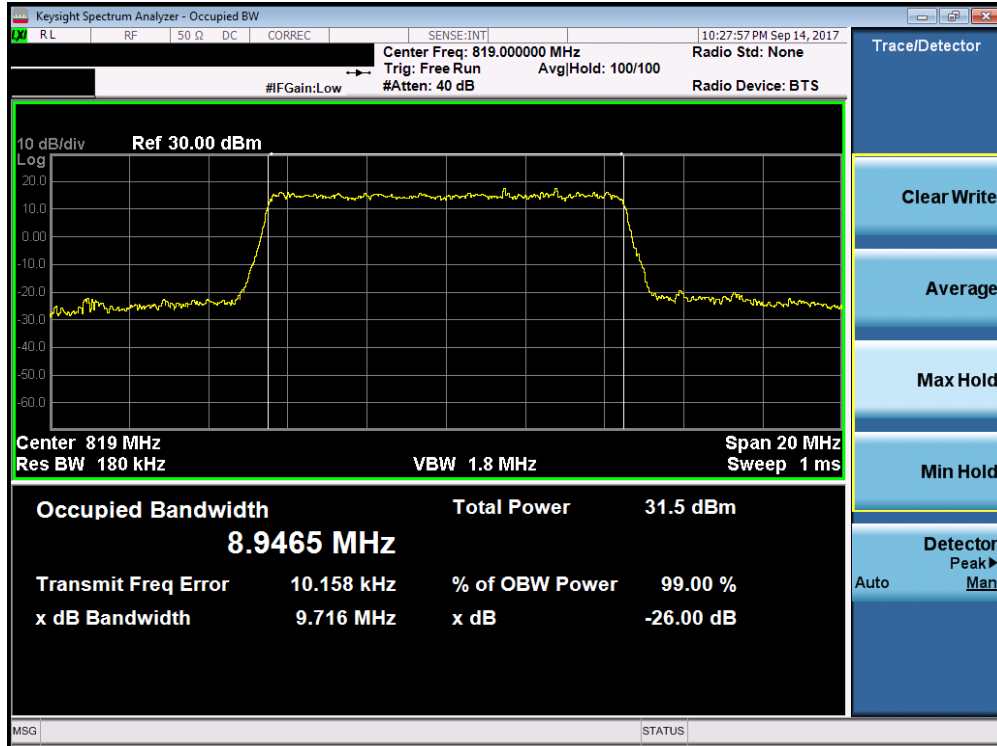
Plot 7-13. Occupied Bandwidth Plot (10MHz 16-QAM – RB Size 50)
