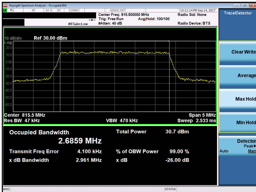
Plot 7-8. Occupied Bandwidth Plot (3MHz 64-QAM – RB Size 15– Low Channel)
