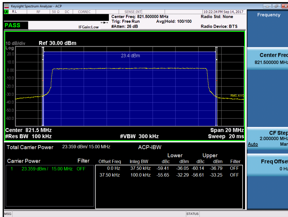
Plot 7-35. Channel Edge Plot (15MHz QPSK – RB Size 75)
