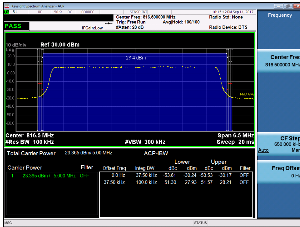
Plot 7-32. Channel Edge Plot (5MHz QPSK – RB Size 25– Low Channel)
