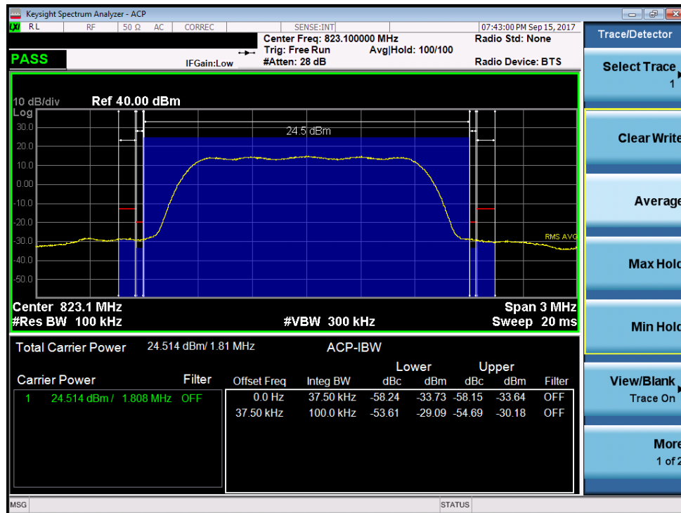
Plot 7-27. Channel Edge Plot (Ch. 684)
