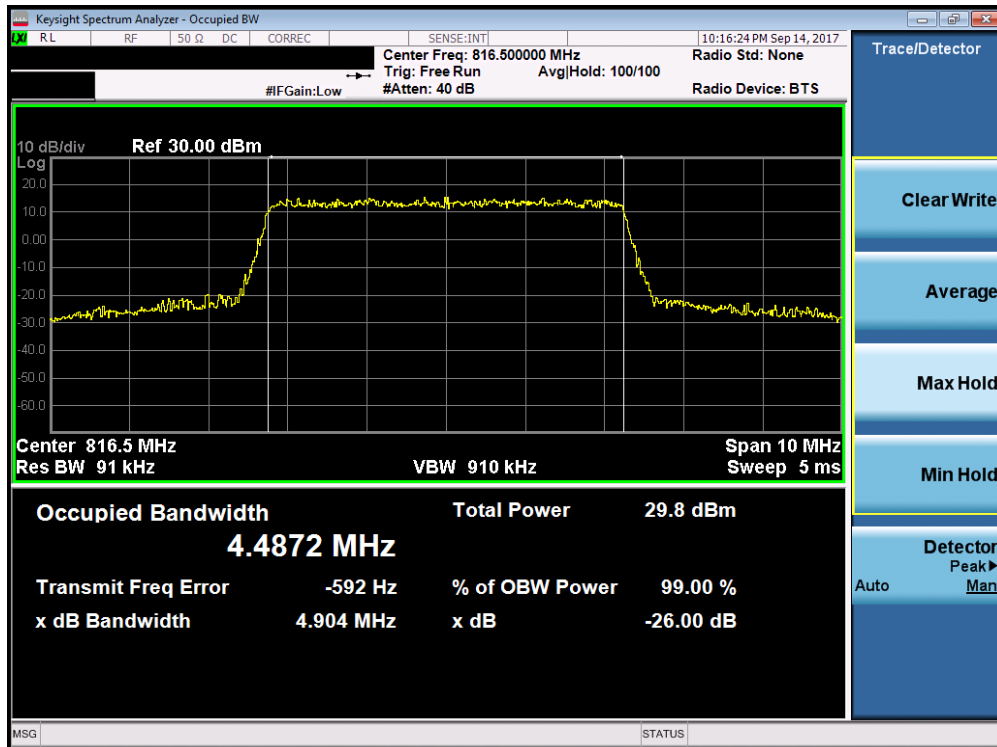
Plot 7-11. Occupied Bandwidth Plot (5MHz 64-QAM – RB Size 25– Low Channel)
