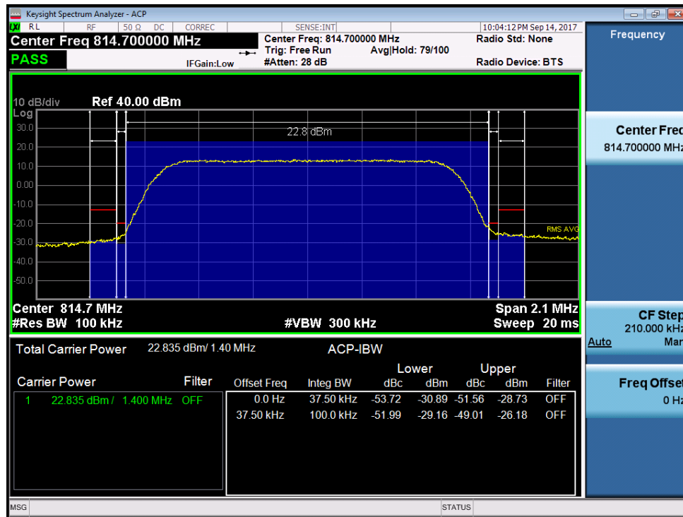
Plot 7-28. Channel Edge Plot (1.4MHz QPSK – RB Size 6– Low Channel)
