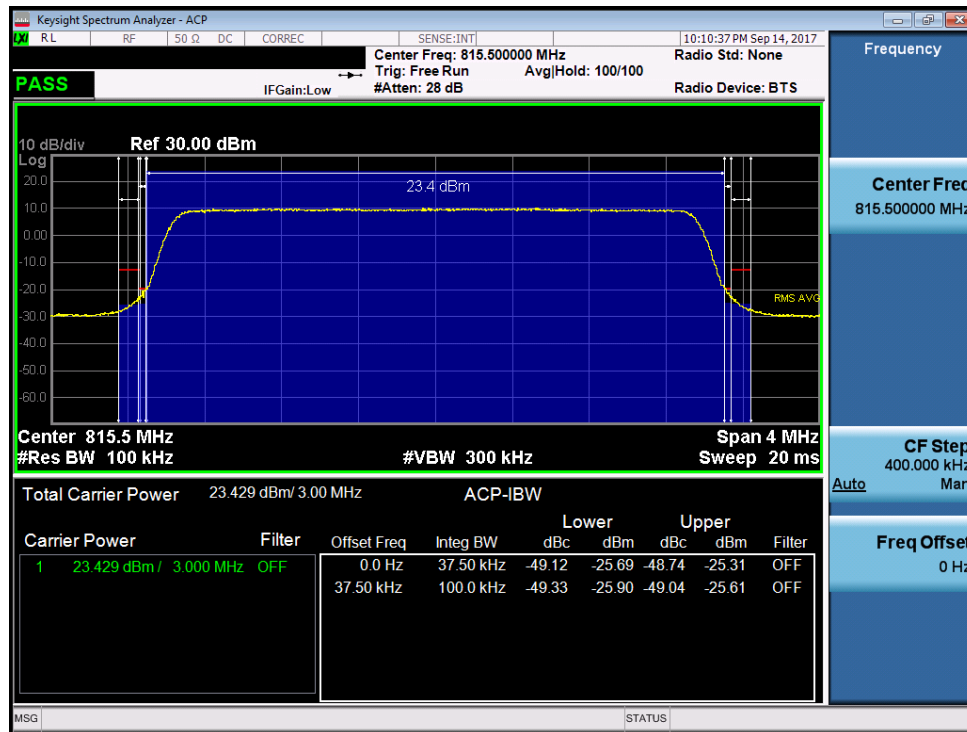
Plot 7-30. Channel Edge Plot (3MHz QPSK – RB Size 15– Low Channel)
