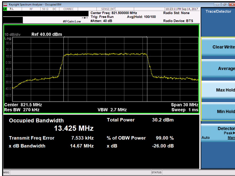
Plot 7-17. Occupied Bandwidth Plot (15MHz 64-QAM – RB Size 75)
