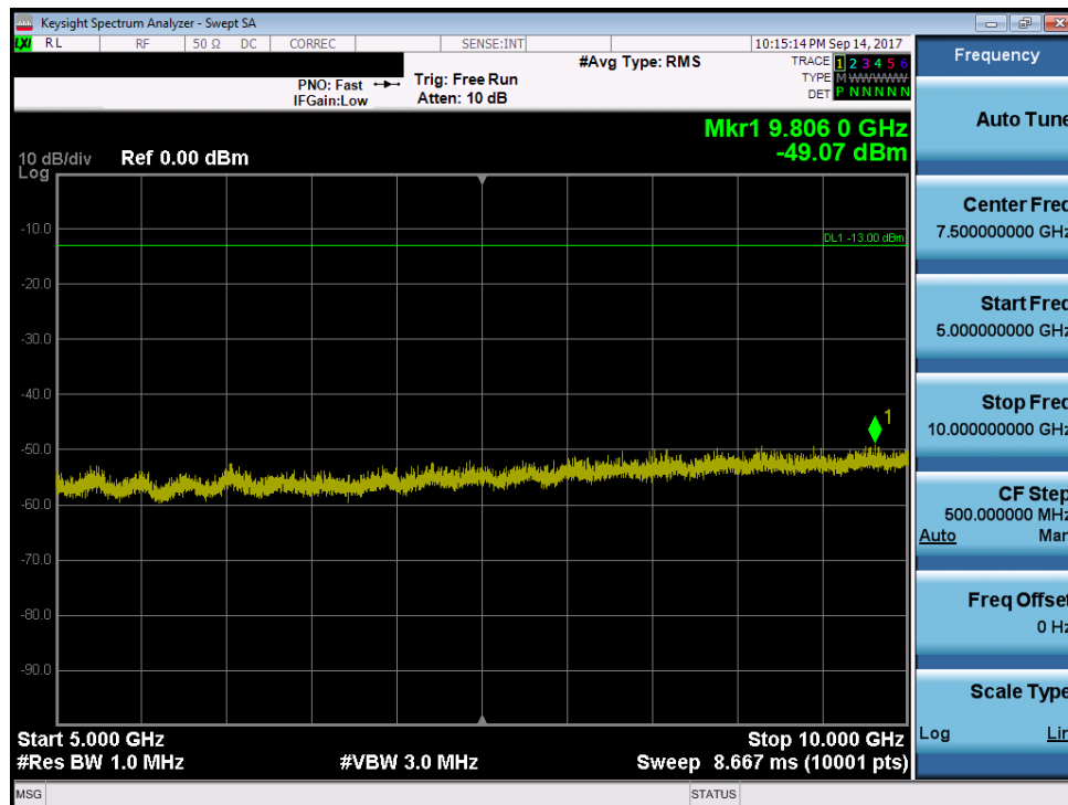
Plot 7-23. Conducted Spurious Plot (5 MHz QPSK – RB Size 1, RB Offset 0 – Low Channel)
