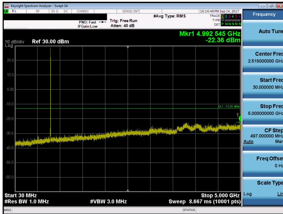
Plot 7-22. Conducted Spurious Plot (5 MHz QPSK – RB Size 1, RB Offset 0 – Low Channel)
