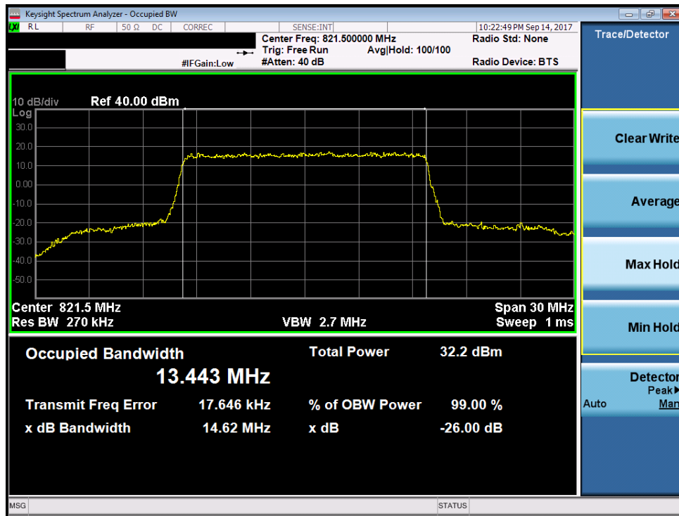
Plot 7-15. Occupied Bandwidth Plot (15MHz QPSK – RB Size 75)
