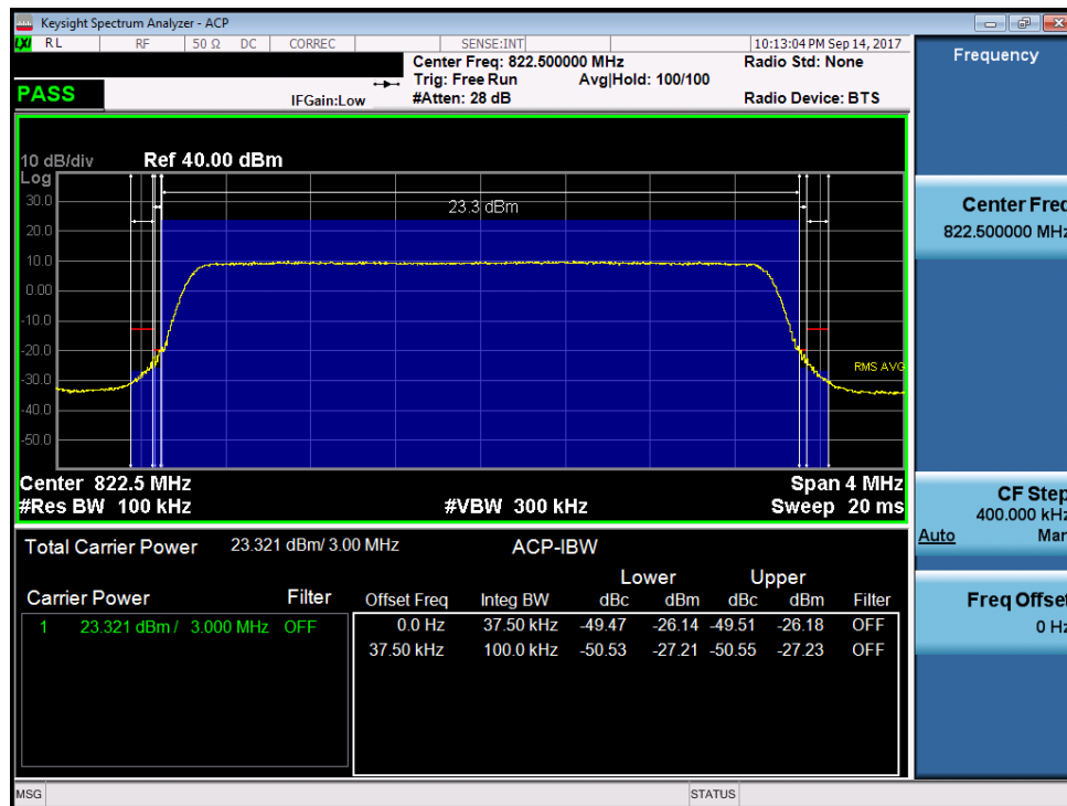
Plot 7-31. Channel Edge Plot (3MHz QPSK – RB Size 15 – High Channel)
