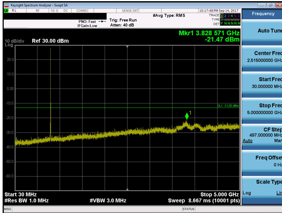
Plot 7-24. Conducted Spurious Plot (5 MHz QPSK – RB Size 1, RB Offset 0 – High Channel)
