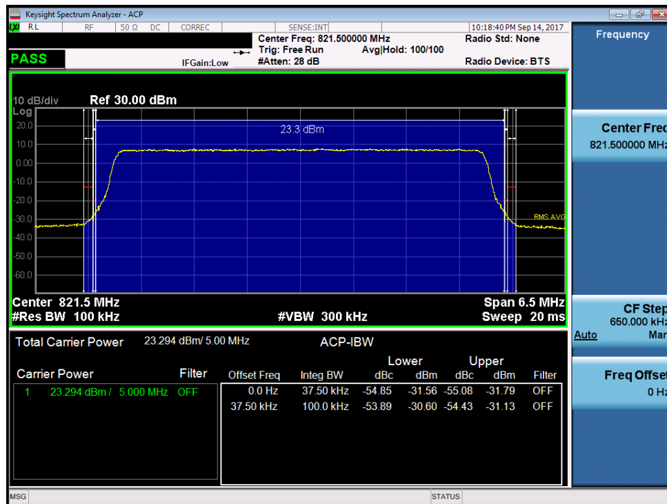
Plot 7-33. Channel Edge Plot (5MHz QPSK – RB Size 25 – High Channel)
