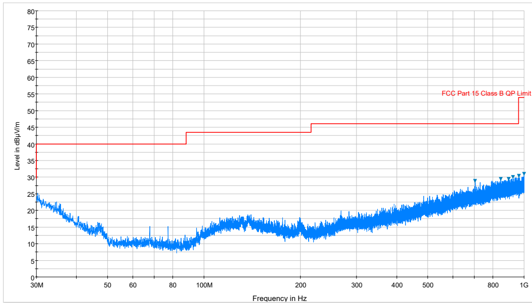
Plot 7-3. Radiated Spurious Plot 30MHz – 1GHz (Pol. H)
