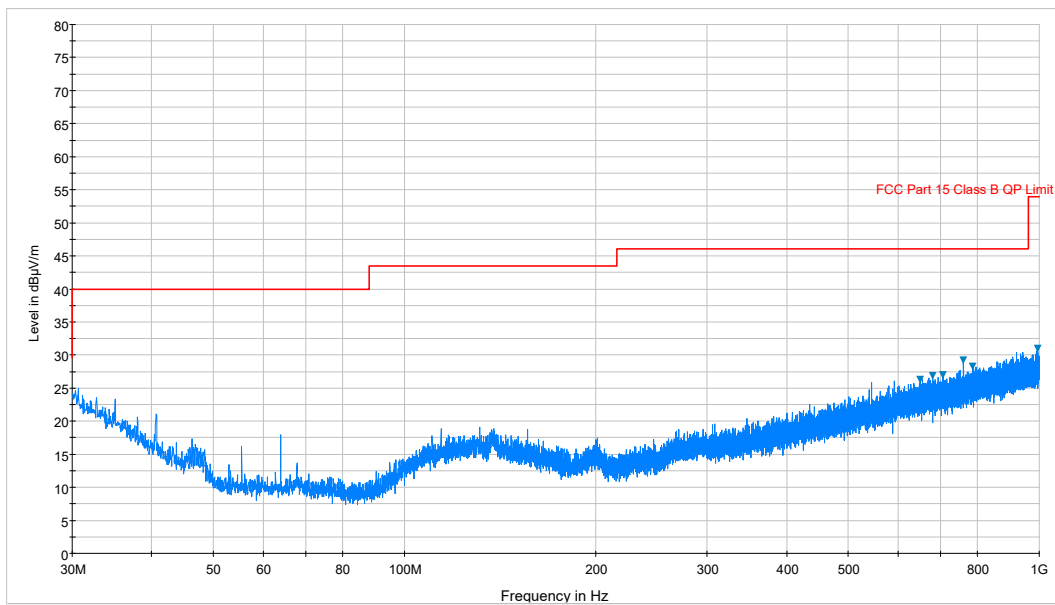
Plot 7-4. Radiated Spurious Plot 30MHz – 1GHz (Pol. V)
