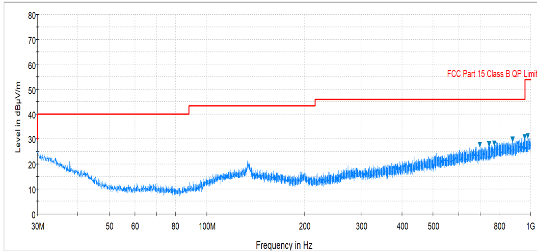
Plot 7-117. Radiated Spurious Plot below 1GHz (Pol. H)
