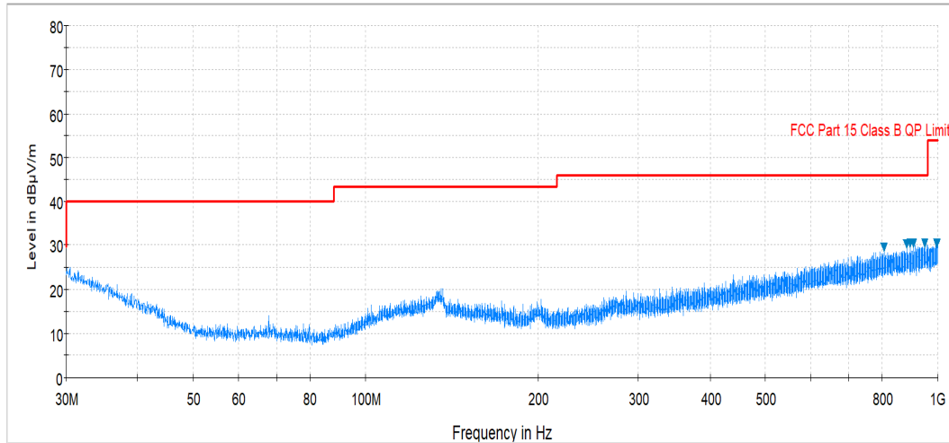
Plot 7-115. Radiated Spurious Plot below 1GHz (Pol. H)
