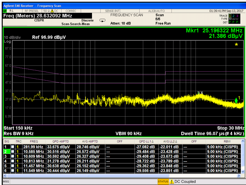
Plot 7-120. Line Conducted Plot with 802.11b (N)
