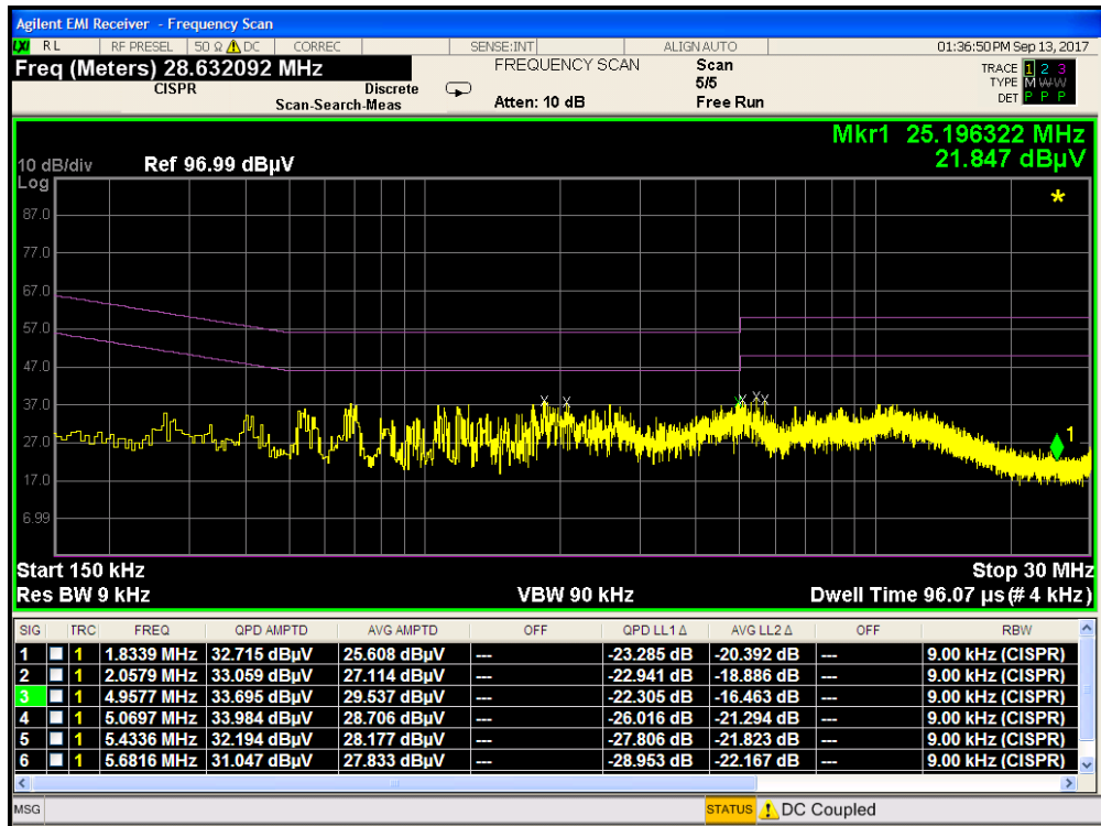
Plot 7-119. Line Conducted Plot with 802.11b (L1)
