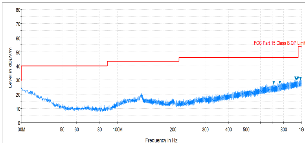
Plot 7-116. Radiated Spurious Plot below 1GHz (Pol. V)
