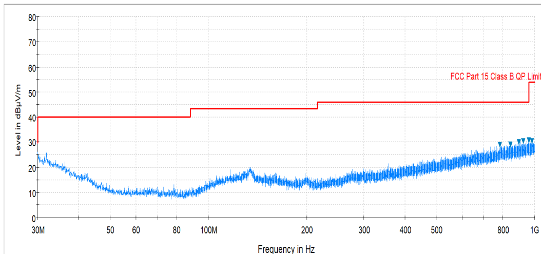
Plot 7-118. Radiated Spurious Plot below 1GHz (Pol. V)
