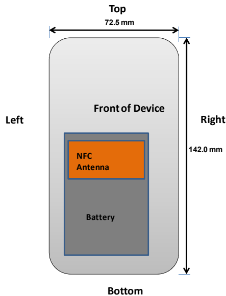
Figure 1-2 NFC Antenna Locations
